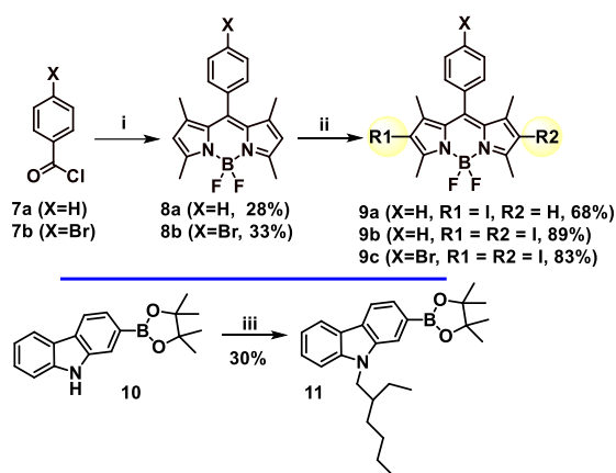
Scheme 3. Reaction conditions: i) 2,4-dimethylpyrrole, \text{CH}_2\text{Cl}_2 , r.t., 16 h, \text{Et}_3\text{N} , \text{BF}_3 \cdot \text{Et}_2\text{O} , 2h; ii) NIS, \text{CH}_2\text{Cl}_2 , r.t., 30 min; iii) \text{Cs}_2\text{CO}_3 , 2-ethylhexyl bromide, 60 °C, 48 h.
