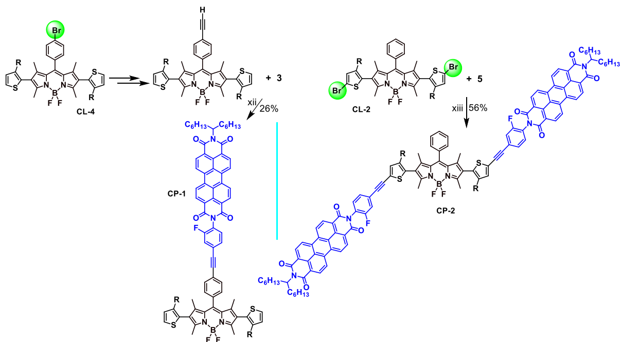
Scheme 6. Reaction conditions: xii) \text{Pd}(\text{PPh}_3)_2\text{Cl}_2 (10% mol), \text{CuI} (5% mol), DMF, \text{Et}_3\text{N} , 80 °C, 4 h; xiii) NBS, \text{CH}_2\text{Cl}_2 , r.t.
