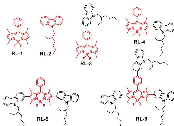
Chart 2. BODIPYs as core and functionalized with carbazole in diverse positions.
