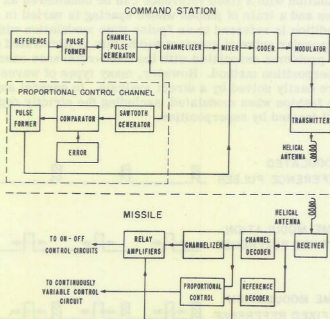
Fig. 1: A Typical Command Control System
