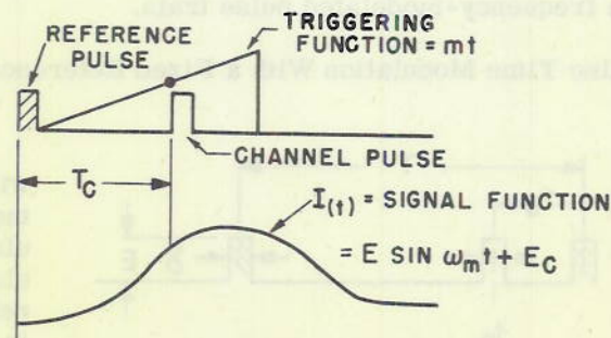
Fig. 4: Proportion Control Channel Pulse Generation.
