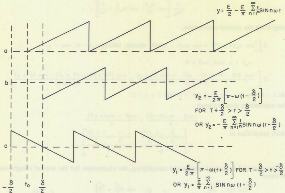
Fig. 16: Sawtooth Wave Components
