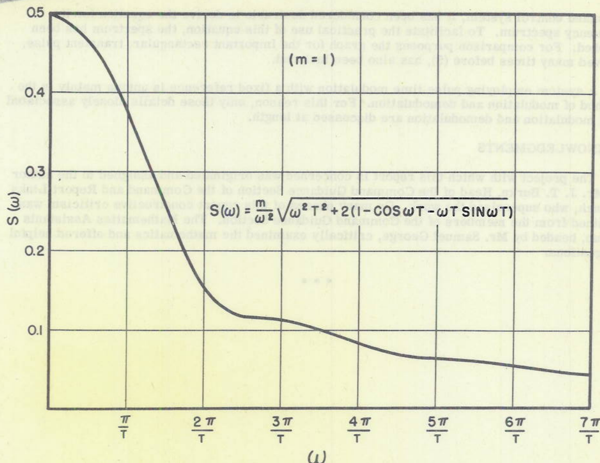
Fig. 11: The Spectrum for a Single Sawtooth Pulse
