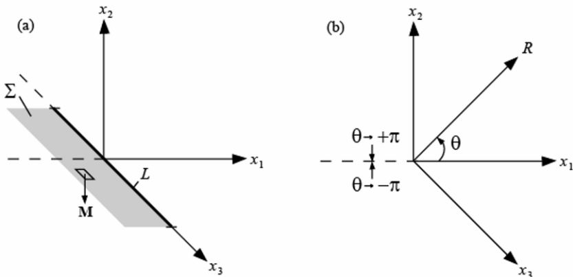
Fig. C.1 Cartesian coordinate system (a) and cylindrical coordinate system (b)
