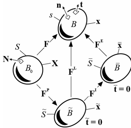
Fig. 7.1 Configurations, surface coordinates and tractions, and tangent maps
