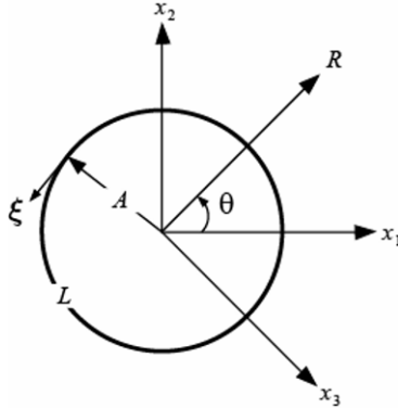
Fig. C.3 Defect loop and cylindrical and Cartesian coordinate systems
