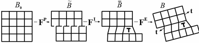
Fig. 3.11 Volume element of cubic crystal containing a single edge dislocation
