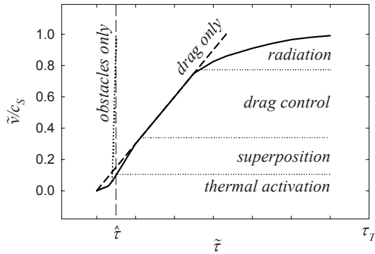
Fig. 6.1 Dislocation velocity-shear stress diagram (Kocks et al. 1975)
