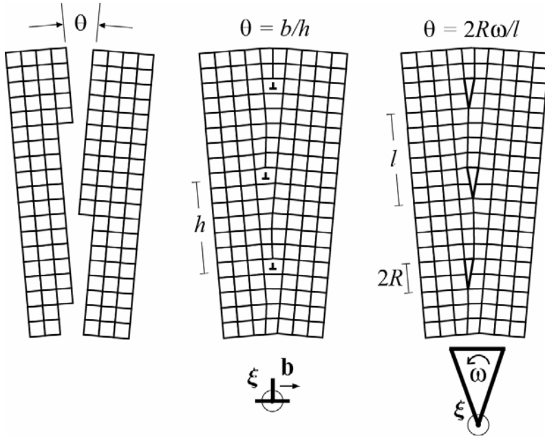
Fig. 3.16 Tilt boundary (left) comprised of edge dislocations (center) or partial disclination dipoles (right)
