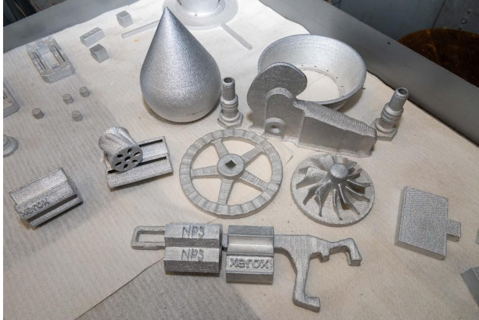
Figure 9. Aluminum Parts Printed at Naval Postgraduate School on the Xerox ElemX printer. Source: Martin (2023).
