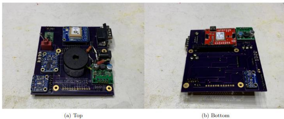
Fig. 1 — SHABHat, custom printed PCB daughterboard for Raspberry Pi with COTS sensors, voltage regulators, and additional parts for autonomous SHAB flights
