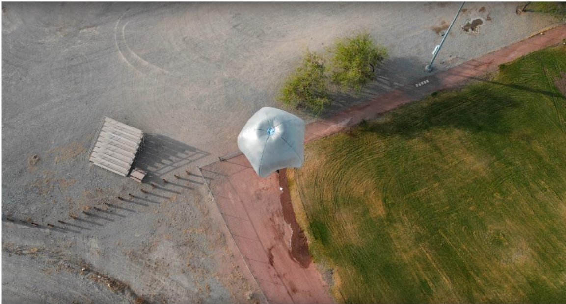
Fig. 3 — Aerial photo of a vented SHAB flight in Tucson with a Styrofoam (EPS) vent mounted to the top of the balloon
