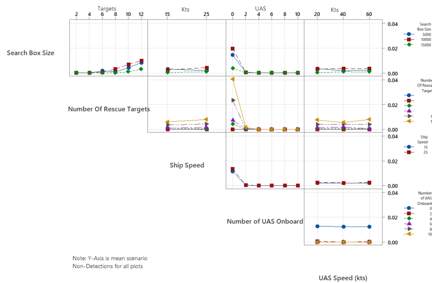
y-axis is mean scenario non-detections. The plot is sectioned by pairs of mutually varied inputs. The variable notated to the left of a given box is stylized by color and shape, each of which represents the varied value (depicted to the right of the plots). The variable notated to the bottom of a given box is varied according to the numbers that line the top of the box (i.e., “Targets” is varied by 2, 4, 6, 8, 10, and 12). This graph represents the change in average scenario non-detections with changes in the paired inputs. Figure 36. ISR Detect and Confirm Interaction Plot for Mean Scenario Non-detections
