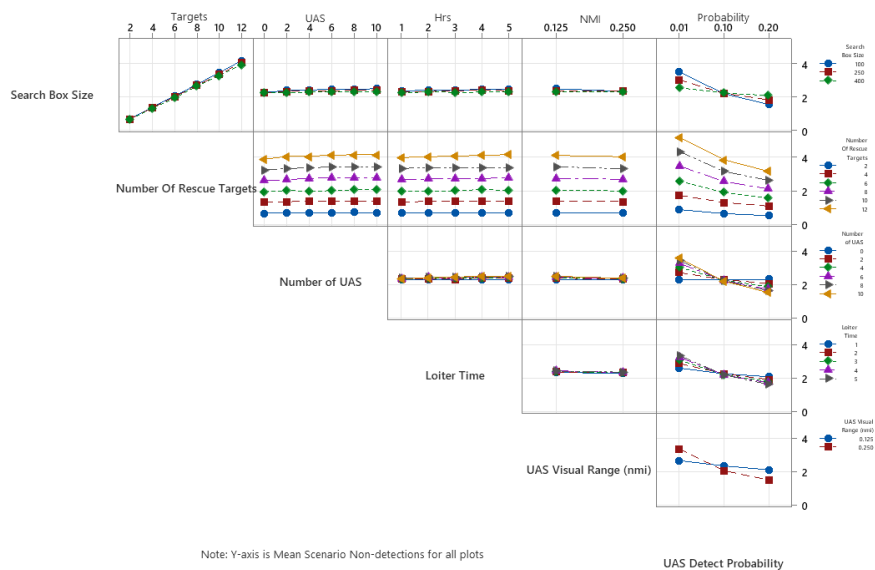
y-axis is mean scenario non-detections. The plot is sectioned by pairs of mutually varied inputs. The variable notated to the left of a given box is stylized by color and shape, each of which represents the varied value (depicted to the right of the plots). The variable notated to the bottom of a given box is varied according to the numbers that line the top of the box (i.e., “Targets” is varied by 2, 4, 6, 8, 10, and 12). This graph represents the change in average scenario non-detections with changes in the paired inputs.
