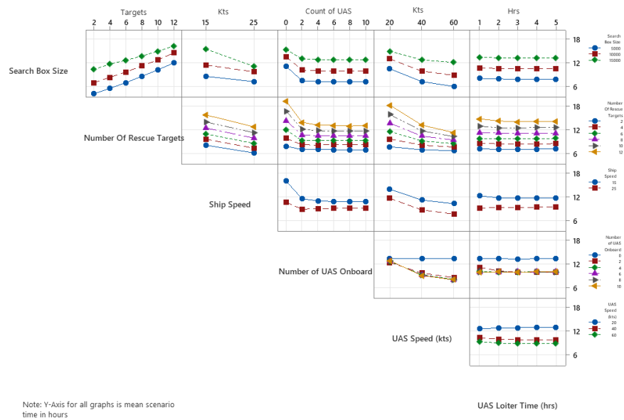
Figure 34. ISR Detect and Confirm Interaction Plot for Mean Scenario Time in Hours
