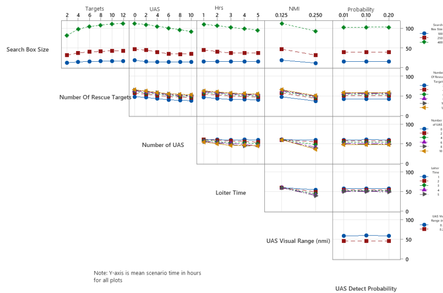
y-axis is mean scenario time. The plot is sectioned by pairs of mutually varied inputs. The variable notated to the left of a given box is stylized by color and shape, each of which represents the varied value (depicted to the right of the plots). The variable notated to the bottom of a given box is varied according to the numbers that line the top of the box (i.e., “Targets” is varied by 2, 4, 6, 8, 10, and 12). This graph represents the change in average scenario time with changes in the paired inputs. Figure 39. SAR Decrease Time Interactions Plot for Mean Scenario Time in Hours
