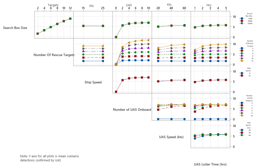
y-axis is mean scenario confirmations by UAS. The plot is sectioned by pairs of mutually varied inputs. The variable notated to the left of a given box is stylized by color and shape, each of which represents the varied value (depicted to the right of the plots). The variable notated to the bottom of a given box is varied according to the numbers that line the top of the box (i.e., “Targets” is varied by 2, 4, 6, 8, 10, and 12). This graph represents the change in average UAS confirmations with changes in the paired inputs. Figure 35. ISR Detect and Confirm Interaction Plot for Mean Scenario UAS Confirmations
