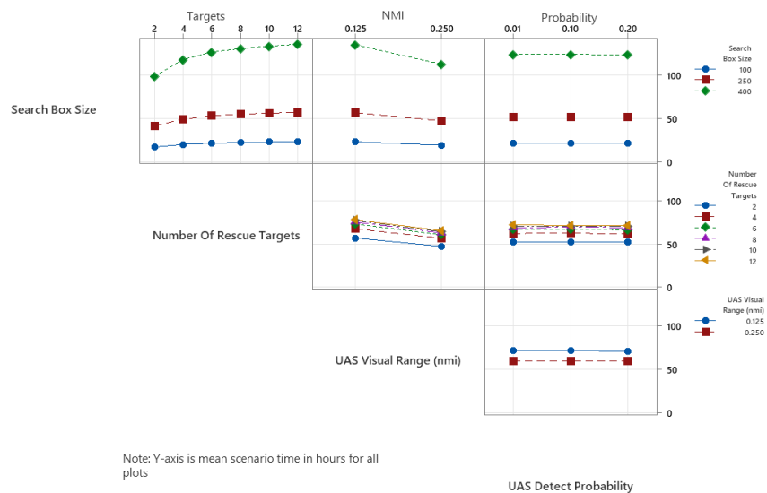
Figure 43. SAR Increase Detections Interaction Plot for Mean Scenario Time in Hours
