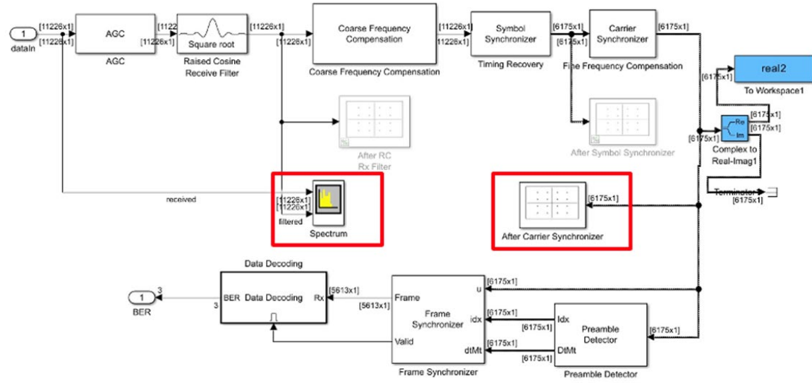
Figure 16. Receiver Block Diagram, I&Q Collection Points in Blue, Display Blocks in Red. Adapted from [37].
