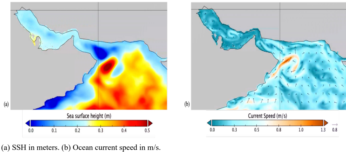
Figure 22. Ocean circulation patterns at 1200 UTC on August 8, 2002
