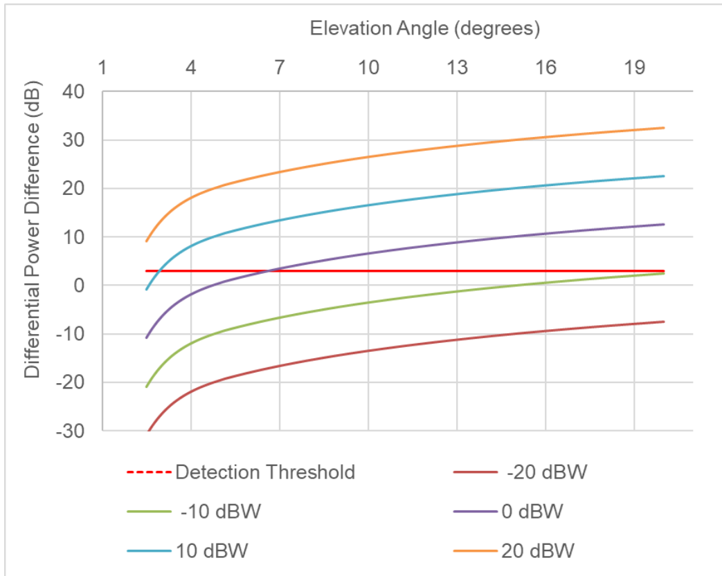
Figure 65. The power difference between attenuated and unattenuated received signal power from a meaconing attack transmitter.
