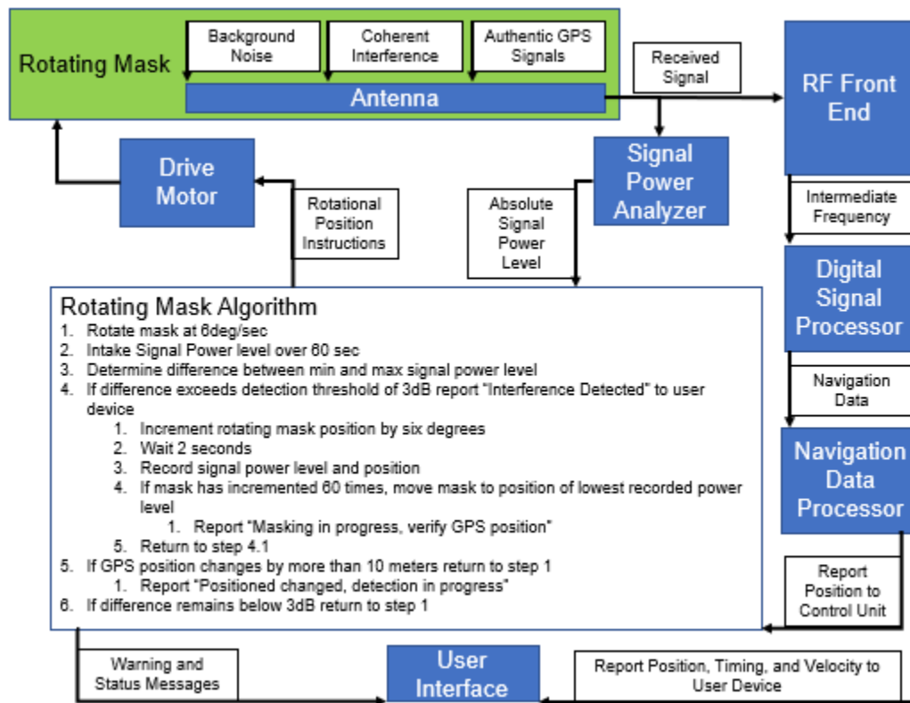
Figure 21. Rotating mask integration into a GPS receiver.
