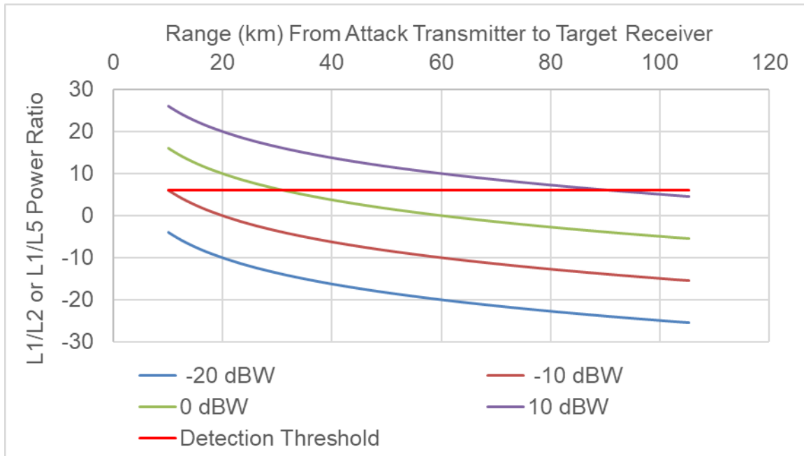
Figure 59. L1/L2 and L1/L5 power ratios from meaoning transmitters at different ranges.
