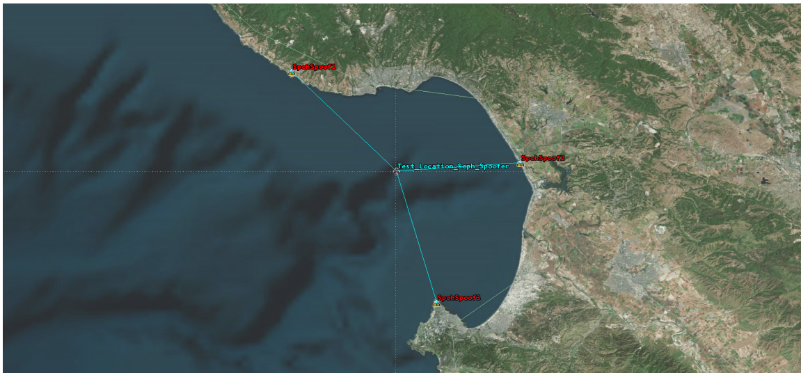
Figure 37. Sophisticated spoofer transmitter positions relative to a ship in Monterey Bay, CA, USA.
