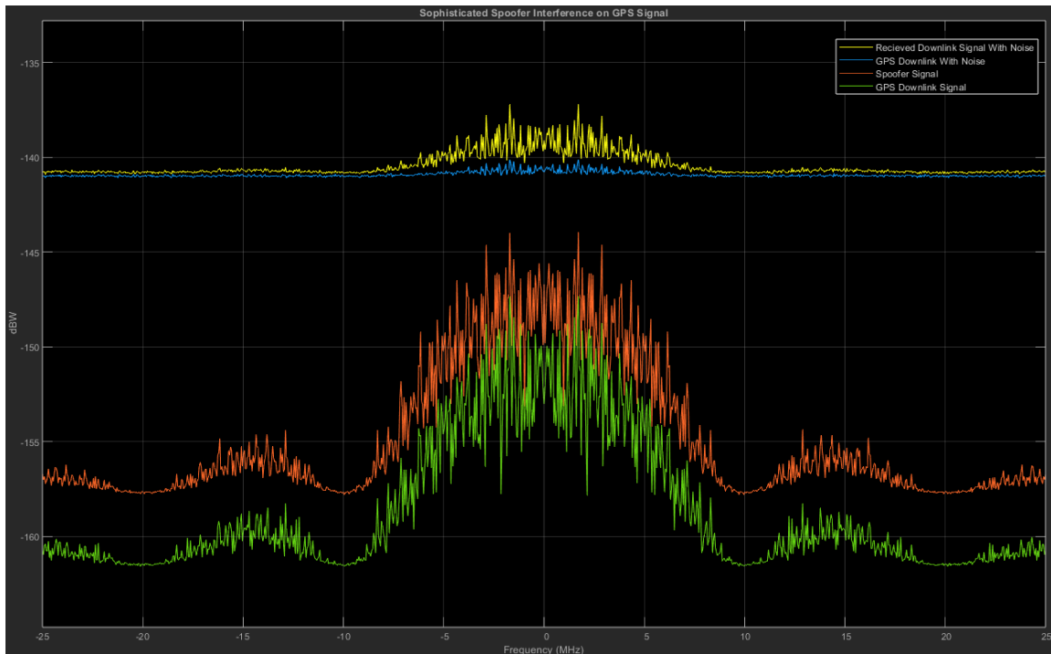
Figure 39. Spectrum analyzer of unmitigated sophisticated spoofing on a GPS receiver from three variable power transmitters at 16km, 21km and 23km.
