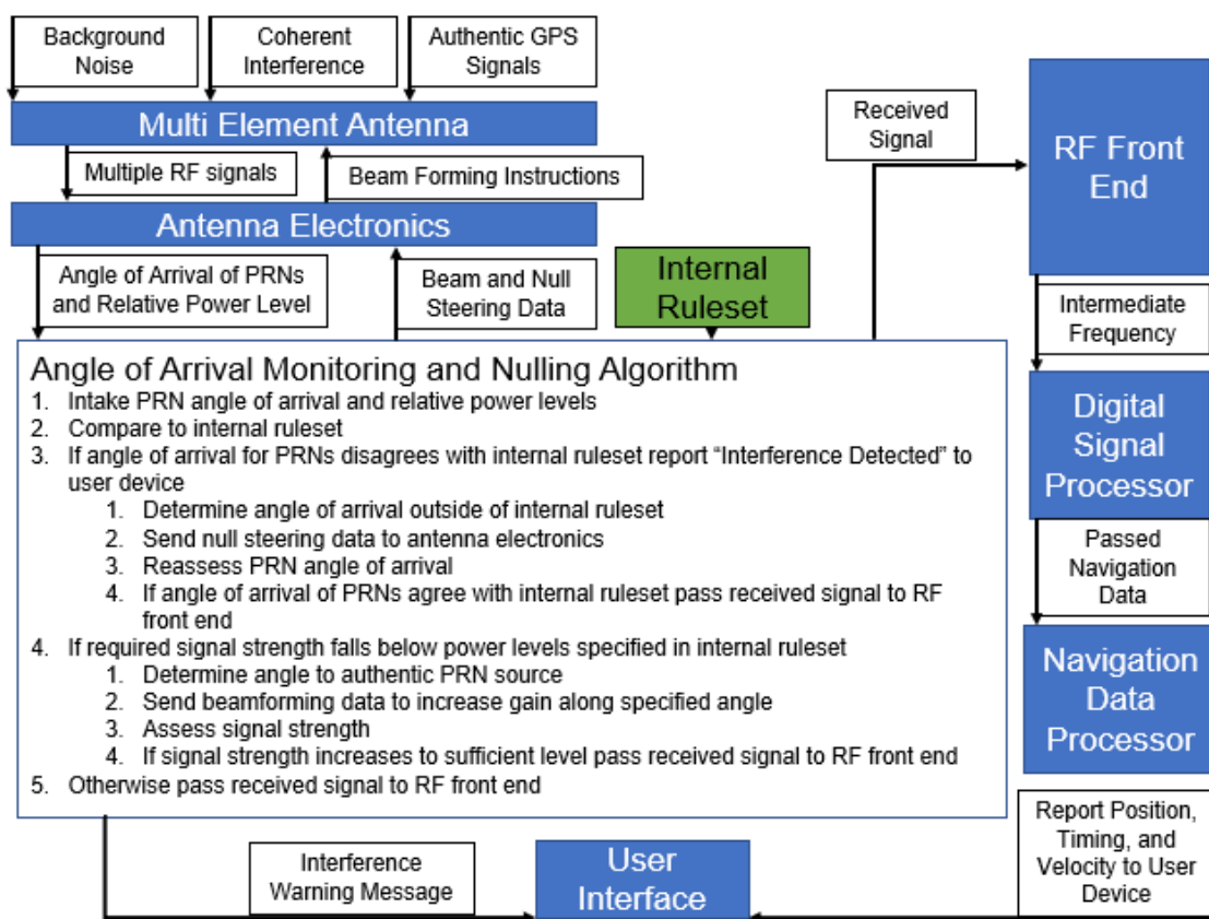
Figure 18. Angle of arrival monitoring and nulling integration into a GPS receiver.
