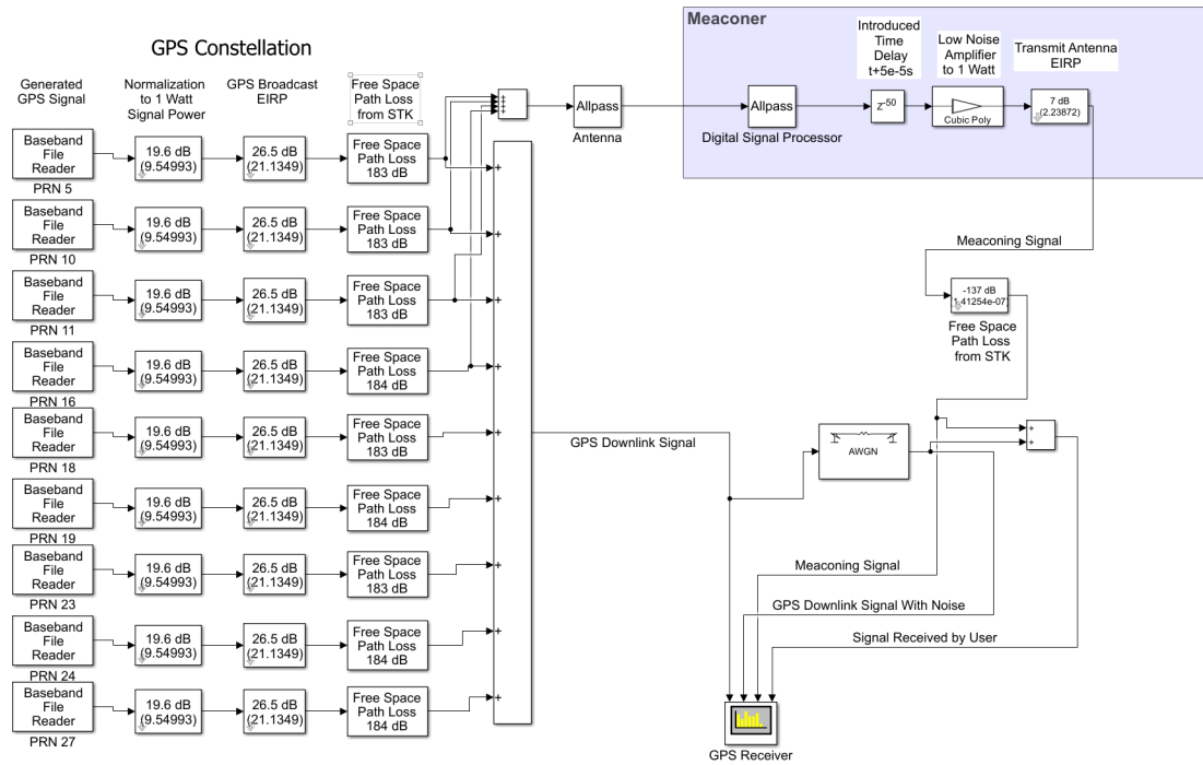
Figure 33. Attack scenario meaconing testing model.
