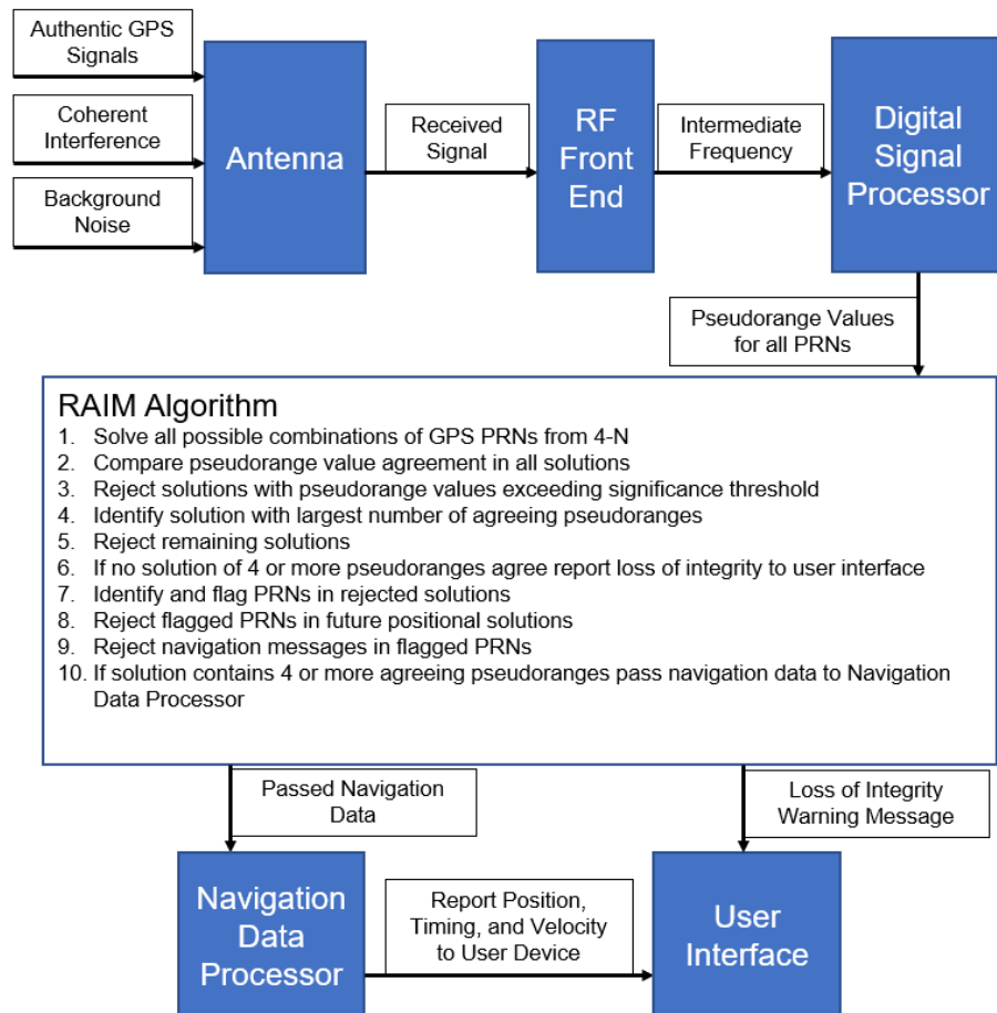
Figure 8. Modified RAIM integration into a GPS receiver.
