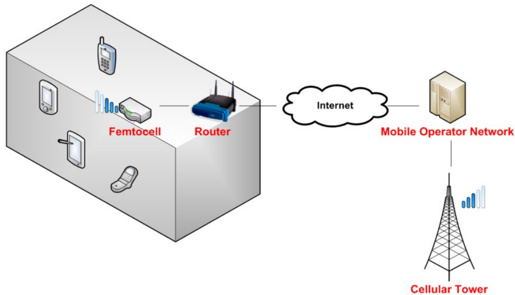
Figure 3. eFemto System Architecture Diagram. Source: Houngrinou (2010).
