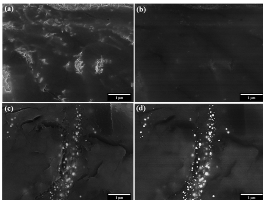
Figure 39. SEM imaging of 0.75 wt% CNT nanocomposites made from: untreated CNTs a) SE image, b) BSE image Eu:Y 2 O 3 -CNTs, c) SE image, and d) BSE image.
