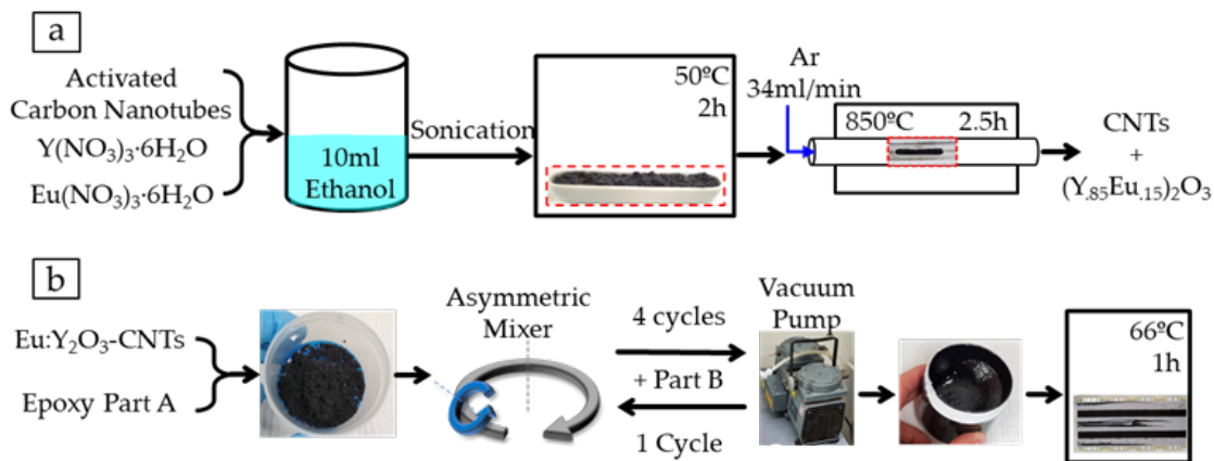
Figure 27. Depiction of the processes for a) synthesizing \text{Eu:Y}_2\text{O}_3 nanoparticles to CNT walls; b) fabrication of composite electrical boards and samples from epoxy and CNT pulp.
