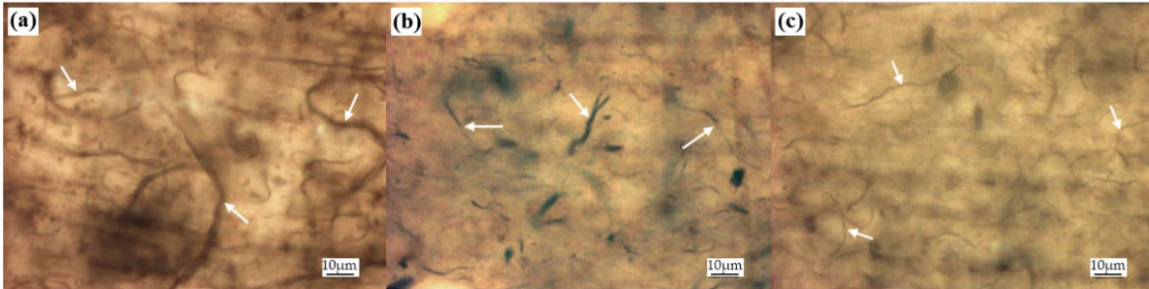
Figure 34. Magnification microscope 50X images revealing CNT bundles, indicated by white arrows, in nanocomposites created from: a) untreated CNT pulp, b) 2.5 h activated CNT pulp, and c) Eu:Y 2 O 3 -CNTs.
