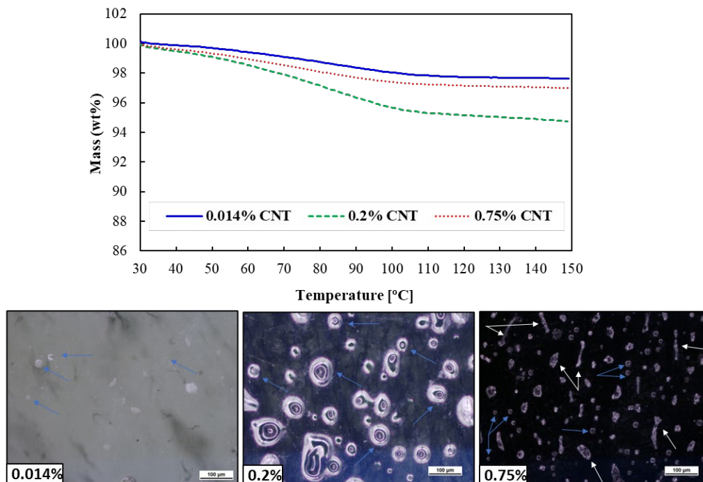
Figure 51. Top: TGA analysis of the 3 composites studied. Bottom: optical microscopy images illustrating differences in porosity.
