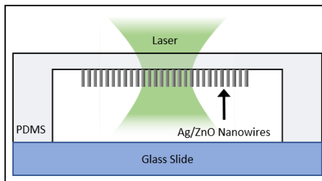
Figure III.1: Illustration of the cross-section of a microchannel integrated with an Ag/ZnO nanoprobe fabricated on the PDMS.
