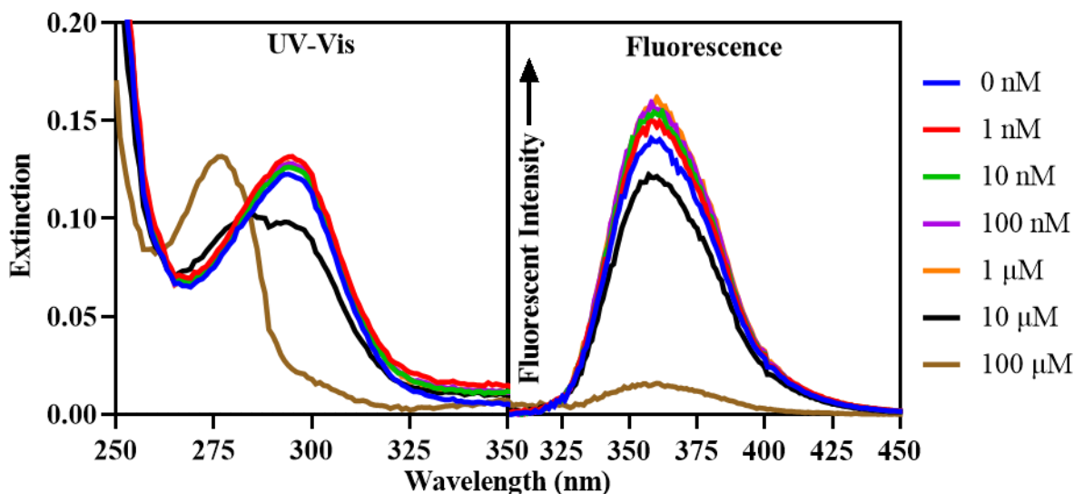
Figure IV.4: UV-Vis and fluorescence spectra of 100- \mu M AB18C6 with concentrations of Mo between 1 nM and 100 \mu M, with a control solution of 100- \mu M AB18C6 unmixed with Mo.
