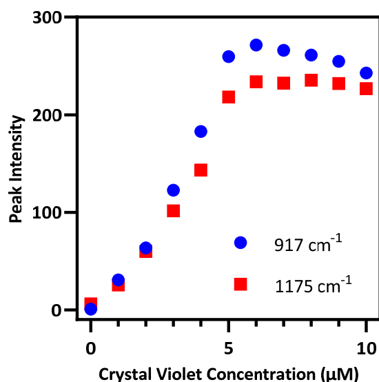
Figure S14: Intensity of two crystal violet peaks as a function of increasing crystal violet concentration
