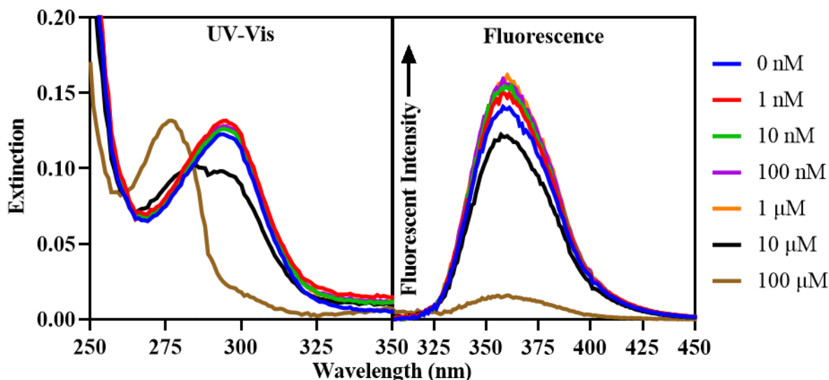
Fig. 4: UV-Vis and fluorescence spectra of 100- \mu\text{M} AB18C6 with concentrations of Mo between 1 nM and 100 \mu\text{M} , with a control solution of 100- \mu\text{M} AB18C6 unmixed with Mo.
