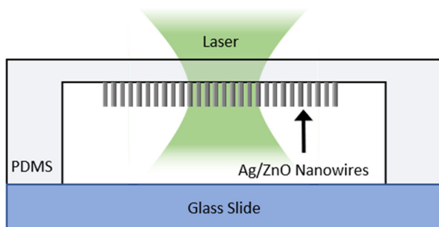
Figure 1: Illustration of the cross-section of a microchannel integrated with an Ag/ZnO nanoprobe fabricated on the PDMS.
