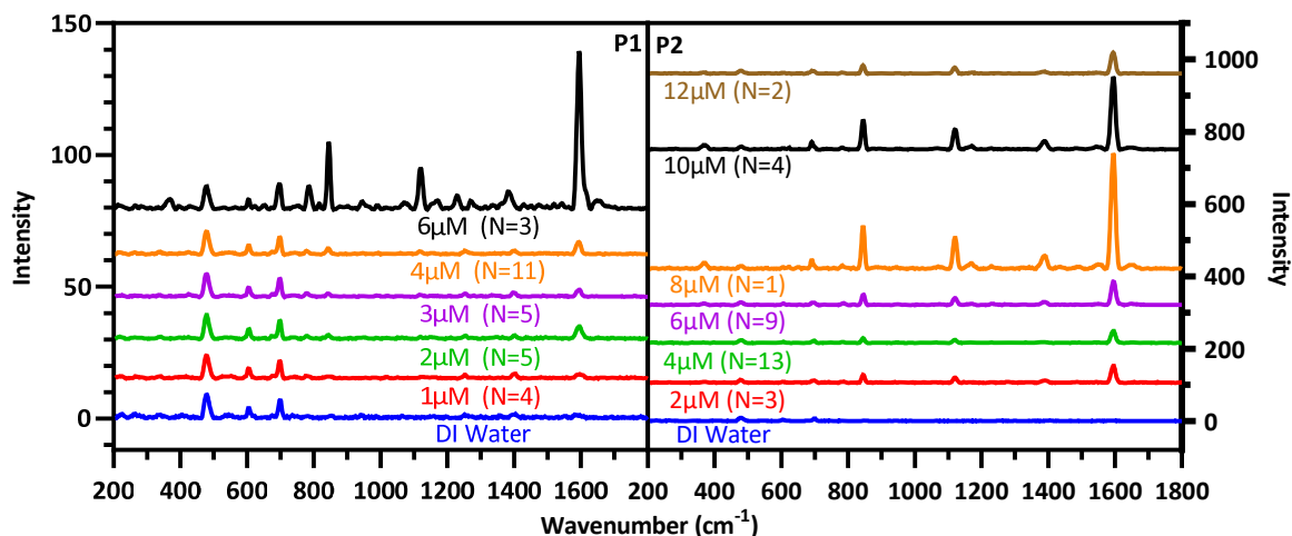
Figure 3: SERS spectra of melamine in DI Water, acquired through P1 on the left and P2 on the right. Number of spectra acquired for each concentration through each substrate in parentheses.
