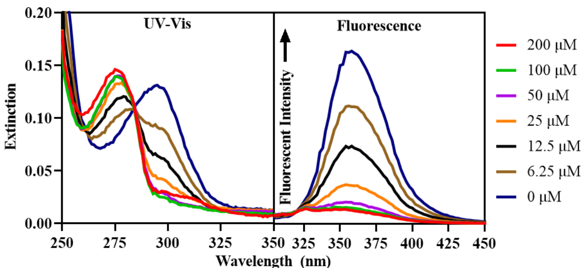
Fig. 5: UV-Vis and fluorescence spectra of 100- \mu\text{M} AB18C6 with concentrations of Mo between 6.25 and 200 \mu\text{M} , with a control solution of 100- \mu\text{M} AB18C6 unmixed with Mo.
