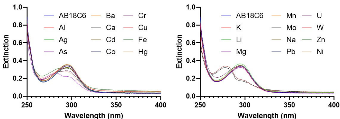
Figure 20: UV-Vis spectra of interactions between 4'-aminobenzo-18-crown-6 and 22 different metals in a 1:1 DMSO:water solution.
