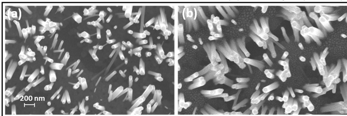
Figure 5: SEM images of ZnO nanowires (a) before and (b) after deposition and anneal of Ag, demonstrating nanowire growth and Ag nanoparticle formation.
