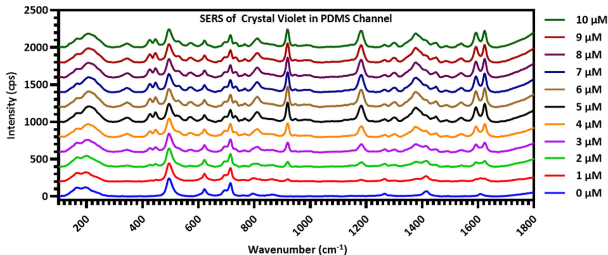
Figure 7: Raman spectra of crystal violet solutions taken inside a fabricated channel, in concentrations ranging from 1 to 10 \mu\text{M} with a DI water control.
