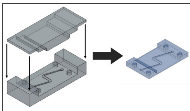
Figure 4: AutoCAD drawing of the microchannel mold designed to enable sensitive SERS through the top channel wall, along with the resultant microchannel.
