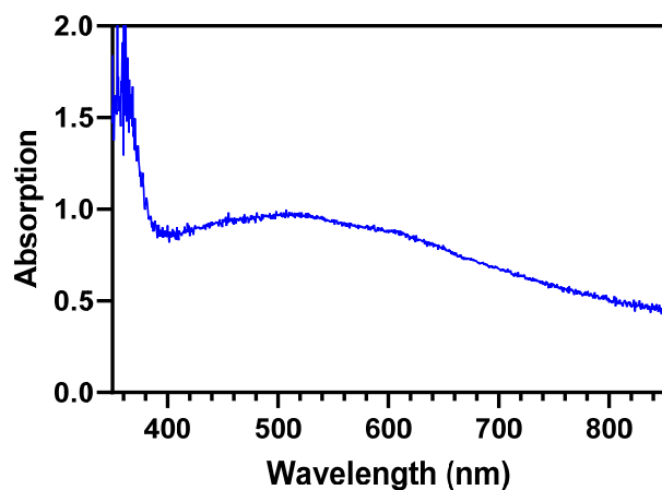
Figure 6: UV-Vis-NIR spectrum of ZnO nanowires decorated with Ag nanoparticles after anneal.
