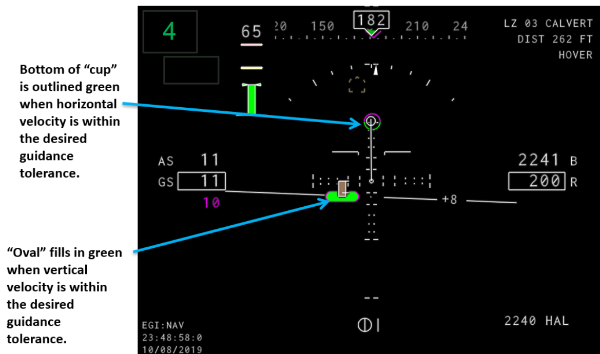
Figure B13. Guidance deviation highlighter.
