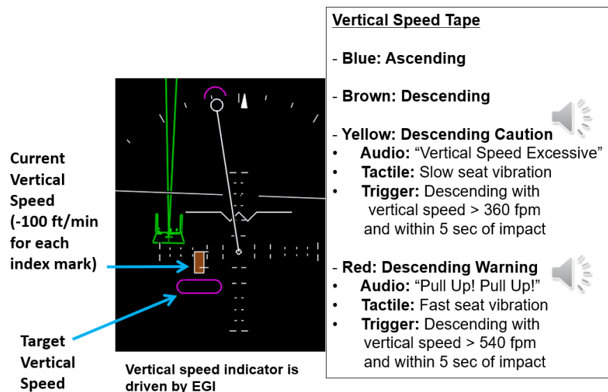
Figure B10. HAT page symbols: vertical speed details.
