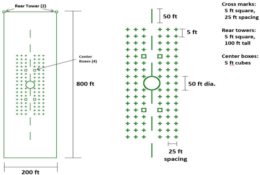
Figure B7. Artificial landing pad dimensions.
