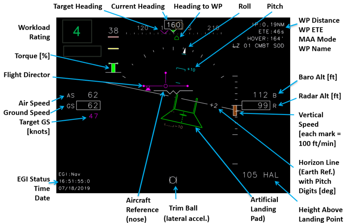
Figure B2. Right display: enroute page.
