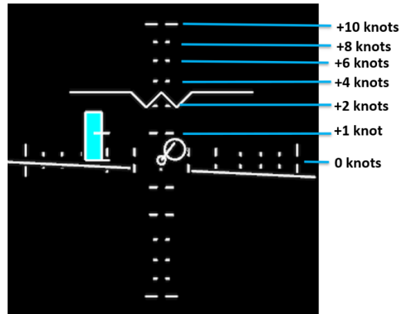
Figure B11. Horizontal velocity vector details.
