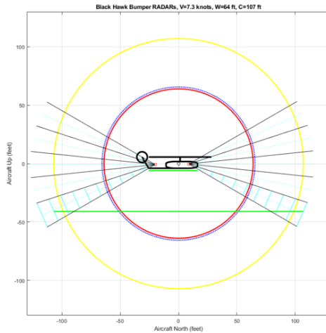
Figure B15. Bumper radar scan: vertical, real vs. synthetic.
