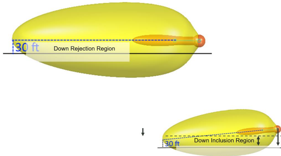
Figure B18. Threat space down inclusion.
