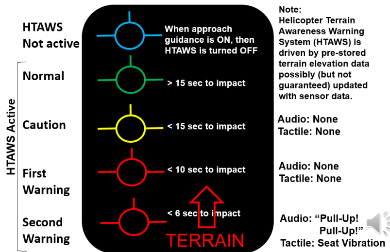
Figure B4. Flight path marker with helicopter terrain avoidance warning system (HTAWS) caution/warning.
