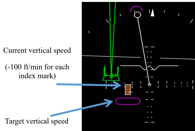
Figure 1. Vertical speed indicator (VSI).
