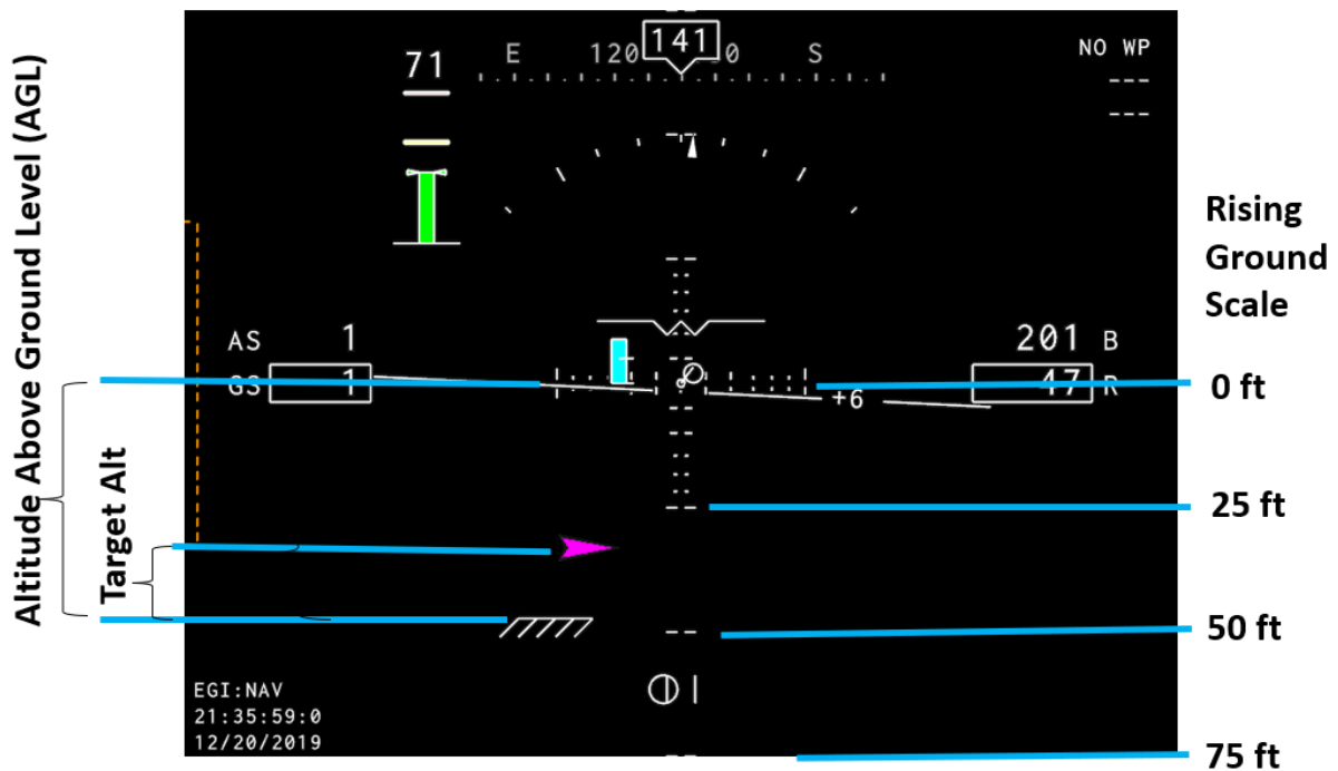
Figure B9. HAT page symbols: altitude details.
