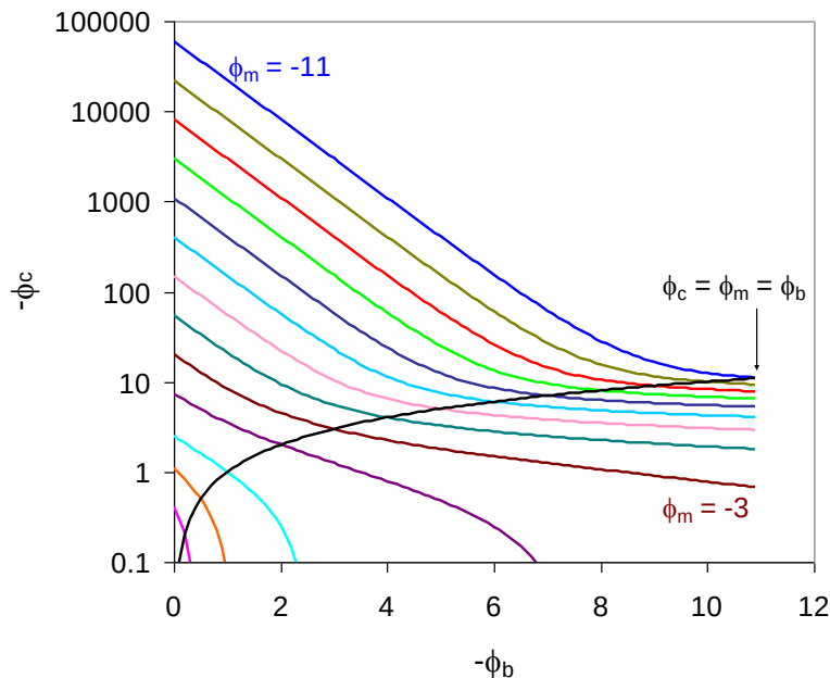
Figure 22. Plot of the Space Charge Cutoff Potential, \Phi_c , Versus Barometric Potential ( \Phi_b = \ln n_i ) for a Series of \Phi_m Values ( -0.2, -0.5, -1.0, -2.0, -3.0, -4.0 \dots -11.0 ). The Point at Which \Phi_m = \Phi_b = \Phi_c is Also Indicated.
