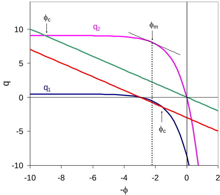
Figure 21. Plots of Space Charge (Curves q_1 and q_2 ) as a Function of Potential as Given by Equation (168). The Straight Lines Represent the Maximum Allowable Charge for Non-oscillatory Potentials. The “Natural” Space Charge, q_1 or q_2 is Acceptable for Cases for Which Slopes of the Curves and the Corresponding Line Are Equal.
