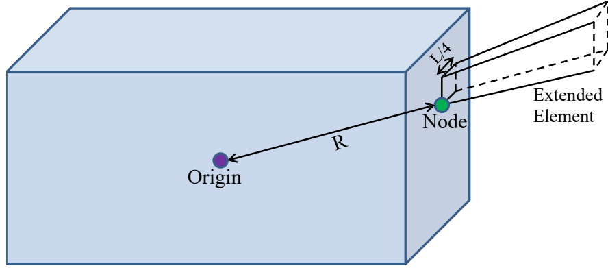
Figure 20. An Extended Element With Analytically Extrapolated Potential is Appended to Each Boundary Quarter-Square to Implement Non-Zero (Monopole) Potential Boundary Conditions.
