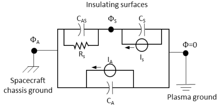
Figure 2. Circuit Model of a Spacecraft with One Insulating Surface Element.
