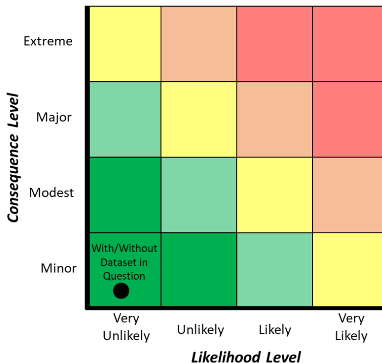
Figure 10. Notional Risk Matrix for Agricultural Case Study
