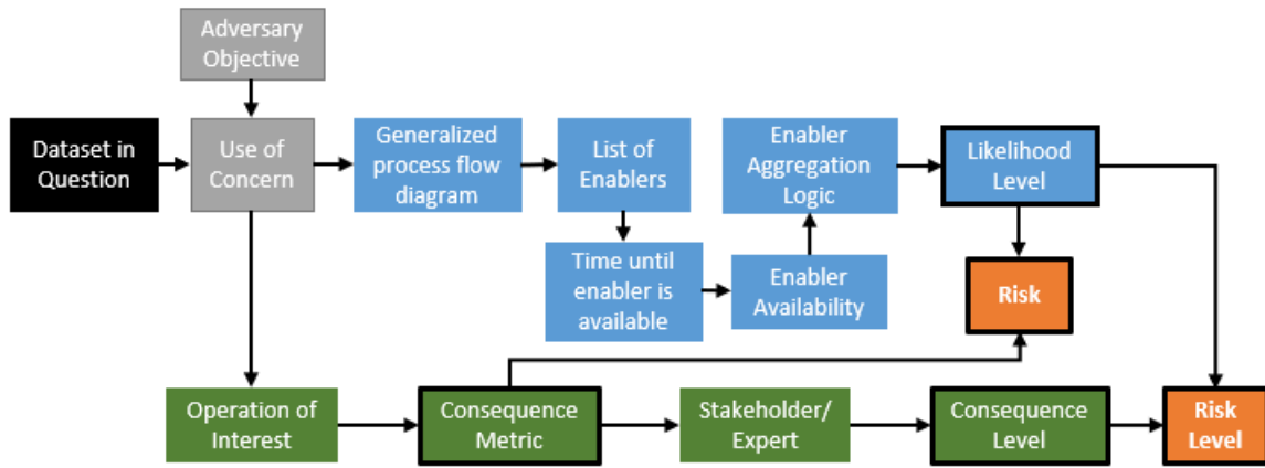
Figure 1. Overview of IDA's Risk Assessment Methodology
