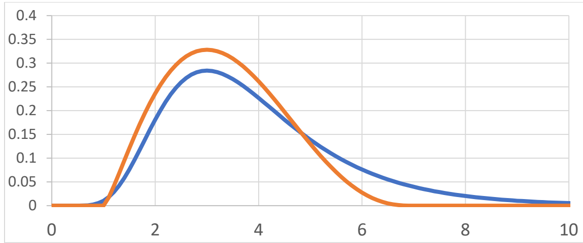
Figure 5. Representative Lognormal Distribution (blue) and PERT Distribution (orange).
