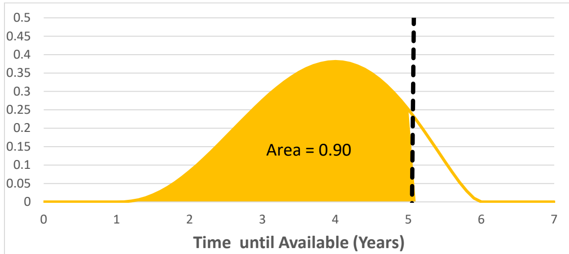
Figure 4. Notional Distribution for an Enabler with a Time until Available of 4 (1-6) years and a Corresponding Availability of 0.90.
