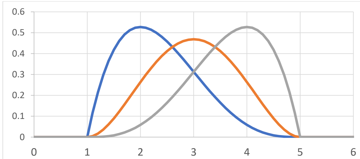
Figure 3. Representative PERT Distributions with a Minimum of 1, a Maximum of 5, and most likely Values of 2 (blue), 3 (orange), and 4 (gray).
