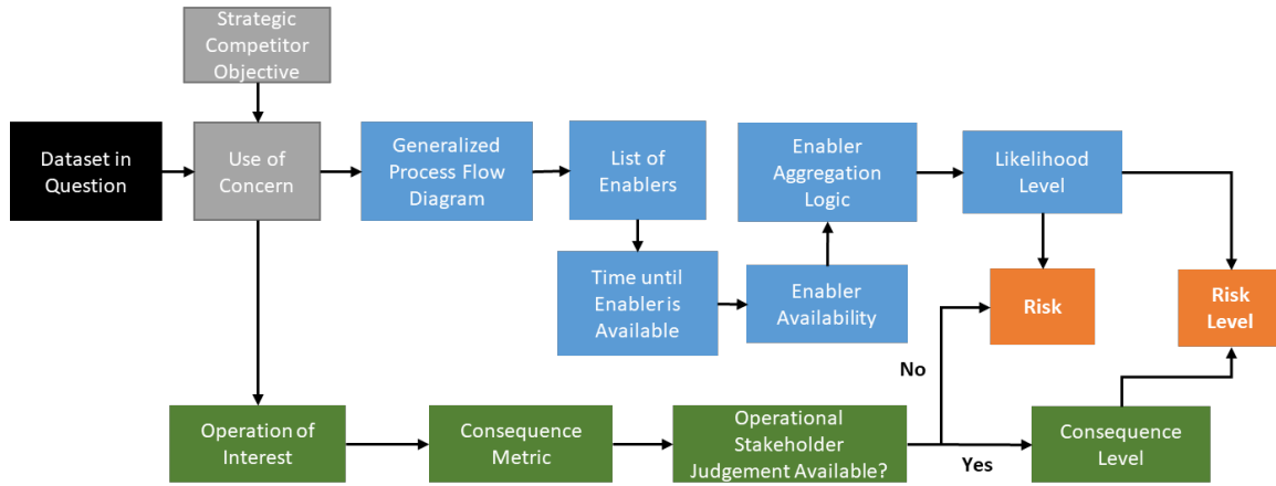
Overview of IDA's Risk Assessment Methodology
