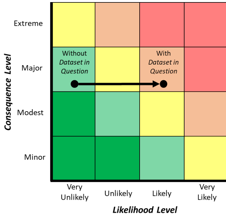
Figure 7. Example Illustrating Change in Risk due to the Strategic Competitor's Access to the Dataset in Question
