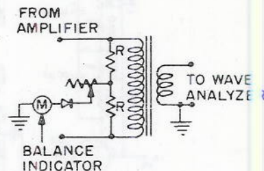
Fig. A4 - Transformer and balance indicator
