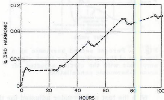
Fig. 12 - Variation of the percent third harmonic of multicoupler with time in the 100-hour stability test
