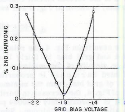
Fig. 6 - Percent second harmonic as a function of the grid bias of the output cathode follower
