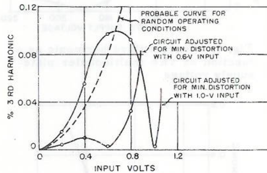
Fig. 8 - Percent third harmonic as a function of the multicoupler input-signal amplitude with the circuit adjusted for third-harmonic cancellation
