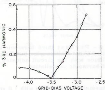
Fig. 11 - Percent third harmonic as a function of the grid bias of the output cathode follower
