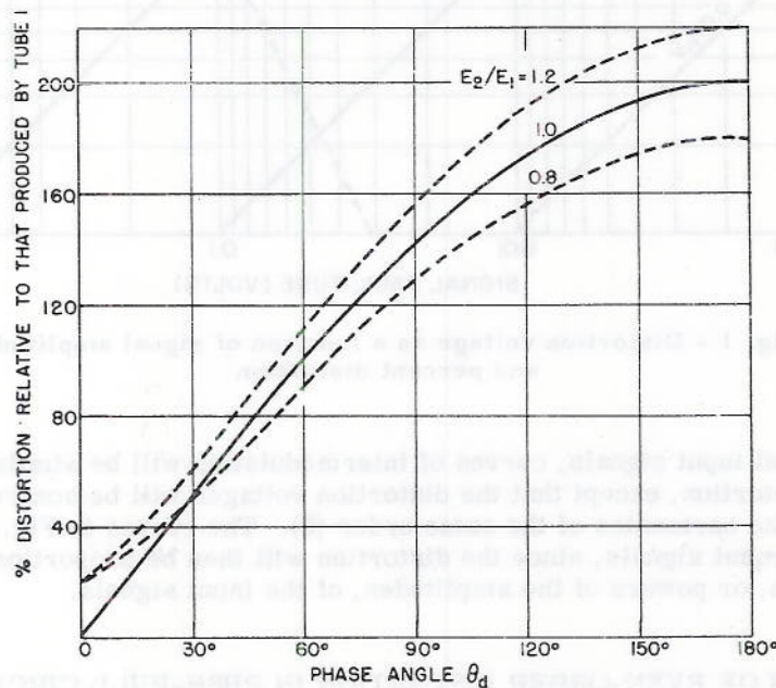
Fig. 2 - Percent even-order distortion in push-pull amplifier relative to that of single tube as a function of amplitude and phase difference
