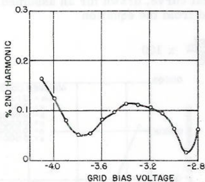
Fig. 5 - Percent second harmonic as a function of grid bias of the input amplifier
