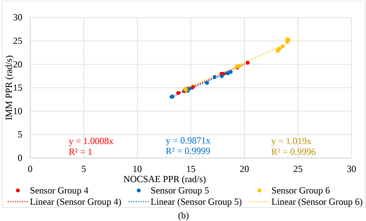
Figure C4. Scatter plots of IMM versus NOCSAE peak kinematics broken down by sensor group for (a) linear acceleration and (b) angular velocity during direct impacts.
