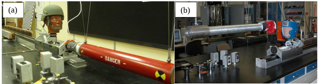
Figure 1. USAARL minisled system showing the (a) indirect or inertial loading setup and the (b) direct loading setup.
