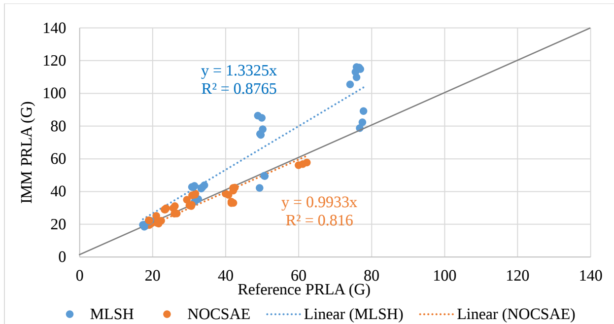
Figure 9. Scatter plot of ATD and instrumented mouthguard peak linear acceleration during direct impacts. The NOCSAE headform had good agreement throughout the test range while the MLSH headform had large errors at the higher test energies.
