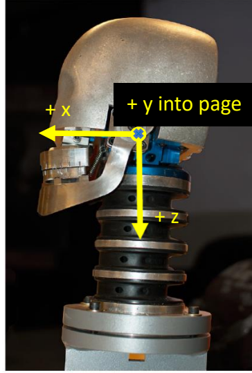
Figure 4. Head CG coordinate system of MLSH without synthetic skin. The coordinate system of the NOCSAE headform is the same as the MLSH.
