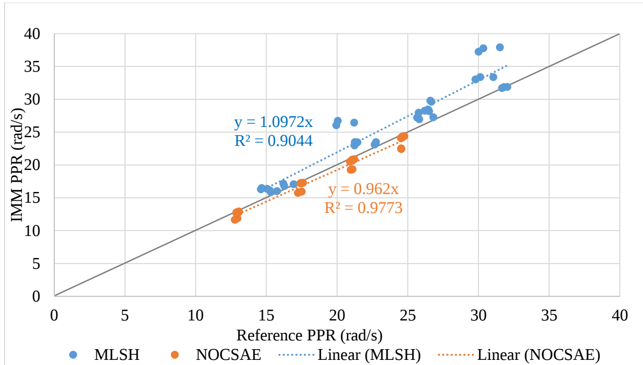
Figure 8. Scatter plot of ATD and instrumented mouthguard peak angular velocity during indirect impacts. For PPR, the instrumented mouthguard response agreed well with both ATDs. *Angular velocity is reported in radians per second (rad/s).
