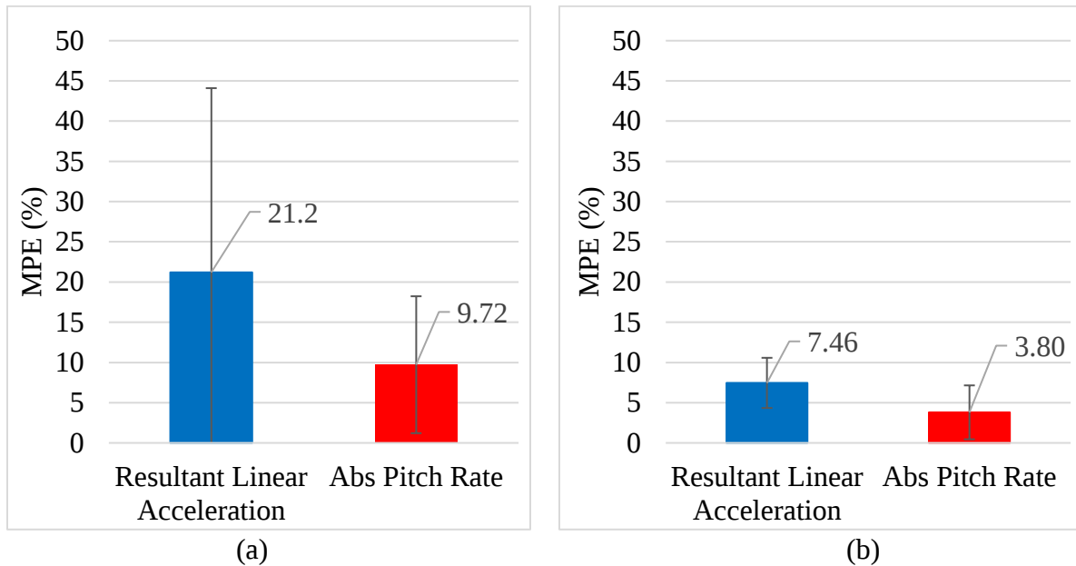
Figure 5. MPE between ATD and instrumented mouthguard peak kinematics for (a) the MLSH and (b) the NOCSAE headform during indirect impacts. For both ATDs, the MPE for the angular rate was consistently lower than the resultant linear acceleration. “Abs Pitch Rate” is the absolute value of the pitch rate.
