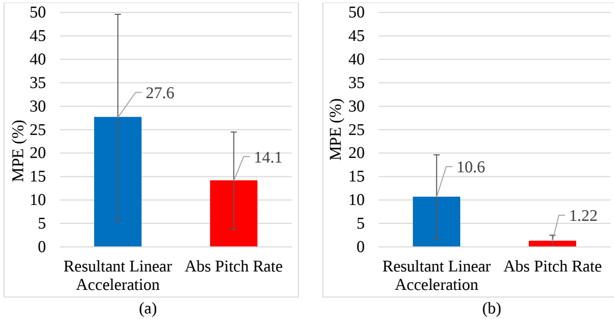
Figure 6. Mean percent error between ATD and instrumented mouthguard peak kinematics for (a) the MLSH and (b) the NOCSAE headform during direct impacts. For both ATDs, the MPE for the angular rate was consistently lower than the resultant linear acceleration. “Abs Pitch Rate” is the absolute value of the pitch rate.
