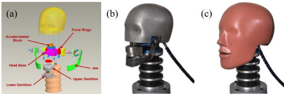
Figure 2. MLSH. (a) Exploded view, (b) assembled and attached to an H-III neck, and (c) with synthetic H-III skin.
