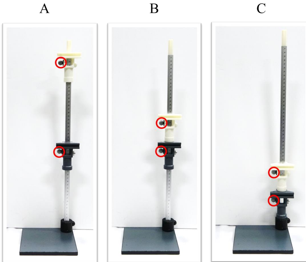
Figure 4. Stadiometer measuring branch holders with attached markers (circled in red) as used in the stadiometer fixture captures. (A) The starting position of the measuring branch holders; (B) the point at which the top measuring branch holder meets the bottom; and (C) the ending position of the measuring branch holders.
