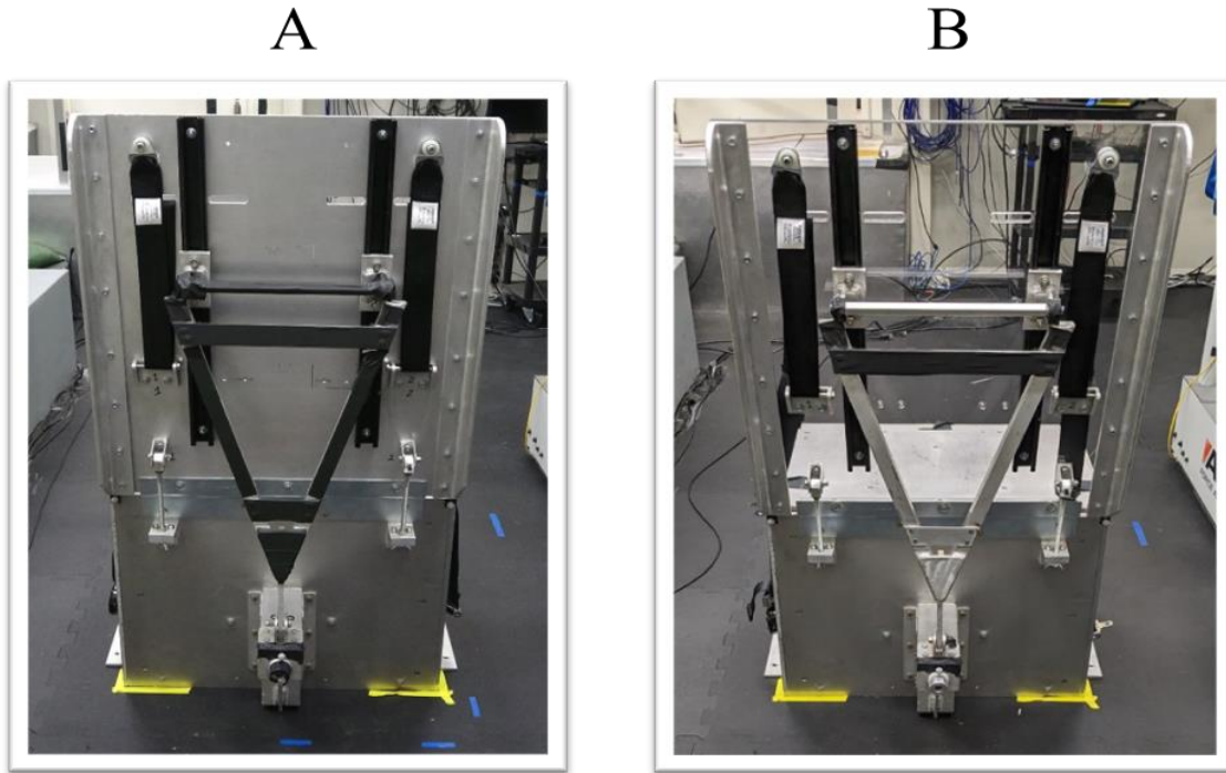
Figure 1. The MARS chair with the (A) existing aluminum seat back retrofitted with a (B) TSB of the same dimensions (except thickness) to investigate whether optical tracking of spinal motion was possible.
