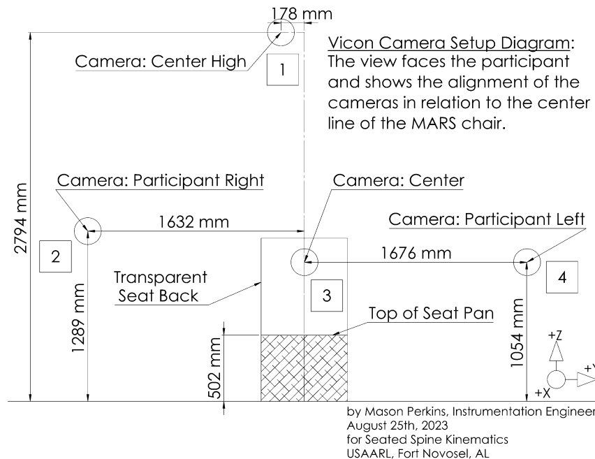
Figure 2. Vicon motion capture cameras (numbered 1 through 4) were positioned on a wall approximately 2387.6 mm behind the chair to examine the effect of camera angle on marker positioning through the TSB. Camera measurements relative to the chair centerline are provided.
