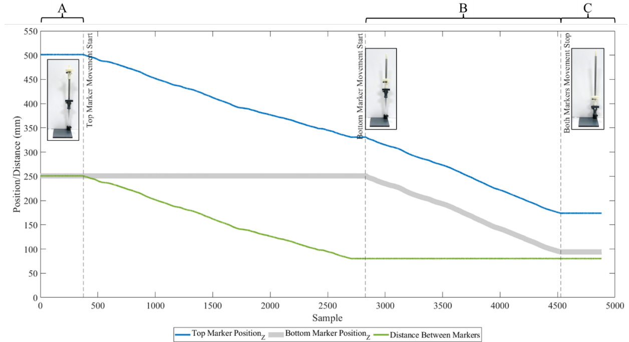
Figure 7. The top measuring branch holder marker z-axis positional data (blue), the bottom measuring branch holder z-axis positional data (gray), and the straight line between-marker distance (green) for stadiometer movement capture trials were plotted to allow the identification of marker movement segments. Segment A is the portion used to compute the between-marker starting distance. Segment B is the portion used to compute the between-marker moving distance. Segment C is the portion used to compute the between-marker ending distance. Also pictured are the stadiometer measuring branch holder positions during segment A, at the beginning of segment B, and during segment C.
