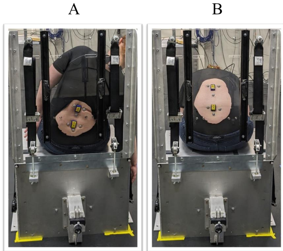
Figure 6. (A) Lateral bending and (B) forward flexion torso directional tasks performed during the human movement captures. While inertial measurement units are pictured, these data are not reported in this effort.
