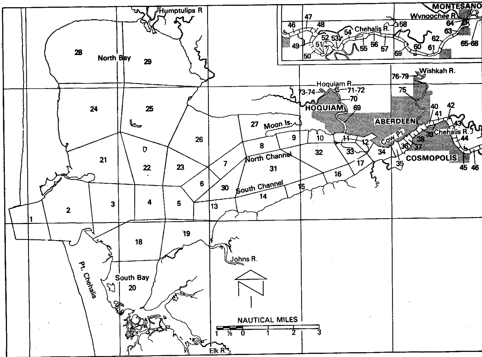
Figure 7-1. Divisions and junctions of the mathematical model of Grays Harbor developed by the EPA. (From Cleland, 1978)
