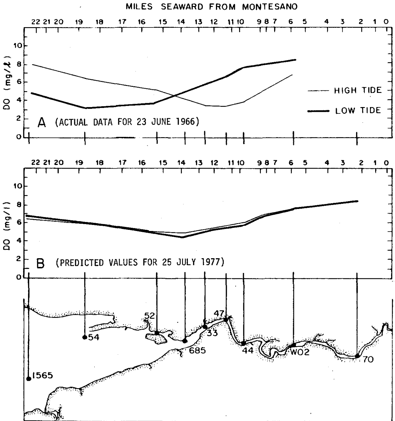
Figure 7-4. Comparison of actual and predicted concentrations of dissolved oxygen for nearly identical tide ranges. (Note - the mathematical model predicted values did not show the migration of the "DO sag".)
