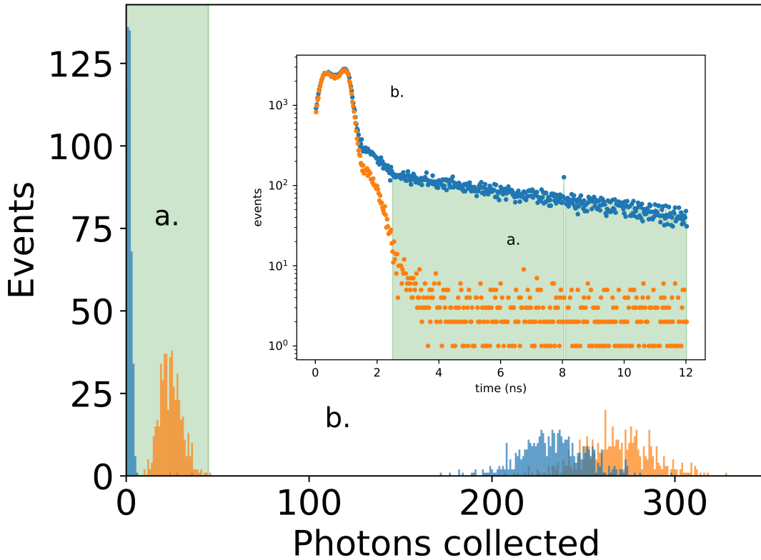
Figure 8.8: Detection of Rabi oscillation of the hyperfine qubit using the frequency comb bright state histogram and are therefore likely due to incomplete shelving, not poor manifold discrimination. Further improvements in shelving [52] can be used to reduce this infidelity, and this type of error will be entirely absent for optical-frequency qubits.
