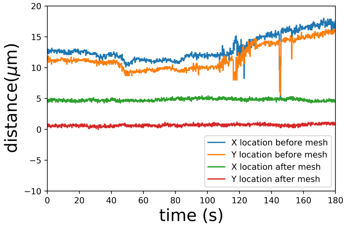
Figure 4.10: Ion drift rate with before mesh on windows (blue X, orange, Y) and after mesh is installed (green X, red Y)
