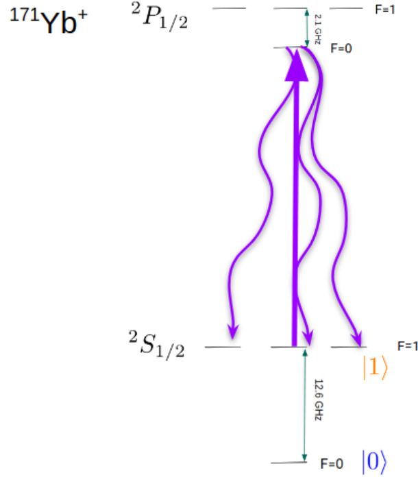
Figure 1.9: State detection is performed by cycling the ^2S_{1/2}F = 1 manifold to the ^2P_{1/2}F = 0 and collecting the resultant state dependant fluorescence
