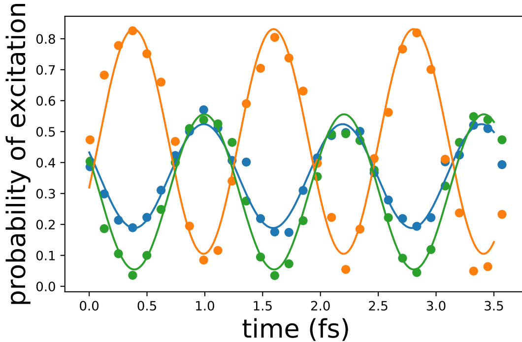
Figure 8.6: Ramsey experiment on the three transitions involved
