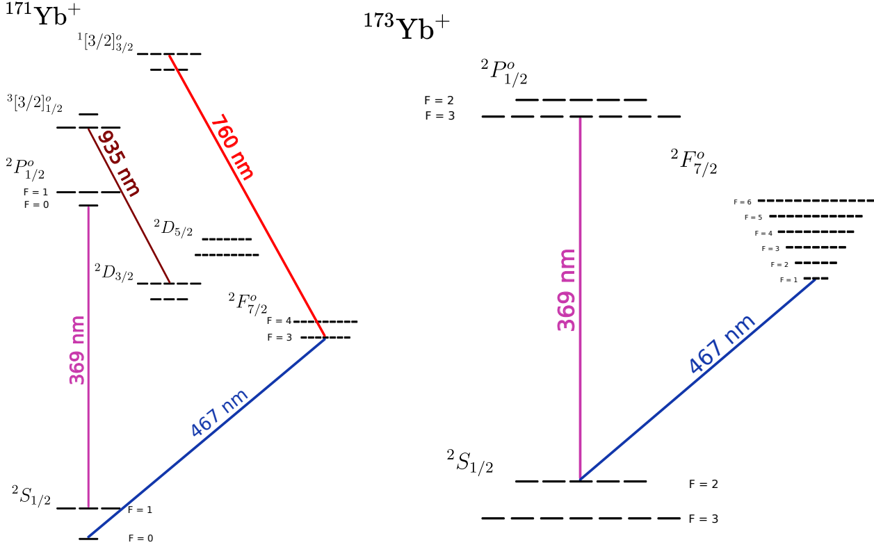
Figure 10.1: Structure of ^{171}\text{Yb}^+ . Frequency-selective driving of the ^2S_{1/2}(F = 0) states to ^2F_{7/2}^o(F = 3) on the octopole transition will coherently shelve this population. ^{173}\text{Yb}^+ structure used in fast excitation and shelving (right)
