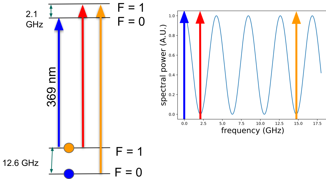
Figure 8.2: Hyperfine structure of ^{171}\text{Yb}^+ (left) showing the transition in blue that we desire to drive and the orange and red transitions which are to be avoided. The right shows the frequency of these transitions relative to the state selective cycling transition (blue) superimposed with the Mach-Zehnder interferometer frequency output.
