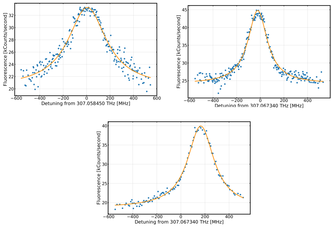
Figure 4.8: 976 nm spectrums. Upper left, F=2 to F=1. Upper right, F=2 to F=2. Bottom F=3 to F=2
