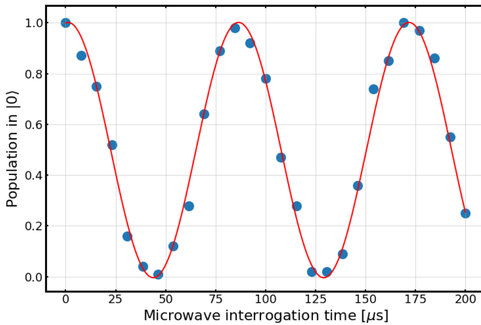
Figure 8.9: Detection of Rabi oscillation of the hyperfine qubit using the frequency comb while shelving to the F state
