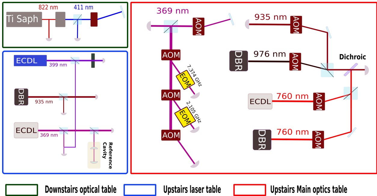
Figure 4.11: Laser setup, all lasers are measured on wavemeters and sent through single pass AOMs for switching except for the 399 nm which is shuttered with a hard drive switch. The 369nm laser is double passed prior to going to the different single pass AOMs for switching. The double pass allows for fast frequency switching as well as slow feedback for cavity drifts.
