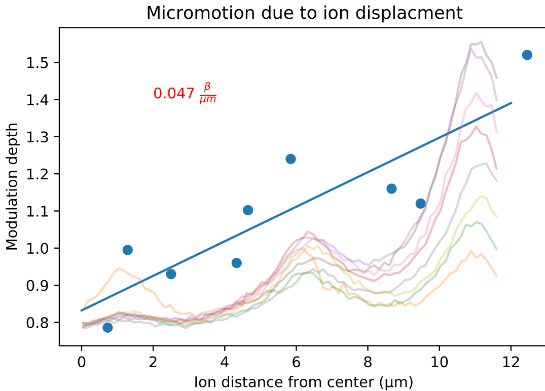
Figure 1.3: Micromotion compensation via minimization of modulation. The ion is moved until no noticeable peaks occur at multiples of the RF drive frequency
