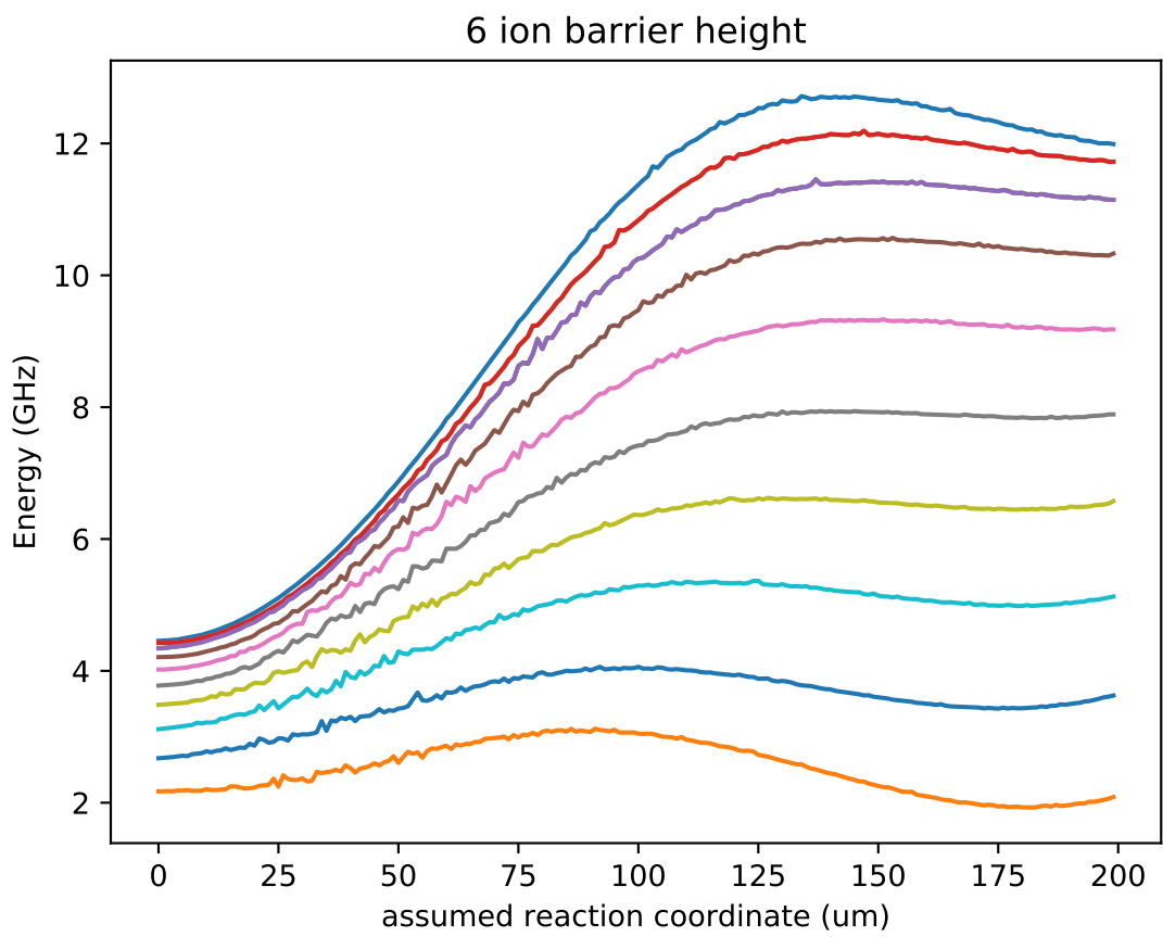
Figure 5.4: 6 ion barrier height at different asymmetries
