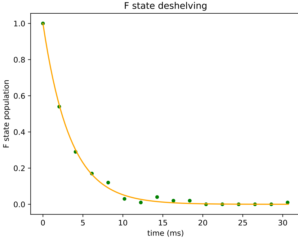
Figure 7.5: Desheling of the F state manifold with the 760 nm repumpers. Time constants of a few ms are achieved with \approx 5\text{mW} of power in a 100\ \mu\text{m} beam waist.
