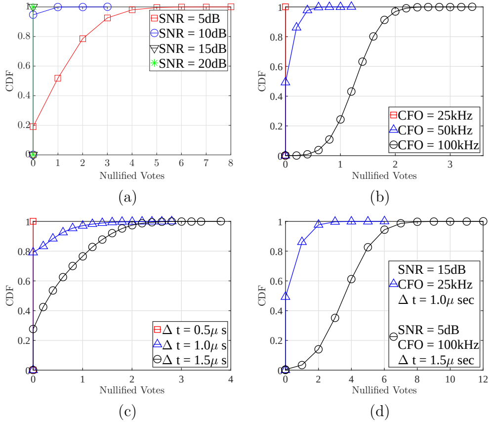
Figure 7.12: (a) CDF plot of number of nullified votes due to wireless channel noise for varying channel SNR, (b) CDF plot of number of nullified votes received due to carrier frequency offset error for varying CFO, (c) CDF plot of number of nullified votes received due to synchronization error for varying time offset, and (d) CDF of the nullified votes when the fading, CFO, and time misalignment phenomena are all combined in the same experiment.
