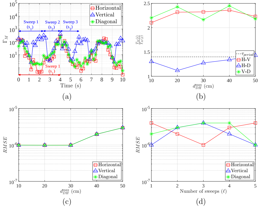
Figure 4.12: (a) RSS ratio fluctuation for a Type 2 adversary as function of the time at 2m from D , (b) T_M(i)/T_M(j) as a function of the maximum D -to- H distances for a Type 3 adversary mimicking transmit power for vertical sweeping motion of H , (c) RMSE as a function of the maximum D -to- H distances for various sweeping motions, and (d) RMSE as a function of the number of sweeps ( \ell ) for various sweeping motions.
