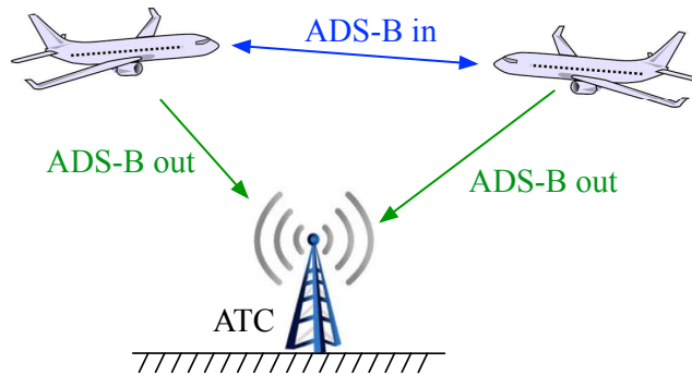
Figure 6.1: The ADS-B architecture.
