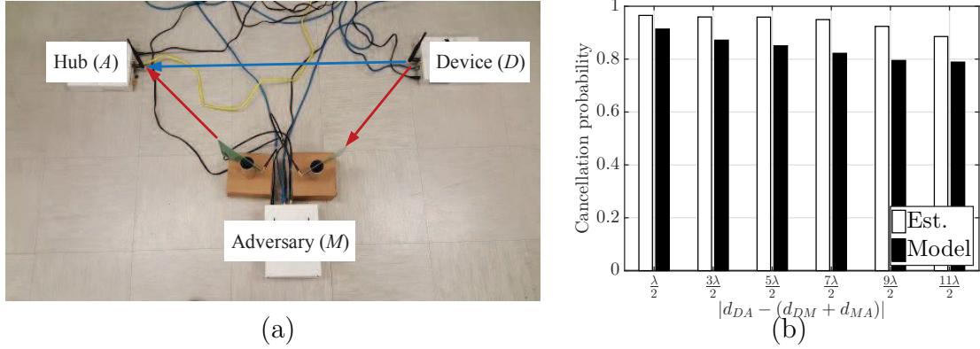
Figure 2.10: (a) Experimental setup for evaluating signal cancellation for a single device-hub pair, and (b) cancellation probability as a function of the distance difference between the direct path from D -to- A and the relay path through M .
