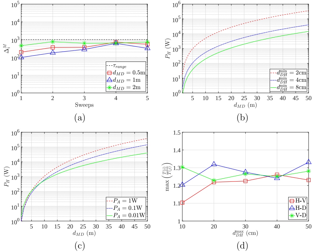
Figure 4.11: (a) RSS ratio range as a function of the sweeps for Type 2 adversary with \tau_{range} selected for d_{DH}^{max} = 50cm and P_A = 0.1W , (b) maximum transmit power of a Type 3 adversary to H as a function of d_{MD} when transmitting with P'_A = 10W for achieving \tau_{range} for various d_{DH}^{min} , (c) maximum transmit power of a Type 3 adversary to H as a function of d_{MD} when transmitting with P'_A = 10W for achieving \tau_{range} for various \tau_A , and (d) \max(T^{(i)}/T^{(j)}) as a function of the maximum D -to- H distances for each motion for various RSS at A .
