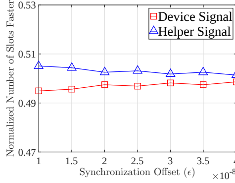
Figure 3.10: Fraction of slots that one device is faster than the other as a function of the delay offset \epsilon .
