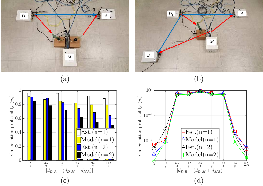
Figure 5.19: (a) Experimental setup for signal cancellation from one TX to one RX, (b) experimental setup for signal cancellation from one TX to two RXs, (c) cancellation probability as a function of the distance difference between the direct and the relay paths when M is placed at an ellipse satisfying eq. (5.4), and (d) cancellation probability as a function of the distance difference between the direct and the relay paths, when M is perturbed from the location with path difference equal to 3\lambda/2 .
