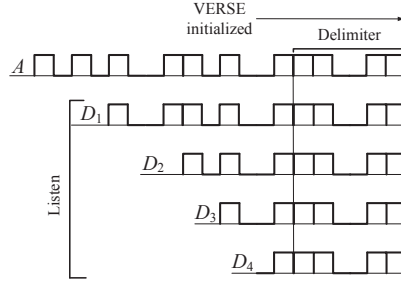
Figure 5.8: Protocol initialization. The hub broadcasts an MC ON-OFF sequence during device activation. This sequence terminates with a known delimiter.
