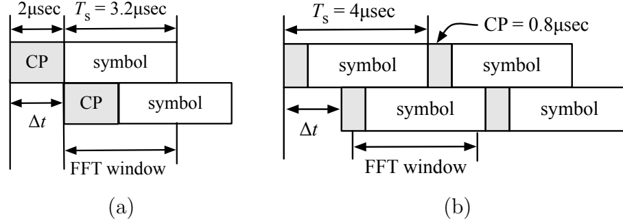
Figure 7.8: (a) Increasing the CP, (b) casting a symbol vote in two symbol durations.
