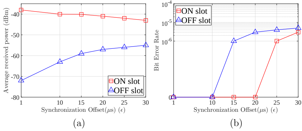
Figure 5.22: (a) Average received power of superimposed signal from D_1 , D_2 , and D_3 on ON and OFF slots as a function of synchronization offset ( \epsilon ), and (b) bit error rate as a function of synchronization offset ( \epsilon ) in \mu s .
