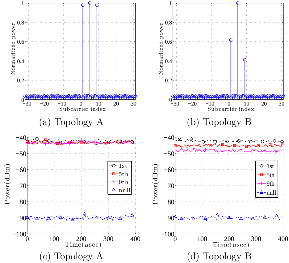
Figure 7.9: (a), (b) Normalized average received power per subcarrier, (c), (d) received power per subcarrier as a function of time.
