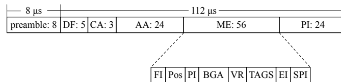
Figure 6.2: The ADS-B frame format.
