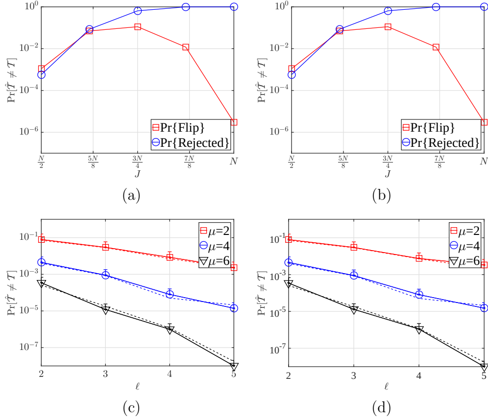
Figure 7.15: (a) Probability of flipping voting outcome and rejecting a voting round as a function of the number of attacked subcarriers ( J ) in presence of an external adversary, and for 26 participants, (b) probability of flipping voting outcome and rejecting a voting round as a function of the number of attacked subcarriers ( J ) in presence of an external adversary, and for 100 participants, (c) probability of flipping the voting outcome as a function of the number of symbol votes ( \ell ) in presence of an internal adversary, and for 26 participants, and (d) probability of flipping the voting outcome as a function of the number of symbol votes ( \ell ) in presence of an internal adversary, and for 100 participants.
