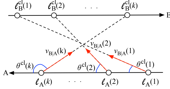
Figure 6.4: Position and relative radial velocity at k distinct locations.
