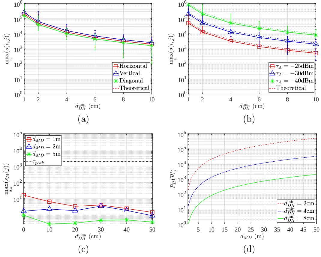
Figure 4.9: (a) Peak RSS ratio as a function of the minimum D -to- H distances in each sweep for various sweeping motions, (b) peak RSS ratio as a function of the minimum D -to- H distances in each sweep for various RSS at A , (c) peak RSS ratio as a function of the maximum D -to- H distances in each sweep for various d_{MD} for a Type 1 adversary, and (d) maximum transmit power of a Type 2 adversary to achieve \tau_{peak} as a function of d_{MD} for various d_{DH}^{\min} .
