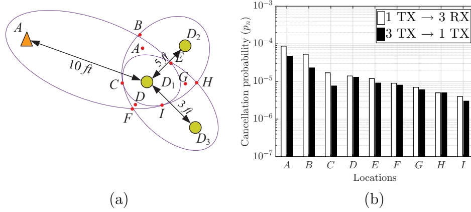
Figure 5.20: (a) Experimental topology for the evaluation of security primitive of VERSE, and (b) cancellation probability for the experimental setup of (a).
