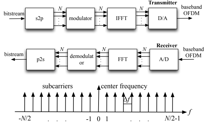
Figure 7.2: Block diagram of OFDM.
