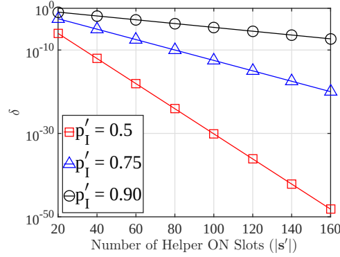
Figure 3.12: Probability of pairing with a rogue A as a function of |s| , for varying inference capabilities of helper activity.
