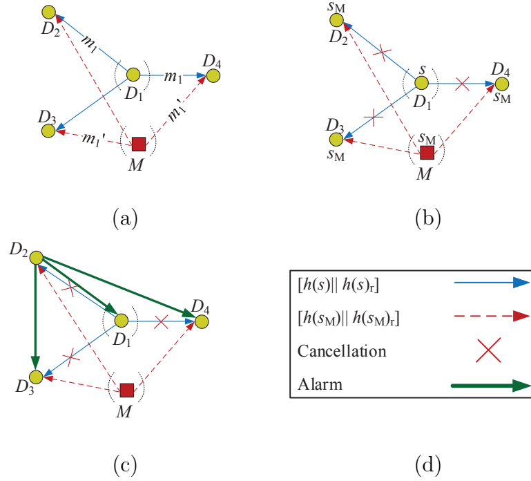
Figure 5.15: (a) M replacing m_1 with m_1' during overshadowing attack, (b) M attempting to perform signal cancellation on D_1 's transmission to D_2 , D_3 and D_4 during the verification phase of the VERSE primitive (c) D_2 raises the alarm after detecting error during the verification phase of the VERSE primitive, and (d) legends for the figure.
