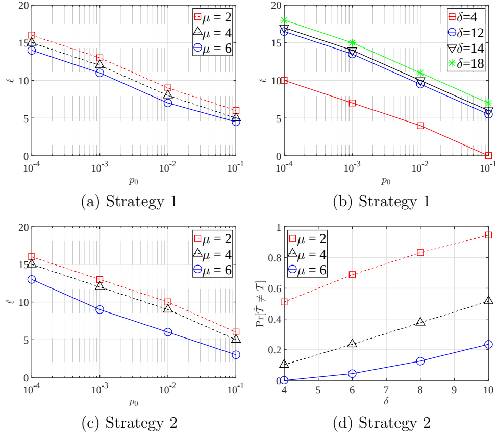
Figure 7.5: Minimum number of symbol votes \ell to guarantee robustness p_0 (a) under the secret vote model for Strategy 1, (b) for \mu = 4 and various \delta , under the secret vote model and for Strategy 1, (c) under the open vote model for Strategy 2, (d) under the secret vote model for Strategy 2.
