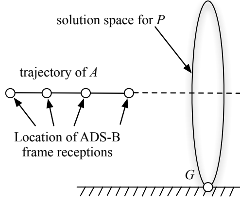
Figure 6.5: The possible spoofed locations of G that satisfy P .
