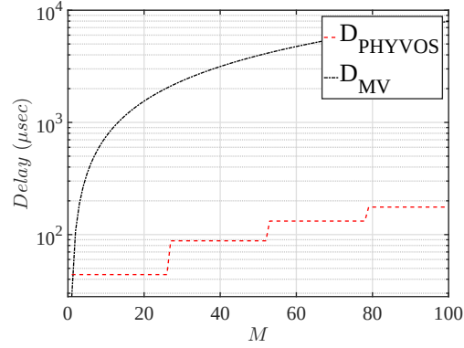
Figure 7.7: Voting overhead as a function of M for message-based voting (MV) and PHYVOS.
