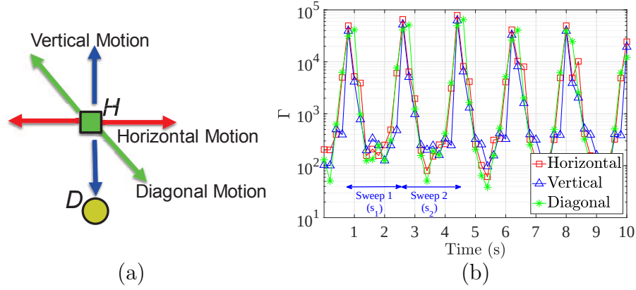
Figure 4.3: (a) Various sweeping motions of H over D , (b) RSS ratio fluctuation as a function of time for various motions.
