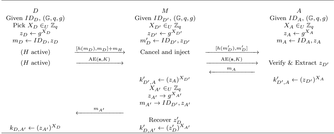
Figure 3.6: MitM attack against the key-agreement phase of HELP-enabled pairing protocol.
