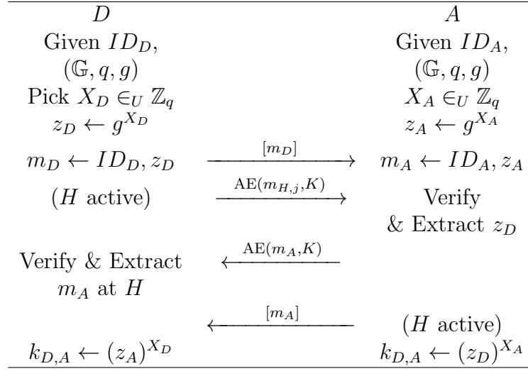
Figure 4.2: DH key agreement using SFIRE as a message authenticator.
