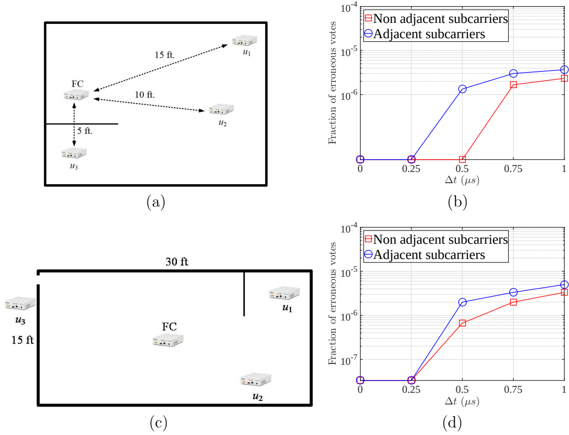
Figure 7.10: (a) The USRP topology used to evaluate the effect of time synchronization, (b) fraction of erroneously decoded votes at the receiver as a function of the synchronization error ( \Delta t ) between participants, c) the USRP topology used to evaluate the effect of NLoS paths, and (d) fraction of erroneously received votes as a function of the synchronization error ( \Delta t ) for the topology of Fig 7.10(c).
