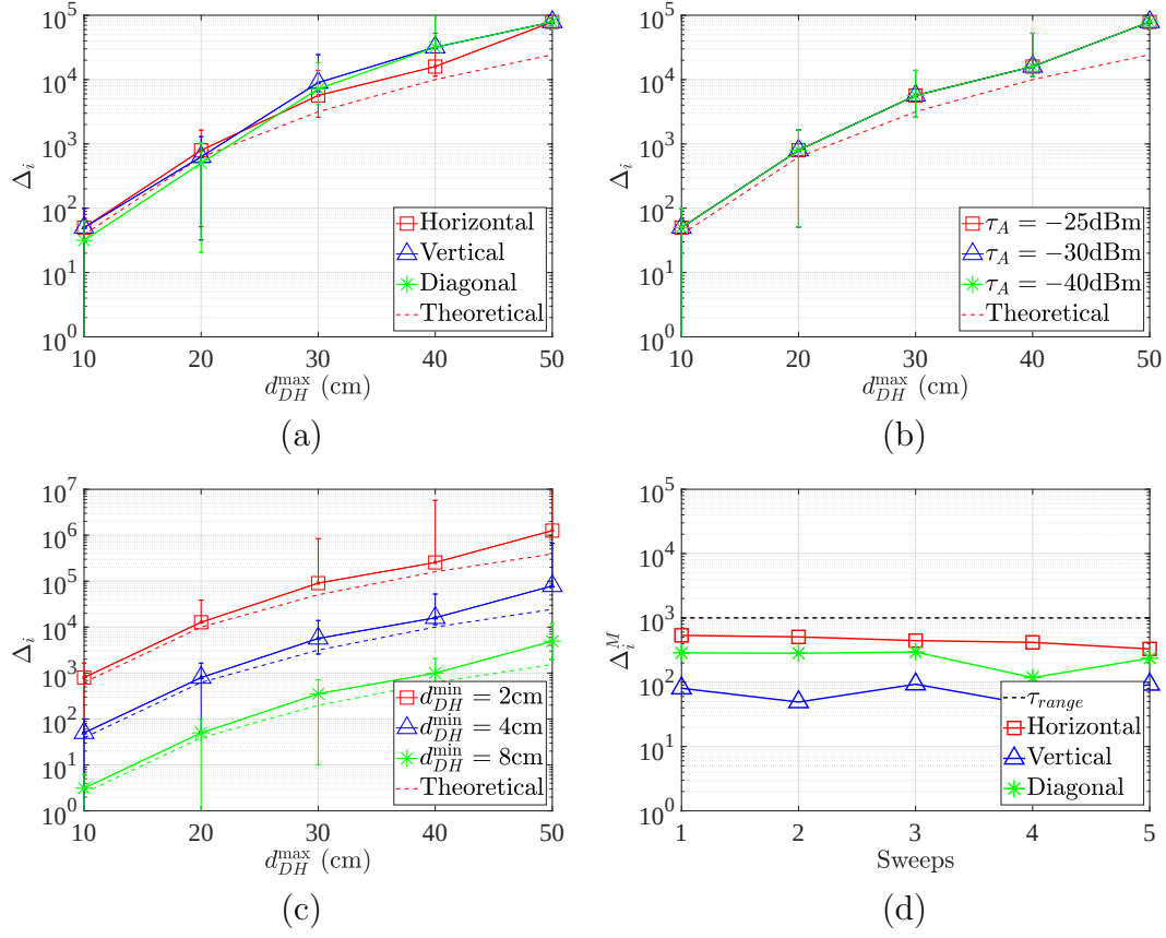
Figure 4.10: (a) RSS ratio range of \mathbf{s}_i as a function of the maximum D -to- H distances in each sweep for various sweeping motions, (b) RSS ratio range of \mathbf{s}_i as a function of the maximum D -to- H distances in each sweep for various RSS at A , (c) RSS ratio range of \mathbf{s}_i as a function of the maximum D -to- H distances in each sweep for various d_{DH}^{\min} , and (d) RSS ratio range as a function of the sweeps for a Type 2 adversary for d_{MD} = 2\text{m} with \tau_{range} selected for d_{DH}^{\max} = 50\text{cm} and P_A = 0.1\text{W} .
