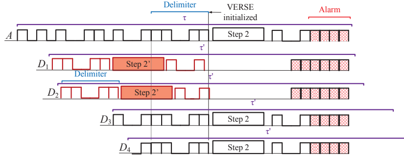
Figure 5.18: Attack on the initialization step of VERSE.
