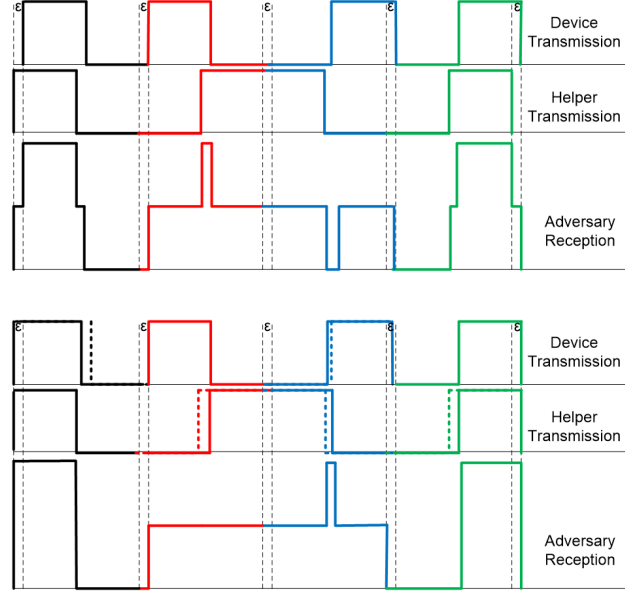
Figure 3.9: Synchronization offset without and with randomized start time of each bit.
