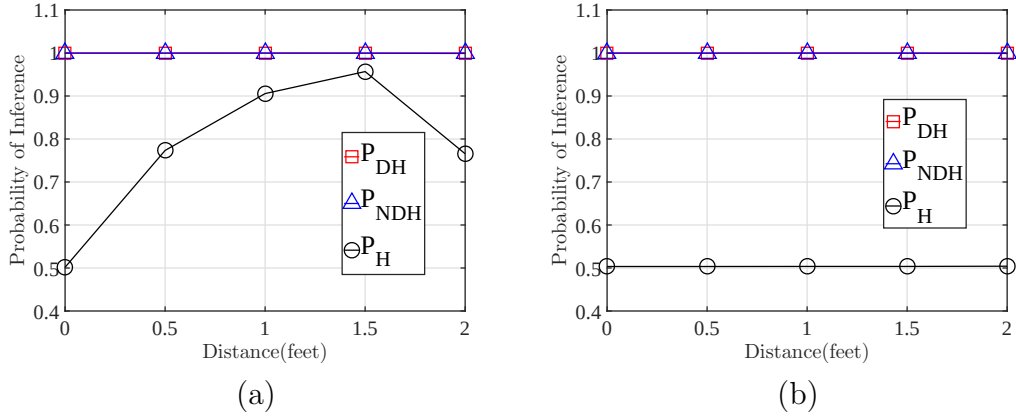
Figure 3.8: (a) Detection probability as a function of the distance between D and H when H is moved towards M , and (b) detection probability as a function of the distance between D and H when H is moved towards M , when D and H are transmitting random powers.
