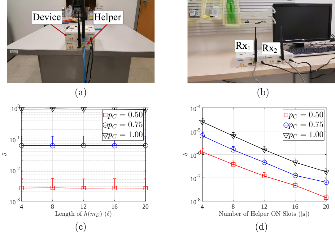
Figure 3.11: (a) Placement of D and H , (b) placement of the A ( RX_1 ) and RX_2 . (c) probability of acceptance of a modified message at the A in the absence of H , and (d) probability of acceptance of a modified message at the A in the presence of H .
