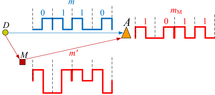
Figure 2.8: MitM attack by M to modify D 's MC ON-OFF transmission such that A decodes m_M instead of m .
