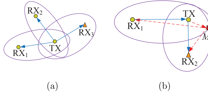
Figure 5.11: (a) TX placed on the shared focus of three ellipses which have RX 1 , RX 2 and RX 3 on the other foci respectively. An adversary positioned on one ellipse can cancel the TX signal at the RX positioned at the ellipse's other focal point. No common intersection point exist among three ellipses, and (b) M is placed on the intersection point between two ellipses to simultaneously cancel the signal at RX 1 and RX 2 .
