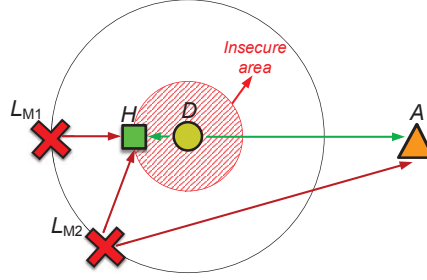
Figure 4.4: The adversary placed at L_{M1} (co-linear with H -to- A line) is the optimal position is outside the insecure area with fixed M -to- D distance for maximizing the RSS peak ratio.
