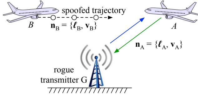
Figure 6.3: Spoofing aircraft B at A by transmitting ADS-B messages from G .
