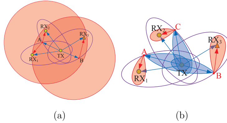
Figure 5.12: (a) The adversary places two colluding devices one at A with omnidirectional transmission antenna and highly directional receiving antenna and other at B with highly directional antenna, the attack fails due to self-interference, and (b) the adversary places three colluding devices at A , B and C with highly directional antenna.
