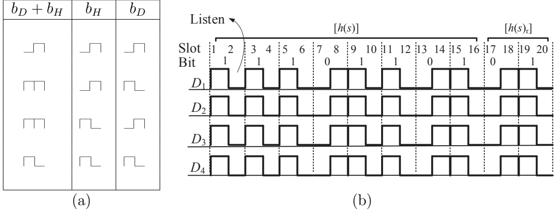
Figure 3.2: (a) Truth table for recovering [h(m_D)]' from ([h(m_D)] + m_H)' , using \mathbf{s} , and (b) an example of recovering [h(m_D)]' from ([h(m_D)] + m_H)' .
