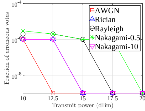
Figure 7.13: Fraction of incorrectly received votes as a function of the transmission power for various wireless channel models.
