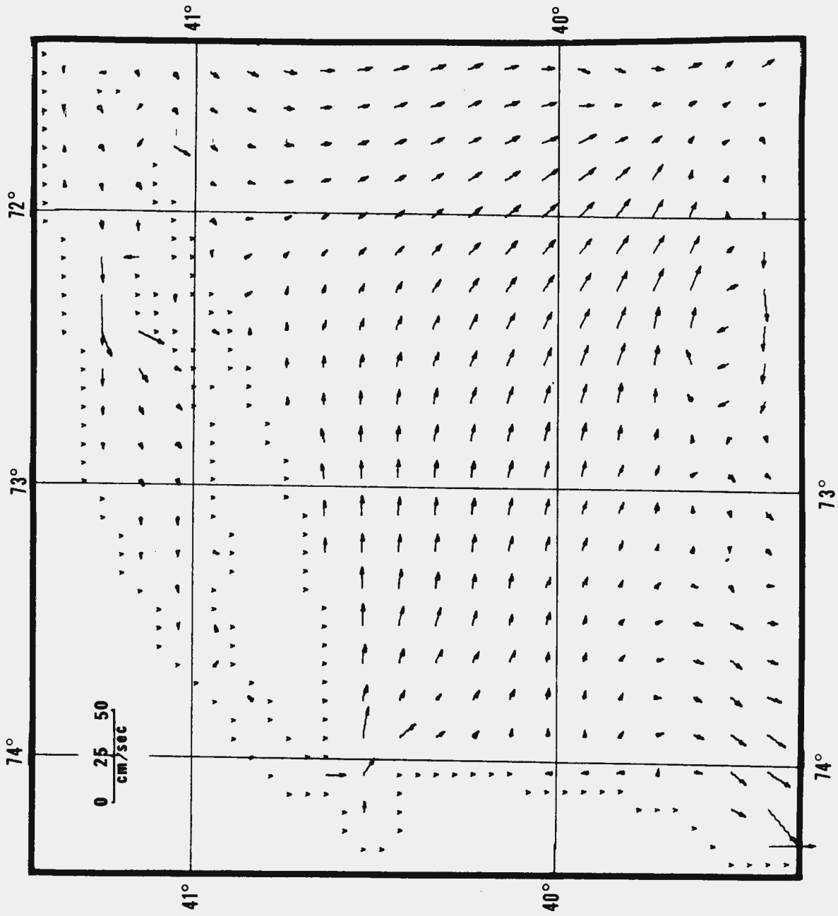
Figure 22 Currents during 2 hours before low water at Sandy Hook
