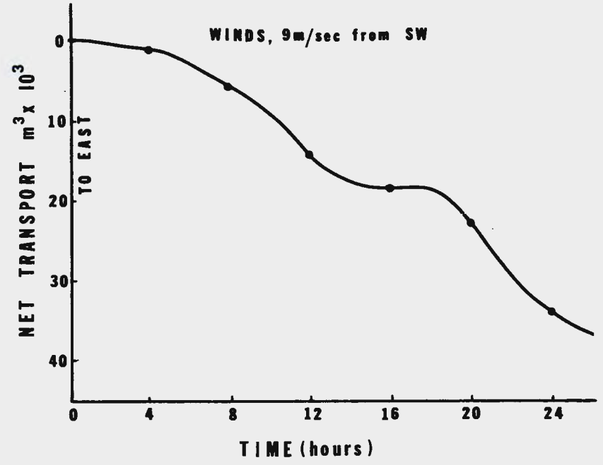
Figure 66 Transport rate through section BB6 in surface layer in calm and with SW wind 9m/sec.
