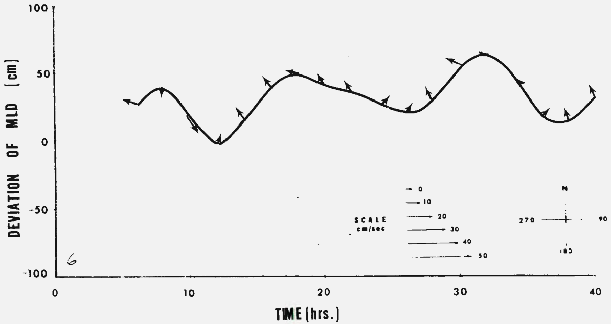
Figure 45 A Sea level changes and currents in upper layer at Point 7 (location see Figure 1) as computed with 2-layer HN model; wind 9\text{m/sec}^{-1} from SW B Change of mixed layer depth from mean and currents in lower layer at Point 7 (location and wind the same as for upper layer)
