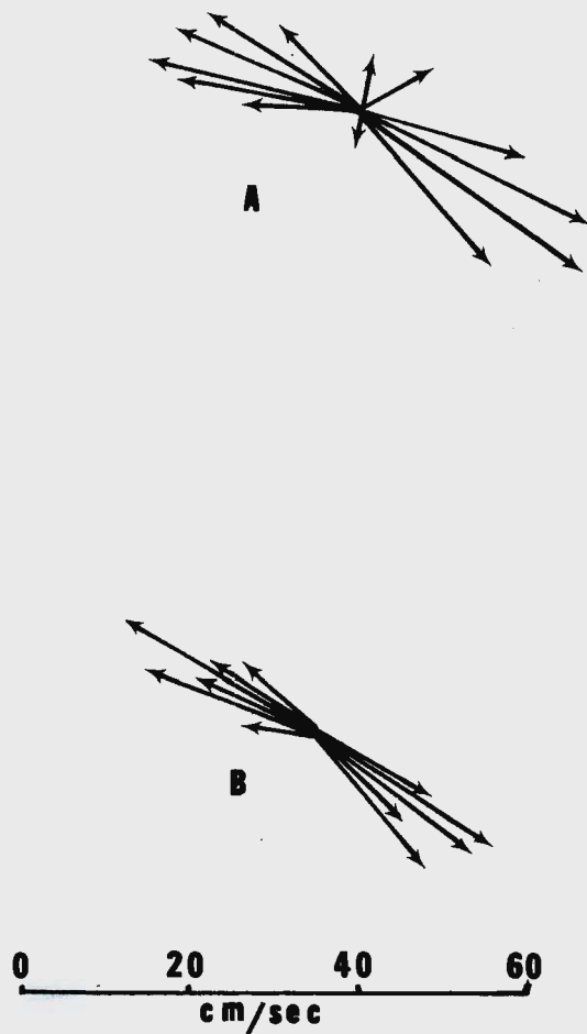
Figure 16 A Mean tidal currents at Scotland Lightship (40°26.6'N; 73°55.2'W) (from Haight, 1942) B Tidal currents (spring tides) at grid point 22,37 (see Figure 1).
