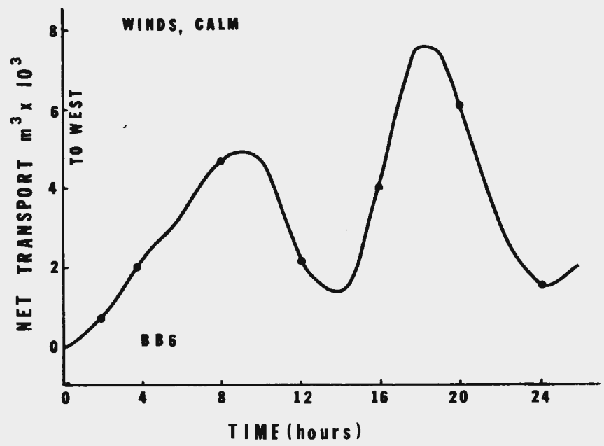
Figure 66 Transport rate through section BB6 in surface layer in calm and with SW wind 9m/sec.
