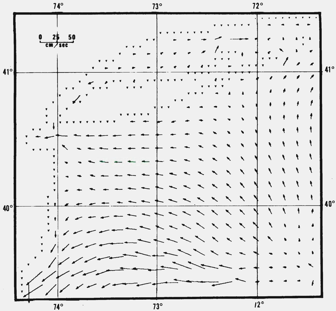
Figure 19 Currents during 2 hours before high water at Sandy Hook
