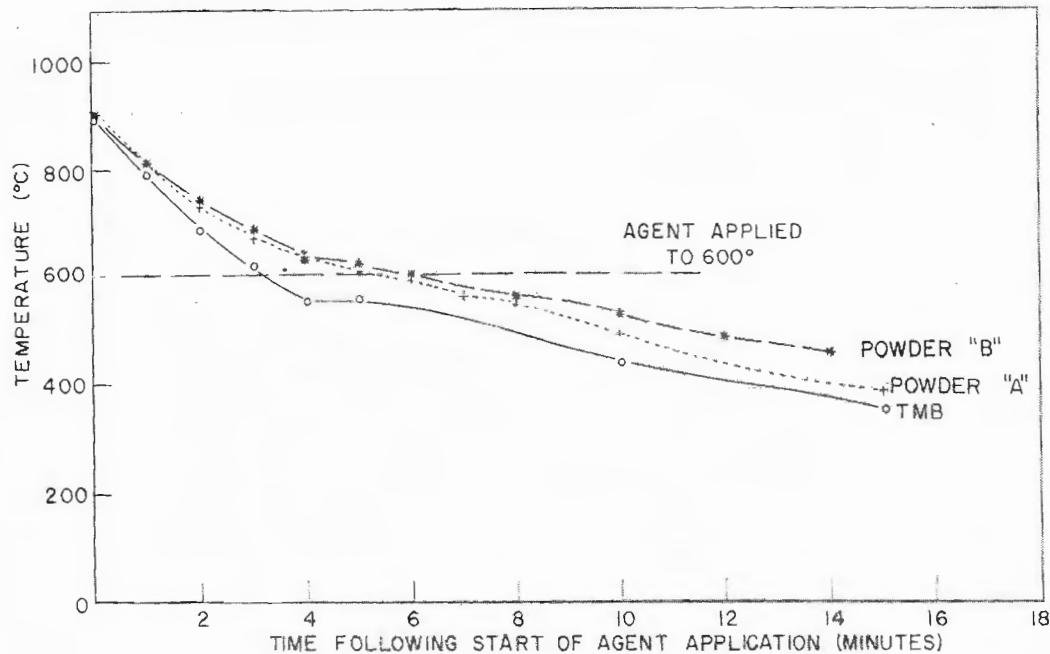
Fig. 6 - Cooling curves for powder agents and TMB application on small-scale fire test with Dowmetal "C"
