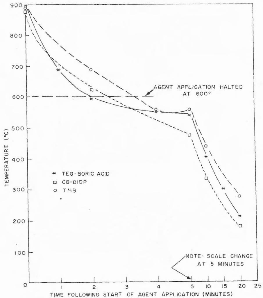
Fig. 5 - Averaged cooling curves for liquid agent application on small-scale fire test with Dowmetal "C"
