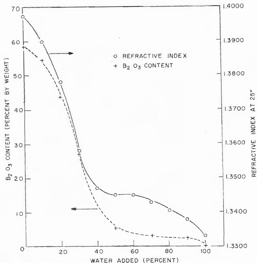
Fig. 8 - Variation in B_2O_3 content and refractive index of TMB on addition of water
