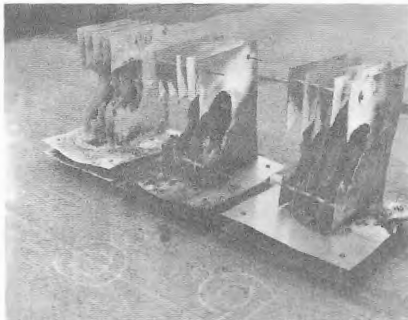
Fig. 12 - Extinguished standard magnesium sheets
