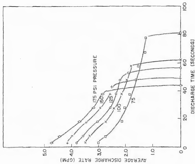
Fig. A2 - TMB discharge rate for varied initial charging pressures with prototype extinguisher - 72°F
