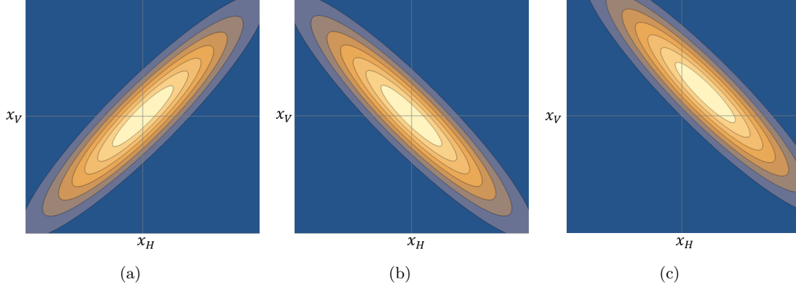
Figure 5.1: (a) The theoretical position joint-probability distribution of the biphoton in the plane of the crystal, where it shows strong positive correlations. (b) The spatial distribution after the H photon is reflected twice while the V photon is reflected three times. The extra reflection flips the distribution about the x -axis. (c) The distribution after being displaced by the moving mirror; note that it shifts along the narrow axis of the final joint spatial distribution.
