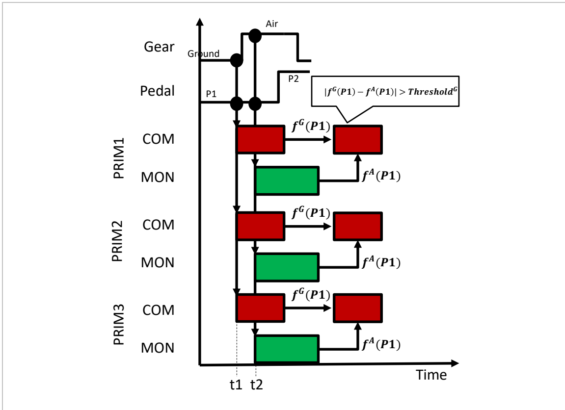
Figure 2: Channel Asynchronism Timeline
