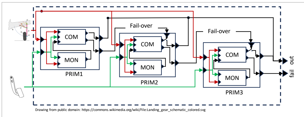
Figure 1: Airbus A330 Flight Control Architecture
