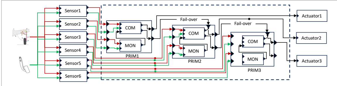
Figure 4: All Independent Channel Threads
