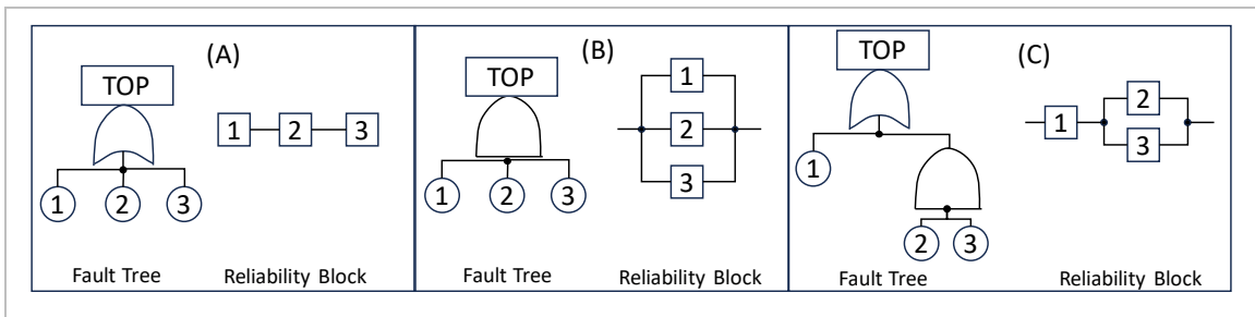
Figure 5: Fault-Tree and Reliability Block Diagrams
