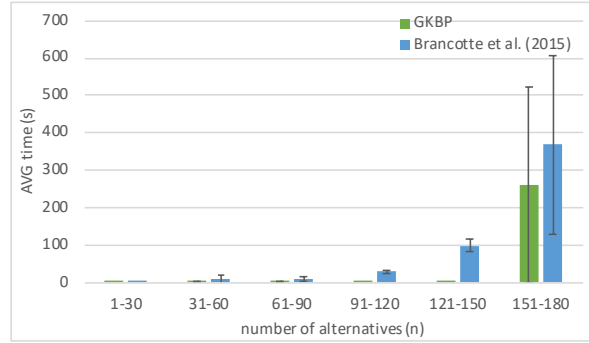
Figure 4.9: The Computing Time of GKBP and ?'s Formulation
