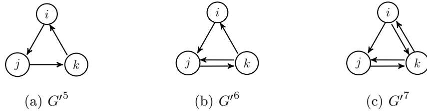
Figure 4.3: Unicyclic Graphs
