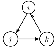
(a) Example of an unweighted directed graph
