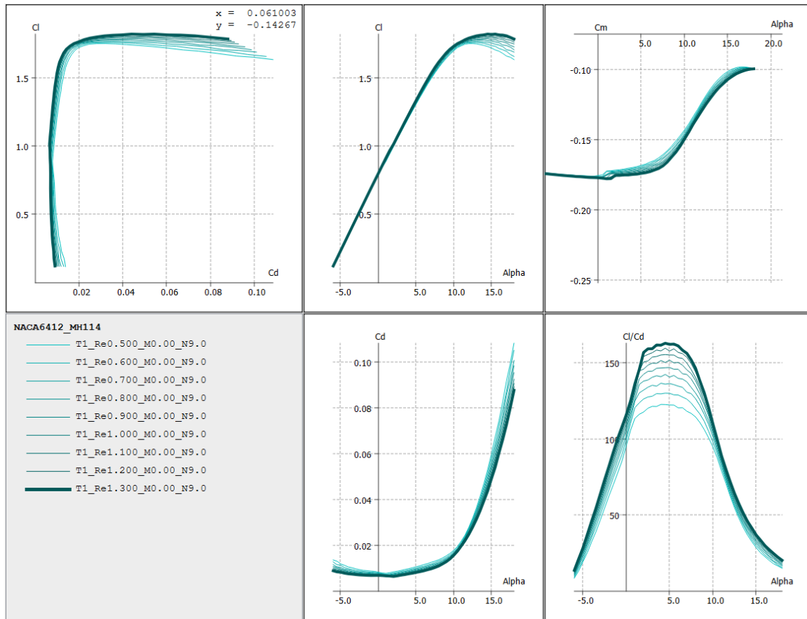
Figure 14. Polars of the NACA-6412-MH114 airfoil generated in Flow5
