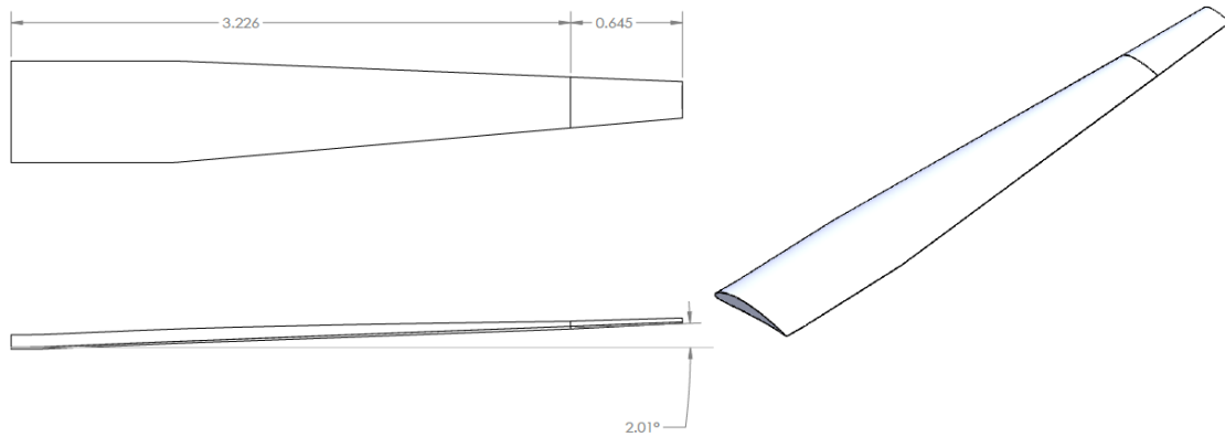
Figure 42. Half of the UAV wing with 10% wing extension. Dimensions are in meters.
