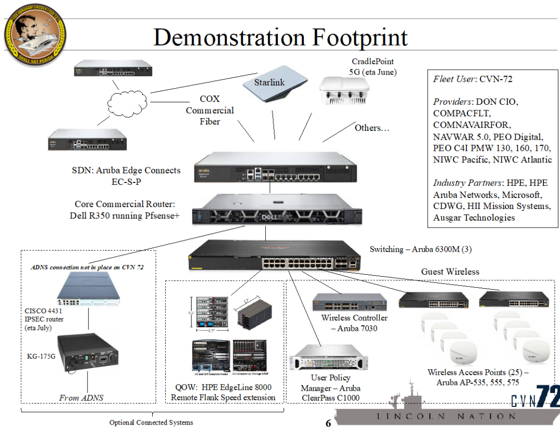
Figure 1. CVN-72 Private Wi-Fi Network Infrastructure. Source: K. White (email to authors, June 11, 2023).
