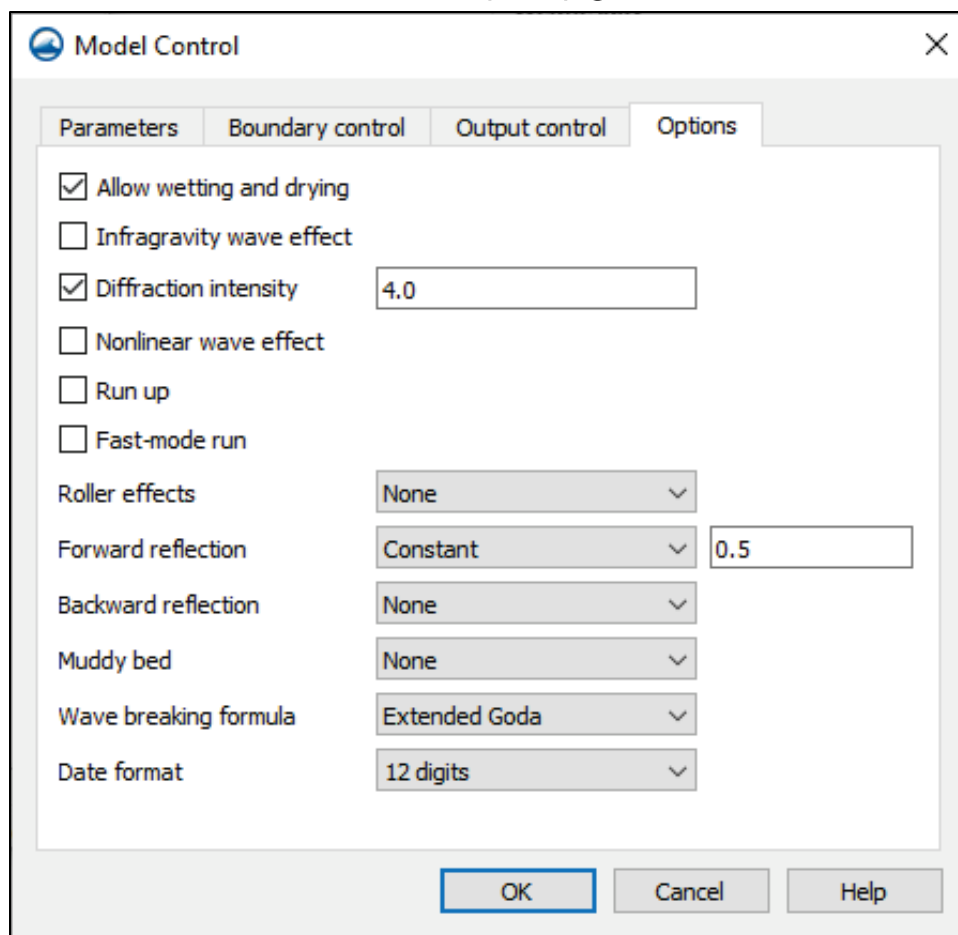
Figure 9-23. Model Control dialog window. Display CMS-Wave simulation Options page.
