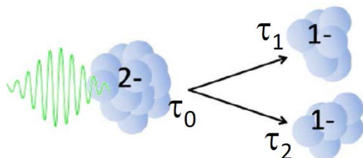
Fig. 1: Schematic of time-resolved photofission study. Decay and appearance constants ( \tau_{0,1,2} ) are observed to match.
