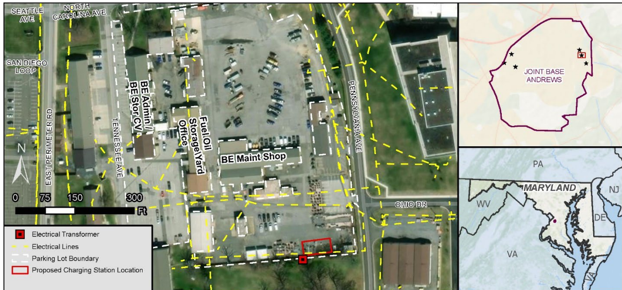
Figure 2-3c. JBA CE Yard Parking Lot
