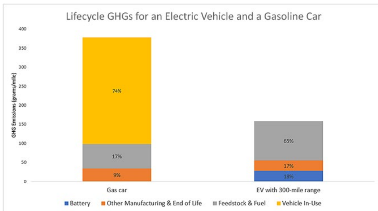
Figure 3.1.3. Lifecycle GHGs for EV and Gasoline Cars
