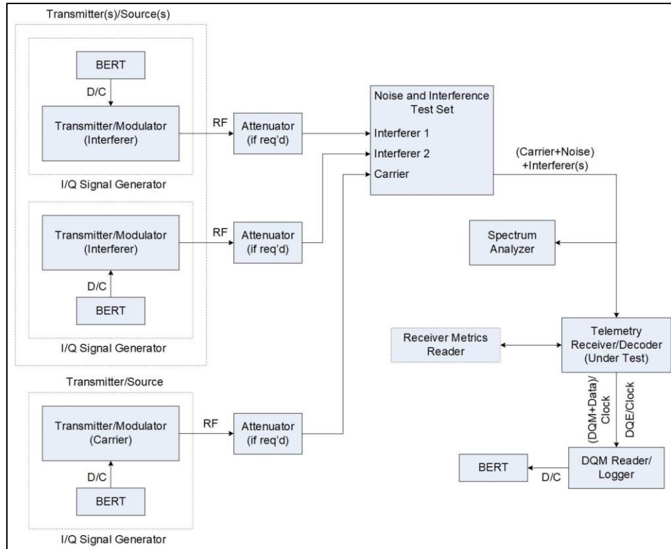
Figure 11-8. Setup for ACI Test using Noise and Interference Test Set
