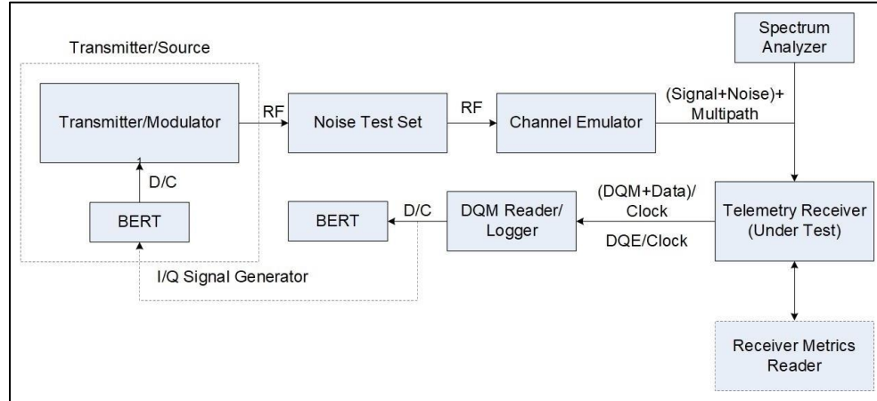
Figure 11-11. Setup for Static 3-ray Multipath Channel Conditions using Channel Emulator
