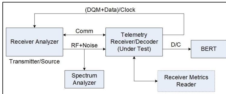
Figure 11-3. Setup using Receiver Analyzer for BER versus BEP Test
