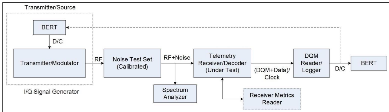
Figure 11-2. Setup using Noise Test Set for BER versus BEP Test
