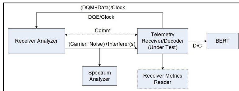
Figure 11-9. Setup for ACI Test using Receiver Analyzer
