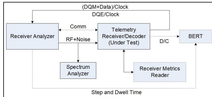
Figure 11-6. Setup for Step and Dwell Test using Receiver Analyzer
