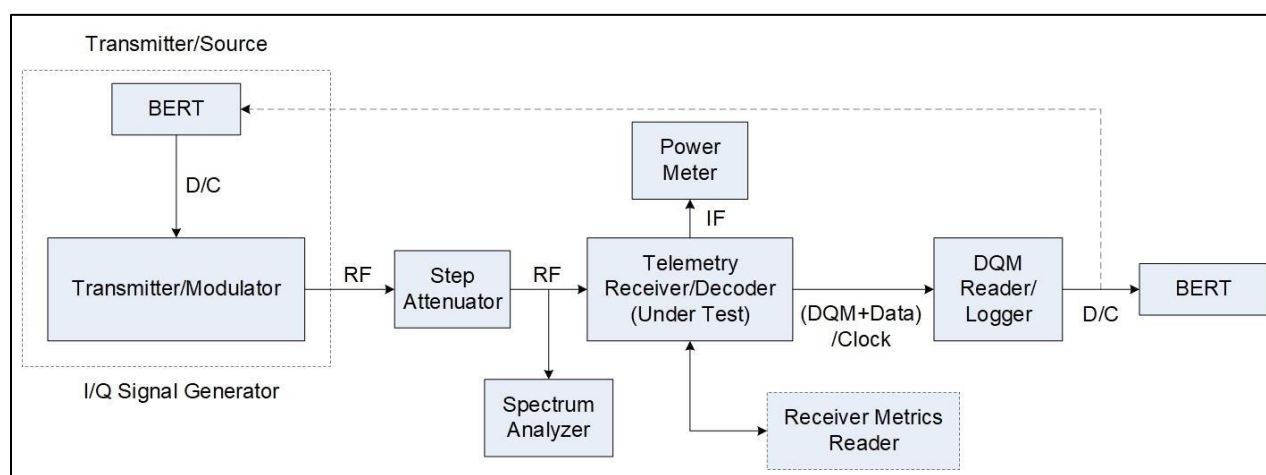
Figure 11-1. Setup for Step Attenuator/Power Meter for BER versus BEP Test
