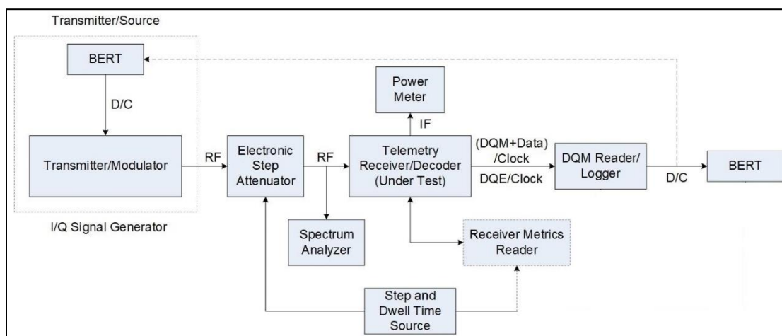
Figure 11-4. Setup for Step and Dwell Testing using Step Attenuator/Power Meter
