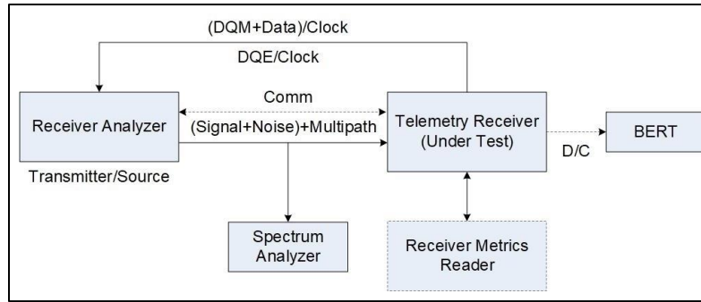
Figure 11-12. Setup for Static 3-ray Multipath Channel Conditions using Receiver Analyzer
