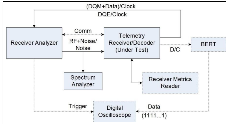
Figure 11-16. Setup for Resynchronization Response using Receiver Analyzer
