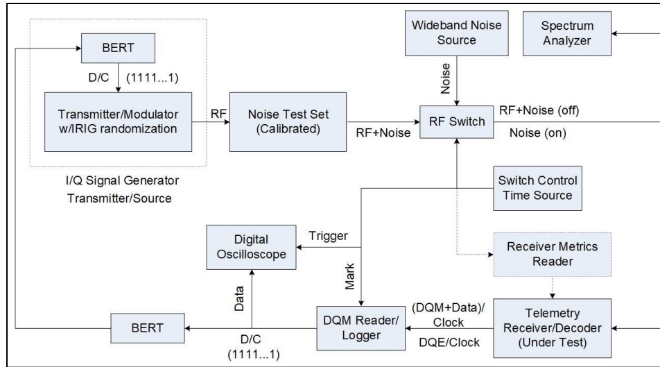
Figure 11-15. Setup for Resynchronization Response using Noise Test Set
