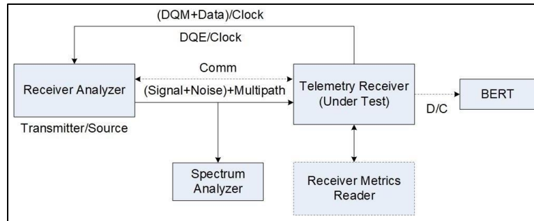
Figure 11-14. Setup for Static 2-ray Multipath Channel Conditions using Channel Emulator
