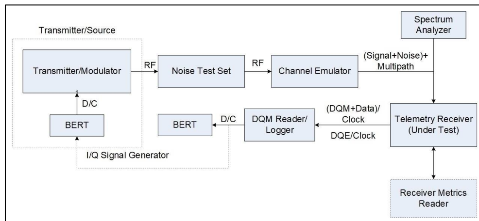
Figure 11-13. Setup for Static 2-ray Multipath Channel Conditions using Channel Emulator
