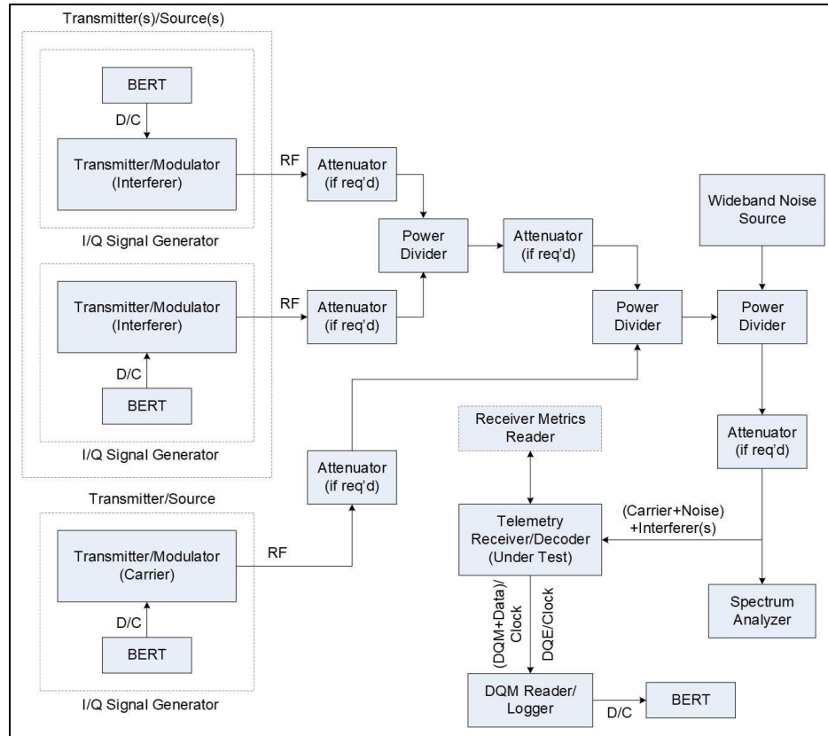
Figure 11-7. Setup for ACI Test using Discrete Components
