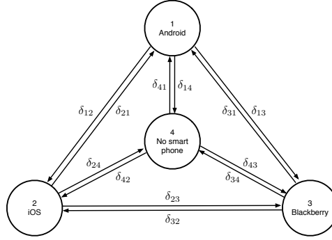
Figure 2.2: An example of the product-conversion graph for different smart phone operation systems. The self loops exist but are not displayed in this graph.
