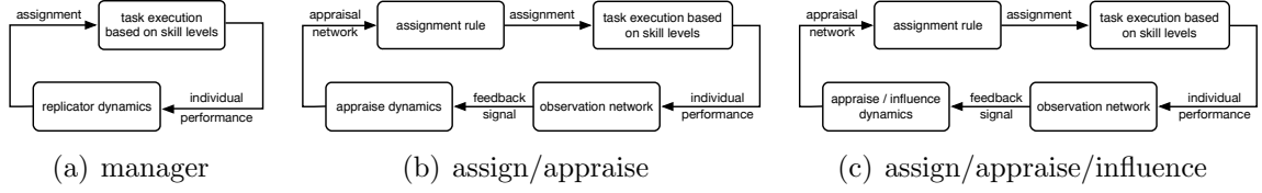
Figure 4.1: Diagram illustrations of manager dynamics, assign/appraise dynamics, and assign/appraise/influence dynamics.
