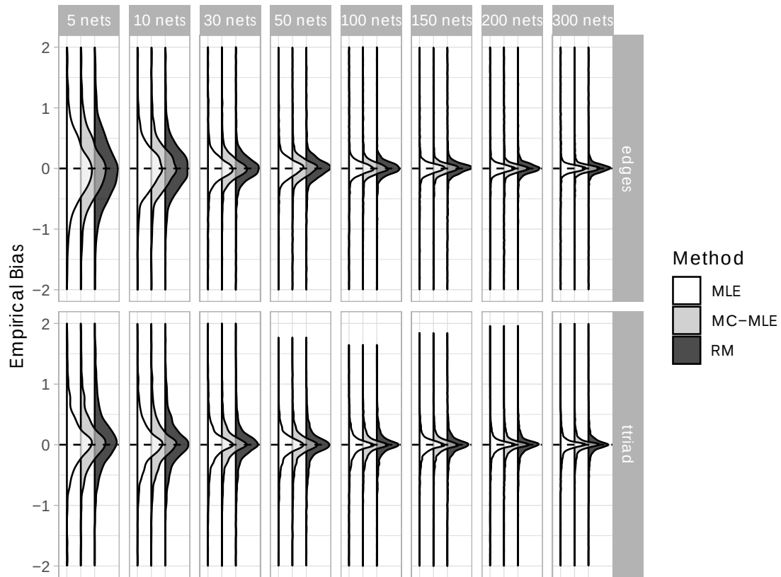
Figure 5.6: Empirical distribution of the bias per model parameter, for MC-MLE and MLE estimation methods. In general we see that the parameter estimates' bias is centered around zero and both MC-MLE (ERGM) and MLE (ERGMito) have about the same bias in our simulation study.
