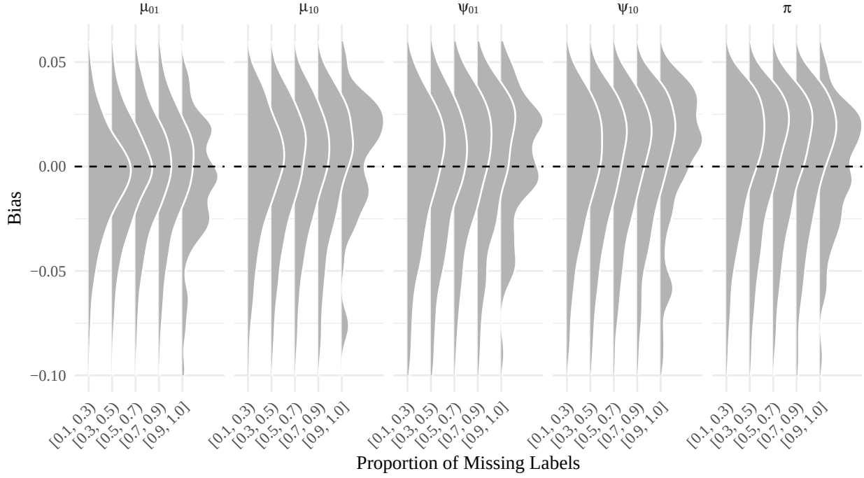
Figure 2.8: Empirical bias distribution for the partially annotated scenario by parameter and proportion of missing labels.
