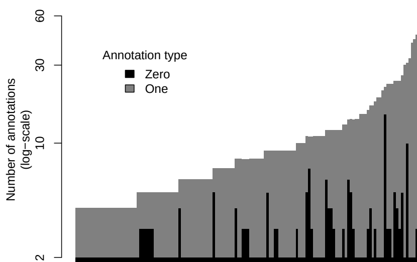
Figure 2.2: Number of annotated leaves for all 141 trees by type of annotation. Most of the annotations available in GO are positive assertions of function, that is, 1s. Furthermore, as observed in the figure, all of the trees used in this study have two “Not” (i.e., 0) annotations, which is a direct consequence of the selection criteria used, as we explicitly set a minimum of two annotations of each type per tree+function.
