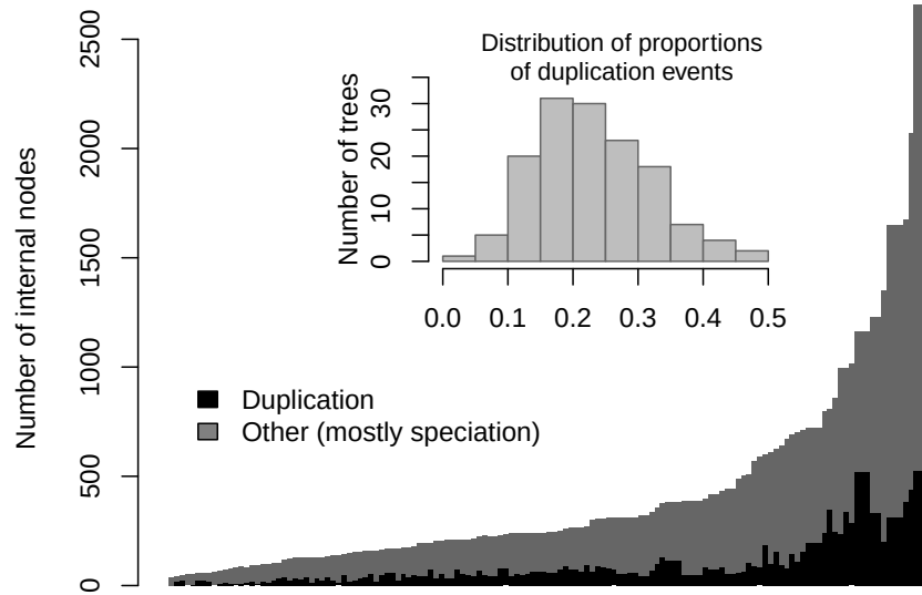
Figure 2.3: Number of internal nodes by type of event. Each bar represents one of the 141 trees used in the paper by type of event (mostly speciation). The embedded histogram shows the distribution of the prevalence of duplication events per tree. The minority of the events, about 20%, are duplications.
