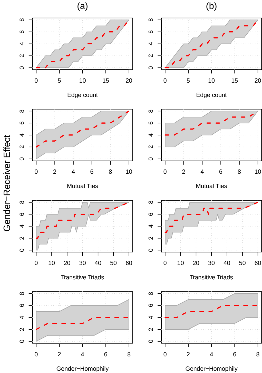
Figure 6.6: Conditional distribution of the value of the gender-receiver effect sufficient statistic. Column (a) shows the distribution under the Bernoulli model, this is, the parameter of receiver-effect is set to zero, whereas column (b) shows the distribution of the statistic assuming its parameter equals one.
