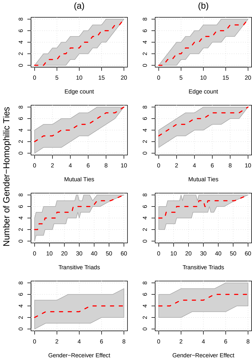
Figure 6.4: Conditional distribution of the number of gender homophilic ties sufficient statistic. Column (a) shows the distribution under the Bernoulli model, this is, the parameter of homophily is set to zero, whereas column (b) shows the distribution of the statistic assuming its parameter equals one.
