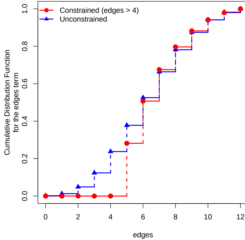
Figure 5.10: Marginalized Cumulative Distribution Function (CDF) for the edges sufficient statistic for a network of size 4 (up to 12 ties). The blue line shows the CDF for the edges term according to model (1) in Table 5.9, which was fitted without constraining the support of the sufficient statistics, while the red line shows the CDF of model (2), also in Table 5.9, which constrained the support to networks with at least 5 ties. Once again, since we can fully enumerate the support, both CDFs are exact, and thus, not simulated.
