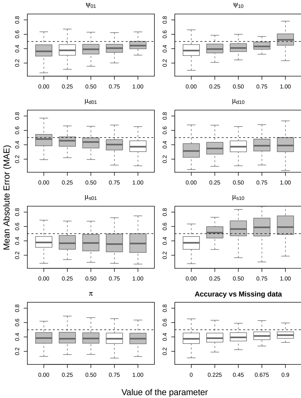
Figure 2.1: Sensitivity analysis. Boxplots of MAEs as a function of single parameter updates. The first seven plots show how the MAEs change as a function of fixing the given parameter value ranging from 0 to 1. In each of these plots, the white box indicates the parameter value used to generate the data (i.e., the “correct” parameter value). The last boxplot shows the distribution of the MAEs as a function of the amount of available annotation data, that is, how accuracy changes as the degree of missing annotations increases.
