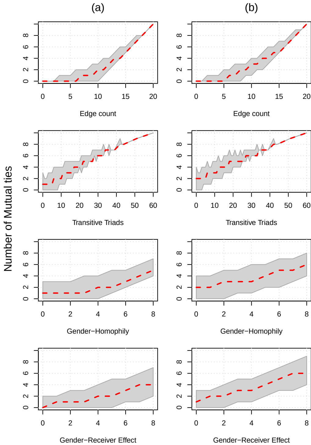
Figure 6.3: Conditional distribution of the number of mutual ties sufficient statistic. Column (a) shows the distribution under the Bernoulli model, this is, the parameter of mutual ties is set to zero, whereas column (b) shows the distribution of the statistic assuming its parameter equals one.
