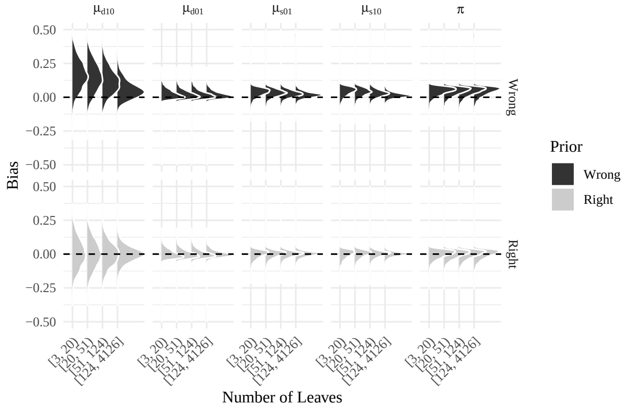
Figure 2.7: Empirical bias distribution for the Fully annotated scenario by type of prior, parameter, and number of leaves.
