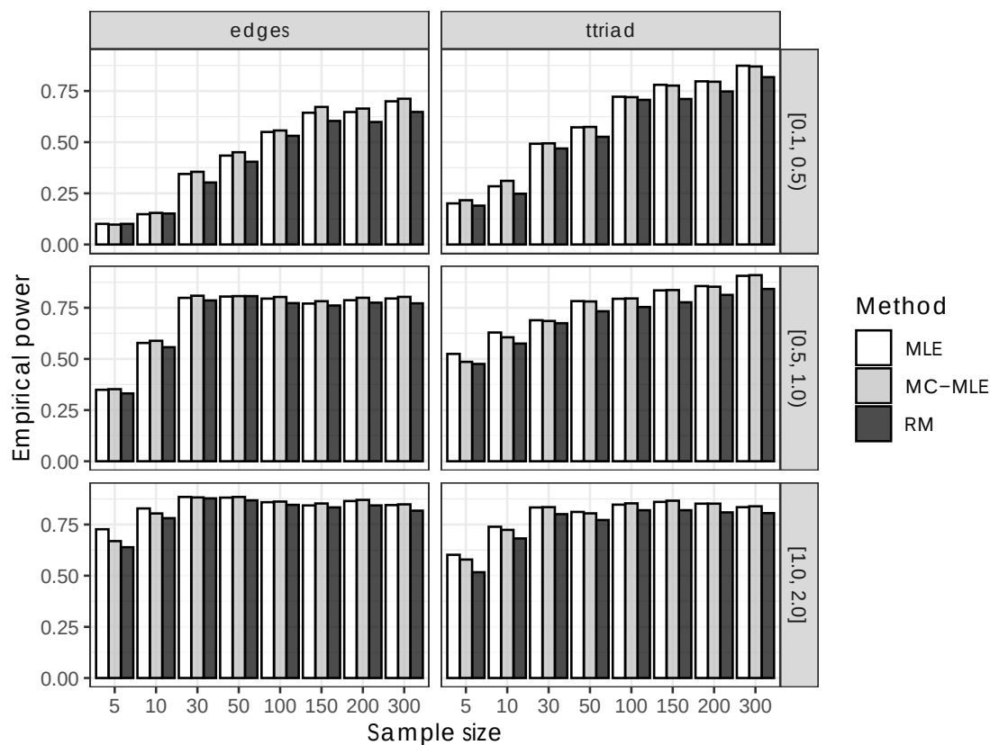
Figure 5.7: Empirical power by dataset size and effect size (the later considering only magnitude), for ERGM and ERGMito estimation methods. Power increases for both MC-MLE (ERGM) and MLE (ERGMito) with increases in the size of the dataset and effect size. There are indistinguishable differences in power between the two estimation methods.
