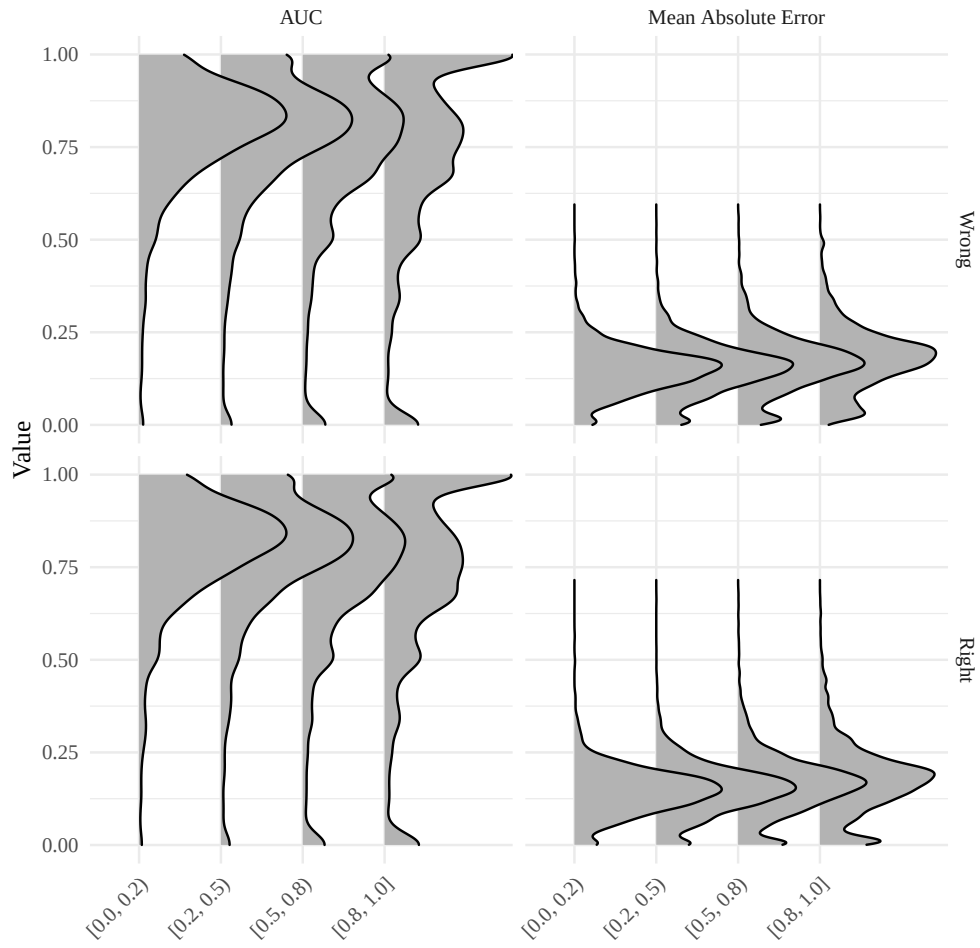
Figure 2.6: Distribution of AUCs and MAEs for the scenario with partially annotated trees and mislabeling. The x-axis shows the proportion of missing annotations, while the y-axis shows the score (AUC or MAE).
