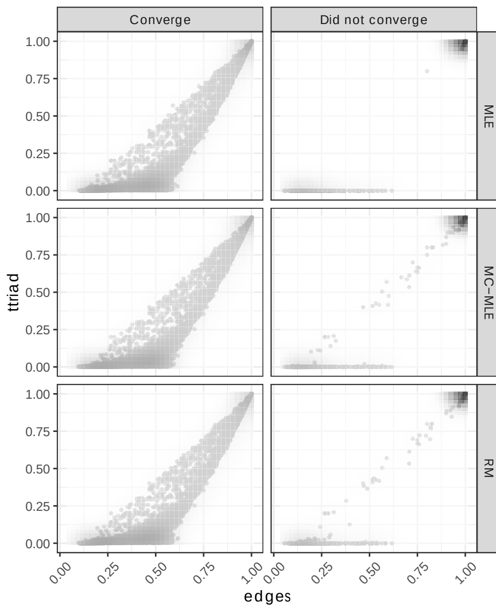
Figure 5.5: Distribution of the average sufficient statistics per sample. Since samples can contain networks of sizes four and five, we have re-scaled the sufficient statistics counts by each network size's corresponding maximum value so these range from zero to one. Most of the cases in which methods failed to converge happened in scenarios where either all the graphs in the sample were fully connected or there was no transitive triad; exactly the cases that we excluded for the reminder of the analysis.
