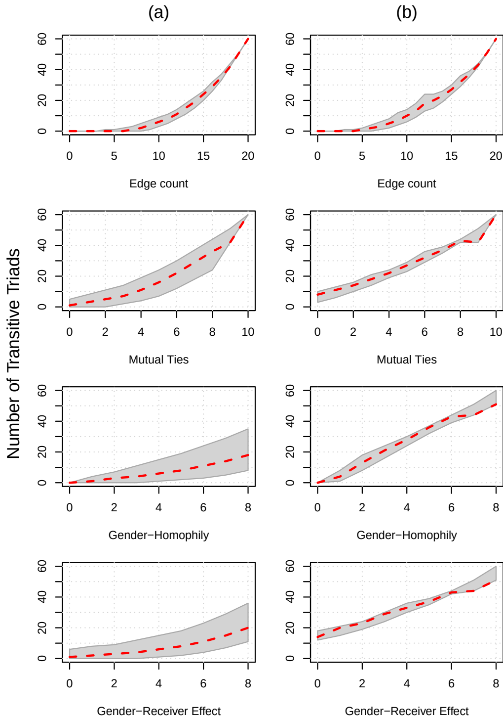
Figure 6.5: Conditional distribution of the number of transitive triads sufficient statistic. Column (a) shows the distribution under the Bernoulli model, this is, the parameter of transitivity is set to zero, whereas column (b) shows the distribution of the statistic assuming its parameter equals one.
