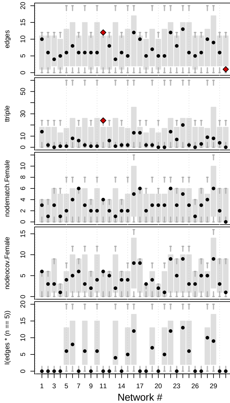
Figure 5.11: Distribution of the sufficient statistics under the ERGM specified by the parameters from model (4) in Table 5.9. Each bar represents the exact 95% confidence interval for the corresponding network+term combination, while the black dots show the location of the corresponding observed statistic. Red diamonds mark the observed statistics that fall out of the 95% confidence interval. Of the 31 networks in the sample, it is only in two networks that the CIs don't cover the observed statistic, one that is fully connected and another that only has one tie.
