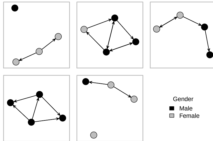
Figure 5.2: Fivenets data set. These graphs were randomly drawn from an ERGM distribution with two parameters: number of edges and gender homophily, with parameters equal to -2.0 and 2.0 respectively.
