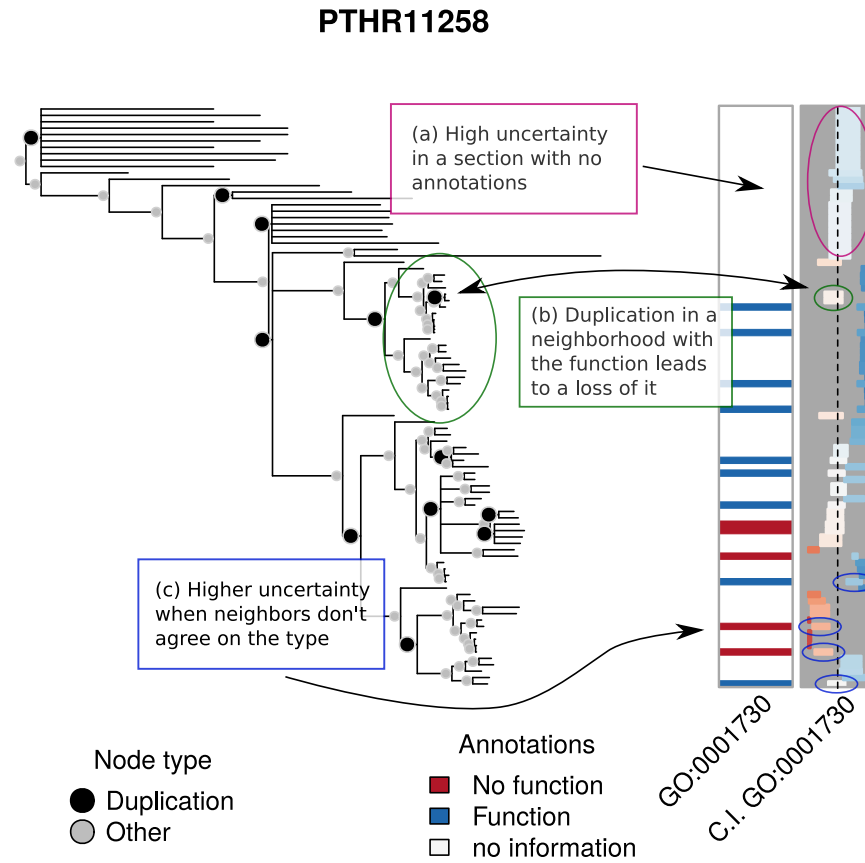
Figure 2.4: High accuracy predictions The first set of annotations, first column, shows the experimental annotations of the term GO:0001730 for PTHR11258. The second column shows the 95% C.I. of the predicted annotations. The column ranges from 0 (left end) to 1 (right-end). Bars closer to the left are colored red to indicate that lack of function is suggested, while bars closer to the right are colored blue to indicate function is suggested. Depth of color corresponds to strength of inference. The AUC for this analysis is 0.91 and the Mean Absolute Error is 0.34.
