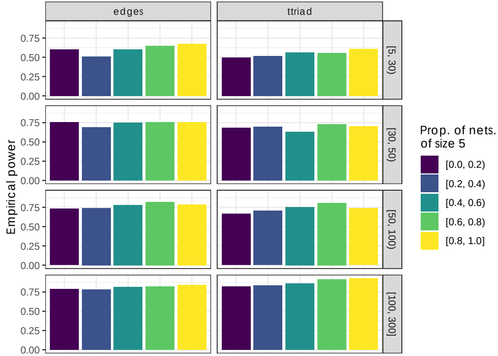
Figure 5.8: Empirical power by proportion of networks of size five in the sample (color coded) and sample size (rows).
