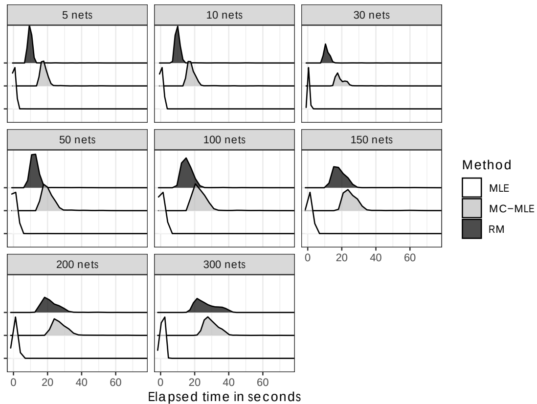
Figure 5.9: Distribution of elapsed time (in seconds) for the estimation process for MC-MLE (ERGM) versus MLE (using ERGMito ). Overall, the MLE implementation is orders of magnitude faster compared to the time required by the MC-MLE implementation to do the parameter estimation.
