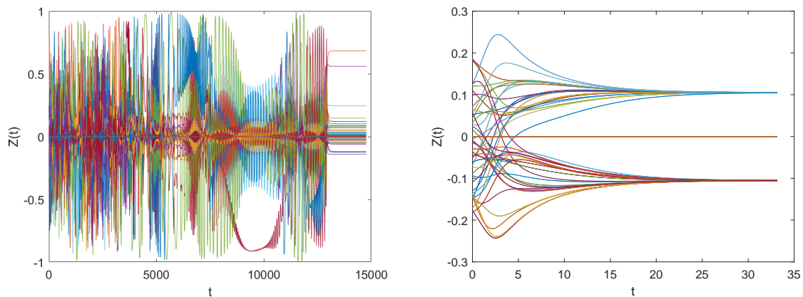
(a) Projected pure-influence model (1.9) with generic asymmetric initial condition
