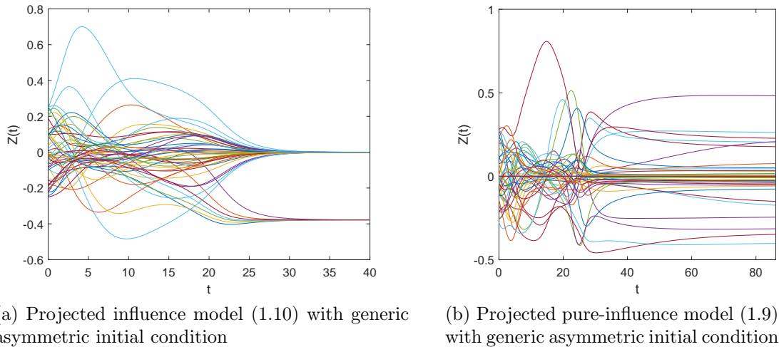
Figure 1.5: Convergence comparison for a network of size n = 7 (a) with and (b) without the consideration of self-appraisals. The setting is the same one as in Figure 1.4, but with a different random initial condition. (a) converged to a network with only diagonal negative entries (all interpersonal appraisals go to zero), whereas (b) converged to structural balance.
