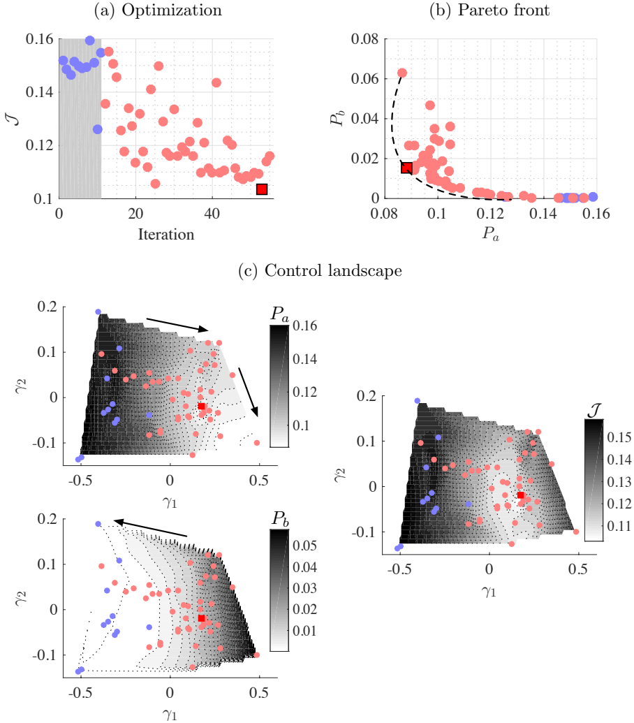
Figure 38: (a) Objective function minimization to determine the optimized control law and (b) Pareto front. The red square symbol denotes the optimized case. The dashed line in (b) indicates the Pareto front of control. (c) Control objective landscape, P_a = P_a(\gamma_1, \gamma_2) , P_b = P_b(\gamma_1, \gamma_2) , and \mathcal{J} = \mathcal{J}(\gamma_1, \gamma_2) balancing P_a and P_b , all three determined using multidimensional scaling. The transparent blue dots indicate initial simplex control cases. The arrows indicate directions of minimization.
