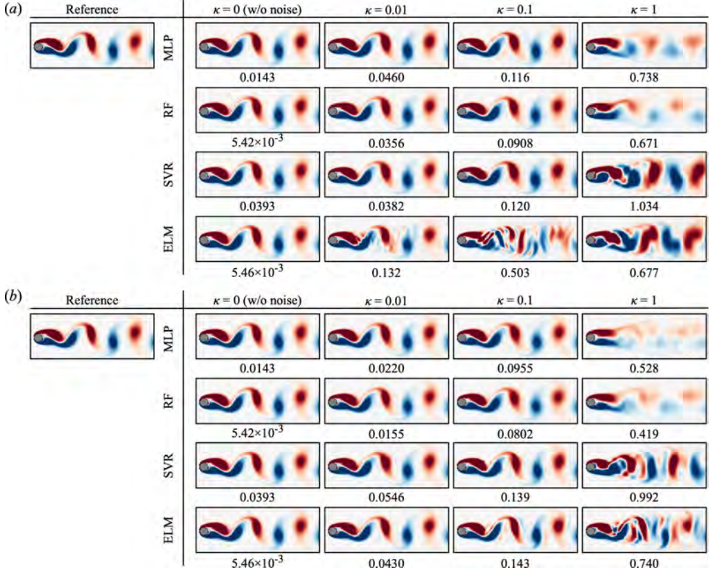
Figure 81: The reconstructed vorticity fields of cylinder wake from five noisy surface-sensor measurements ( \mathbf{s} + \kappa \mathbf{n} ). The values listed underneath each flow field represent the L_2 error norms. (a) Without noise addition and (b) with noise addition in training data.
