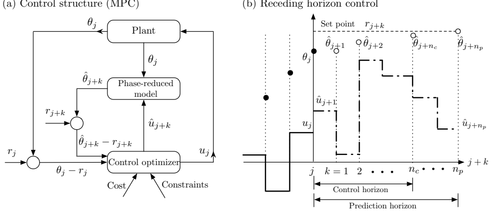
Figure 57: (a) Schematic of model-predictive control (MPC) structure and (b) receding horizon framework (adapted from Kaiser et al. (2018)).
