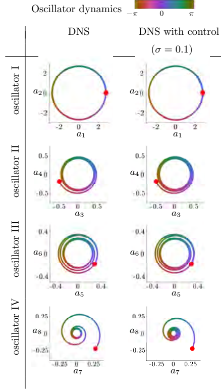
Figure 30: Oscillator dynamics without control and with control implemented in DNS for suppressing perturbations to limit cycle.
