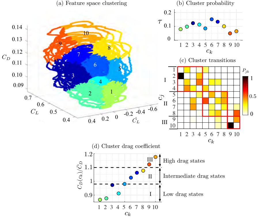
Figure 41: (a) Feature space clustering of 3D baseline flow data. (b) Cluster probabilities, (c) transitions probabilities and (d) normalized, average drag coefficient across clusters. The red boxes and the dashed circles indicate the cluster subsets.
