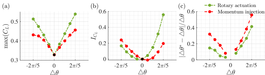
Figure 53: Comparison of control performance for rotary actuation and momentum injection: (a) Maximum lift coefficient, (b) lift impulse and (c) error in asymptotic phase shift for varying desired phase shifts.
