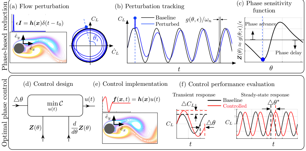
Figure 47: Overview of phase reduction analysis: (a) Introduction of impulse flow perturbation, (b) baseline and perturbed lift coefficient trajectories (left: phase portrait of oscillations in \dot{C}_L - C_L plane, right: time history) and (c) phase sensitivity function \mathbf{Z}(\theta) . Overview of energy-optimal phase control: (d) Design of optimal control input u(t) for desired phase shift \Delta\theta and (e) controlled flow with the forcing \mathbf{f}(t) , (f) transient and steady-state response of lift coefficient on application of control.
