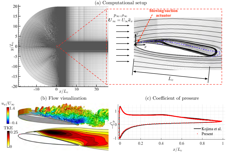
Figure 34: (a) Computational domain, x - y plane (left) and near field of a NACA 0012 airfoil at an angle of attack of \alpha = 9^\circ (right) indicating the streamlines for 3D spanwise-periodic baseline flow. The actuator surface is indicated in red. The blue dashed line indicates contour line corresponding to \bar{u}_x/U_\infty = 0 . (b) Instantaneous flow field (highlighted by Q-criterion) colored by streamwise velocity and turbulent kinetic energy (TKE) and (c) time-averaged coefficient of pressure distribution on suction and pressure side of the airfoil for 3D baseline flow.
