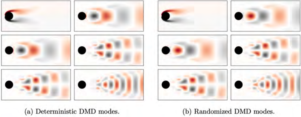
Figure 62: Leading dynamic modes extracted from the fluid flow behind a cylinder.
