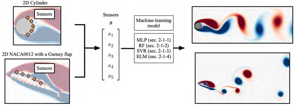
Figure 79: Wake reconstruction using machine learning with five surface-sensor measurements.
