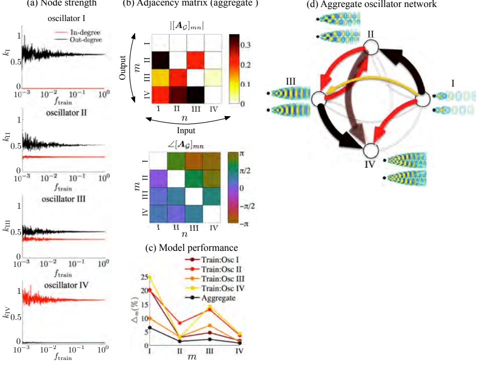
Figure 25: (a) Network degrees for varying fractions of training data. (b) Adjacency matrix of the aggregate network model and (c) the associated model performance. (d) Aggregate network structure of oscillator interactions. The color and thickness of the edges in the network represent the magnitude of the elements of \mathbf{A}_G .
