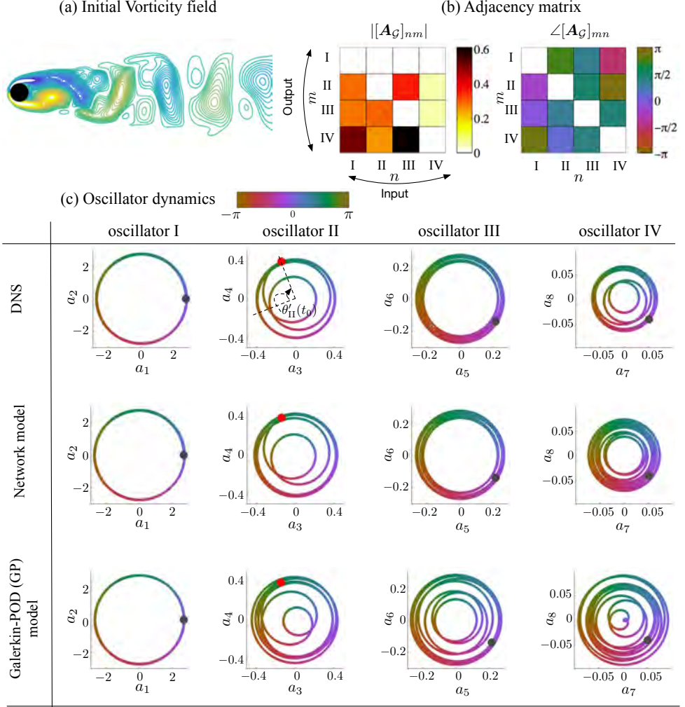
Figure 23: Phase perturbation introduced at oscillator II. (a) Initial vorticity field corresponding to phase perturbation, (b) Adjacency matrix of networked oscillator model. (c) Dynamics of DNS, networked oscillator model and Galerkin-POD model (color of oscillators indicates phase). Red dot indicates perturbed state.
