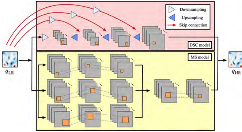
Figure 86: The two-dimensional hybrid downsampled skip-connection/multi-scale (DSC/MS) model.
