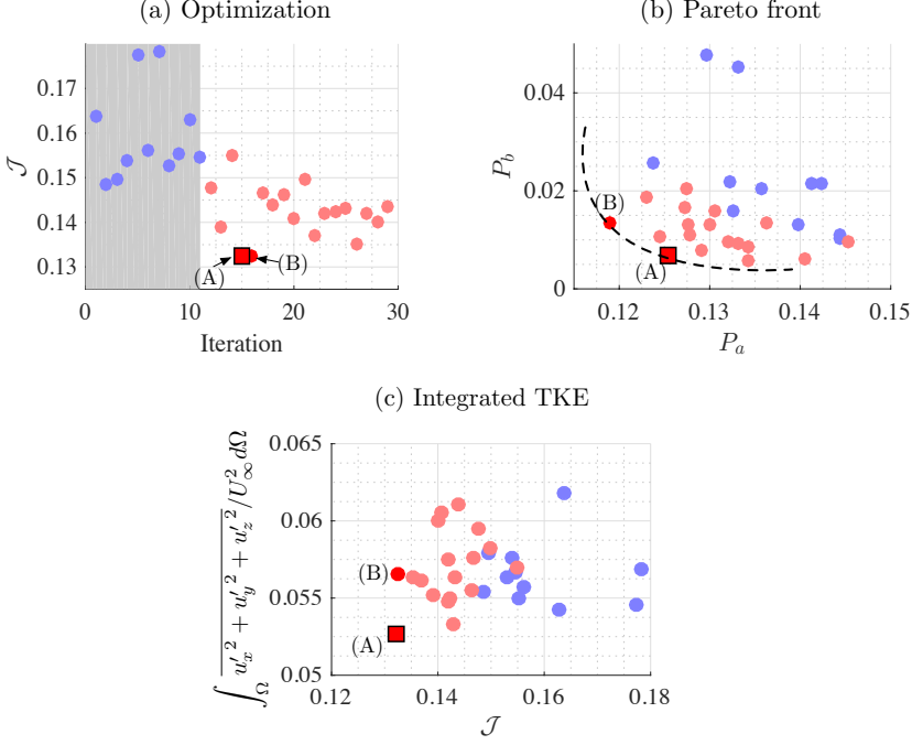
Figure 43: (a) Objective function \mathcal{J} minimization to determine the optimized control case, and (b) Pareto front ( P_a, P_b ). The square symbol denotes the optimized case. (c) Integrated turbulent kinetic energy over the entire computational domain. The transparent blue dots indicate initial simplex control cases and the red square symbol denotes the optimized case.
