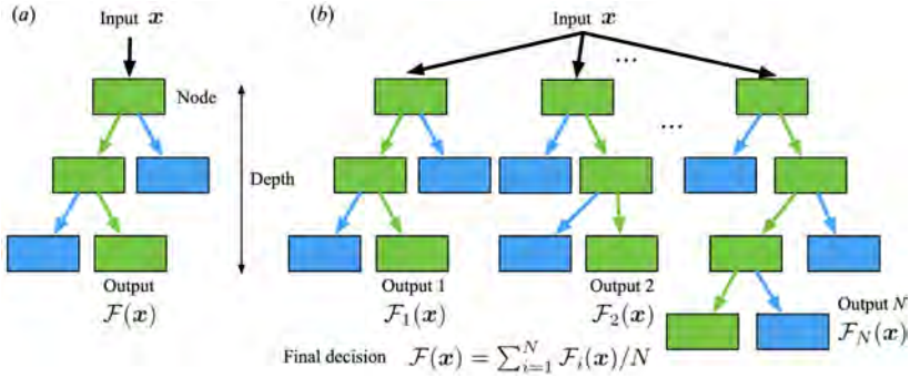
Figure 70: (a) Decision tree. (b) Random forest, which can be regarded as ensemble average of decision trees.
