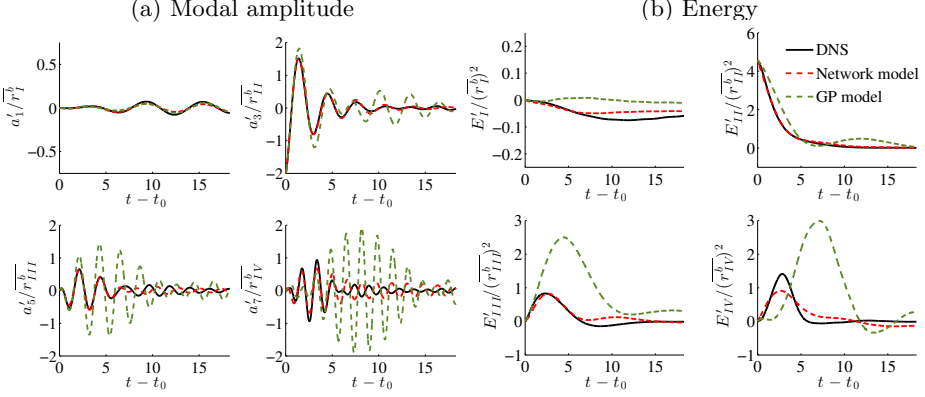
Figure 22: (a) Modal amplitude and (b) energy tracking for amplitude perturbation introduced at oscillator II.
