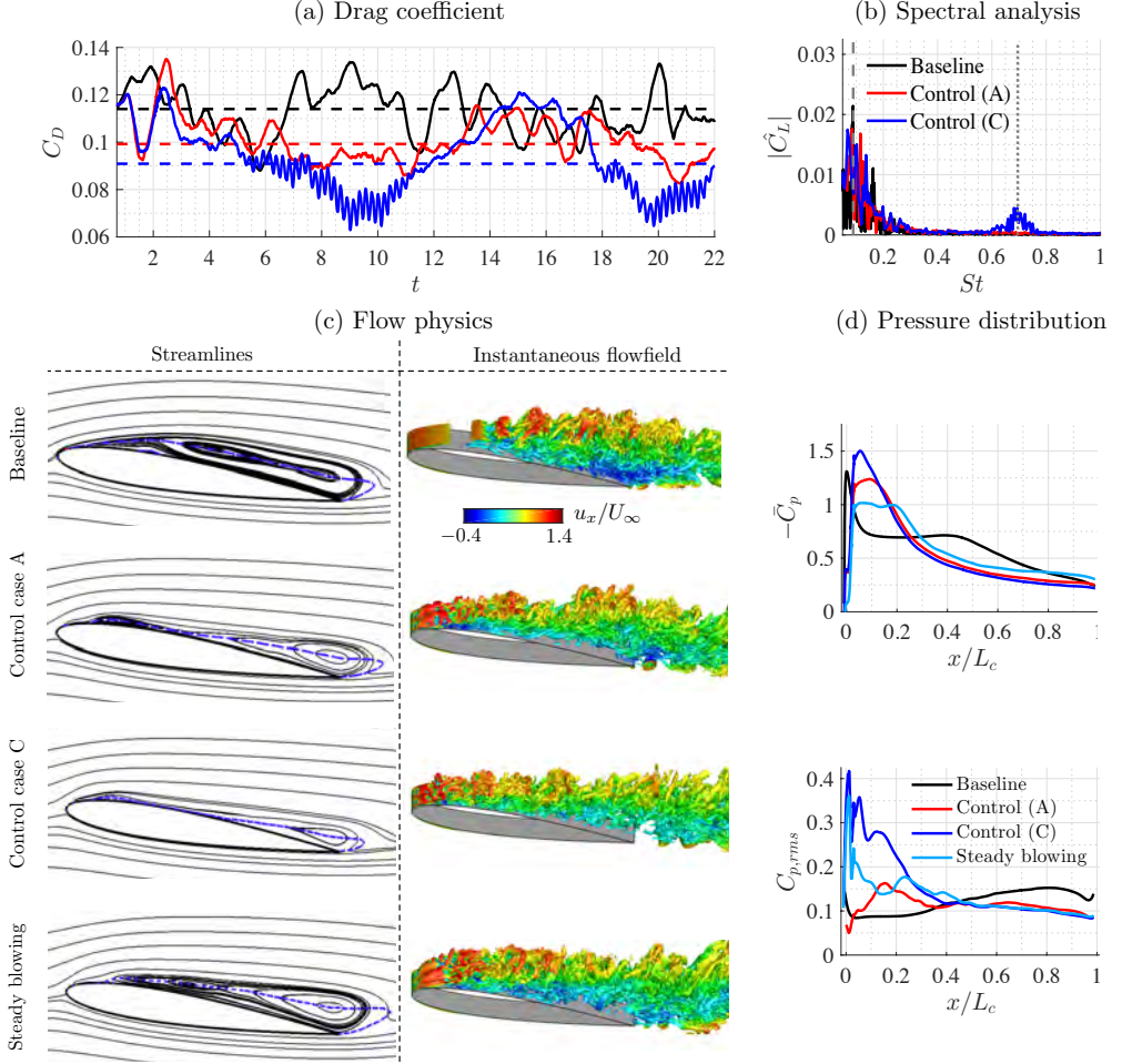
Figure 45: Comparison of baseline, optimized control case A and control case C with higher feedback gain: (a) Drag coefficient, (b) spectral analysis of lift data, (c) time-averaged streamlines and instantaneous flow field (highlighted by Q-criterion) colored by streamwise velocity, and (d) time-averaged and root-mean square fluctuation of coefficient of pressure distribution on suction side of the airfoil. The dashed lines in (a) indicate the mean drag. The dashed line in (b) corresponds to the dominant shedding frequency and dotted line corresponds to the shear layer frequency. The blue dashed line in (c) indicates the contour line of zero time- and spanwise-averaged streamwise velocity.
