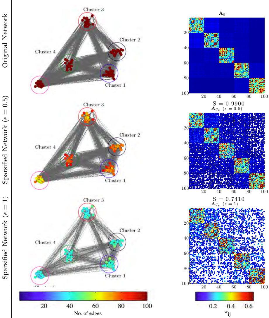
Figure 3: Original and sparsified graphs and their respective sparsity patterns of the adjacency matrix for N = 100 vortices. The color of the nodes of the vortex network represents the unweighted connections (number of connected edges) of the individual point vortices. The color in the sparsity patterns of the adjacency matrix indicates the adjacency weights w_{ij} for original graph \mathbf{A}_G and \tilde{w}_{ij} for sparse graphs \mathbf{A}_{G_S} . The empty white spaces indicate sparsity in the adjacency matrix. Sparsity index is S \equiv n_{\text{non-zero}}/N^2 , where n_{\text{non-zero}} is the number of non-zero weights (elements) in adjacency matrix and N is the number of vortices. The colored circles in the vortex network represent the individual cluster groups.
