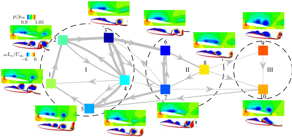
Figure 36: Graph of Markov chain highlighting transitions between clusters. 2D cluster-averaged pressure flow fields ( p/p_\infty ) and instantaneous vorticity contours ( \omega L_c/U_\infty ) corresponding to each cluster are shown. The dashed circles indicate the cluster subsets.
