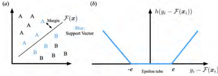
Figure 71: (a) Support vector machine with two-group classification. (b) The concept of epsilon tube.
