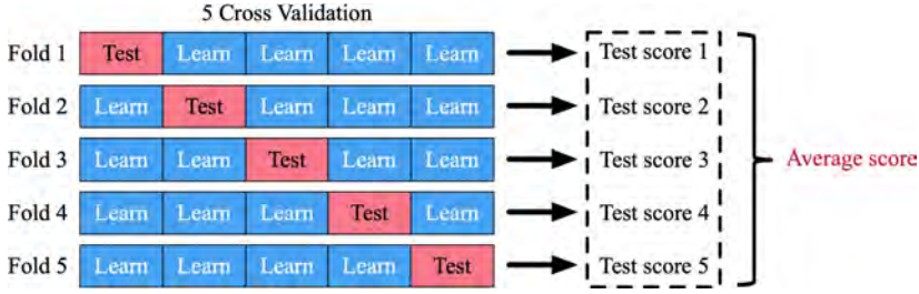
Figure 73: An example of five-fold cross validation. The blue boxes indicate training data used for deriving machine learning model. The red boxes indicate test data used to obtain test scores. An average score of five test scores are used for the optimization procedure and assessment.
