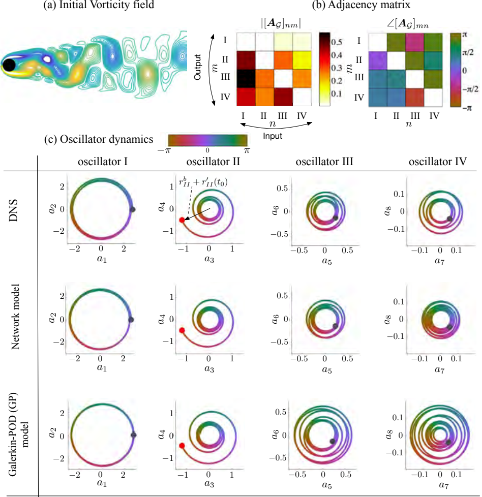
Figure 21: Amplitude perturbation introduced at oscillator II. (a) Initial vorticity field corresponding to amplitude perturbation, (b) Adjacency matrix of networked oscillator model. (c) Oscillator dynamics from DNS, networked oscillator model and Galerkin-POD model (color of temporal dynamics of oscillators indicates phase). Red dot indicates the initial perturbation.
