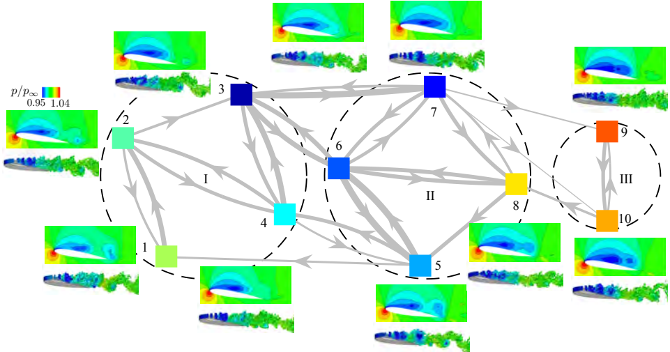
Figure 42: Graph of Markov chain highlighting transitions between clusters for the 3D baseline flow. The dashed circles indicate the cluster subsets.
