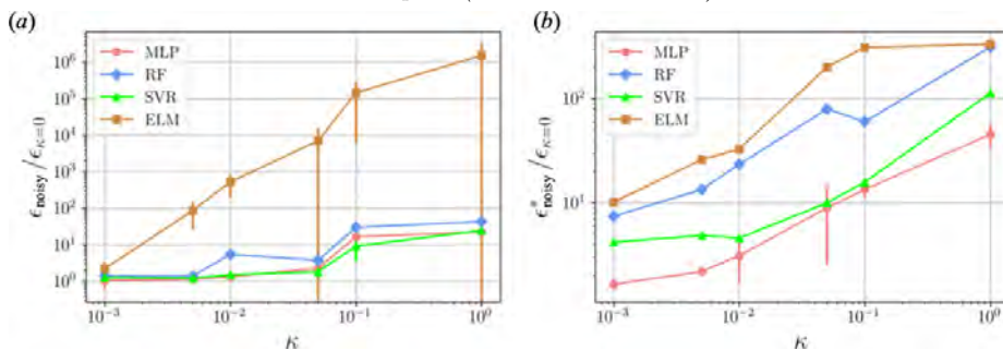
Figure 82: The L_2 error norms of the four machine-learned models over varied noise level \kappa . The error levels are normalized by the error level without noise added to training data. (a) Without noise addition and (b) with noise addition in training data.
