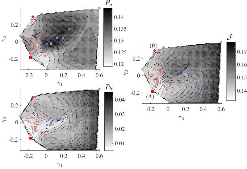
Figure 44: Control landscape, P_a = P_a(\gamma_1, \gamma_2) , P_b = P_b(\gamma_1, \gamma_2) , and \mathcal{J} = \mathcal{J}(\gamma_1, \gamma_2) , using multidimensional scaling. The transparent blue dots indicate initial simplex control cases and the red square symbol denotes the optimized case.
