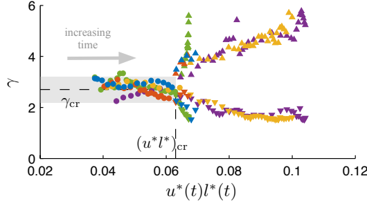
Figure 17: Exponent \gamma for the network strength distribution P(s) \sim s^{-\gamma} plotted over u^*(t)l^*(t) with different initial Reynolds numbers (green: Re(t_0) = 75 , purple: Re(t_0) = 439 , yellow: Re(t_0) = 814 , red: Re(t_0) = 1607 , and blue: Re(t_0) = 2485 ). Scale-free distributions are observed with \gamma coalescing to \gamma_{cr} \approx 2.7 up until a bifurcation at (u^*l^*)_{cr} \approx 0.063 . The gray box shows \gamma = -2.7 \pm 0.5 as reference.
