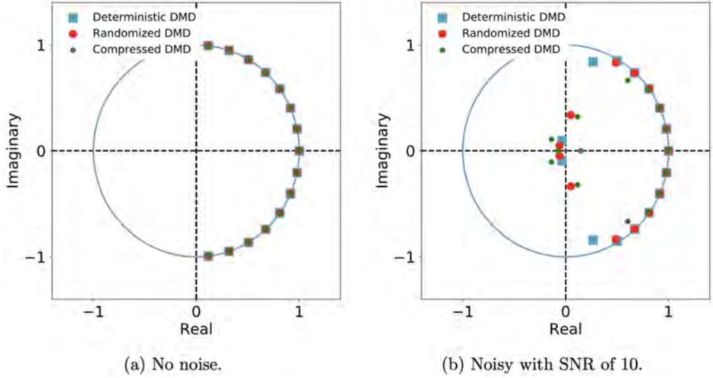
Figure 61: DMD eigenvalues for fluid flow behind a cylinder. Both the compressed and randomized DMD algorithms capture the eigenvalues in the absence of noise (a). In the presence of white noise with SNR of 10, rDMD performs better than sampling rows (b).
