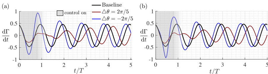
Figure 54: Vorticity flux comparison with respect to the baseline for (a) rotary control and (b) momentum injection.
