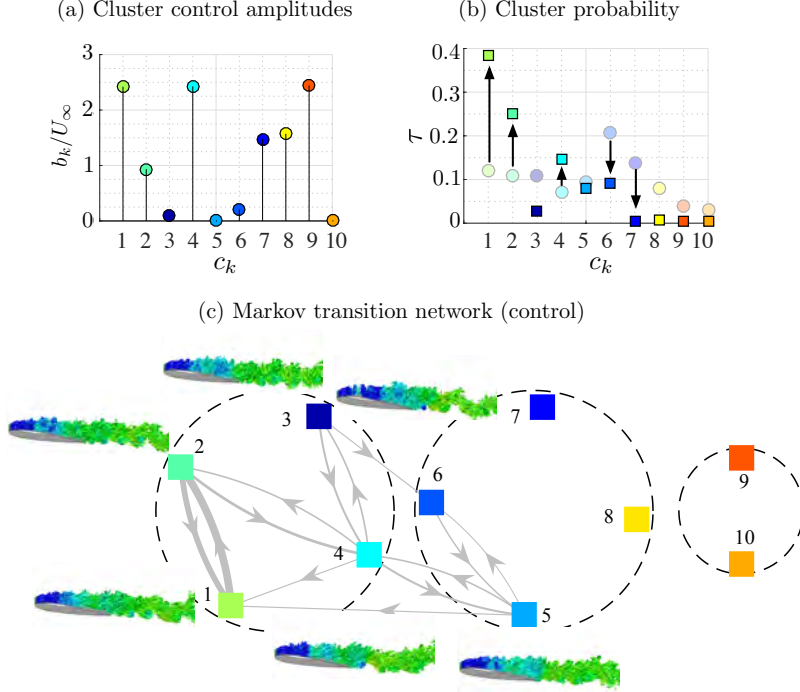
Figure 46: Comparison of optimized control case A with baseline: (a) Cluster jet velocities, (b) cluster probability for baseline (shown in transparent round symbols) and controlled flows (shown in square symbols) and (c) graph of optimally controlled Markov chain.
