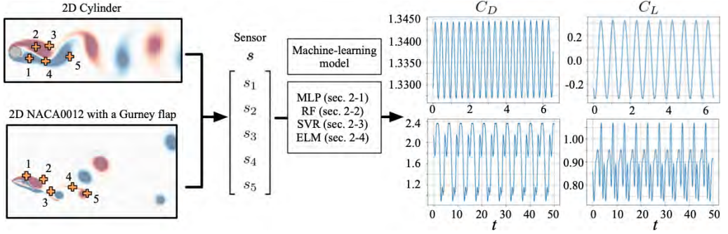
Figure 74: Estimation of C_D and C_L values with laminar flow. Models for estimating C_D and C_L are constructed individually.
