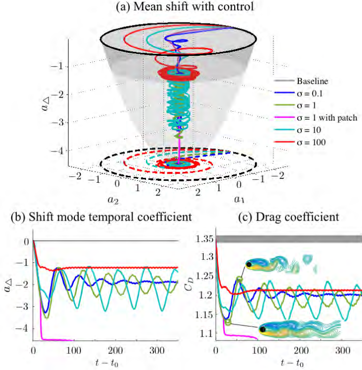
Figure 32: (a) Shift mode temporal dynamics on parabolic inertial manifold for a range of \sigma and (b) shift mode temporal dynamics in the time domain. (c) Drag force compared to the baseline.
