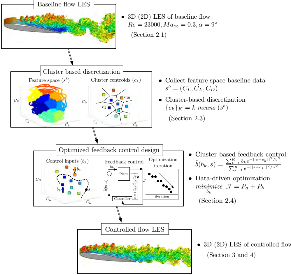
Figure 33: Overview of cluster-based control framework.
