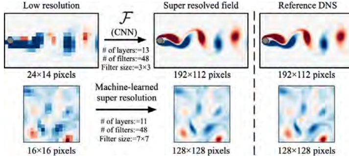
Figure 85: Super-resolution reconstruction with machine learning. The vorticity field \omega are used as input and output attributes.
