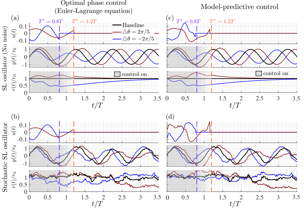
Figure 50: Optimal phase control (using Euler–Lagrange equation) of Stuart–Landau oscillator with (a) no noise ( \sigma = 0 ) and (b) stochastic dynamics \sigma = 0.05 . Model-predictive control of Stuart–Landau oscillator with (c) no noise ( \sigma = 0 ) and (d) stochastic dynamics \sigma = 0.05 . For each case, the control input u(t) , trajectory y(t) and radial amplitude r(t) are shown.
