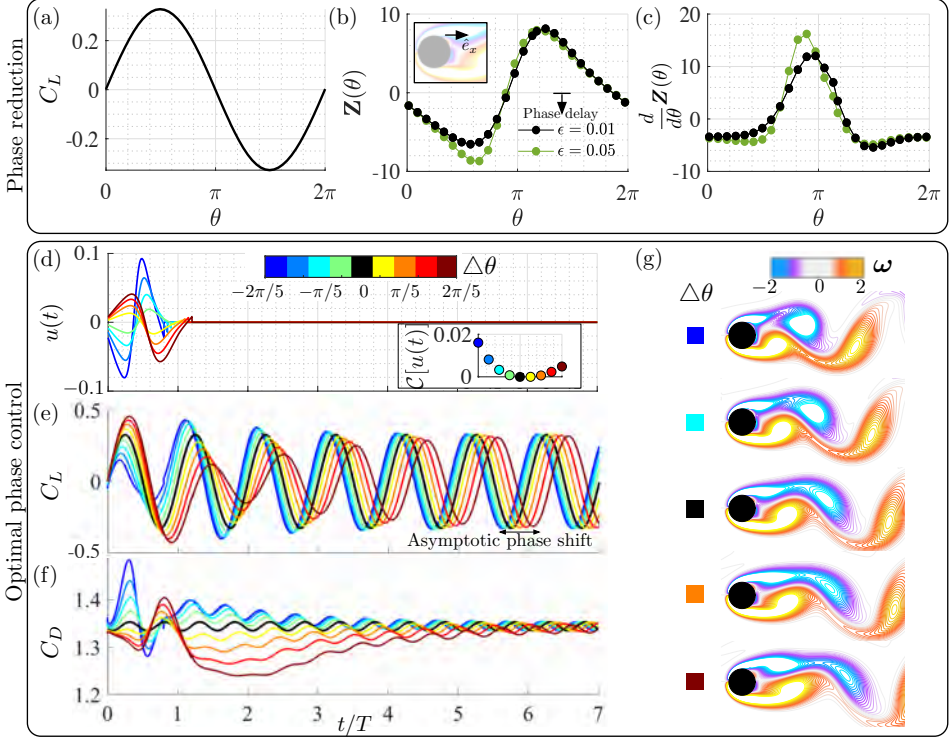
Figure 52: Overview of phase-reduction and optimal phase control for cylinder flow using momentum injection : (a) Lift coefficient ( C_L ) of baseline cylinder flow with respect to the phase coordinate \theta , (b) phase sensitivity function and (c) its gradient (right) for impulse perturbation introduced at an actuator located near the top separation point in the \hat{e}_x direction, (d) energy-optimal control input needed to shift the phase of oscillation (with associated cost function in inset), (e) lift and (f) drag characteristics after application of forcing in direct numerical simulations, and (g) instantaneous flow fields immediately after control is turned off ( t = T^* ). The color of the lines correspond to the cases with desired phase shift \Delta\theta with \Delta\theta = 0 indicates baseline.
