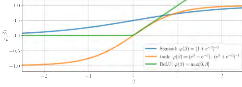
Figure 69: An example of activation functions \varphi(\beta) . In the present paper, we use ReLU \varphi(\beta) = \max[0, \beta] .
