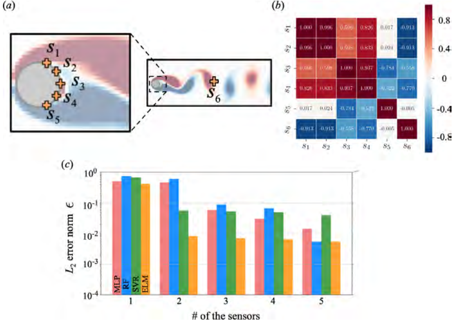
Figure 83: Influence of the number of sensors on the cylinder wake reconstruction. (a) Positions of each sensor. (b) Covariance matrix. (c) Relationship between the number of sensors and L_2 error norm.
