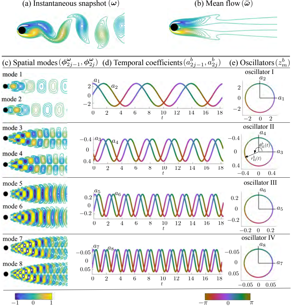
Figure 20: (a) Instantaneous snapshot of vorticity field and (b) time-averaged (mean) vorticity field. Proper orthogonal decomposition (POD) technique applied to cylinder flow problem results in (c) spatial modes and (d) temporal coefficients associated with the modes. (e) temporal coefficients of oscillators in complex plane. The colorbar of the spatial modes indicates the contour level and colorbar of the temporal coefficients and oscillators indicates phase of the oscillators varying from [-\pi, \pi] in a periodic limit-cycle manner. The colors (Thyng et al. 2016) of the lines in Figure 70 (d) and (e) helps us easily identify the correspondence of the temporal coefficients in the time domain and phase space. Polar coordinates associated with the oscillator II is shown.
