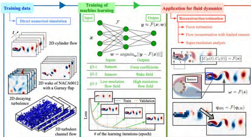
Figure 67: Overview of supervised machine learning problems for fluid flows discussed in this paper. We focus on reconstruction and estimation tasks for direct numerical simulation data.
