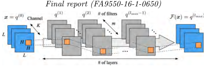
Figure 72: Two-dimensional convolutional neural network.
