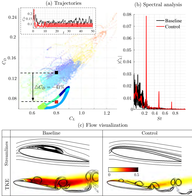
Figure 39: Comparison of baseline and optimized control case: (a) Trajectories, (b) spectral analysis of lift data, and (c) time-averaged streamlines and turbulent kinetic energy (TKE) fluctuations. Baseline trajectories are shown in transparent in (a). The contour lines in (c) (bottom) indicate instantaneous vorticity fields.
