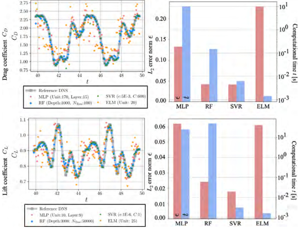
Figure 76: Summary of C_D and C_L estimations for wakes of NACA0012 airfoil with a Gurney flap at Re_c = 1000 . The top left shows C_D estimations and bottom left presents C_L estimations. The optimized parameters are provided in the graph legends. The color bars located on the right show the relationship between L_2 error norm \epsilon of each coefficient (red) and computational time (blue) for each machine learning model.
