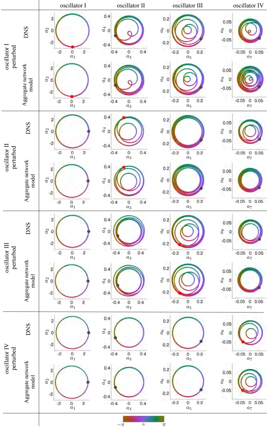
Figure 27: Oscillator dynamics of DNS and aggregate networked oscillator model for phase perturbations to oscillators corresponding to \theta'_n(t_0) = -\pi/2 .
