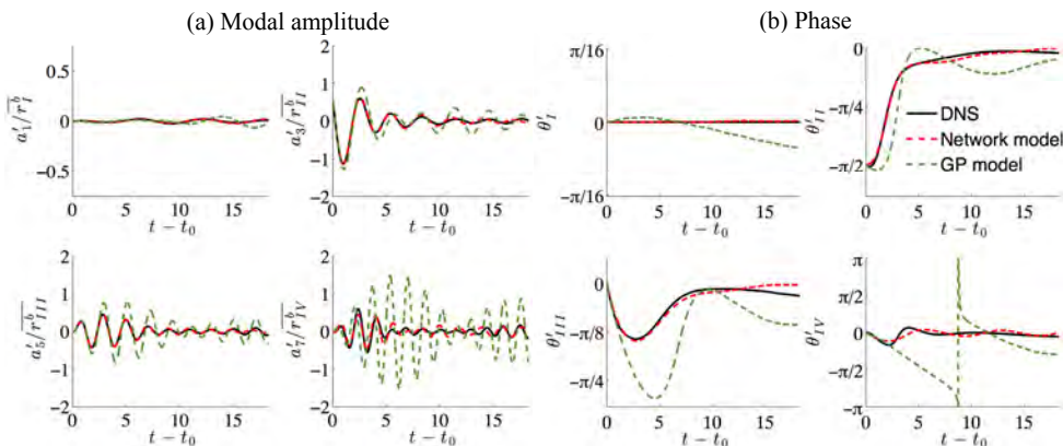
Figure 24: (a) Modal amplitude and (b) phase tracking for amplitude perturbation introduced at oscillator II.
