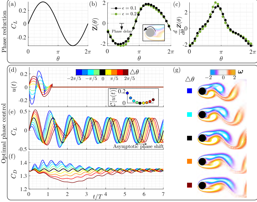
Figure 51: Overview of phase-reduction and optimal phase control for cylinder flow using rotary actuation : (a) Lift coefficient ( C_L ) of baseline cylinder flow with respect to the phase coordinate \theta , (b) phase sensitivity function and (c) its gradient (right) for impulse perturbation introduced at an actuator located near the top separation point in the \hat{e}_x direction, (d) energy-optimal control input needed to shift the phase of oscillation (with associated cost function in inset), (e) lift and (f) drag characteristics after application of forcing in direct numerical simulations, and (g) instantaneous flow fields immediately after control is turned off ( t = T^* ). The color of the lines correspond to the cases with desired phase shift \Delta\theta with \Delta\theta = 0 indicates baseline.
