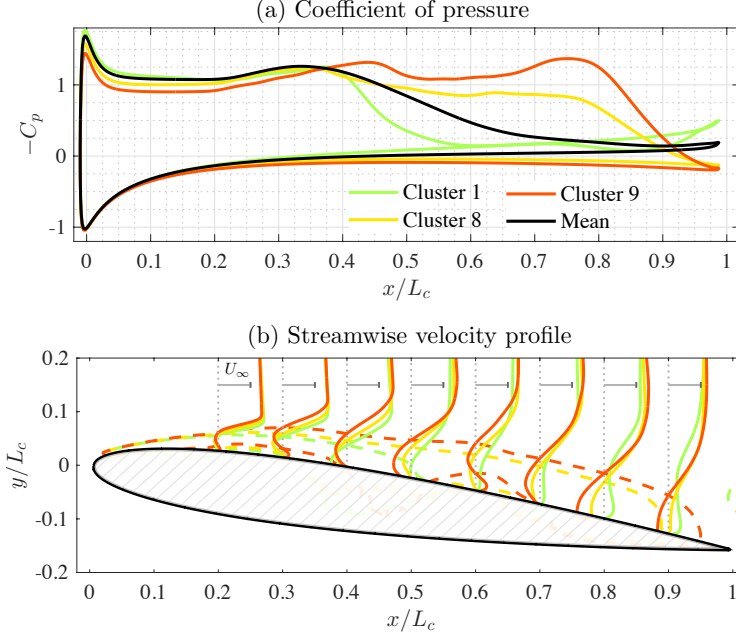
Figure 37: (a) Cluster-averaged pressure distribution over the suction and pressure surface of airfoil and (b) cluster-averaged streamwise velocity profiles for 2D baseline flow.
