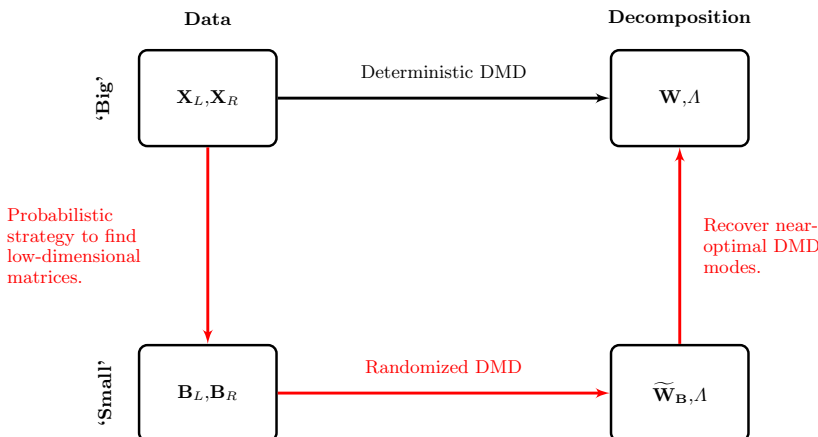
Figure 58: Conceptual architecture of the randomized dynamic mode decomposition (rDMD). First, small matrices are derived from the high-dimensional input data. The low-dimensional snapshot matrices \mathbf{B}_L and \mathbf{B}_R are then used to compute the approximate dynamic modes \tilde{\mathbf{W}}_B , and eigenvalues \Lambda . Finally, the near-optimal modes \mathbf{W} may be recovered.
