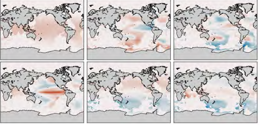
Figure 64: Leading dynamic modes of the full high-resolution SST dataset.
