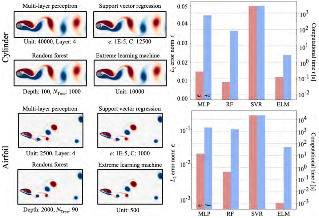
Figure 80: Summary of wake reconstruction for cylinder and NACA0012 with Gurney flap wakes. The left side shows the compilation of vorticity fields reconstructed by the four machine learning models. Optimal parameters are listed below the vorticity fields. The color bars located on the right side show the relationship between L_2 error norm \epsilon (red) and computational time (blue) for the selected machine learning models.
