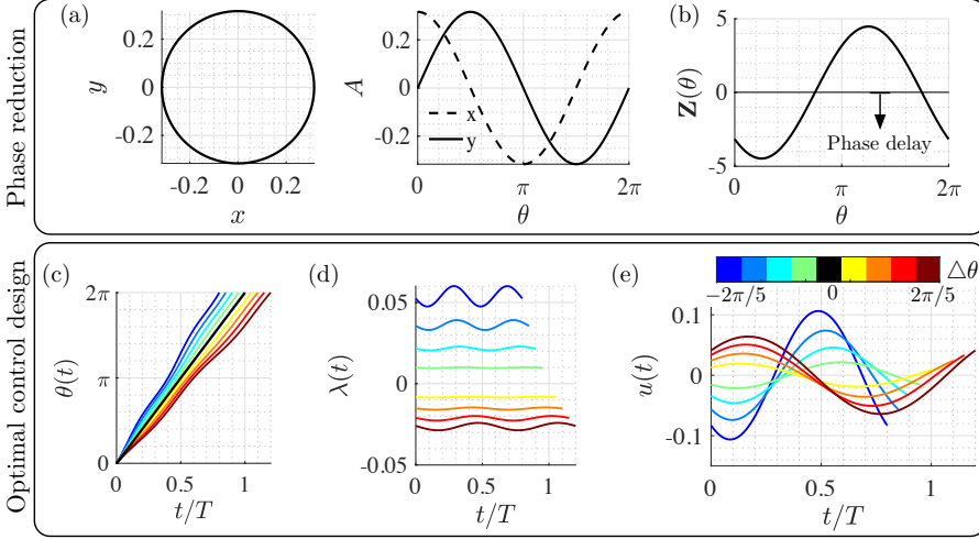
Figure 49: Overview of phase-reduction and optimal phase control for a Stuart-Landau oscillator: (a) Baseline trajectories; (b) analytical phase-sensitivity function and optimal control design for desired phase shifts of -2\pi/5 \leq \Delta\theta \leq 2\pi/5 ; (c) phase coordinate dynamics; (d) dynamics of the Lagrange multiplier; and (e) the optimal control input from the Euler-Lagrange equations.
