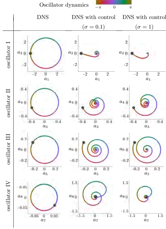
Figure 31: Oscillator dynamics without control and with control implemented in DNS for suppressing modal oscillations.
