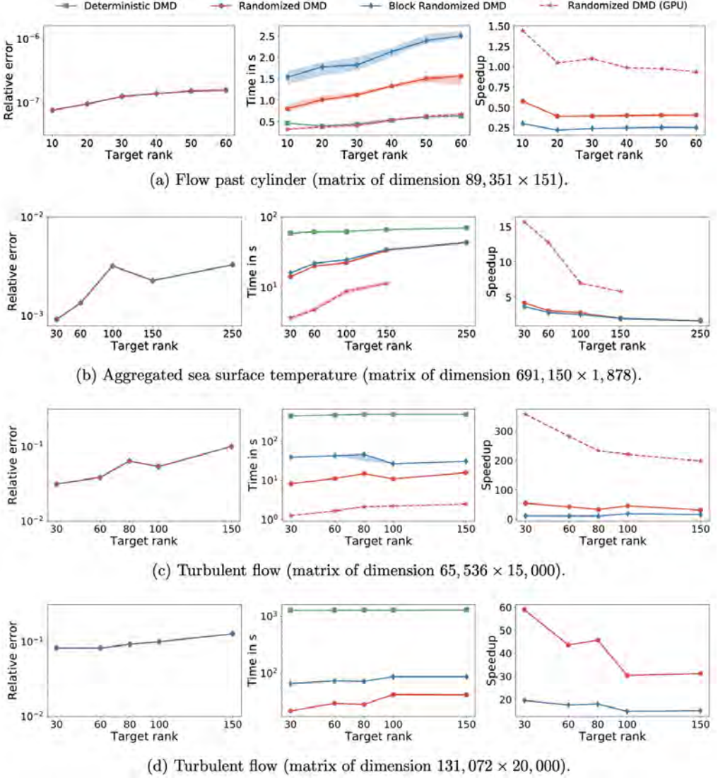
Figure 65: Average runtimes and errors, over 20 runs, for varying target ranks. Further, the gained speedup compared to the deterministic algorithm (baseline) is shown.
