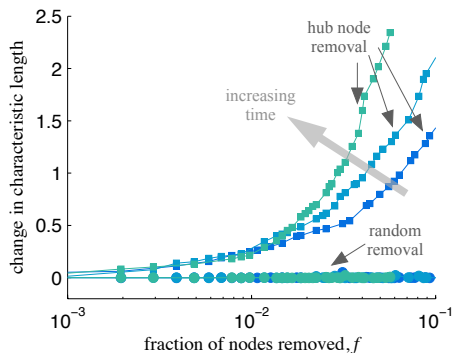
Figure 18: The resilience of turbulence network against node removals for t = 15, 30 , and 75 with Re(t_0) = 814 . Shown are relative changes in the characteristic network length \Delta \tilde{l}_{\text{network}} of turbulent flow for random node and hub node removals. The colors of the curves represent the time when node removal is considered and follows Figure 16.
