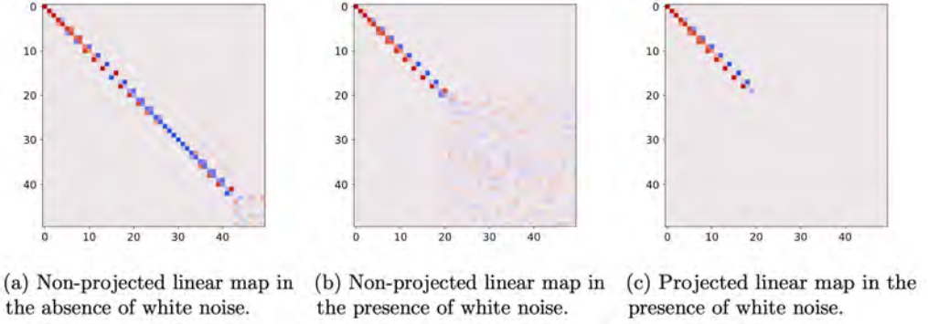
Figure 60: Illustration of the non-projected and projected map for toy data in the absence and presence of white noise. The regularization effect of the projected map reduces the influence of noise, while preserving the dominant information.
