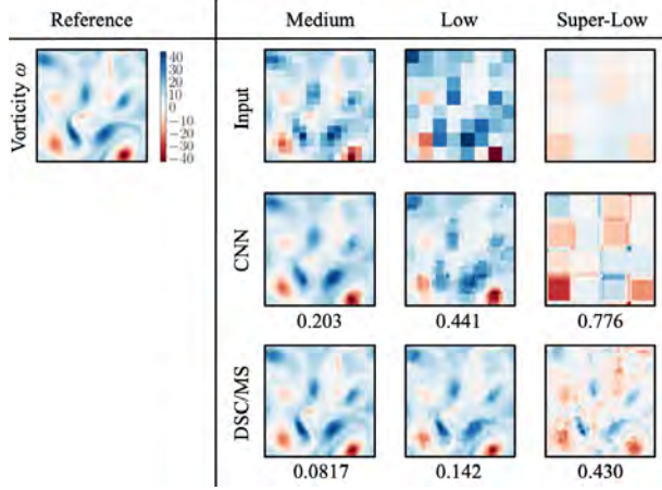
Figure 87: Super-resolution reconstruction with machine learning of two-dimensional turbulence. Reprinted with permission from Cambridge University Press.
