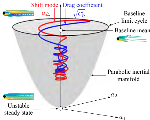
Figure 28: Shift mode temporal coefficient (red) and drag coefficient (blue) variation (indicated by arrows) with application of control. Parabolic inertial manifold shown in grey.
