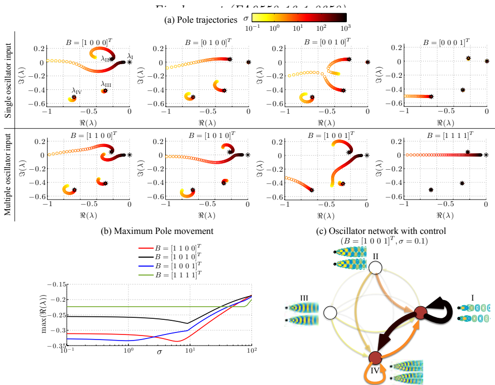
Figure 29: (a) Pole trajectories with application of different control inputs to the aggregate network model for a range of \sigma . Stars indicate \lambda(-L_G) . (b) Movement of \max(\Re(\lambda)) for the multiple oscillator input cases. (c) Network structure with control. The oscillators to which control is added is indicated by red (filled) circles. The color and thickness of the network edges in the network represent the magnitude of elements of (-L_G - BK) .
