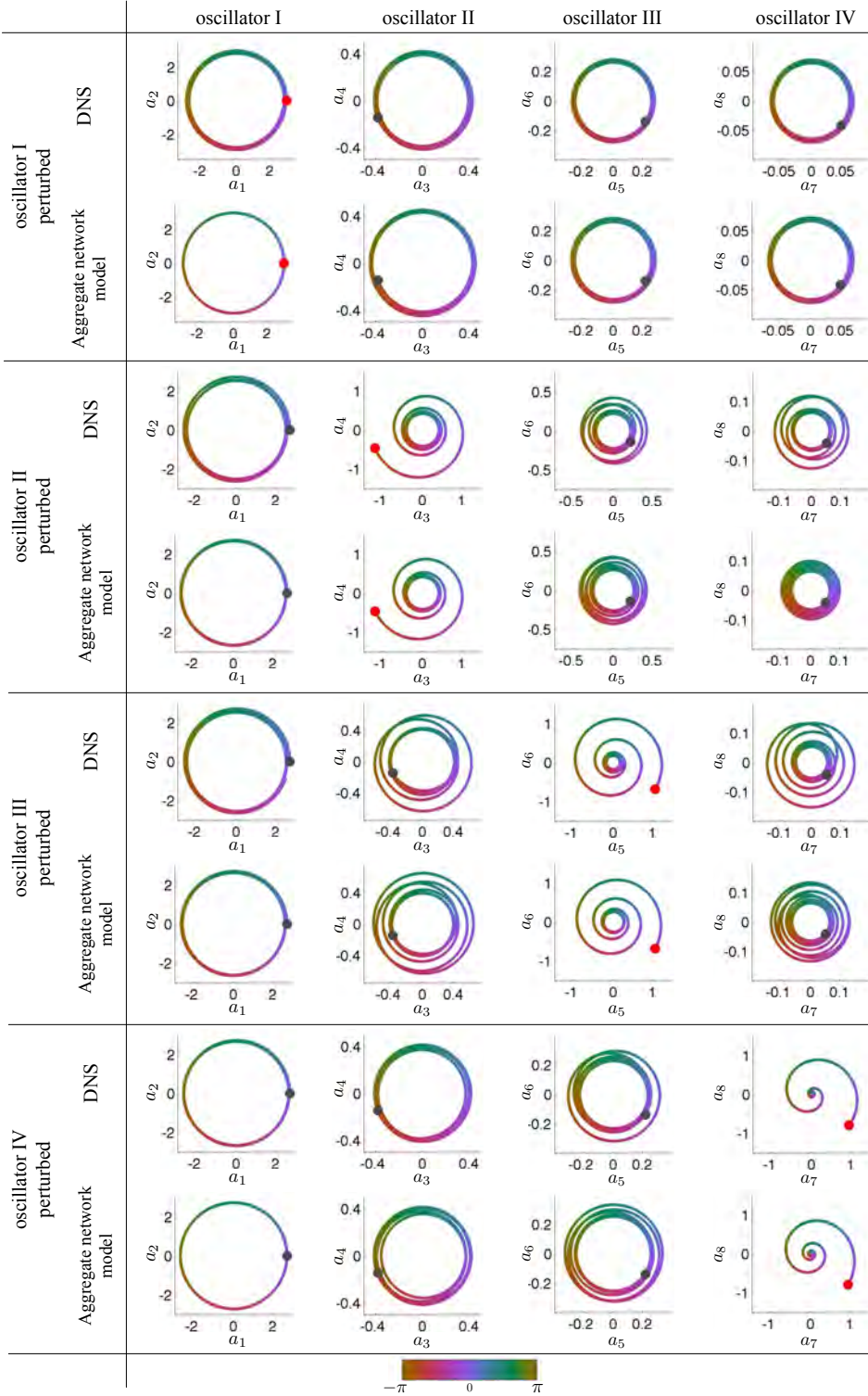
Figure 26: Oscillator dynamics of DNS and aggregate networked oscillator model for amplitude perturbations to oscillators corresponding to energy input of \beta_m = 0.2 .
