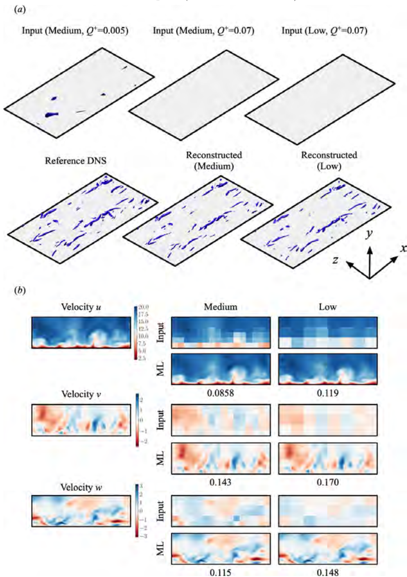
Figure 88: (a) The Q -criterion ( Q^+ = 0.07 ) contour plots of (a) input coarse data, (b) reference DNS data, and machine-learned super-resolved data from (c) medium- and (d) low-resolution inputs. (b) The y - z section contours of velocity u , v , and w are for x^+ = 1127 .
