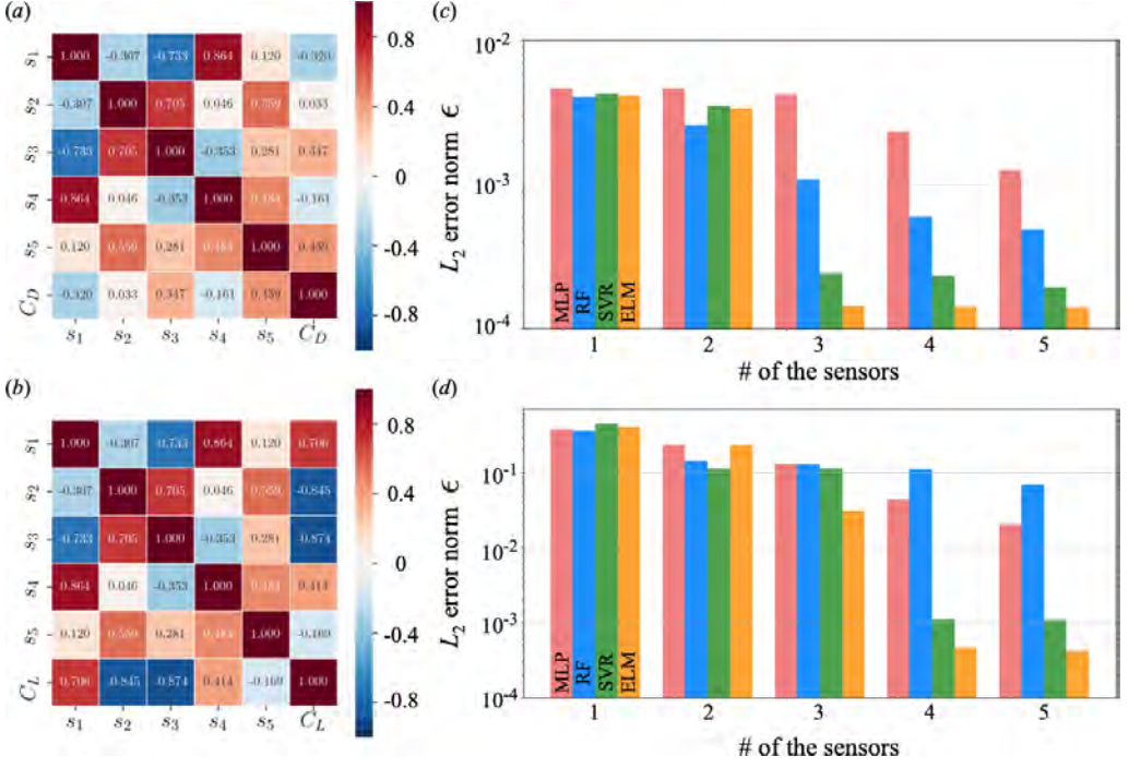
Figure 78: The influence of the number of sensors n_{\text{sensor}} on the accuracy of the force estimations. Correlation matrix of (a) C_D and (b) C_L estimations. The relationship between n_{\text{sensor}} and L_2 error norm of (c) C_D and (d) C_L estimations.
