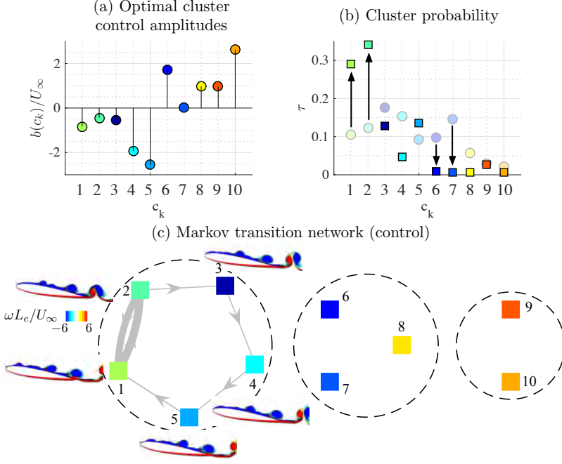
Figure 40: (a) Cluster jet velocity, (b) cluster residence probability for baseline (shown in transparent round symbols) and controlled flows (shown in bright square symbols) and (c) controlled Markov transition network with instantaneous vorticity contours ( \omega L_c/U_\infty ).
