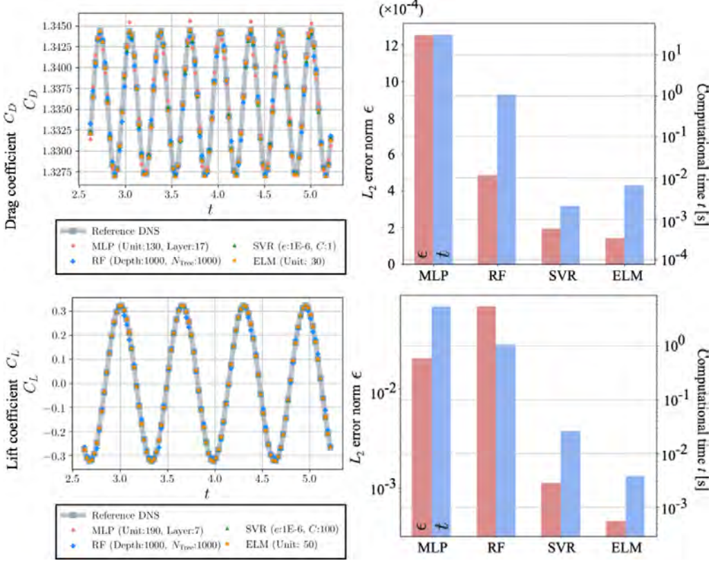
Figure 75: Summary of C_D and C_L estimations for laminar cylinder wake at Re_D = 100 . In the top and bottom, C_D and C_L estimations, respectively, are presented. The left side shows temporal variations of force coefficients. The optimized parameters are provided in the graph legends. The color bars on the right show the relationship between L_2 error norm \epsilon of each coefficient (red) and computational time (blue) for each machine learning model.
