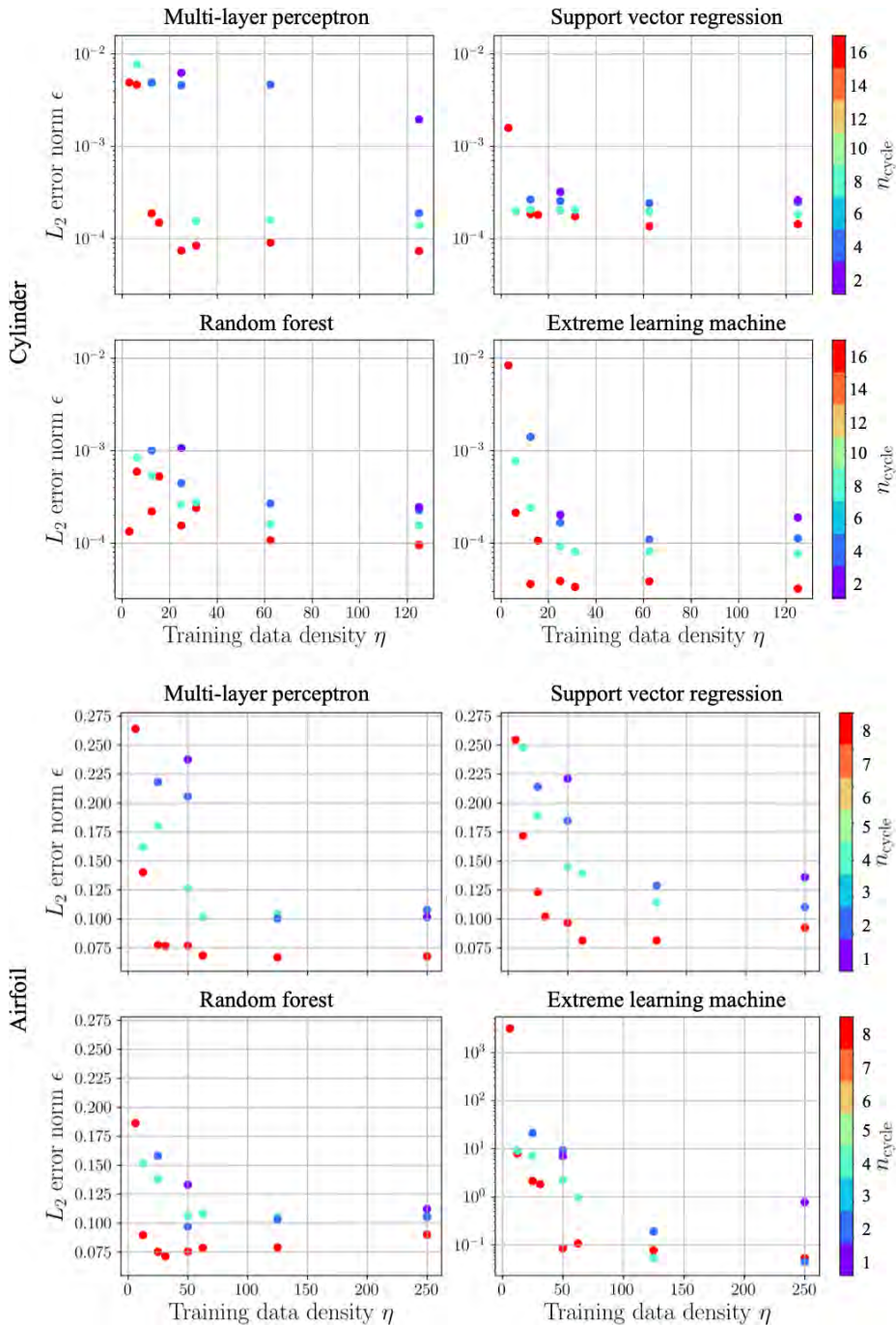
Figure 77: The relationship between the training data density \eta and L_2 error norm \epsilon of C_D prediction for four machine learning models. Note that the range of y -axis with extreme learning machine for the airfoil problem is different from the others.
