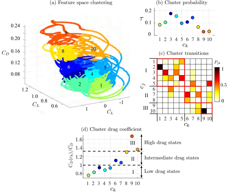
Figure 35: (a) Feature space clustering of the 2D baseline flow. (b) Cluster residence probabilities and (c) cluster transition probabilities. The red boxes indicate cluster subsets. (d) Normalized drag corresponding to cluster centroids.
