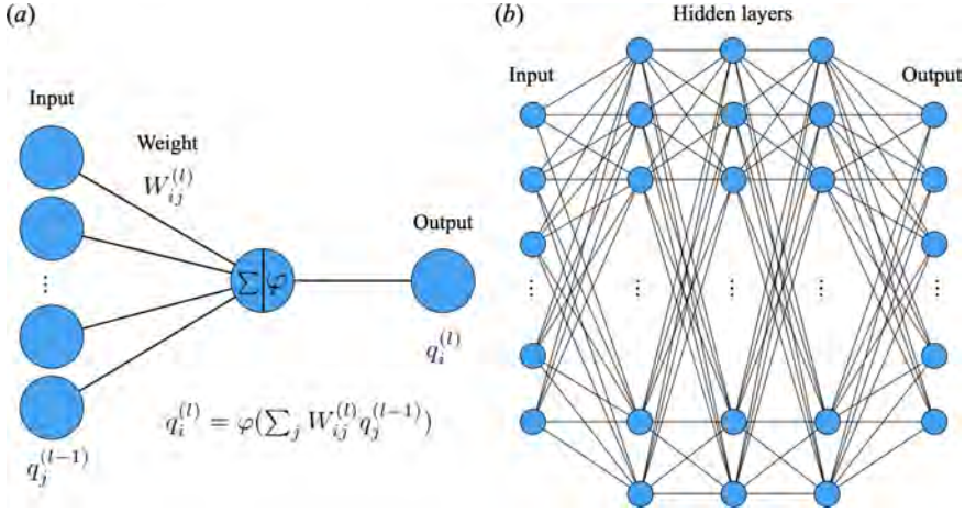
Figure 68: (a) A perceptron. (b) Multi-layer perceptron is an aggregate of perceptrons.
