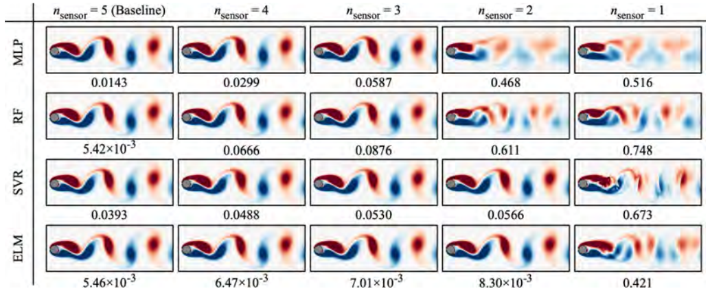
Figure 84: The reconstructed vorticity fields of cylinder wake with n_{\text{sensor}} = 1, 2, 3, 4 , and 5.
