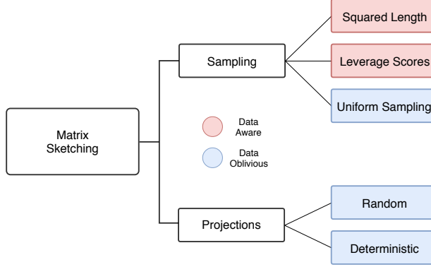
Figure 59: Sketching techniques for high-dimensional data; this work uses random projections.
