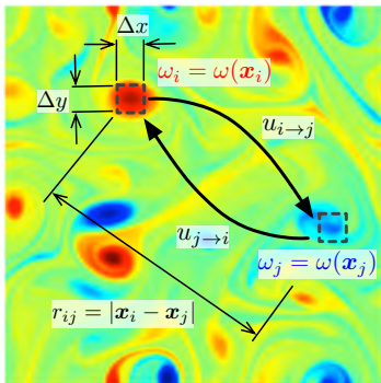
Figure 14: Interaction of fluid elements in two-dimensional turbulence. The strength of the vortical interaction between elements i and j having vorticity \omega_i and \omega_j is quantified through the induced velocities u_{i \rightarrow j} and u_{j \rightarrow i} , respectively. For discretizing the Cartesian domain, we take n_x and n_y points in the horizontal and vertical directions, respectively, providing the adjacency matrix \mathbf{A} of size n \times n with n = n_x n_y . Shown in the background with a contour plot is the corresponding vorticity field with initial Re(t_0) = 814 at t = 18 .
