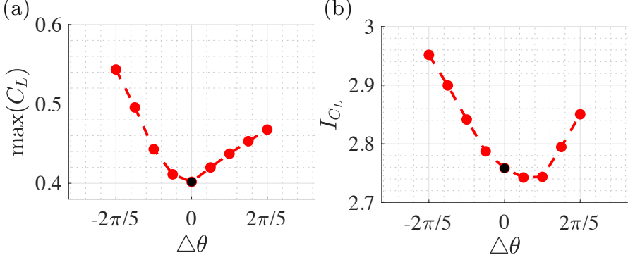
Figure 56: Evaluation of control performance: (a) Maximum lift coefficient and (b) lift impulse for varying phase shifts.
