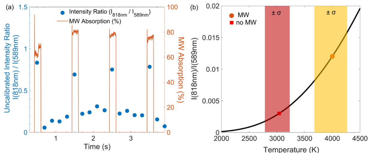
Figure 12. (a) Time history of line intensity ratio shown with the microwave absorption during a propellant burn with a 20% duty cycle modulated microwave field. (b) Average inferred sodium electronic temperature of aluminized, doped composite propellant (Al/AP/NaNO 3 -3.5%) with and without microwave enhancement. Banded temperature regions indicate temperature ranges corresponding to \pm one standard deviation of measured sodium band emission intensity ratios for three propellant strand combustion experiment.
