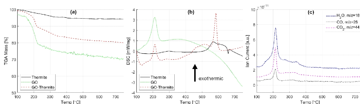
Figure 29. TGA (a) and DSC (b) of n-Al/n-Fe 2 O 3 thermite, GO, and GO-wrapped thermite (30 wt.% GO) with mass spectrometry of significant evolved products for GO-wrapped thermite (c).
