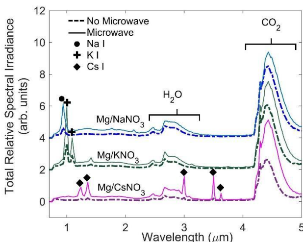
Figure 22. Time-integrated, infrared total spectral irradiance of each Mg/alkali nitrate/epoxy energetic material with and without microwave illumination. Species of significant electronic atomic and molecular emission enhancements observed are noted. Irradiance values for each formulation are offset for presentation purposes.
