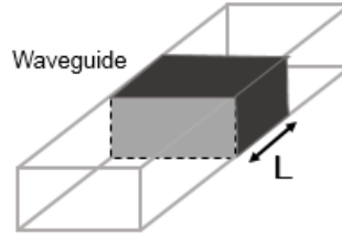
Figure 7. Schematic of propellant test article in waveguide transmission measurement. Propellant test articles are 2.912 cm long ( \sim\lambda/4 at \sim 2.7 GHz).
