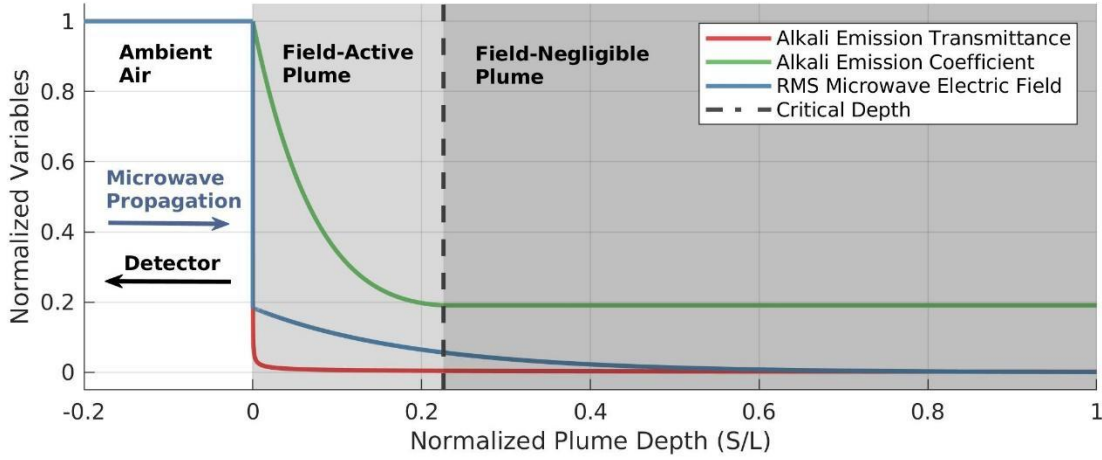
Figure 2. Example configuration of the homogenous plume model with an incident electric field propagating left to right, perpendicular to the plume surface. Radiance is computed at surface, s = 0 , simulating light available for detection.
