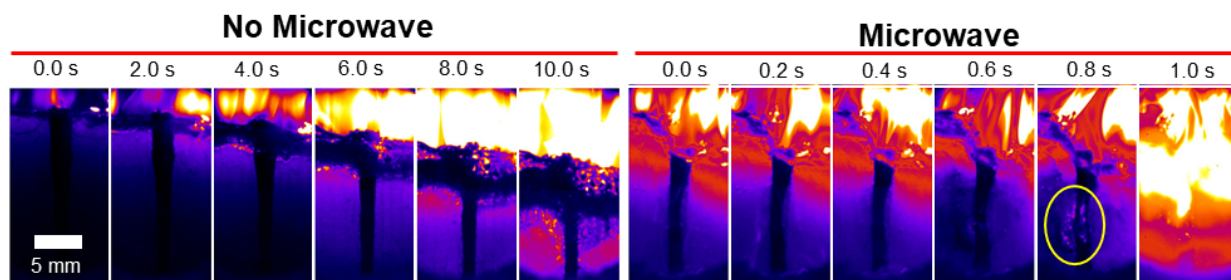
Figure 34. Light emission still image sequence of UV-Cured Propellant Manufacture with Functionalize Energetic Wires strands burning without (left) and with microwave field application (right). False coloring is used to indicate emission intensity. The yellow circle indicates a burning surface pocket formed near the energetic wire. Camera exposure and aperture settings are the same for each formulation with and without microwave.
