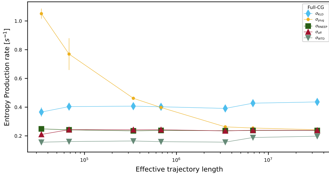
Fig. S1. Convergence of EPR estimators, \sigma_{\text{KLD}} (blue diamonds), \sigma_{\text{plug}} (light orange dots), \sigma_{\text{RNEEP}} (dark green squares), \sigma_{\text{aff}} (red triangles) and \sigma_{\text{WTD}} (gray triangles), as a function of effective trajectory length, calculated for the 4-states system and x = -0.15 . The effective trajectory length is calculated after full-CG .
