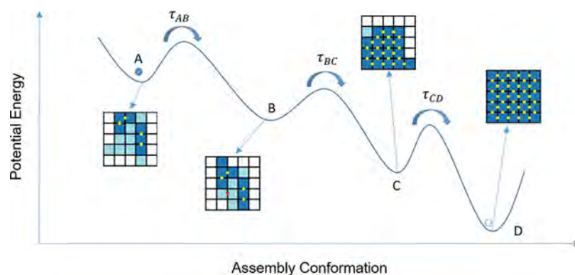
Figure 4. Self-assembly and Kramer's escape rate illustration. The self-assembly process has a rugged energy landscape, and the system needs to cross multiple barriers between local minima (A–C) on the path to the target structure (D). Each barrier is associated with a typical escape rate, so the time to the first assembly can be approximated by the sum of the dwell times in the local minima, T_{\text{FAS}} \approx \tau_{\text{AB}} + \tau_{\text{BC}} + \tau_{\text{CD}} , in this case.
