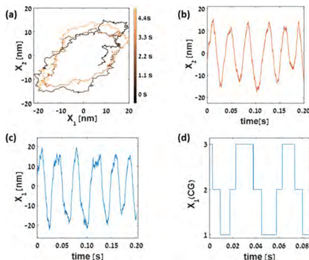
Fig. 1 Simulated trajectories of the observed ( X_1 , the tip position of the hair bundle) and the hidden ( X_2 , the position of the molecular motors) variables and the coarse-grained trajectory of the observed variable after spatial coarse-graining (a) the trajectories in the X_1 - X_2 plane for fixed values of driving parameters: ( F_{max} = 70 pN, S = 1 , T_{eff}/T = 1.5 ). The color of the curve represents time going from dark to bright (b) X_2 = X_2 - \langle X_2 \rangle , as a function of time for fixed values of driving ( F_{max} = 70 pN, S = 1 , T_{eff}/T = 1.5 ). (c) X_1 = X_1 - \langle X_1 \rangle , as a function of time for the same values of driving parameters, which does not show any sign of net flux, (d) the coarse-grained trajectory for 3 CG states at above mentioned parameter values. All the quantities plotted are calculated for the following additional parameter values: \lambda_1 = 2.8 pN ms nm -1 , \lambda_2 = 10 pN ms nm -1 , k_{gs} = 0.75 pN nm -1 , k_{sp} = 0.6 pN nm -1 , D = 61 nm, k_B T = 4 pN nm, \Delta G = 10 k_B T .
