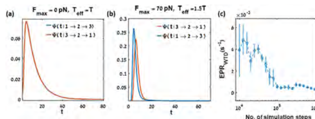
Fig. 3 Entropy production rate estimation from the Kullback–Leibler divergence between the waiting time distributions for 3 equally spaced coarse-grained states of the active hair bundle’s tip position: probability density functions of the time ( t [s]) that the system stays at state 2 for an upward transition (blue solid line), and for a downward transition (red solid line) for two different parameter values: (a) F_{\text{max}} = 0 pN, T_{\text{eff}} = T , and S = 1.5 , (b) F_{\text{max}} = 70 pN, T_{\text{eff}} = 1.5 T , and S = 1.5 , (c) \text{EPR}_{\text{WTD}} as a function of length of the simulation for F_{\text{max}} = 70 pN, T_{\text{eff}}/T = 1.5 , and S = 1.5 . The error bar at each point describes the standard error of the mean.
