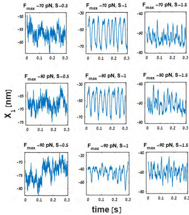
Figure S1. The trajectories of the position of the tip of the hair bundle ( X_1 ) as calculated by solving the coupled differential equations, Eq. 1 and Eq. 2 in the main text for different values of the parameter choices as a function of time. The driving parameter values are written in the subtitles with T_{eff} = 1.5 T . All other parameter values are the same as mentioned in Figure 1 in the main text.
