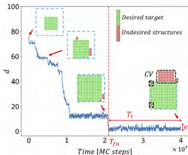
FIG. 3. Distance from the desired target structure as a function of time, measured in Monte Carlo steps. Highlighted on the plot, T_{fa} is the time until first assembly, T_t is the time spent in the desired target structure, and e is the fluctuation deviation. The images show the state of the lattice at certain timepoints. Structures that belong to the desired target structure are marked in green, and other, undesired, structures are marked in red. The boundaries of the target structure are marked in blue (for more elaboration on the coloring scheme, see the supplementary material , Sec. S2). The chimeric structures, whose size is the chimeric value, are also highlighted. This example dataset was taken from a simulation of 10^5 lattice sweeps, with parameters \{m = 6, M = 100, N_0 = 400, E = 9, \mu/E = 1.78, S = 5, \text{ and } \Delta\lambda = 1.5\} .
