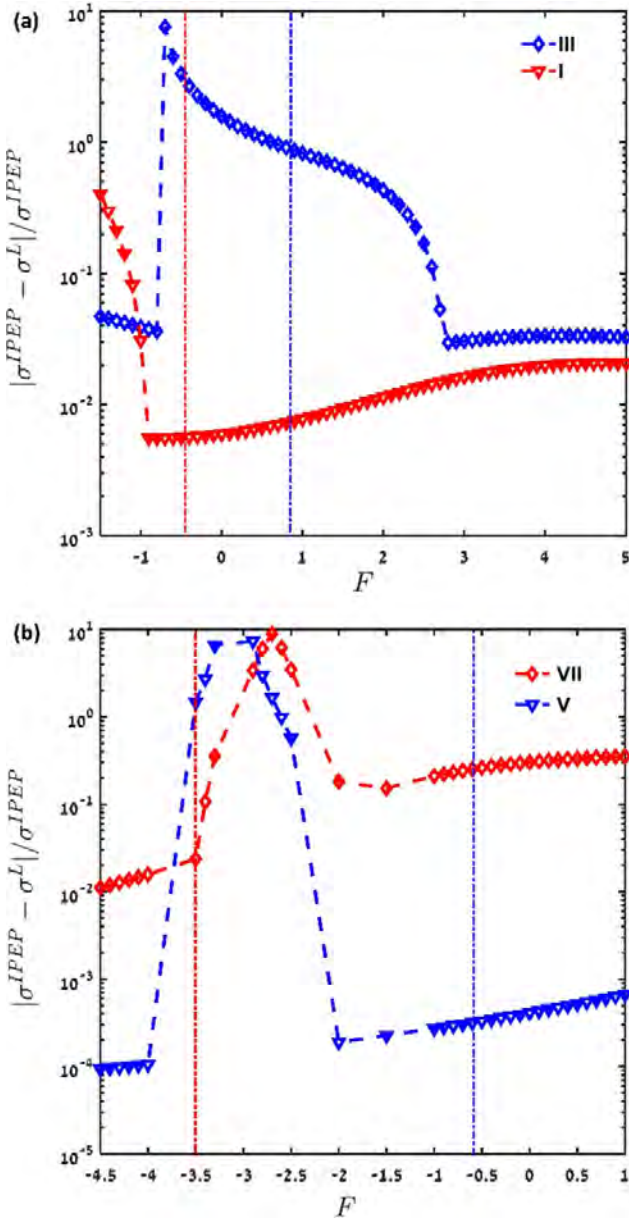
Figure 3. Comparison of \sigma^{\text{IPEP}} and \sigma^L as a function of the dimensionless driving force ( F ) for different network topologies: weight of the connectivity of the hidden substates and in between state 1 and state 3 are given by \nu and \mu , respectively. The parameters used have the same values as mentioned in figure 1. (a) Red downward triangles and blue diamonds refer to network topology I and III, respectively. (b) Blue downward triangles and red diamonds refer to network topologies V and VII, respectively. The lines are drawn to guide the eye. The stalling forces are labeled by dash-dotted lines for each topology.
