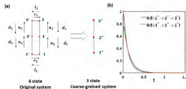
Fig. 2 The X_1 - X_2 trajectory of the hair bundle system coarse-grained into a linear topology in X_1 state space after decimation of the X_2 states with zero net flux motivates to use KLD estimator of the waiting times ( t [s]): (a) The circles with the lines represents a 6 state system, which after decimation is reduced to a linear 3 state system, (b) non-zero contribution from the Kullback–Leibler divergence of the waiting time distributions: the distribution of the waiting times ( t [s]) the system waits at CG state 2'' for an ( 1'' \rightarrow 2'' \rightarrow 3'' ) upward transition (blue solid line) and ( 3'' \rightarrow 2'' \rightarrow 1'' ) the downward transition (red solid line) for the following parameter values: u_1 = 10 , u_2 = 3 , d_1 = 2 , d_2 = 4 , r_1 = 3 , r_2 = 3 , l_1 = 1 , l_2 = 1 .
