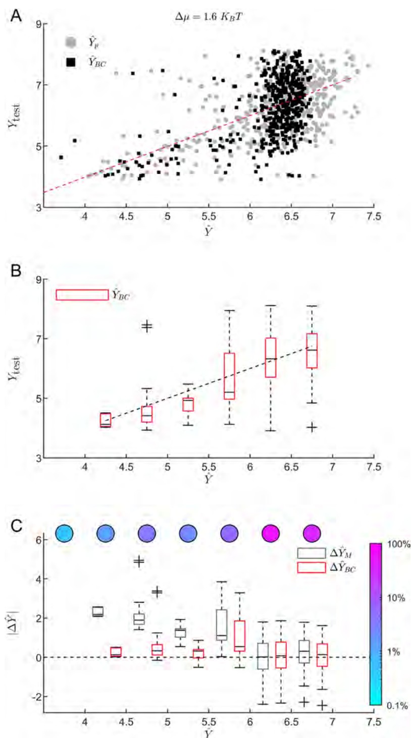
Figure 7. Results of the SLM prediction for the remaining time to the first assembly for the test set, for \Delta\mu = 1.6 k_B T . (A) Y_{\text{test}} results are shown vs their predicted values \hat{Y} , before the bias correction ( \hat{Y}_p , gray circles) and after the bias correction ( \hat{Y}_{BC} , black squares). The red line shows the linear regression of the data. (B) Box plot of the Y_{\text{test}} vs the calculated \hat{Y}_{BC} , where the data are binned according to the \hat{Y}_{BC} values (see main text). The box plot whiskers represent the standard interquartile range (IQR), and outliers are defined to be above 1.5 IQR (plus markers). The dashed unit slope, linear line ( y = x ) represents the results of a perfect predictor. (C) Absolute values of \Delta\hat{Y}_M (black) and \Delta\hat{Y}_{BC} (red) vs the respective predictor value \hat{Y} for each bin. The dashed black line at \Delta\hat{Y} = 0 represents a perfect predictor with zero error. The color bar indicates the relative weight of the data for each bin, calculated from the relative number of data points. Bins with weights less than 1% are omitted.
