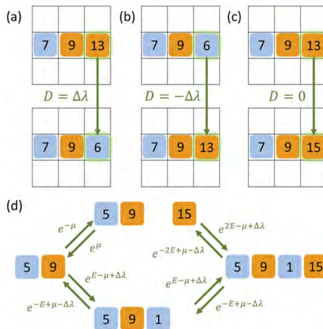
FIG. 2. Local driving force. (a)–(c) Examples of situations yielding different D values. The initial state is presented on top, and the proposed step at the bottom. (a) The initial state does not include an intermittent subunit triplet, and the proposed step does; thus, D = \Delta\lambda . (b) The initial state includes an intermittent subunit triplet, and the proposed step does not; thus, D = -\Delta\lambda . (c) Neither the initial state nor the proposed one includes an intermittent subunit triplet; thus, D = 0 . (d) Example of a cycle breaking detailed balance. The acceptance probabilities of the moves appear near the corresponding arrows. The probability of moving from the leftmost state to the rightmost state depends on the path taken: the probability for the upper path is p_u = \exp\{2E - 2\mu + \Delta\lambda\} , while for the lower path p_l = \exp\{2E - 2\mu + 2\Delta\lambda\} , meaning \ln(p_u/p_l) \neq 0 , i.e., broken detailed balance. Here, we assumed that the target structure from Fig. 1(b) is the only one encoded.
