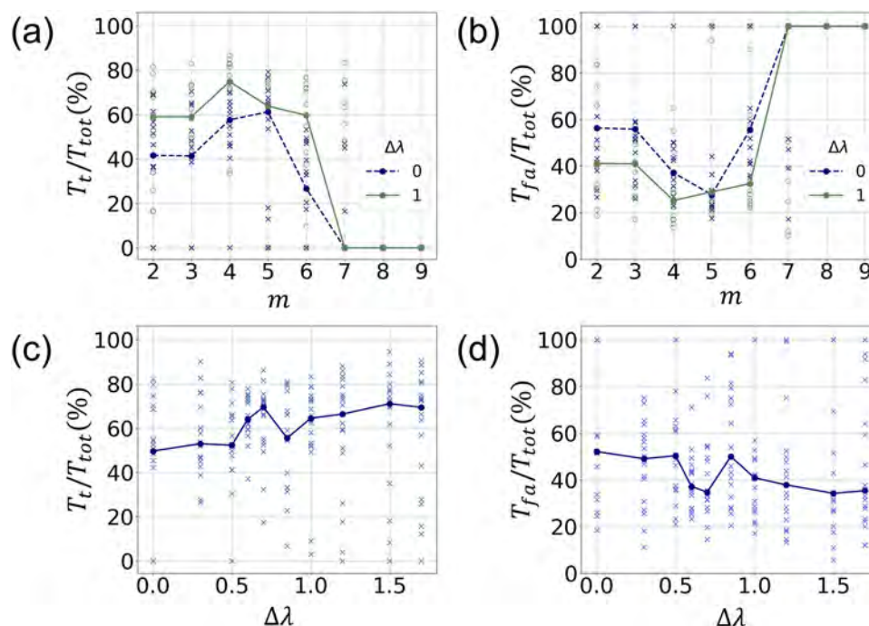
FIG. 5. Time spent in the target and first assembly time, normalized by the total number of MC steps. (a) Time spent in the target as a function of the number of target structures. (b) First assembly time as a function of the number of target structures. (c) Time spent in the target as a function of driving force for m = 3 . (d) First assembly time as a function of driving force for m = 3 . Each marker, "X" or "o" symbol, represents a result from one realization, and each point represents the median of 14 simulations for (a) and (b) or 18 simulations for (c) and (d).
