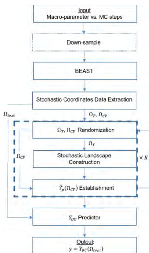
Figure 6. Flowchart of the SLM prediction process. The different steps are described in the text. The dotted rectangle is an optional step, and the dashed frame represents the repeated steps for cross-validation bias correction.
