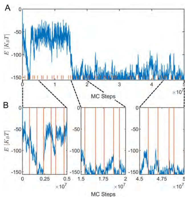
Figure 5. BEAST Segmentation. (A) Energy E of the system as a function of the MC steps for a realization of the system under nonequilibrium drive. The parameters are listed in Table 1 , with \Delta\mu = 1 . The minimum value of the energy corresponds to a successful target assembly. The vertical orange lines indicate the change points in the statistics detected by the BEAST algorithm with a minimal segment–duration constraint of one percent of the total simulation time. Each segment between two change points is considered a “macrostate.” (B) Zoom-in on three different windows of the trajectory. Vertical orange lines mark the corresponding change points.
