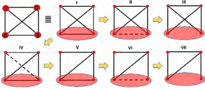
Figure 1. Different network topologies in which states 1 and 2 are observed, and states 3 and 4 are indistinguishable, and collectively called ‘hidden state’ (shaded with red color). The weights of the 3–4 link and 1–3 link are denoted by \nu and \mu , respectively. The networks are denoted by these two parameters (I) \mu = 1, \nu = 1 ; (II) \mu = 1, \nu = 0.2 ; (III) \mu = 1, \nu = 0 ; (IV) \mu = 0.05, \nu = 1 ; (V) \mu = 0, \nu = 1 ; (VI) \mu = 0, \nu = 0.05 ; (VII) \mu = 0, \nu = 0 . The other transition rates are: \bar{w}_{12} = 2 \text{ s}^{-1} , \bar{w}_{21} = 3 \text{ s}^{-1} , w_{14} = 1 \text{ s}^{-1} , w_{41} = 8 \text{ s}^{-1} , w_{24} = 35 \text{ s}^{-1} , w_{42} = 0.2 \text{ s}^{-1} , w_{23} = 2 \text{ s}^{-1} , w_{32} = 50 \text{ s}^{-1} , w_{13} = 13 \mu \text{ s}^{-1} , w_{31} = 20 \mu \text{ s}^{-1} , w_{34} = 0.7 \nu \text{ s}^{-1} , w_{43} = 75 \nu \text{ s}^{-1} .
