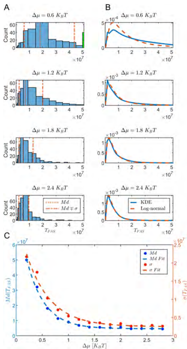
Figure 3. Simulation result statistics. (A) Simulation realizations histograms of the time to the first assembly for nonequilibrium drives, \Delta\mu = 0.6, 1.2, 1.8 , and 2.4 K_B T . The dotted vertical lines are the median values, Md , of the histogram, and the dashed lines are the 16th and 84th percentiles of the data, respectively, corresponding to the standard deviation, \sigma . The green bins stand for the realizations in which no assembly occurred. (B) Fit for the simulations realization histograms with a kernel density estimator (KDE, blue) and a log-normal distribution (dashed orange). (C) Median Md (blue), and the standard deviation \sigma (red) of the time to the first assembly histograms as a function of the drive value, \Delta\mu , with an exponential fit, Ae^{-b\Delta\mu} + C (dashed curves).
