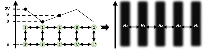
FIG. 2. Discrete flashing ratchet of 3 states with periodic boundaries, and a potential that can be switched on ( i ) and off ( i' ) but is not accessible to the observer. State of the same position i , regardless of the potential, are coarse-grained into a single macrostate H_1, H_2, H_3 . In the semi-CG framework, intra-transitions i \leftrightarrow i' are recorded.
