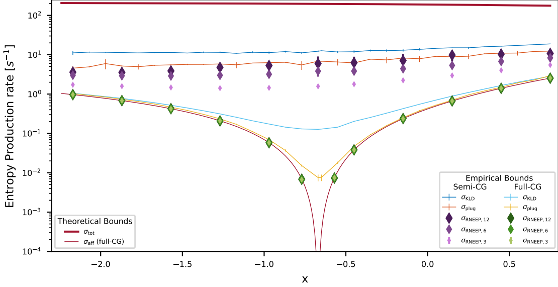
FIG. 3. Entropy production rates for the 4-state system. Total EPR, \sigma_{\text{tot}} (dark red), KLD estimator, \sigma_{\text{KLD}} , for the semi-CG (dark blue) and full-CG (light blue) data, Plug-in estimator, \sigma_{\text{plug}} , for the semi-CG (dark orange) and full-CG (light orange), RNEEP estimator, \sigma_{\text{RNEEP},m} , for the semi-CG (light to dark purple for increasing sequence length m ) and full-CG (light to dark green for increasing sequence length m ) data, and the affinity contribution, \sigma_{\text{aff}} , for the full-CG data (red). Rates: \bar{\omega}_{12} = 2s^{-1} , \bar{\omega}_{21} = 3s^{-1} , \omega_{13} = 0s^{-1} , \omega_{14} = 1s^{-1} , \omega_{23} = 2s^{-1} , \omega_{24} = 35s^{-1} , \omega_{31} = 0s^{-1} , \omega_{32} = 50s^{-1} , \omega_{34} = 0.7s^{-1} , \omega_{41} = 8s^{-1} , \omega_{42} = 0.2s^{-1} , \omega_{43} = 75s^{-1} .
