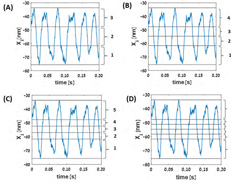
Figure S2. Coarse-graining of the hair bundle tip position ( X_1 ) for parameter values F_{max} = 70 \text{ pN} , S = 1 , T_{eff} = 1.5 \text{ T} . The index numbers on the right side of each panel indicate the number of the coarse-grained states: (A) 3 CG states (1:1:1 division), (B) 4 CG states ( 1:\frac{1}{2}:\frac{1}{2}:1 division) (C) 5 CG states ( 1:\frac{1}{3}:\frac{1}{3}:\frac{1}{3}:1 division) and (D) 6 CG states ( 1:\frac{1}{4}:\frac{1}{4}:\frac{1}{4}:\frac{1}{4}:1 division). Panels (B), (C), and (D) show coarse-graining with unequal division of the X_1 trajectory as mentioned in the main manuscript. The top and bottom borders are determined by the extremum values of the X_1 parameter.
