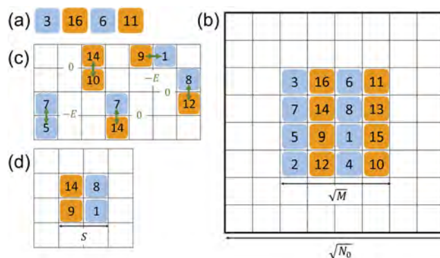
FIG. 1. Lattice model for M = N = 16 . The blue squares represent \alpha -subunits, the orange squares represent \beta -subunits, and the numbers represent the different species. (a) A possible target chain. (b) A possible target structure, containing the target chain from (a). The bold line represents the lattice borders. (c) Examples for interaction energies between pairs of particles, assuming that the target structure from (b) is the only one encoded. The interaction energy is non-zero only if the two particles are in the same configuration as in a certain target structure, including the same directionality. (d) A seed of the target structure from (b), which is the initial state of the lattice in our simulations.
