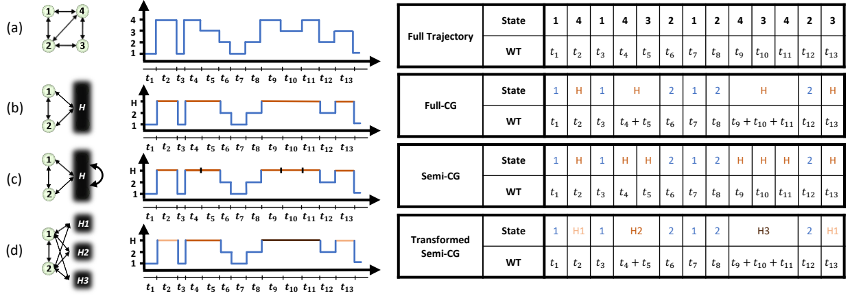
FIG. 1. Illustration of the partial information frameworks for arbitrary 4-states system. (a) A fully-observed 4-states system. The trajectory (blue line) is described by the sequence of microstates and the corresponding waiting times (WT). (b) Full coarse graining ( full-CG ). States 3 and 4 cannot be resolved, and are lumped together to a single macrostate H (orange line) (c) Semi-coarse graining ( semi-CG ). States 3 and 4 cannot be resolved, but intra-transitions between the hidden microstates can be recorded, where consecutive visits in the hidden microstates (orange line with black markers) are recorded as sequence of H , with the corresponding WT of each hidden microstate between intra-transition events. (d) Transformed Semi-coarse graining ( Transformed semi-CG ). Each n consecutive visits to the hidden microstates in H are recorded as H_n (light orange, orange, and brown represent different sequence lengths) and the WT in H_n are the sum of the WT in consecutive visits in the hidden microstates 3 and 4.
