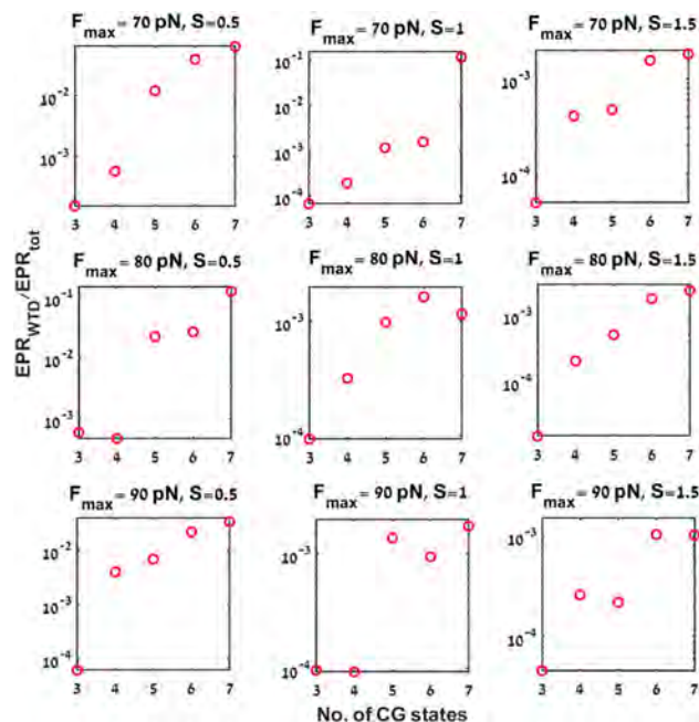
Fig. 6 Tightness of the EPR bound ( EPR_{WTD} ) as a function of number of CG states: ratio between the EPR estimates from the waiting time distribution ( EPR_{WTD} ( s^{-1} )) and the total entropy production rate ( EPR_{tot} ( s^{-1} )) for different parameter values. The coarse-graining corresponds to unequal divisions of the X_1 state space. The parameter values are F_{max} = 70 pN, S = 0.5, 1, 1.5 (upper row), F_{max} = 80 pN, S = 0.5, 1, 1.5 (middle row), F_{max} = 90 pN, S = 0.5, 1, 1.5 (lower row). The other parameter values used in this figure are as mentioned in Fig. 1.
