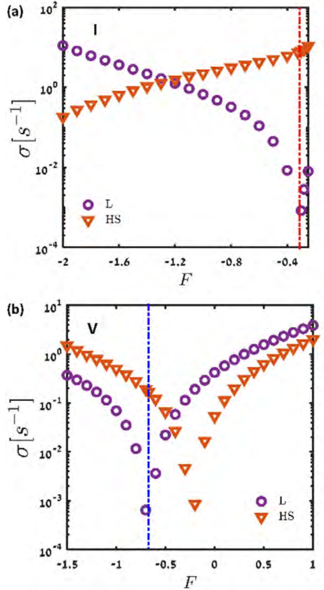
Figure 4. Comparison between two lumping methods (L and HS) for (a) network topology I and (b) network topology V. The parameter values are the same as given in figure 1. The red downward triangles denote the HS method, and the purple circles refer to the L method. The stalling forces are labeled with dashed-dotted (a) red line for topology I, and (b) blue line for topology V.
