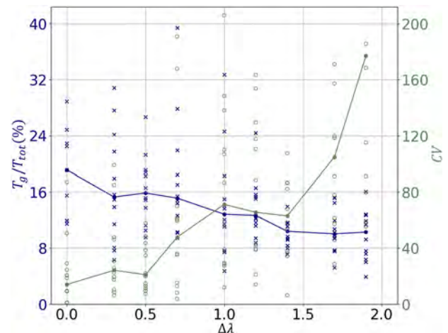
FIG. 7. Two quality parameters for varied drive intensity, \Delta\lambda : characteristic growth time, normalized by the total number of MC steps (blue) and chimeric value (green). Each “x” or “o” symbol represents one simulation, and each point represents the median of 12 simulations.
