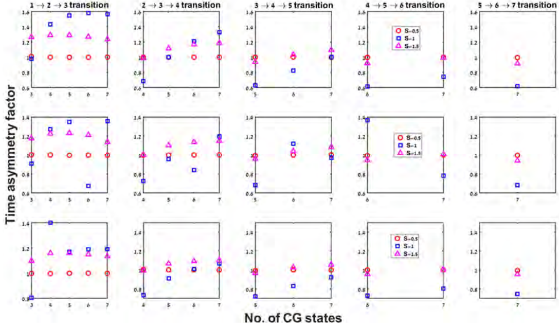
Figure S3. The mean dwell-time asymmetry factors (MDAF, \langle \tau_{kji} \rangle / \langle \tau_{ijk} \rangle ) as a function of the number of coarse-grained states for different transitions (shown in the subtitles) between the coarse-grained states for different parameter values: F_{max} = 70 \text{ pN} (upper panel), F_{max} = 80 \text{ pN} (middle panel), F_{max} = 90 \text{ pN} (lower panel), S = 0.5 (red open circles), S = 1 (blue open square), S = 1.5 (magenta open triangle), and T_{eff} = 1.5 T . All other parameter values are the same as mentioned in Figure 1 in the main text.
