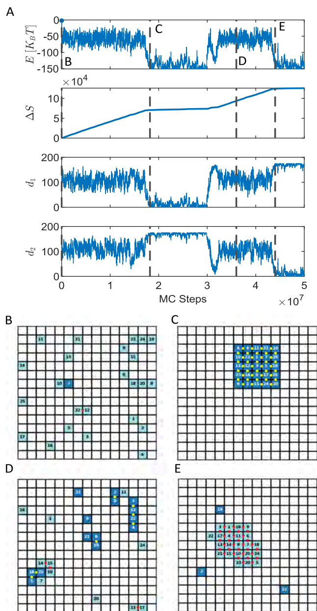
Figure 2. Simulation trajectories. (A) Energy E , total entropy production \Delta S , and the distance from the two stored targets, d_1 and d_2 , are plotted as a function of the MC steps. The vertical dashed lines indicate selected time points along the realization, corresponding to (B) initial conditions, (C) the first self-assembly event of target 1, (D) a potential kinetic trap characterized by energy fluctuations around a value higher than the global minima, and (E) approaching the successful self-assembly of target 2. The corresponding lattice states are plotted.
