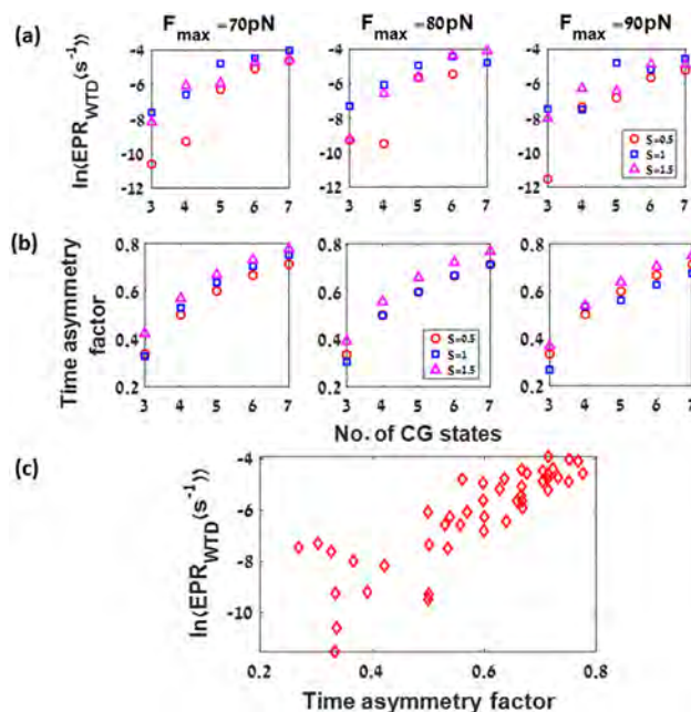
Fig. 5 Effect of coarse-graining on the \text{EPR}_{\text{WTD}} ( \text{s}^{-1} ) and the mean dwell-time asymmetry factor (MDAF): (a) \text{EPR}_{\text{WTD}} ( \text{s}^{-1} ) as a function of number of CG states (3 CG: 1:1:1, 4 CG: 1:1/2:1/2:1, 5 CG: 1:1/3:1/3:1/3:1, 6 CG: 1:1/4:1/4:1/4:1/4:1, and 7 CG: 1:1/5:1/5:1/5:1/5:1/5:1) for different parameter values, (left) F_{\text{max}} = 70 pN for S = 0.5, 1, 1.5 , (middle) F_{\text{max}} = 80 pN for S = 0.5, 1, 1.5 , and (right) F_{\text{max}} = 90 pN, S = 0.5, 1, 1.5 . (b) The MDAF as a function of number of CG states for different parameter values: (left) F_{\text{max}} = 70 pN, S = 0.5, 1, 1.5 ; (middle) F_{\text{max}} = 80 pN, S = 0.5, 1, 1.5 ; (right) F_{\text{max}} = 90 pN, S = 0.5, 1, 1.5 . In both panels: red circle symbols correspond to S = 0.5 , blue square symbols correspond to S = 1 , and magenta triangle symbols correspond to S = 1.5 . (c) The values of \text{EPR}_{\text{WTD}} as a function of the MDAF for all transitions and all parameter values as mentioned earlier. The other parameter values used in these figures are mentioned in Fig. 1.
