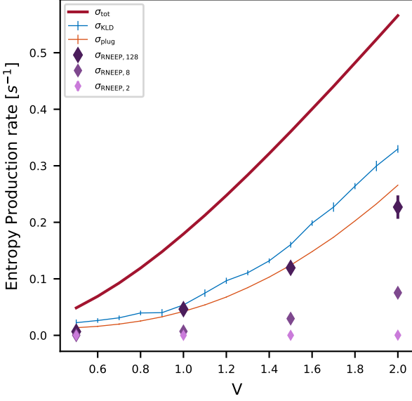
FIG. 4. Entropy production rates for the flashing ratchet. Total EPR, \sigma_{\text{tot}} (dark red) of the full trajectory, KLD estimator, \sigma_{\text{KLD}} (dark blue), Plug-in estimator, \sigma_{\text{plug}} (dark orange), and RNEEP estimator, \sigma_{\text{RNEEP},m} (light to dark purple for increasing sequence length m ) for semi-CG data. The transition rates for \forall i \neq j are: \omega_{ii'} = \omega_{i'i} = \omega_{i'j'} = 1 , \omega_{ij} = e^{(V_j - V_i)/2} , where states i ( i' ) are with turned-on (off) potential.
