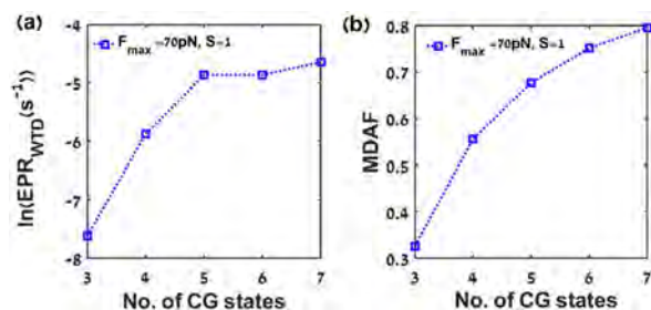
Fig. 4 Entropy production rate estimation and the mean dwell-time asymmetry factor (MDAF) for equal spacing coarse-graining of X_1 trajectory: (a) \text{EPR}_{\text{WTD}} ( \text{s}^{-1} ) (WTD estimate of the EPR) as a function of the number of CG states with equal spacing for parameter values F_{\text{max}} = 70 pN, S = 1 , and T_{\text{eff}}/T = 1.5 (b) MDAF (mean dwell-time asymmetry factor) as a function of the number of CG states. The other parameter values are the same as mentioned in Fig. 1. The lines are drawn to as a guide to the eye. The total EPR for this set of parameter values is 7.3312 \text{ s}^{-1} .
