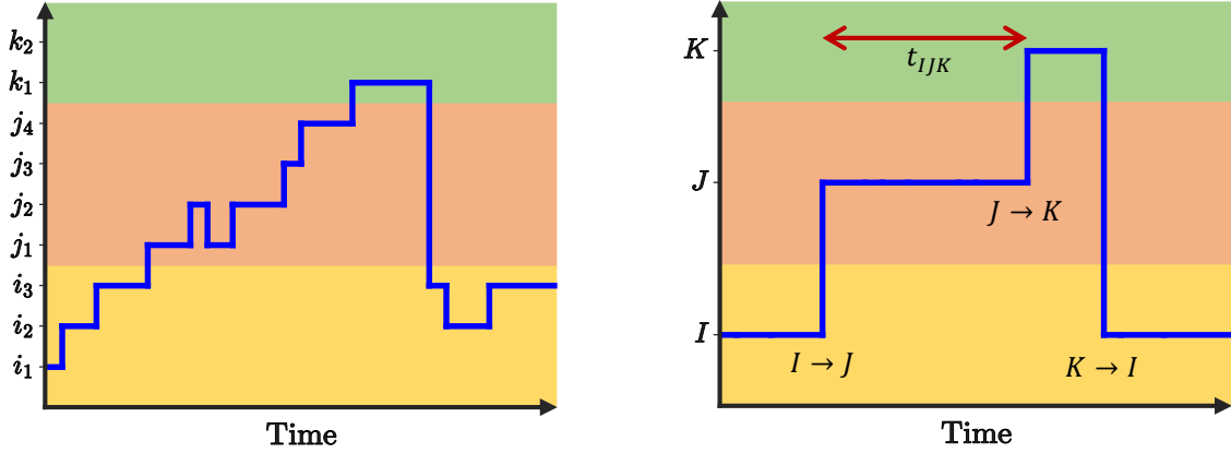
FIG. 1. Coarse graining. (a) The full Markovian system (left) and the coarse-grained system (right). (b) An example for a full trajectory (left) containing the actual states and the corresponding coarse-grained trajectory (right) containing only the observed states.
