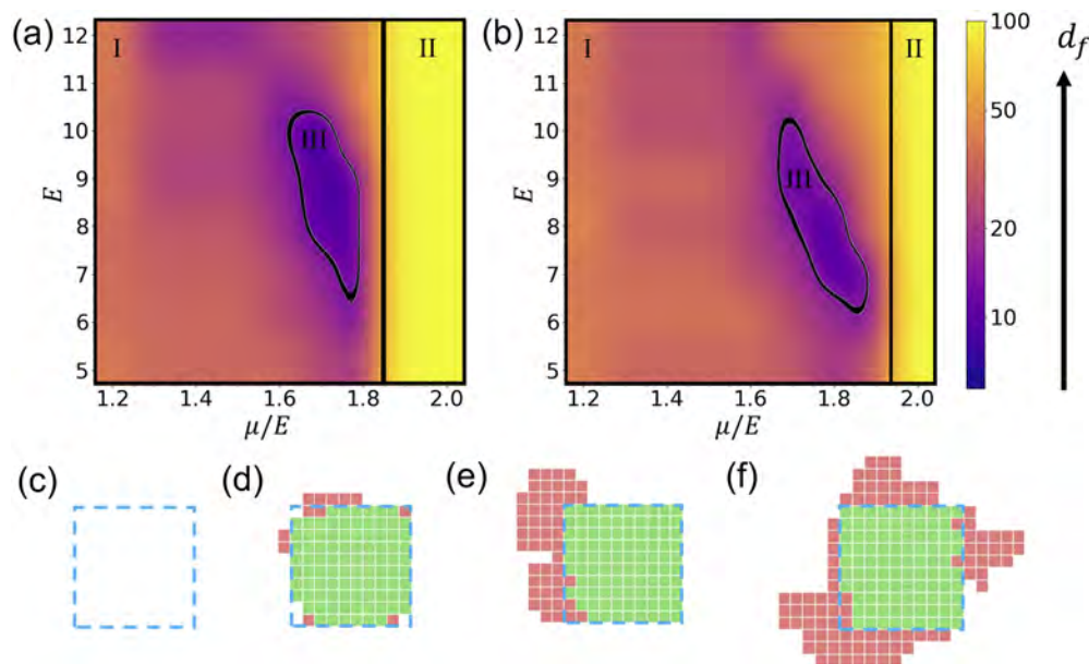
FIG. 4. (a) and (b) Final distance from the seeded target as a function of \mu/E and E at equilibrium ( \Delta\lambda = 0 ) (a) and nonequilibrium ( \Delta\lambda = 1 ) (b), following Gaussian interpolation. Colors represent final distances in a logarithmic scale. Each data point is averaged over ten realizations (see the supplementary material , Sec. S6). [(c)–(f)] The state of the lattice by the end of the simulation on the boundaries of nonequilibrium regime III, colored as described in Fig. 3. (c) Right boundary (namely, \mu/E and E values, which correspond to the right boundary of nonequilibrium regime III) at equilibrium: E = 7 , \mu/E = 1.9 , \Delta\lambda = 0 . (d) Right boundary out-of-equilibrium: E = 7 , \mu/E = 1.9 , \Delta\lambda = 1 . (e) Left boundary at equilibrium: E = 8 , \mu/E = 1.7 , \Delta\lambda = 0 . (f) Left boundary out-of-equilibrium: E = 8 , \mu/E = 1.7 , \Delta\lambda = 1 .
