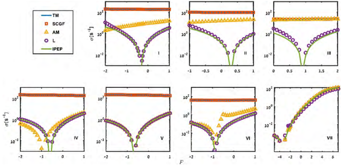
Figure 2. Mean EPR estimation from the total mean (TM) or \sigma^{\text{TM}} , scaled cumulant generating function (SCGF or \sigma^{\text{SCGF}} ), from approximated master equation (AM or \sigma^{\text{AM}} ), lumping by preserving the transition flux and steady-state probabilities (L or \sigma^{\text{L}} ), informed partial entropy production (IPEP or \sigma^{\text{IPEP}} ) for different network topologies. The parameter values for each subplot (network topology, I–VII) are the same as mentioned in figure 1. The ranges of the x-axes were chosen to include the stall force and to show the behavior of the estimators around and away from it.
