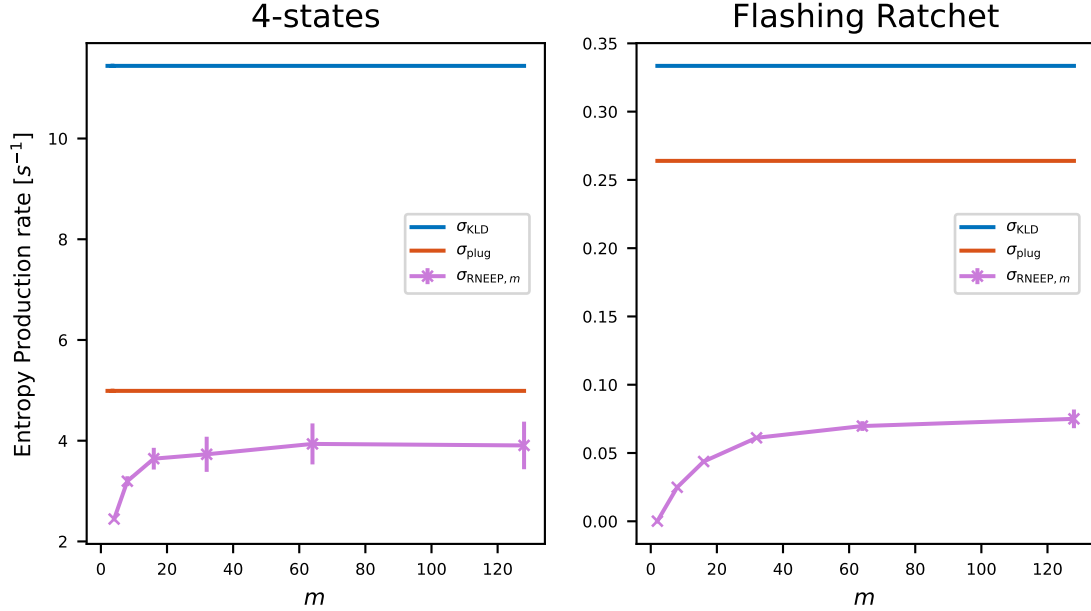
Fig. S2. Convergence of \sigma_{\text{RNEEP},m} as a function of m (purple) for semi-CG data, compared to the values of the \sigma_{\text{KLD}} (blue diamo), and \sigma_{\text{plug}} (orange), which do not depend of m , for the 4-state system with x = -2.17 (left) and for the Discrete Flashing Ratchet with V = 2 (right).
