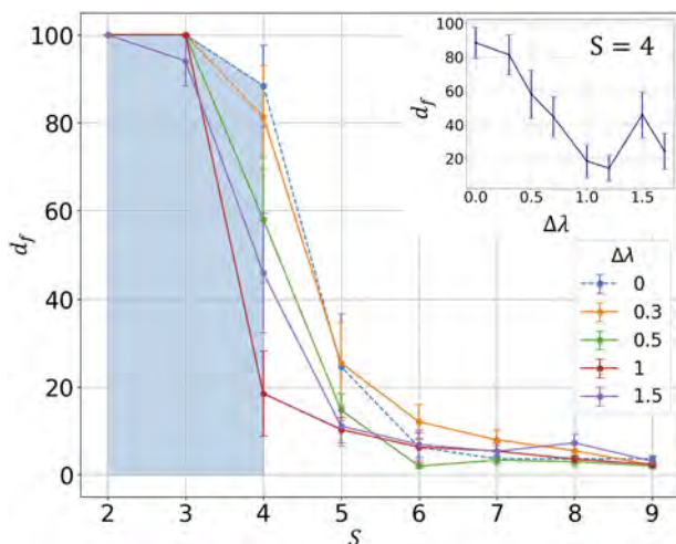
FIG. 6. Final distance from the desired target structure as a function of seed length. The blue area is the sub-critical seed region. The inset shows the final distance for the maximal equilibrium sub-critical seed, S = 4 < S_c , as a function of the drive value. Each point is the average value over ten simulations, with the error bars representing the statistical error.
