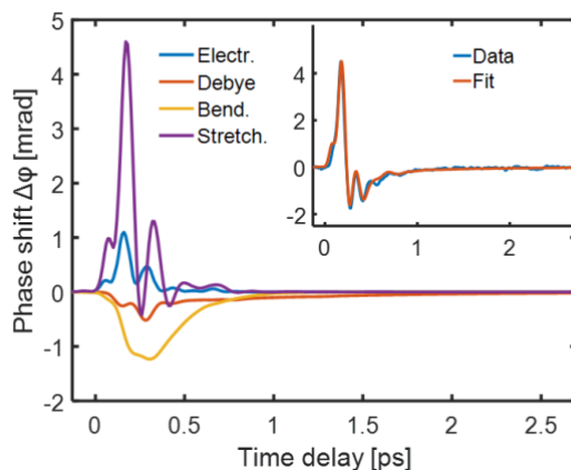
Figure 15. Simulation of the TKE response. [85] The simulation results of the TKE response in the time domain for the electronic (Electr.), Debye relaxation (Debye), hydrogen bond bending vibration (Bend.) and hydrogen bond stretching vibration (Stretch.) contributions. Inset: a comparison between the sum of all the contributions and the measured data.
