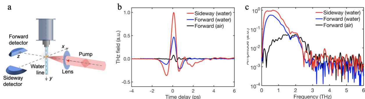
Figure 8. Comparison of forward and sideways detection. a Setup schematic for forward and sideways detection. The pump beam is along z -axis. The water line flows in y direction. Two EO detectors are in z and -x directions, respectively. b Comparison of THz waveforms. The pulse energy is 0.4 mJ. Corresponding spectra are shown in c .
