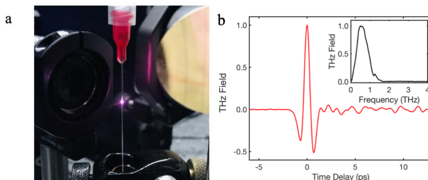
Figure 5. THz generation from liquid water under single-color ionization. a A photo of a fluorescence from a laser induced micro-plasma of a water line. b A typical THz waveform generated from a water line and its corresponding spectrum (inset).
