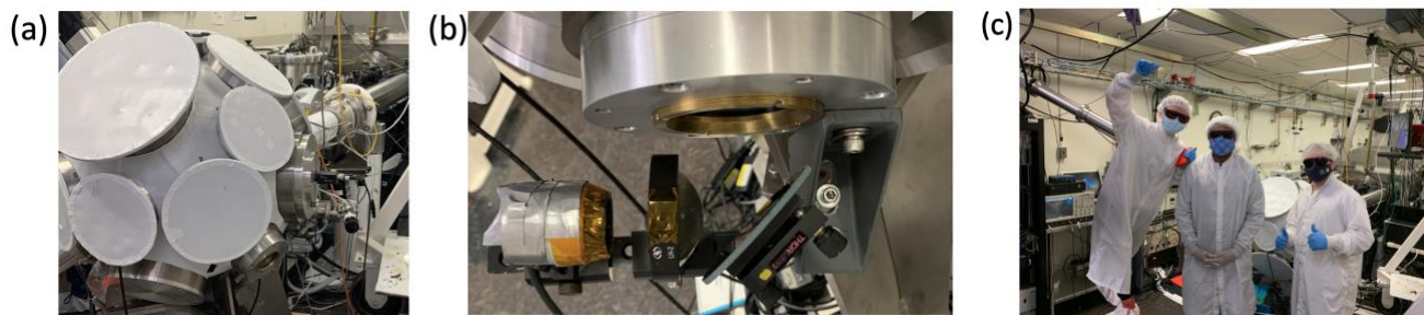
Figure 19. (a) The target chamber for THz wave generation using a multi-terawatt laser at LLE, Rochester. (b) THz detection from one of the chamber windows. (c) PhD students, Gerrit Bauhuag (right) and Kareem Garriga (middle) and Research Associate Dr. Yiwen E (left) in the testing room.
