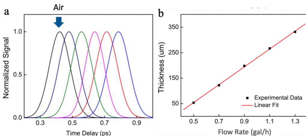
Figure 3. Calibration of the water film thickness. a The original (air) signal from the autocorrelation system is plotted in the black line. With the water film in one of the two beams of the autocorrelation system, the signal peak will move linearly with the increase of thickness. b The linear dependence of the thickness on the flow rate. The thickness of the water film can be continuously tuned from 50 \text{ }\mu\text{m} to 350 \text{ }\mu\text{m} .
