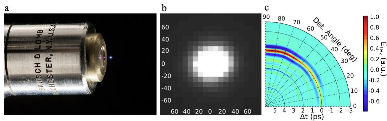
Figure 4. Micro-plasma and the signal distribution. [34] a A photo of the micro-plasma fluorescence obtained by focusing the laser beam with a high NA microscope objective. b A magnified image of the micro-plasma (unit is \mu\text{m} ). However, the plasma spot's contribution to the THz wave is about one \mu\text{m} or less. c Measured THz field as a function of the THz emission angle. The optimal angle is 80 degree from laser propagation direction.
