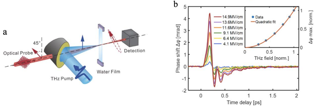
Figure 14. Terahertz Kerr effect (TKE) in a water film. [85] a. Diagram of the experimental setup. An intense THz pulse is focused onto a free-standing water film. The THz field induced Kerr effect is detected through an optical probe. b. TKE with different THz peak field strengths. Inset: THz field strength dependence.
