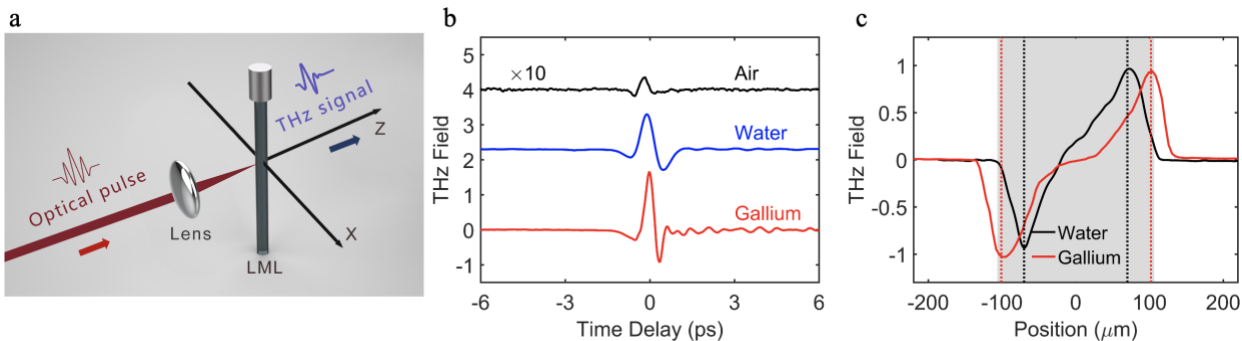
Figure 11. THz generation from liquid Gallium. [71] a Schematic of the experimental setup. A two-dimensional translation stage is used to control the position of the x-axis and the z-axis of the liquid metal line. The optical beam propagates along the z-axis. THz emission is measured by a standard electro-optical sampling. b Comparison of THz waveforms generated from air, water and liquid gallium under single-color excitation. The target diameter is 210 μm. The signal from air plasma is enlarged by 10 times. c Normalized THz field strength as a function of the x-axis position. The dashed lines represent the x-axis position of the maximum THz fields. The gray area shows the diameter of the liquid line.
