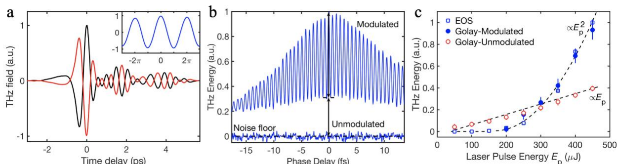
Figure 9. THz generation from liquid water under two-color excitation. [13] a Two THz waveforms obtained when the relative phase is \pi and 2\pi . Inset, THz electric field as a function of the phase delay. b THz wave energy with a tuned phase between 800 nm and 400 nm pulses. The THz energy was monitored by a Golay cell. c Normalized THz energy from liquid water as a function of the total excitation laser pulse energy. Blue squares show the THz energy calculated from the temporal integral of the THz waveform measured by EOS. Blue dots indicate modulated THz energy measured by a Golay cell. Red circles present unmodulated THz energy measured by the Golay cell.
