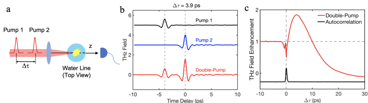
Figure 13. THz generation under double-pump excitation. [79] a Schematic of double pump excitation. Two optical pumps propagating collinearly with a certain time delay \Delta\tau are focused on a water line (top view). \Delta\tau is controlled by a delay stage. The THz signal is detected through EOS. b THz waveforms generated by pump 1 (black line) and pump 2 (blue line), respectively. The bottom red line shows the waveform generated by two pumps when \Delta\tau is 3.9 ps. c The red line shows the dynamic of the THz peak field versus \Delta\tau . The black line plots the autocorrelation signal of the two pumps, from which the 0 timing is determined. \Delta\tau > 0 means that the pump 1 ionizes the target first.
