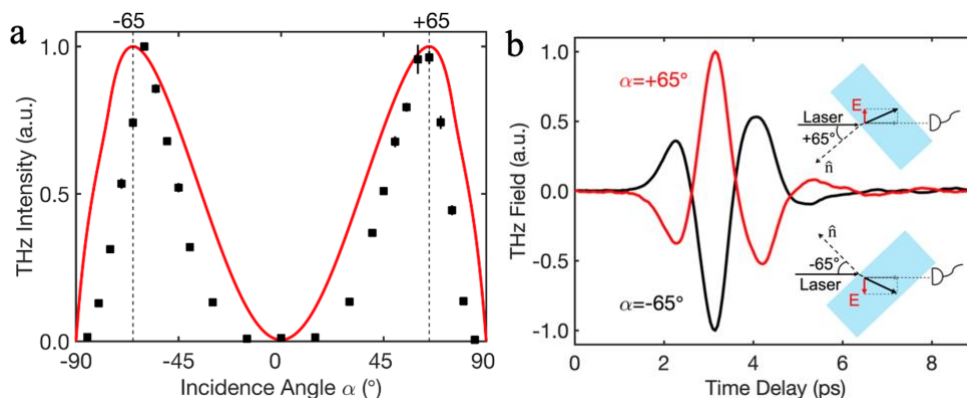
Figure 6. The dependence of THz signal on the incidence angle \alpha . [10, 12] a THz intensity with different incidence angles is studied by rotating the water film. The signal is maximized when \alpha is 65^\circ . The squares are the experimental results, and the red line is a simulated result from a dipole model. b The waveforms show optics polarities with opposite incidence angle. The insets explain the observation with a contribution of the flipped dipole projection (E) of opposite incidence angles.
