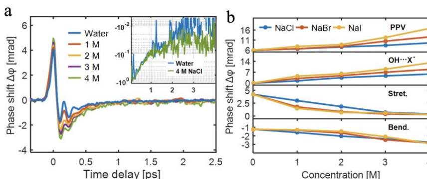
Figure 16. Terahertz Kerr effect response on different concentrations. [89] a TKE responses of water and NaCl solutions with different concentrations. Inset: an enlarged logarithmic view of the negative polarity responses. b The upper panel shows the measured peak-to-peak values (PPV) of TKE responses for NaCl, NaBr, NaI solutions with different concentrations. The other panels show the extracted maximum values of TKE responses induced by \text{OH}\cdots\text{X}^- hydrogen bond vibration ( \text{OH}\cdots\text{X}^- ), the hydrogen bond bending (Bend.), and hydrogen bond stretching modes (Stret.).
