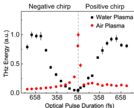
Figure 7. Normalized THz energy with different optical pulse durations. [10] THz signal generated by water plasma prefers an optical excitation with a longer pulse duration. However, the generation from air plasma is always in favor of the shortest pulse.
