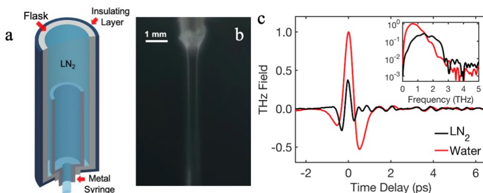
Figure 10. THz generation from liquid nitrogen. [67] a Diagram of the apparatus for guiding an LN 2 line. By filling it with LN 2 , the liquid in the flask prevents the liquid in the syringe transferring heat. b A photo of a flowing LN 2 line in an ambient environment. The transparency of the line indicates the liquid phase clearly with a smooth surface. c Comparison of THz waveforms from water and LN 2 under the same optical excitation. Inset: Corresponding spectra.
