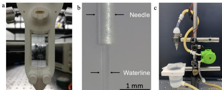
Figure 2. Liquid targets and the liquid system. a A gravity-driven water film. The thickness is 210 \text{ }\mu\text{m} . b A pump-driven water line with a diameter of 260 \text{ }\mu\text{m} , which is guided by a syringe needle. c A home-built liquid system, which needs only 50 ml water for several hours running. A syringe is used as a jet for producing a liquid line.
