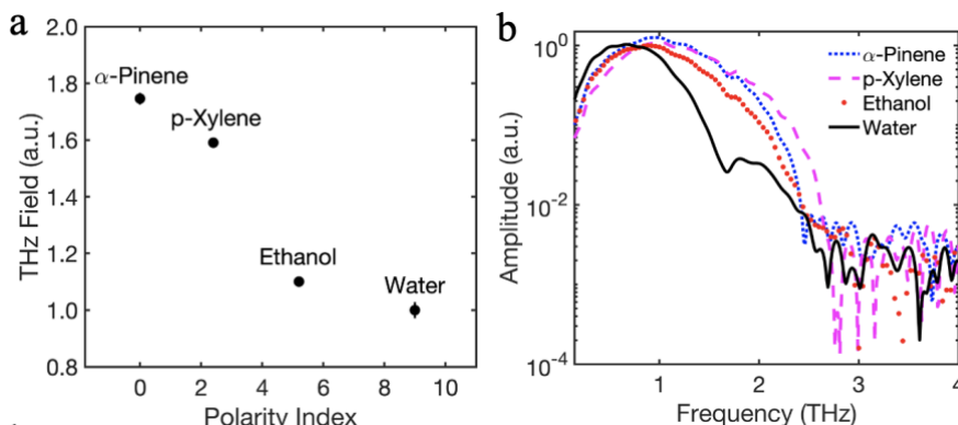
Figure 12. THz generation from liquids with different polarity indices. a THz fields generated from four liquids, which are \alpha -pinene, p-xylene, ethanol, and water. Their polarity indices are 0, 2.4, 5.2, and 9, respectively. b Corresponding spectra.
