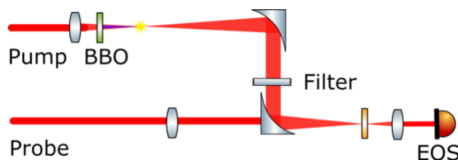
Figure 1. A typical THz two-color air plasma system. The laser beam is split into pump beam and probe beam. The air plasma is produced by focusing the pump beam. One BBO crystal is inserted to create the second harmonic pulse. The THz signal is detected through electro-optic sampling (EOS).
