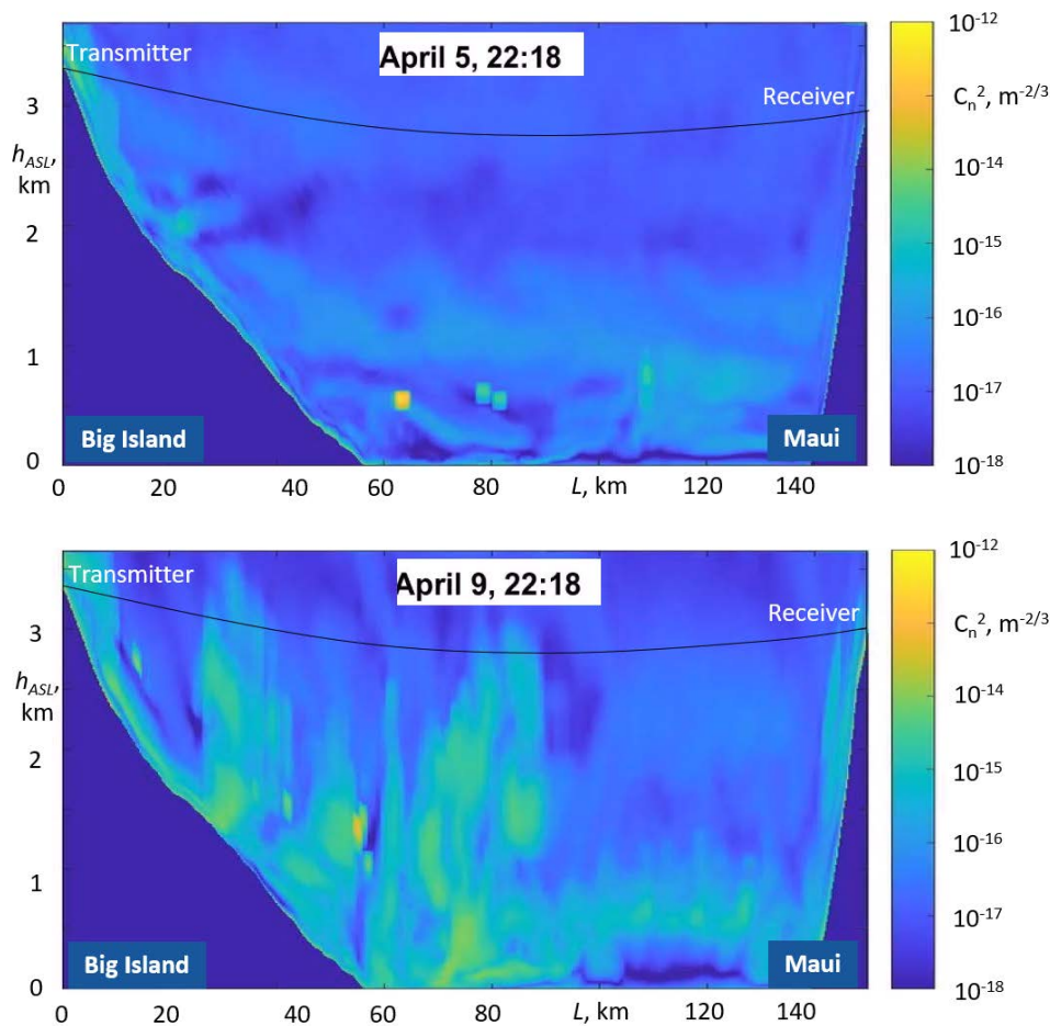
Figure 6. Refractive index structure constant ( C_n^2 ) distributions along the ERCAOS propagation path between a transmitter at Hawaii (Big Island) and receivers at Maui obtained from WRF simulations for April 5 and 9, 2019 (top and bottom panels, respectively). The line near the top indicates the optical propagation path, which is shown curved because its height above sea level varies, mainly due to the Earth's curvature. The simulations confirm the much stronger turbulence observed on April 9 in comparison to conditions on April 5.
