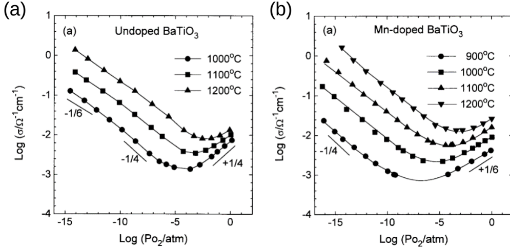
Figure 2.6 Electrical conductivity of (a) undoped BaTiO 3 and (b) Mn-doped BaTiO 3 vs. oxygen partial pressure at different temperatures. Reproduced with permission from [43].
