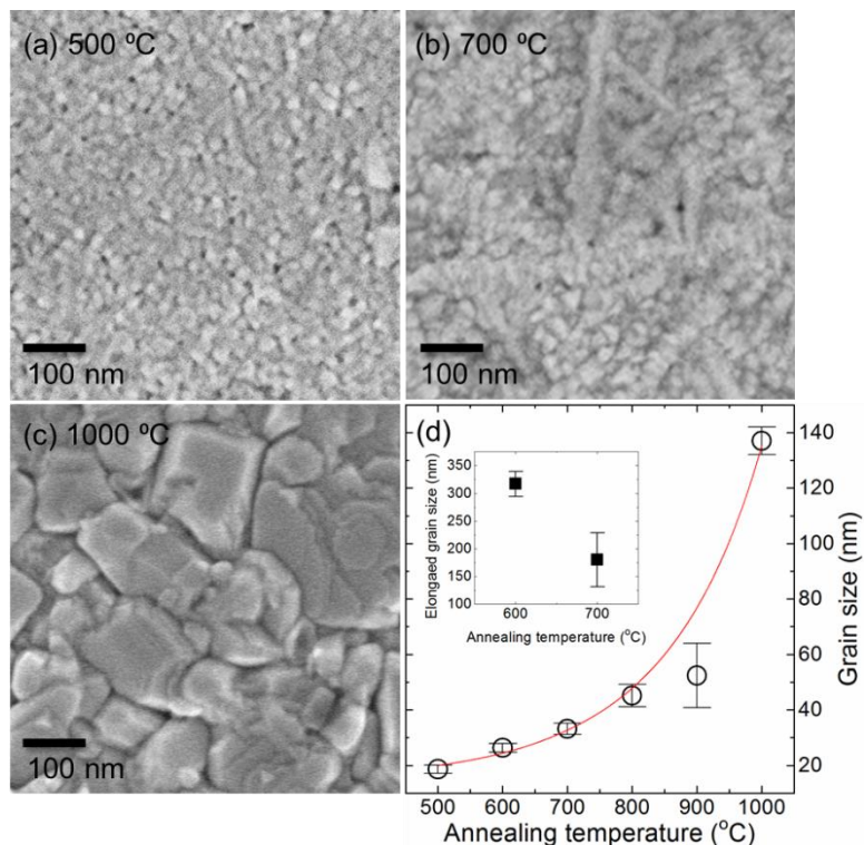
Fig. 3. Surface images of BaTiO 3 thin films isothermally annealed at (a) 500 °C, (b) 700 °C and (c) 1000 °C, and (d) grain size variation versus annealing temperature.
