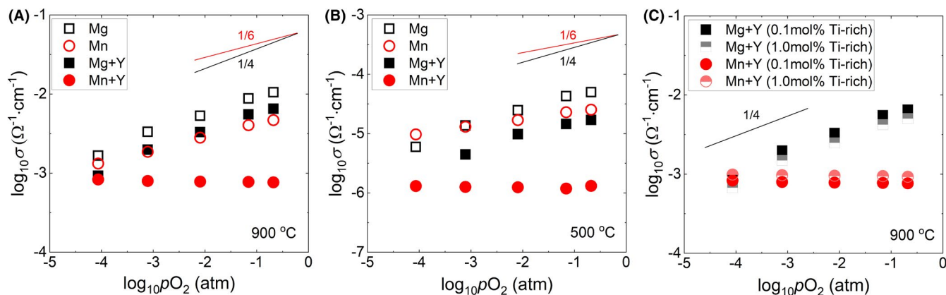
FIGURE 1 DC electrical conductivity as a function of oxygen partial pressure in doped BaTiO 3 with 0.1 mol% Ti-rich at (A) 900°C and (B) 500°C. (C) The comparison of high-temperature DC electrical conductivity with respect to the amount of Ti-excess
