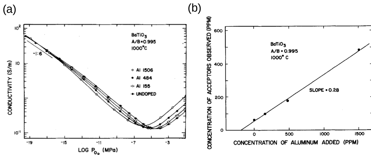
Figure 2.5 (a) Equilibrium electrical conductivity of undoped and Al-doped BaTiO 3 at 1000°C. (b) Apparent net acceptor concentration derived from conductivity data, compared with the amount of added Al. Reproduced with permission from [40].
