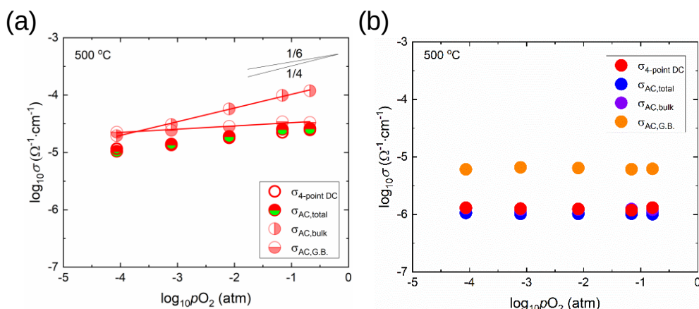
Figure 7.3 DC and AC electrical conductivities versus pO_2 of (a) 0.5 mol% Mn-doped and (b) (0.5 mol% Mn and 0.5 mol% Y) co-doped BaTiO 3 at 500 °C.
