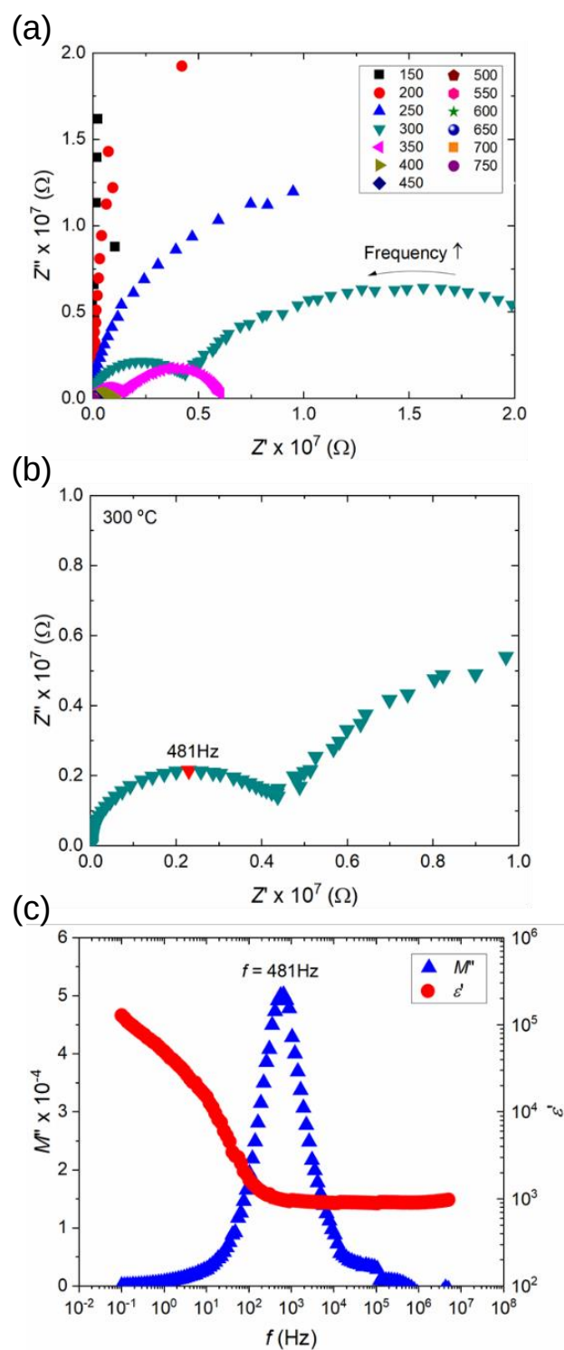
Figure 4.3 (a) Cole-Cole plot of Mn-doped BaTiO 3 as a function of temperature. (b) High-frequency arc and (c) corresponding imaginary part of modulus and real part of relative permittivity at 300 °C.
