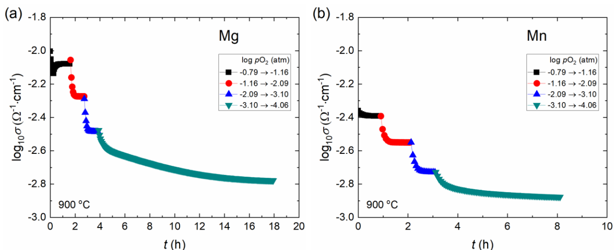
Figure 4.1 Time-dependent DC electrical conductivity at various oxygen partial pressure in (a) Mg-doped BaTiO 3 and (b) Mn-doped BaTiO 3 at 900 °C.
