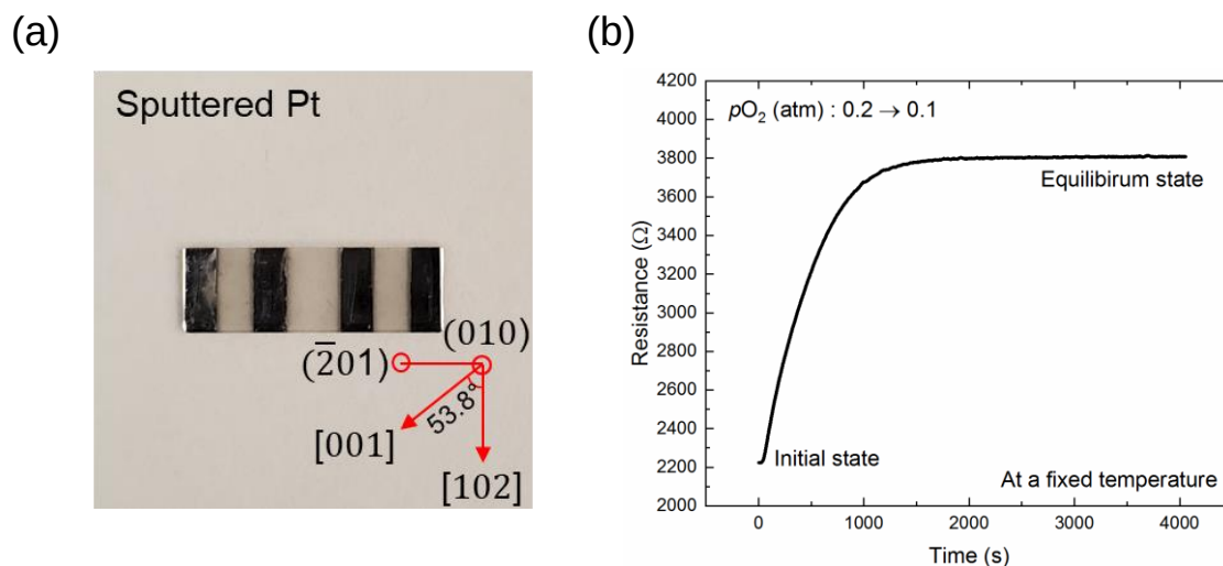
Figure 3.2 (a) Top view of Fe-doped (010) \beta\text{-Ga}_2\text{O}_3 single crystal and sputtered Pt electrodes the black arrow indicates the measurement direction (b) time-dependent four-wire resistance with a change in p\text{O}_2 at a given temperature.
