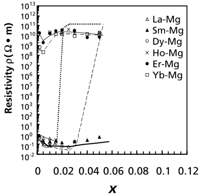
Figure 2.13 Room temperature resistivities of (\text{Ba}_{1-2x}\text{R}_{2x})(\text{Ti}_{1-x}\text{Mg}_x)\text{O}_3 sintered at 1380 °C in a reducing atmosphere as a function of x ( \text{R} = \text{La}, \text{Sm}, \text{Dy}, \text{Ho}, \text{Er} or \text{Yb} ). Reproduced with permission from [14].
