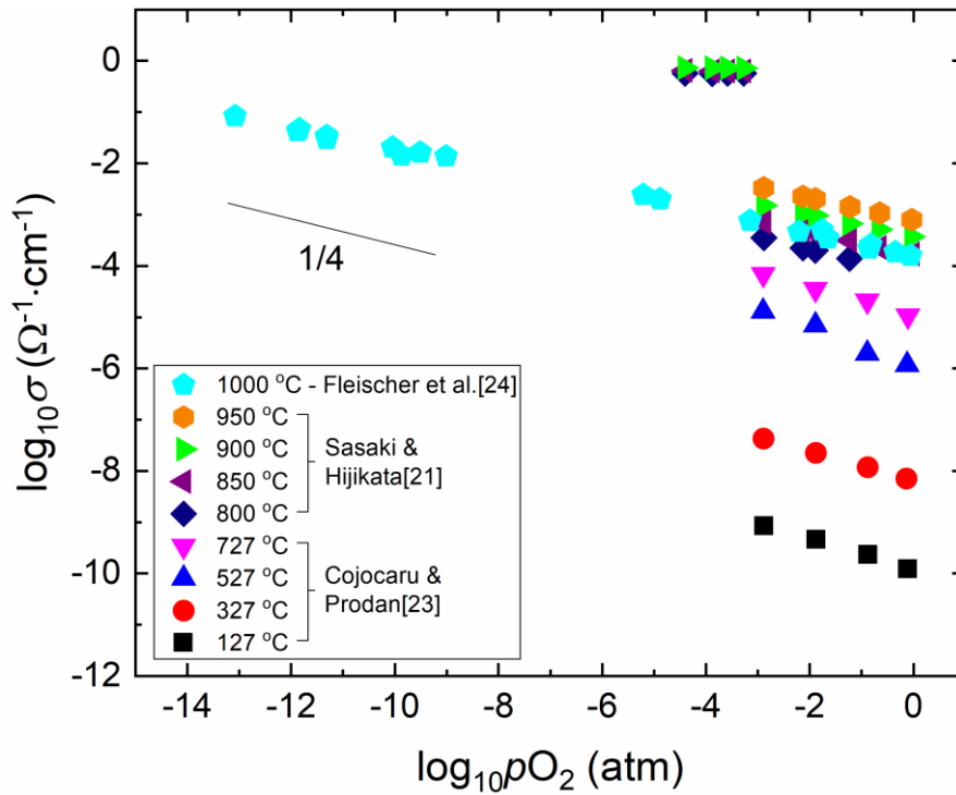
Figure 6.1 Electrical conductivity versus oxygen partial pressure in unintentionally doped \beta -Ga 2 O 3 polycrystalline.
