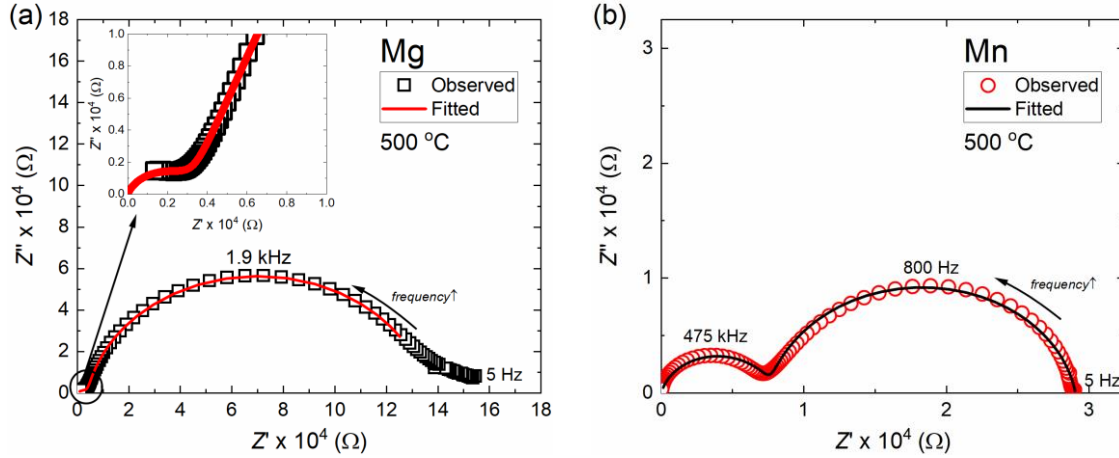
Figure 4.5 Observed and fitted Cole-Cole plots of (a) Mg-doped BaTiO 3 and (b) Mn-doped BaTiO 3 at 500 °C.
