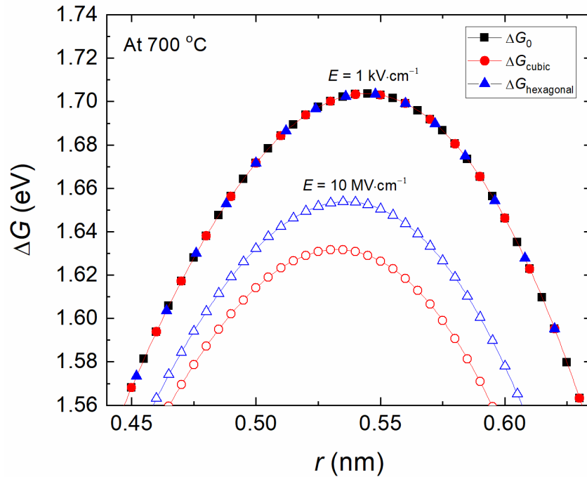
Fig. 6. Free energy change in the nucleation process as a function of cluster radius at 700 °C under 1 \text{ kV}\cdot\text{cm}^{-1} (solid symbols) and 10 \text{ MV}\cdot\text{cm}^{-1} (open symbols) electric field.
