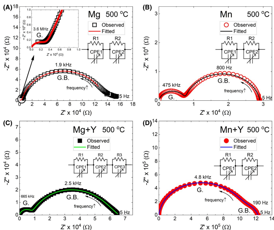
FIGURE 2 Observed and fitted Cole–Cole plots of (A) Mg-doped, (B) Mn-doped, (C) (Mg+Y) co-doped, and (D) (Mn+Y) co-doped BaTiO 3 at 500°C in air. Note that the real and imaginary parts of impedance were scaled by the sample geometry for the direct comparison of impedance magnitudes. G. and G.B. indicate the grain and grain-boundary response, respectively
