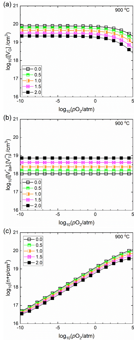
Figure 5.6 Predicted concentration of (a) oxygen vacancy, (b) cation vacancy, and (c) electronic charge carrier at 900 °C in (Mg+Y) co-doped \text{BaTiO}_3 with [Y_{Ba}]/[Mg_{Ti}^{''}] = 0.0, 0.5, 1.0, 1.5, and 2.0 .
