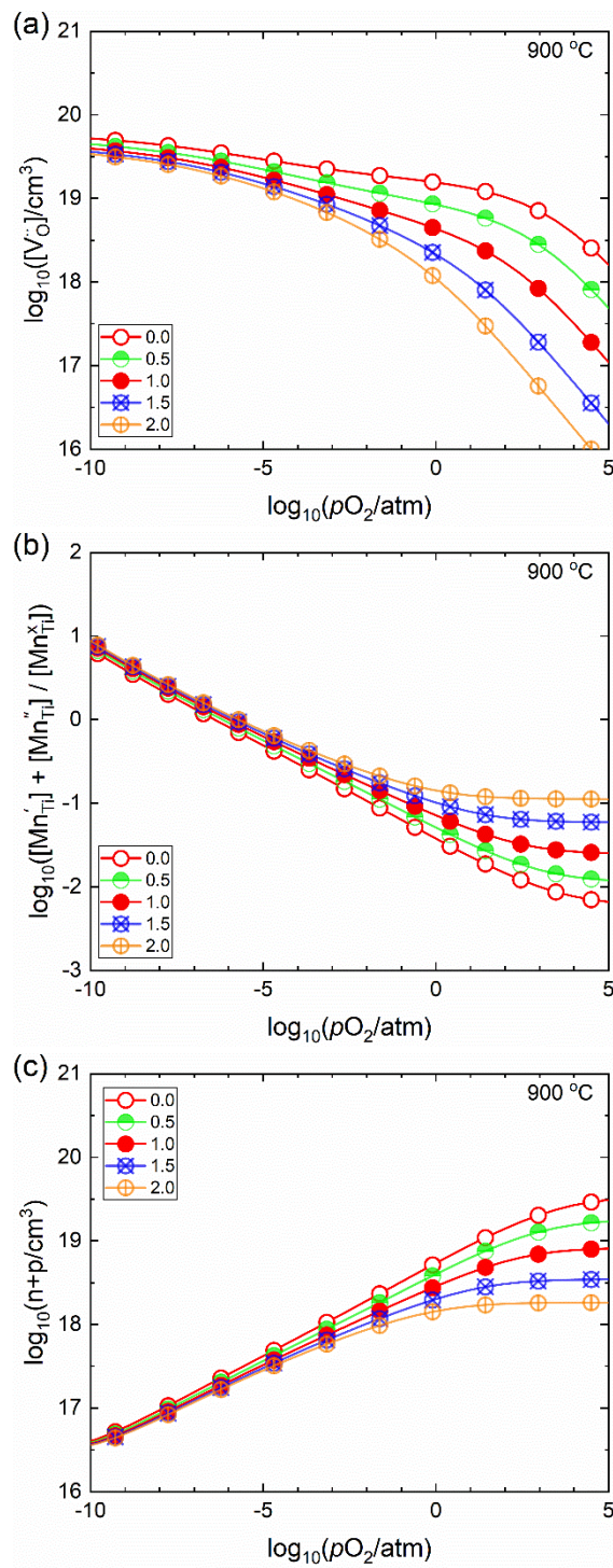
Figure 5.7 Predicted defect concentration of (a) oxygen vacancy, (b) neutral and ionized Mn, and (c) electron and hole in (Mn+Y) co-doped BaTiO 3 with [Y_{Ba}]/[Mn_{Ti}]_T = 0, 0.5, 1.0, 1.5, and 2.0 at 900 °C.
