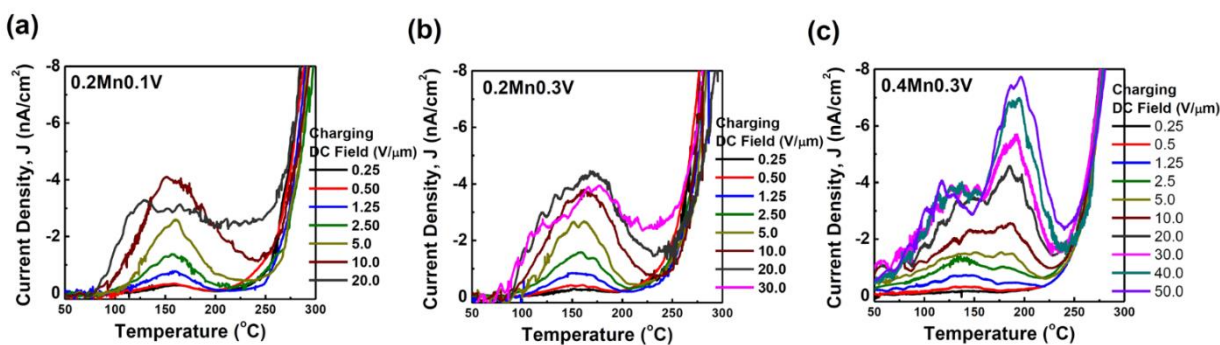
Figure 2.18 TSDC plots for Mn and V co-doped BaTiO 3 MLCC with (a) 0.2 mol% Mn and 0.1 mol% V, (b) 0.2 mol% Mn and 0.3 mol% V, and (c) 0.4 mol% and 0.3 mol% V. Reproduced with permission from [73].
