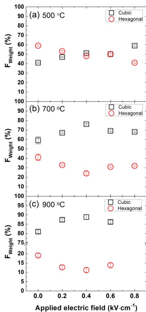
Fig. 4. Weight percent of cubic and hexagonal BT a as a function of the applied electric field in BaTiO 3 thin films during annealing process at (a) 500^\circ\text{C} , (b) 700^\circ\text{C} and (c) 900^\circ\text{C} .
