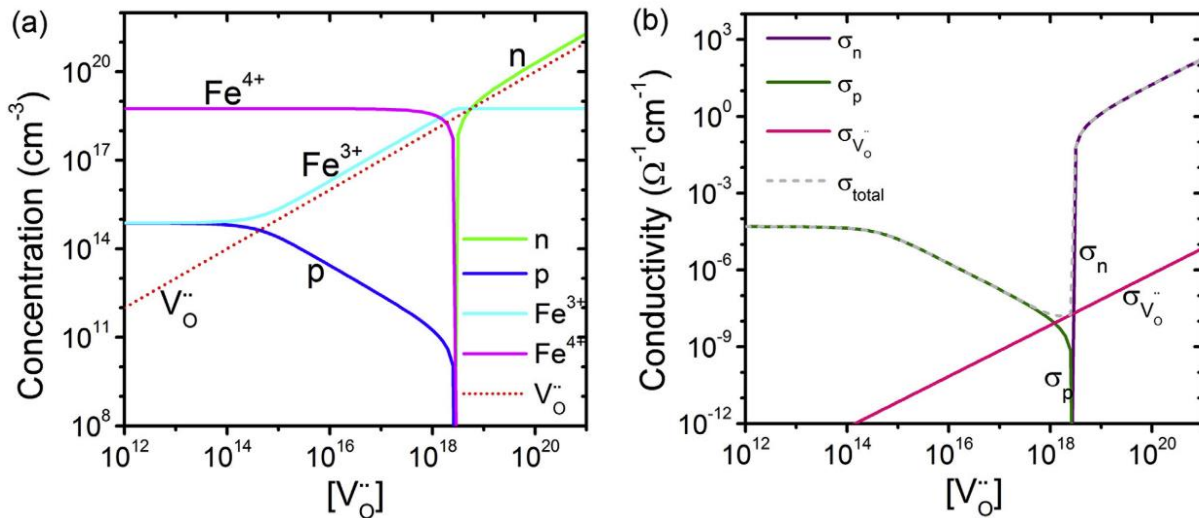
Figure 1.2 Oxygen vacancy concentration-dependent (a) electronic carrier and ionized Fe concentrations and (b) total and partial electrical conductivities of Fe-doped SrTiO 3 at 210 °C. The sample was equilibrated at 900 °C and p\text{O}_2 of 10^{-5} atm and quenched to room temperature. Reproduced with permission from [19].
