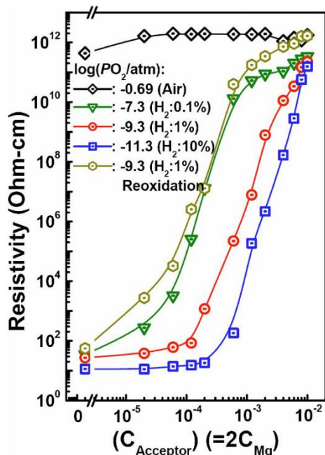
Figure 2.8 Mg concentration-dependent room temperature electrical resistivities of Mg-doped BaTiO 3 sintered in different oxygen partial pressures. Reproduced with permission from [60].
