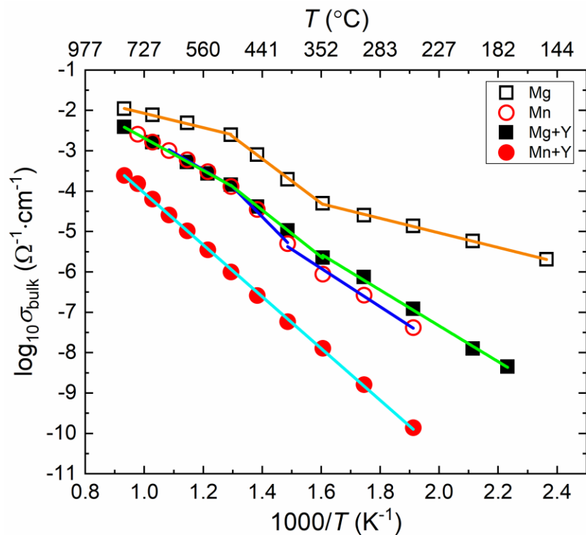
Figure 7.1 Temperature-dependent bulk conductivity of 0.5 mol% Mg-doped, 0.5 mol% Mn-doped, (0.5 mol% Mg and 1.0 mol% Y) co-doped, and (0.5 mol% Mn and 0.5 mol% Y) co-doped BaTiO 3 compositions in air.
