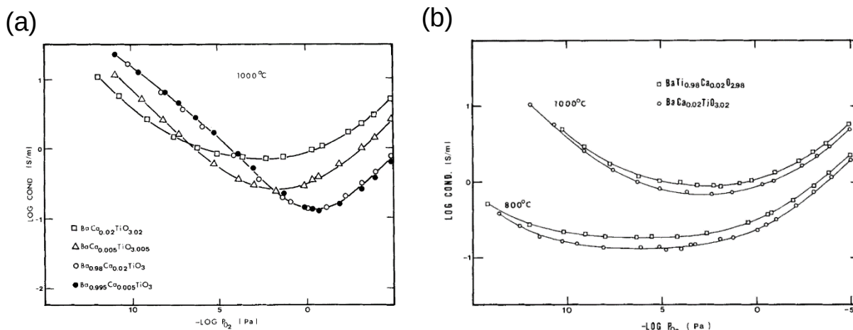
Figure 2.7 (a) Equilibrium electrical conductivity of (Ba_{1-x}Ca_x)TiO_3 and (BaTiO_3 + xCaO) with x = 0.5 mol% and 2 mol% at 1000 °C. (b) Equilibrium electrical conductivities at 800 °C and 1000 °C of (BaTiO_3 + xCaO) and Ba(Ti_{1-x}Ca_x)O_3 with x = 2 mol %. Reproduced with permission from [54].
