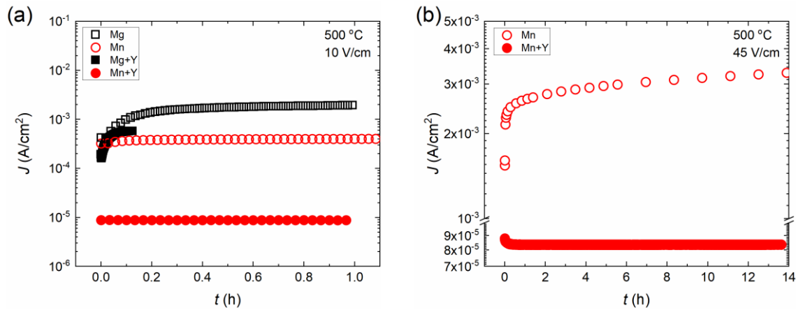
Figure 5.5 Time-dependent current density at 500 °C under (a) 10 V/cm and (b) 45 V/cm DC electric field.
