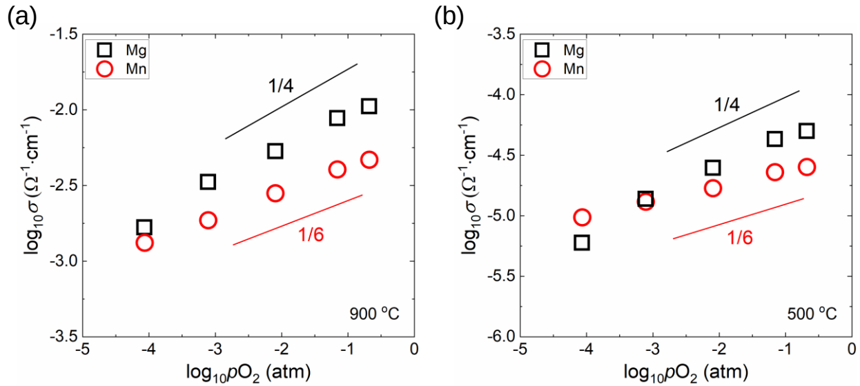
Figure 4.2 DC electrical conductivity as a function of oxygen partial pressure in Mg or Mn-doped BaTiO 3 at (a) 900 °C and (b) 500 °C.
