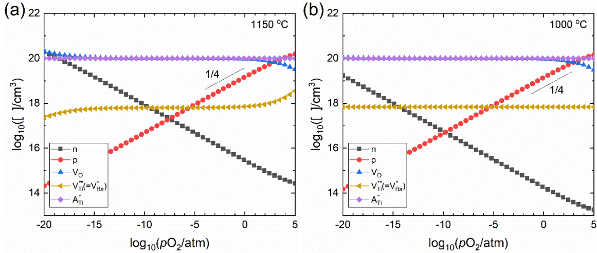
Figure 2.3 (a) Equilibrium defect structure at 1150 °C and (b) partial equilibrium defect structure at 1000 °C with the fixed cation vacancies (equilibrated at T_E = 1150 °C and p\text{O}_2 = 0.21 atm) in single-valent acceptor-doped BaTiO 3 .
