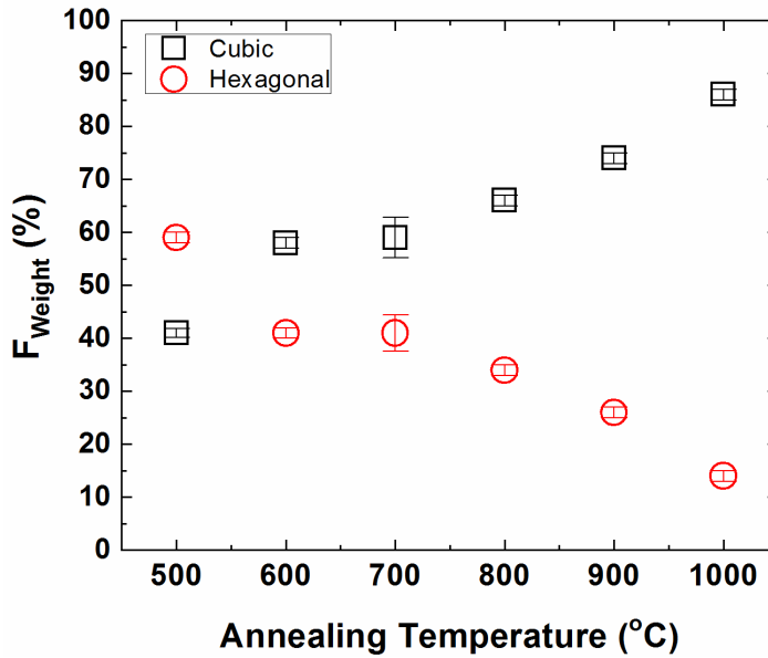
Fig. 2. Weight fraction of the cubic and hexagonal phases versus annealing temperature for 2 hour isothermal holds.
