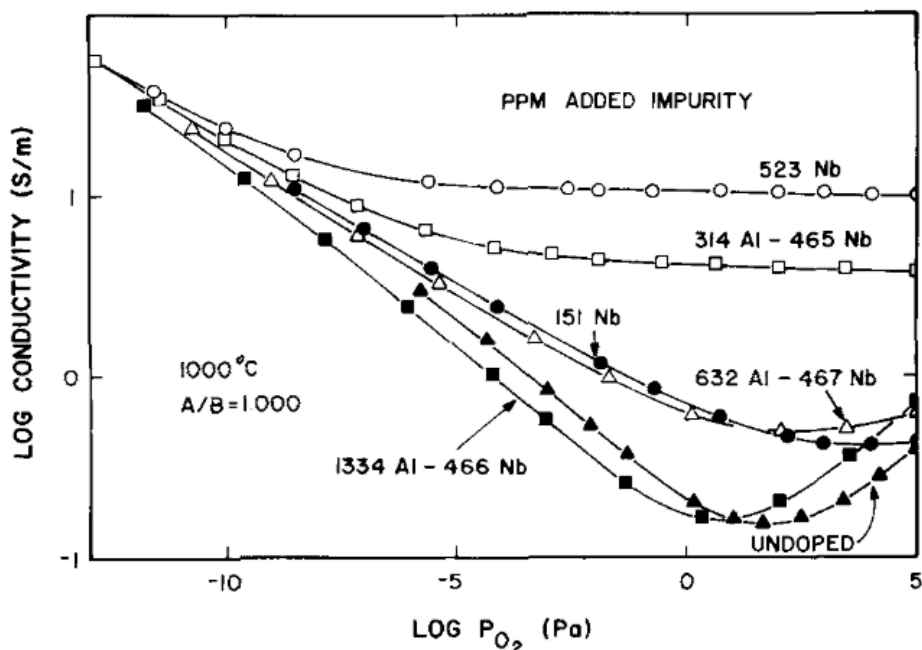
Figure 2.10 Equilibrium electrical conductivity at 1000 °C of BaTiO 3 . Reproduced with permission from [62].
