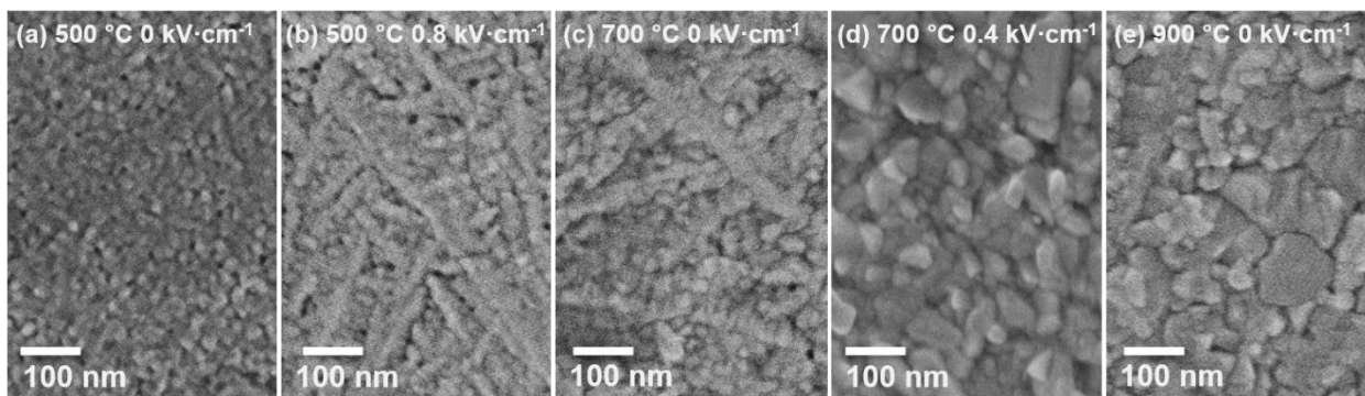
Fig. 5. SEM images of BaTiO 3 thin films after a 2 hour isothermal annealing. (a) 500 °C, 0 kV·cm -1 , (b) 500 °C, 0.8 kV·cm -1 , (c) 700 °C, 0 kV·cm -1 , (d) 700 °C, 0.4 kV·cm -1 and (e) 900 °C, 0 kV·cm -1 .
