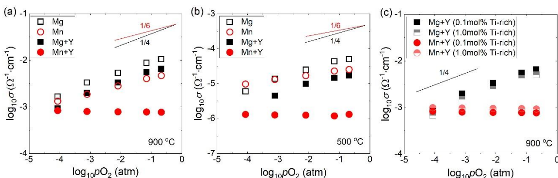
Figure 5.1 DC electrical conductivity as a function of oxygen partial pressure in doped BaTiO 3 with 0.1 mol% Ti-rich at (a) 900 °C and (b) 500 °C. (c) The comparison of high-temperature DC electrical conductivity with respect to the amount of Ti-excess.
