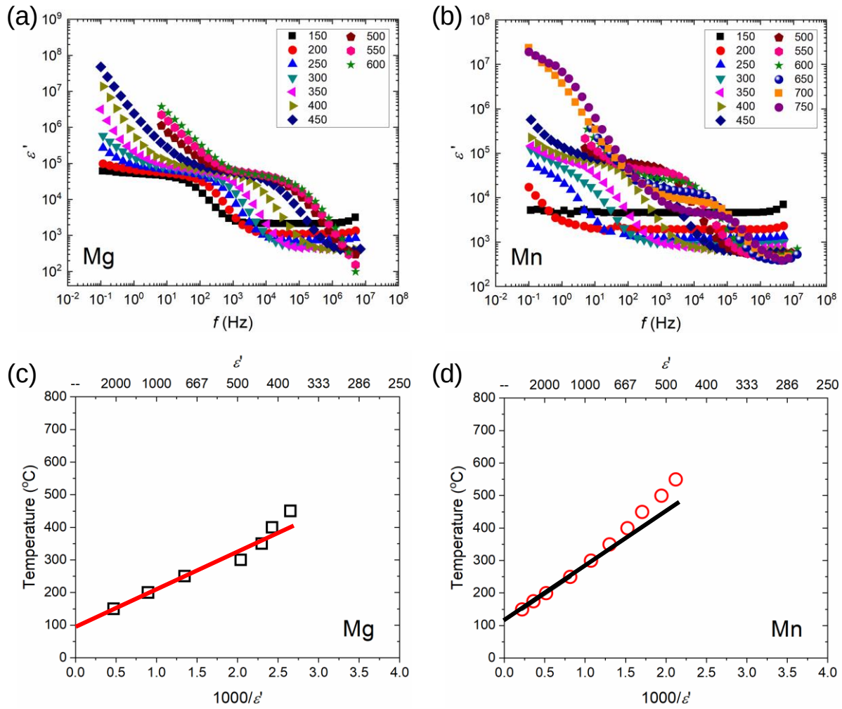
Figure 4.4 Real part of relative permittivity at various temperature in (a) Mg-doped and (b) Mn-doped BaTiO 3 . Curie-Weiss fitting in (c) Mg-doping and (d) Mn-doping.
