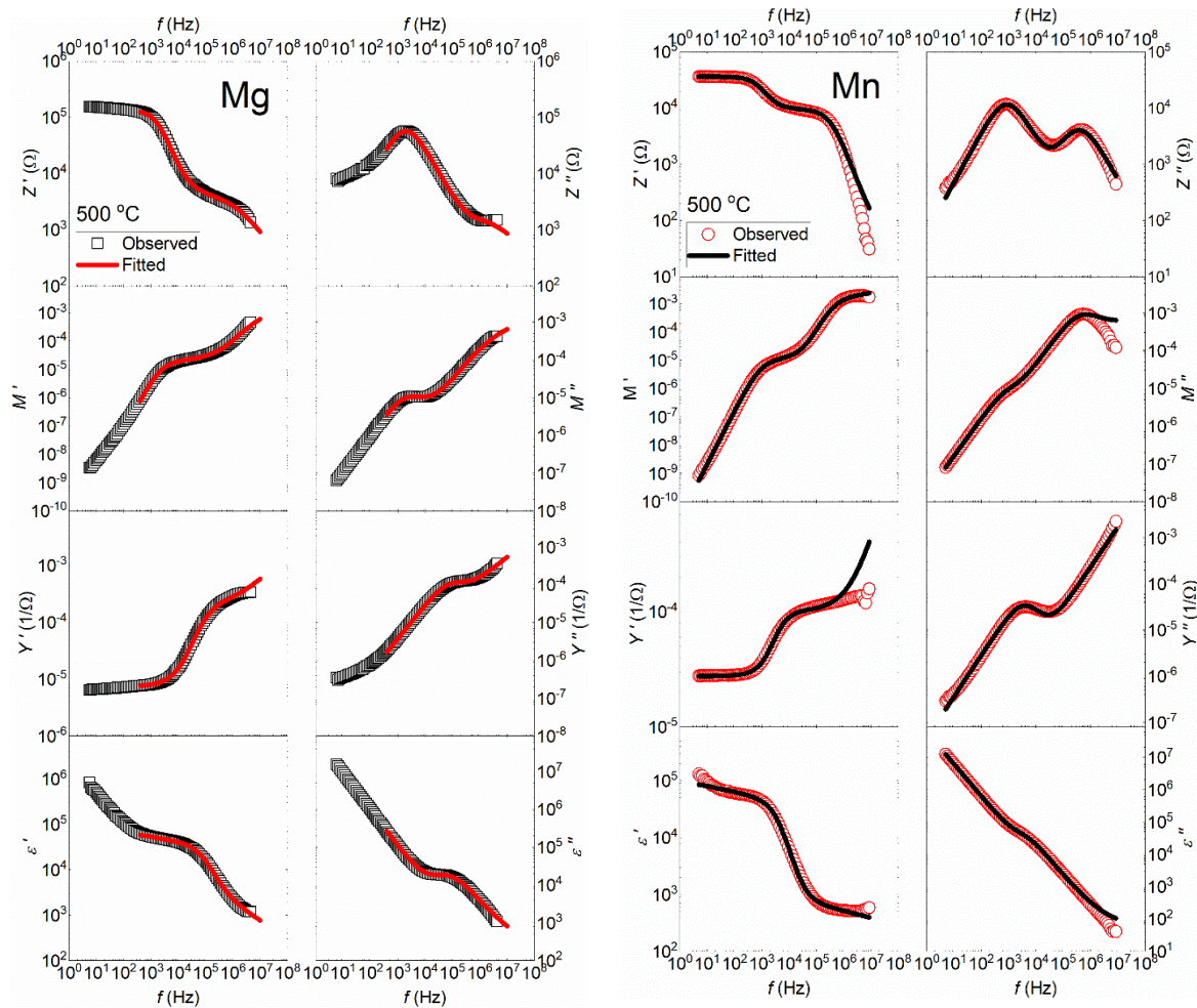
Figure 4.6 Observed and simulated AC formalisms of (a) Mg-doped BaTiO 3 and (b) Mn-doped BaTiO 3 at 500 °C.
