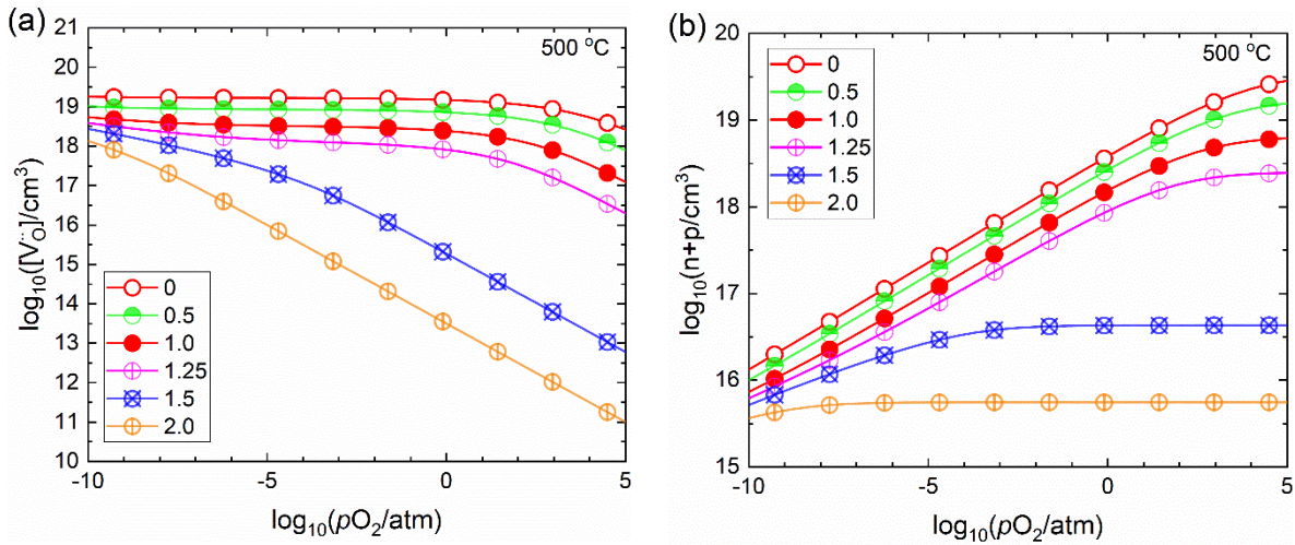
Figure 5.8 Predicted defect concentration of (a) oxygen vacancy and (b) electron and hole in (Mn+Y) co-doped BaTiO 3 with [Y_{Ba}]/[Mn_{Ti}]_T = 0, 0.5, 1.0, 1.5, \text{ and } 2.0 at 500 °C.
