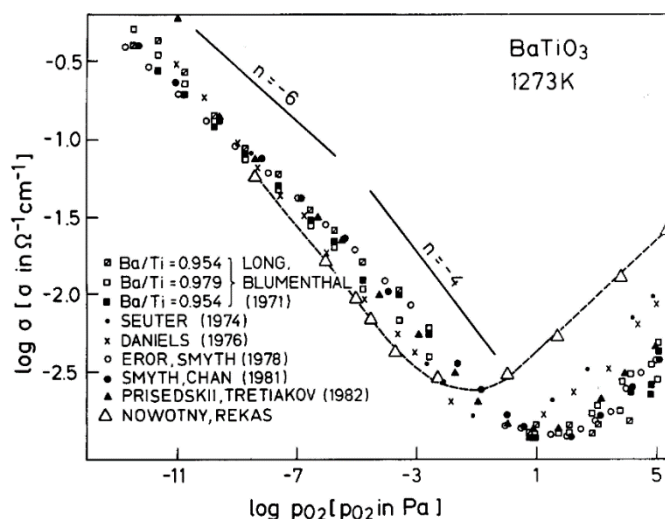
Figure 2.2 Electrical conductivity versus pO_2 of undoped BaTiO_3 ceramics and single crystals at 1000 °C.
