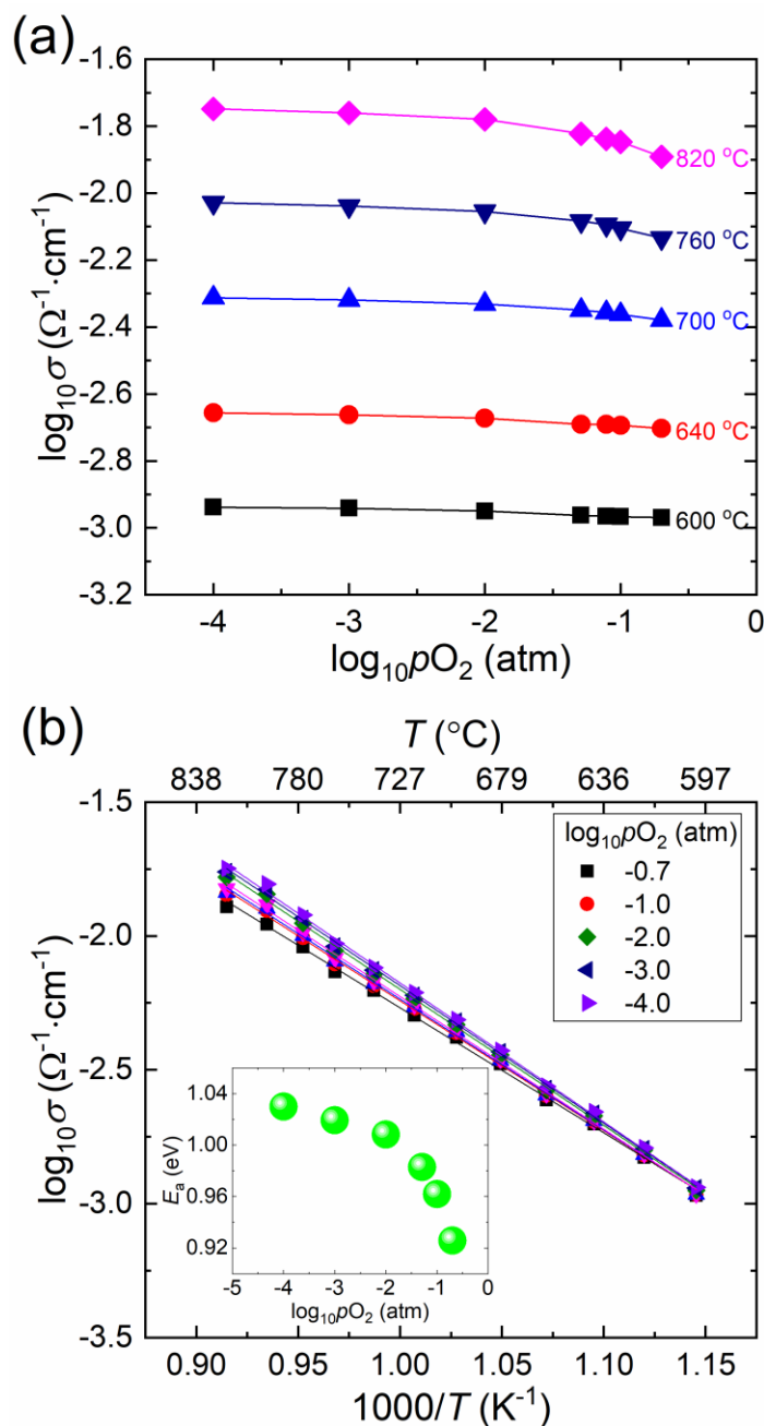
Figure 6.5. (a) Oxygen partial pressure dependent DC electrical conductivity at various temperature. (b) DC electrical conductivity versus temperature with change in activation energy (inset Figure) at each p\text{O}_2 condition.
