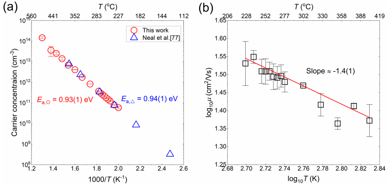
Figure 6.3 Temperature dependent (a) carrier concentration and (b) mobility.
