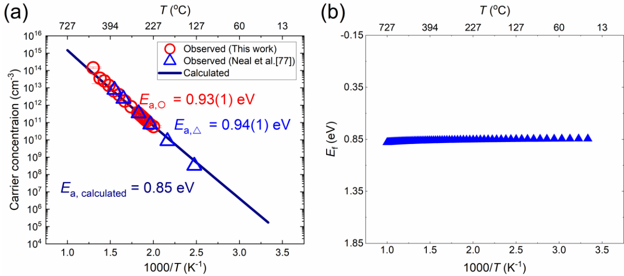
Figure 6.4. (a) Observed and calculated carrier concentrations versus temperature and (b) predicted Fermi level.
