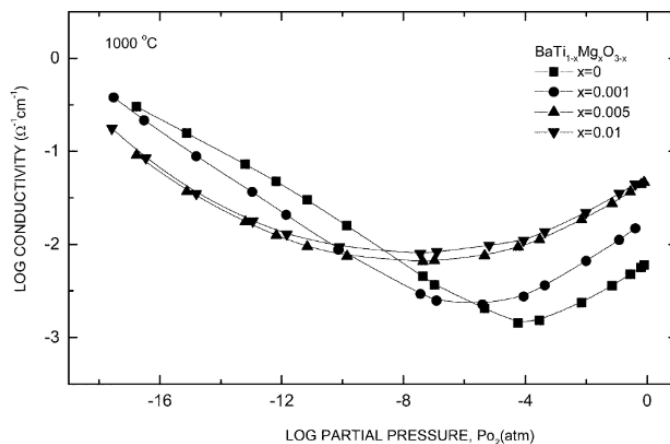
Figure 2.4 Equilibrium electrical conductivity of undoped BaTiO 3 and Ba(Ti 1-x Mg x )O 3-x ( x = 0, 0.001, 0.005, 0.01 ) at 1000 °C. Reproduced with permission from [55].
