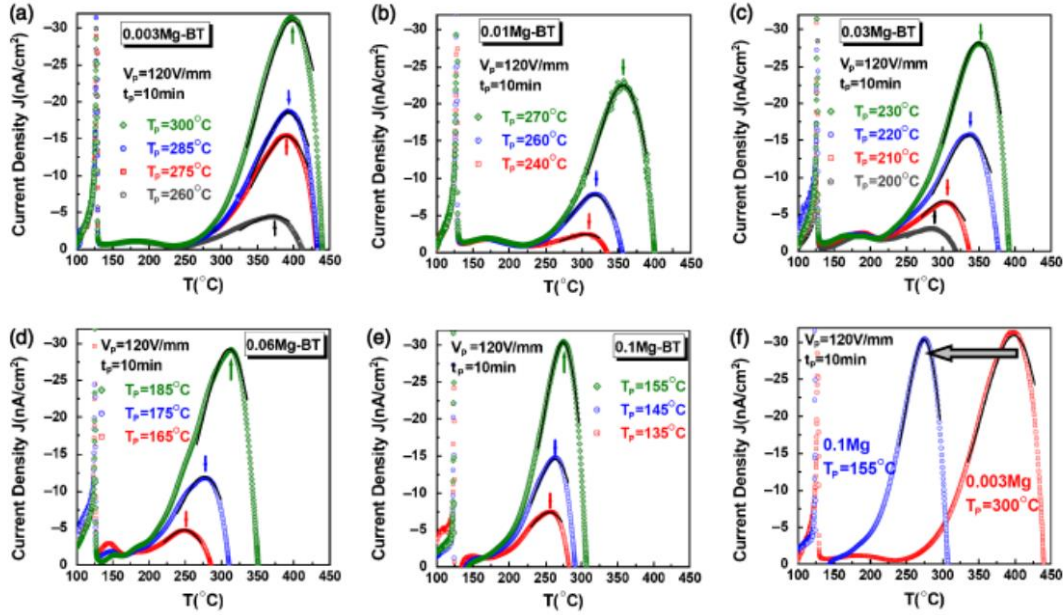
Figure 2.16 TSDC plots in Mg-doped BaTiO 3 ceramics with Mg concentration of (a) 0.003 mol%, (b) 0.01 mol% (c) 0.03 mol% (d) 0.06 mol% (e) 0.1 mol%. (f) Comparison of same magnitude of TSDC peaks of lowest (0.003 mol%) and highest Mg concentration (0.1 mol%) of Mg-doped BaTiO 3 ceramics. Reproduced with permission from [70].
