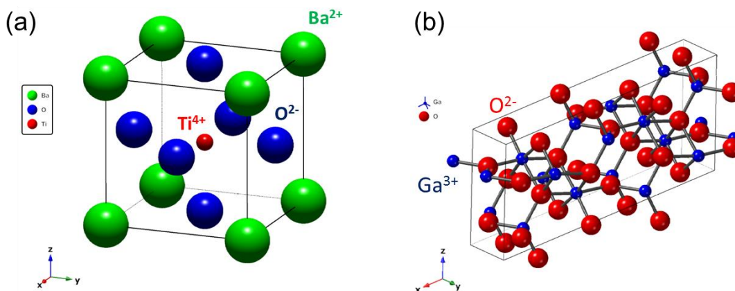
Figure 1.1 Crystal structure of (a) BaTiO 3 and (b) \beta -Ga 2 O 3 .
