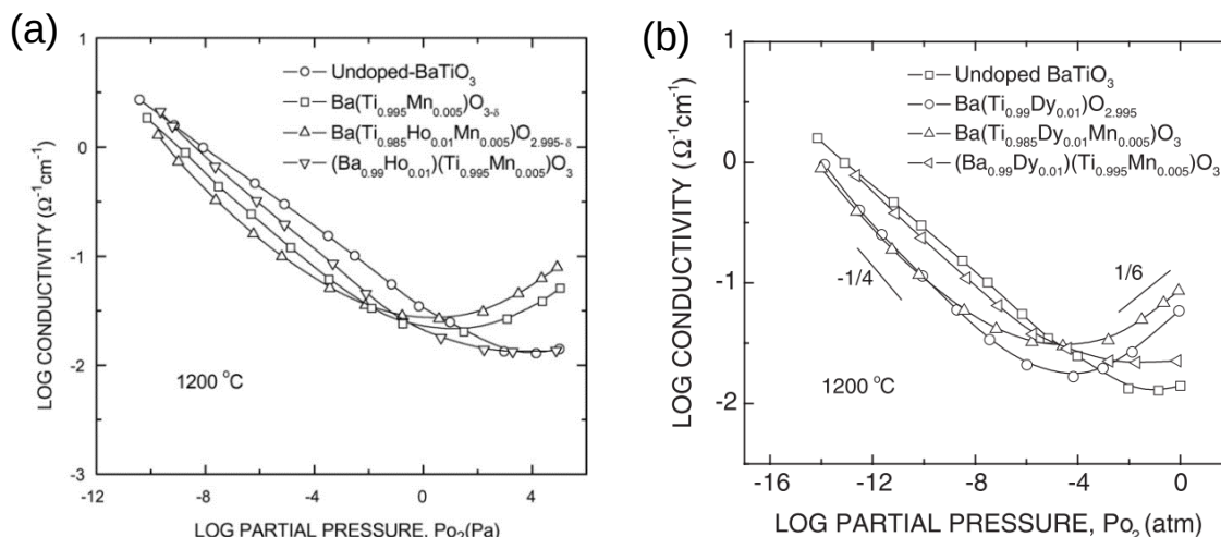
Figure 2.12 (a) Equilibrium electrical conductivities of BaTiO 3 co-doped with (a) Ho and Mn (b) Dy and Mn at 1200 °C. Reproduced with permission from [65,66].
