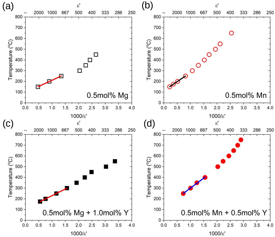
Figure 5.3 Curie-Weiss law fitting in (a) Mg-doped (b) Mn-doped (c) (Mg+Y) co-doped and (d) (Mn+Y) co-doped BaTiO 3 .
