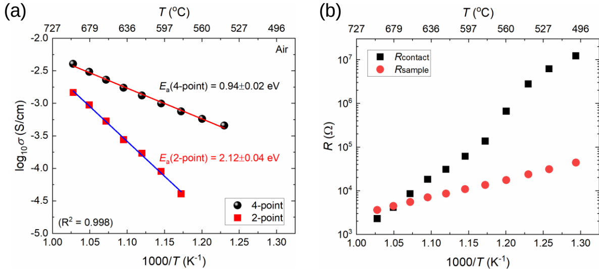
Figure 3.1 Comparison of (a) four-point and two-point-probe DC conductivities and (b) contact and sample resistances in Fe-doped \beta -Ga 2 O 3 single crystal at different temperature in air.
