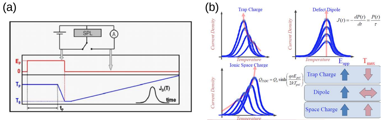
Figure 2.14 Schematic of (a) experimental procedure of TSDC and (b) analysis of TSDC with various polarization mechanisms. Courtesy of Dr. Clive Randall at Penn State University.
