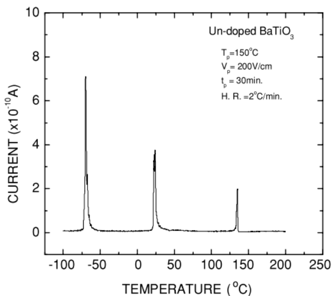
Figure 2.15 TSDC spectrum of undoped BaTiO 3 . Reproduced with permission from [69].
