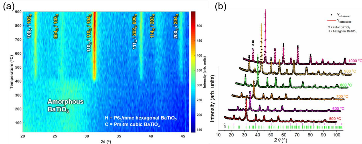
Fig. 1. (a) In-situ high-temperature x-ray diffraction patterns of amorphous BaTiO 3 film on c-sapphire. (b) Observed and fitted room temperature GIXRD patterns of BaTiO 3 films isothermally annealed at 500 °C – 1000 °C for 2 hours in air.
