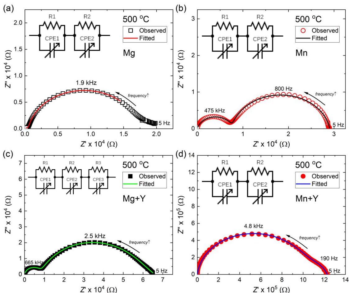
Figure 5.2 Observed and fitted Cole-Cole plots of (a) Mg-doped (b) Mn-doped (c) (Mg+Y) co-doped and (d) (Mn+Y) co-doped BaTiO 3 at 500 °C in air. Note that the real and imaginary parts of impedance were scaled by the sample geometry for the direct comparison of impedance magnitudes.
