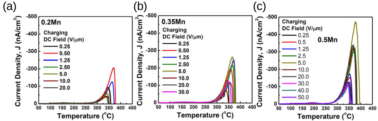
Figure 2.17 TSDC plots for Mn-doped BaTiO 3 MLCC with (a) 0.2 mol% Mn, (b) 0.35 mol% Mn and (c) 0.5 mol% Mn. Reproduced with permission from [72].
