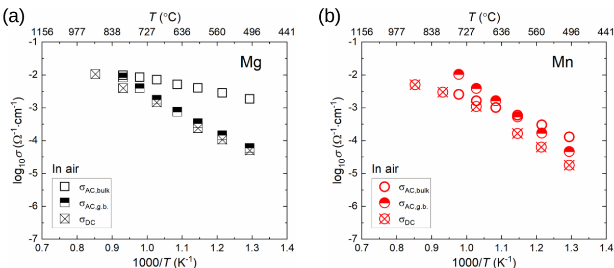
Figure 4.7 Temperature-dependent DC and AC electrical conductivities of (a) Mg-doped BaTiO 3 and (b) Mn-doped BaTiO 3 in air.
