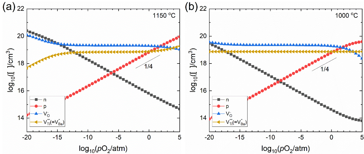
Figure 2.1 (a) Full equilibrium defect structure at 1150 °C and (b) partial equilibrium defect structure at 1000 °C with the fixed cation vacancies equilibrated from the high-temperature condition (1150 °C and pO_2 = 0.21 atm) in undoped BaTiO 3 .
