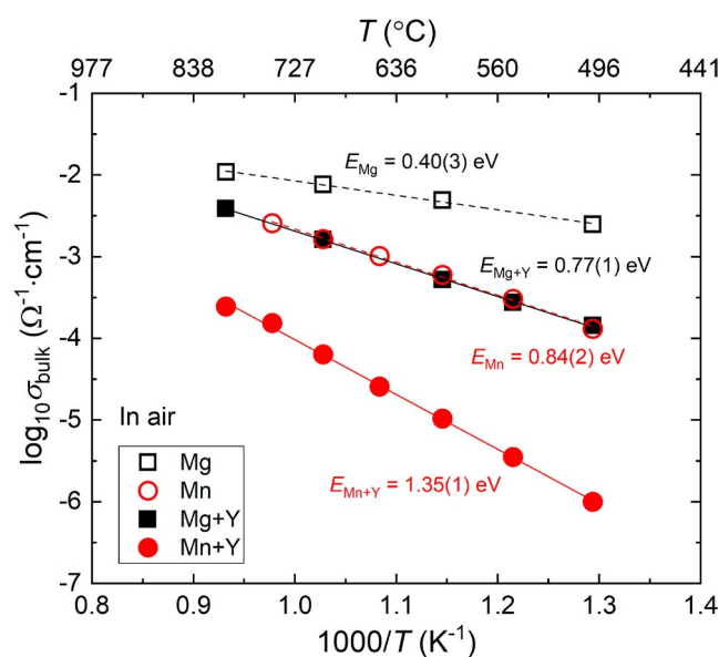
FIGURE 3 Temperature-dependent bulk conductivities, extracted from the impedance spectra, and activation energies in air
