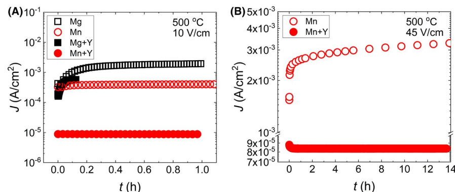
FIGURE 4 Time-dependent current density at 500°C under (A) 10 V/cm and (B) 45 V/cm DC electric field
