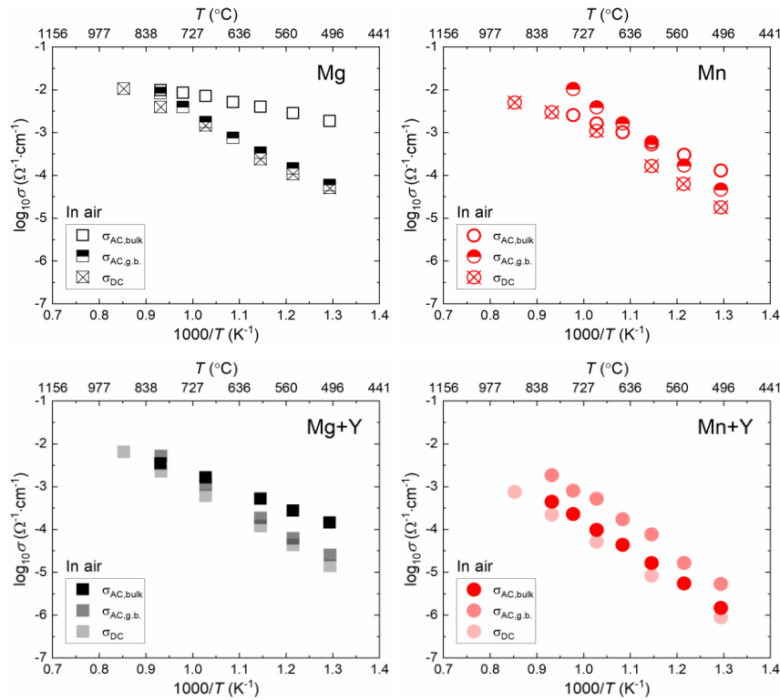
Figure 7.2 Temperature dependent bulk and grain-boundary conductivities of (a) 0.5 mol% Mg-doped, (b) 0.5 mol% Mn-doped, (c) (0.5 mol% Mg and 1.0 mol% Y) co-doped, and (d) (0.5 mol% Mn and 0.5 mol% Y) co-doped BaTiO 3 in air.
