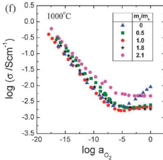
Figure 2.11 Electrical conductivity versus oxygen activity of BaTiO 3 co-doped by Mn and Y with different donor-to-acceptor ratios m_d/m_a = 0.0 (a), 0.5 (b), 1.0 (c), 1.8 (d), and 2.1 (e) at 1000 °C. Reproduced with permission from [64].
