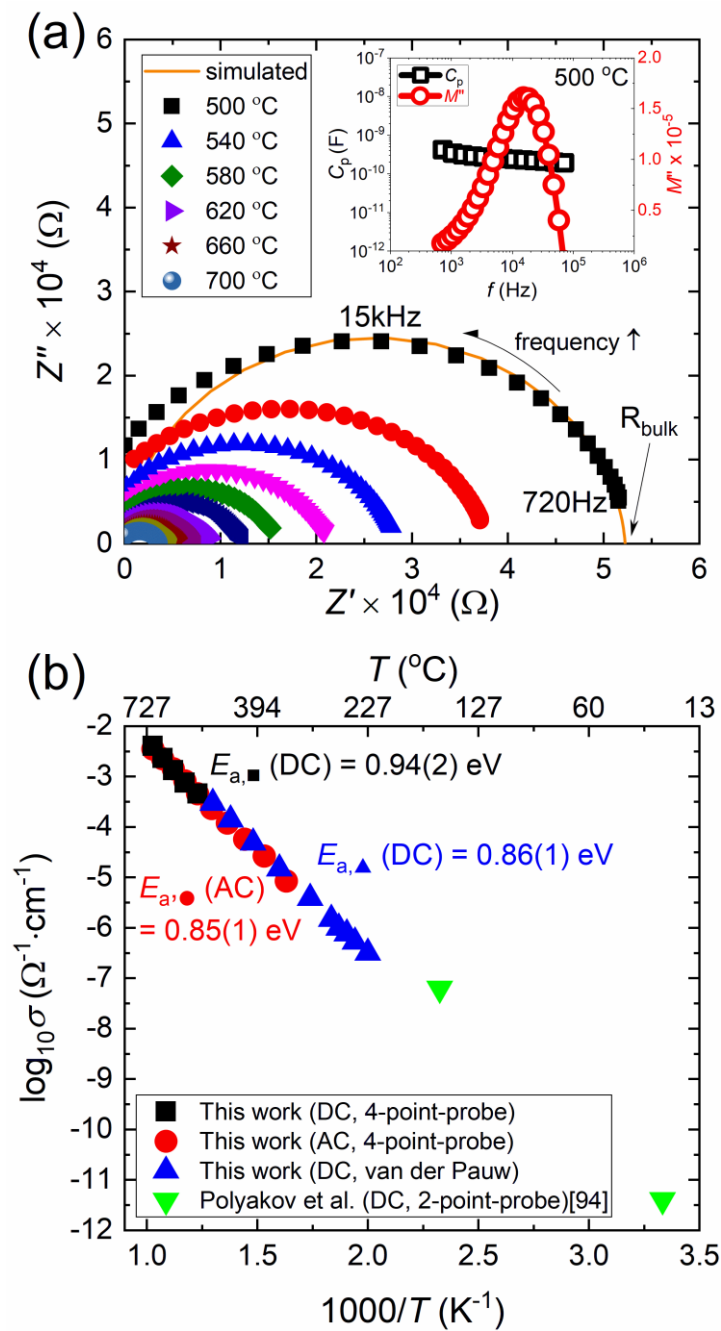
Figure 6.2 (a) Cole-Cole plots versus temperature in air and capacitance and imaginary part of modulus as a function of frequency at 500 °C in inset Figure. (b) Temperature-dependent electrical conductivities obtained from the different techniques.
