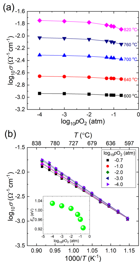
FIG. 4. (a) Oxygen partial pressure dependent DC electrical conductivity at various temperatures. (b) DC electrical conductivity vs temperature with a change in activation energy (inset) at each p\text{O}_2 condition.
