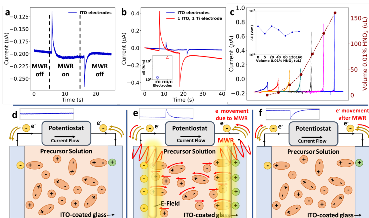
Figure 8: (a) MW-CV results indicating the change in current when the MWR is turned on (positive spike) and off (negative spike). (b) The role of the substrate on local electric field intensity. Using a higher electrical conductivity Ti layer leads to an order of magnitude increase in the electric field at the surface. (c) The role of ion concentration on local electric field intensity. Higher ion concentration increases the peak intensity, but decreases peak width, leading to no effect on the electric field at the surface. (d-f) Schematic of the mechanism of local electric field enhancement during MWR exposure. Initially, polar molecules and ions are oriented randomly in solution (d). When MWR is introduced, it is absorbed by the conducting layer and creates a large electric field at the surface. This electric field draws additional ions or molecules to the surface, leading to a spike in current to balance the additional surface charge (e). When MWR is turned off, the ions drawn to the surface release back to a random orientation, leading to a sharp negative flow in current (f).
