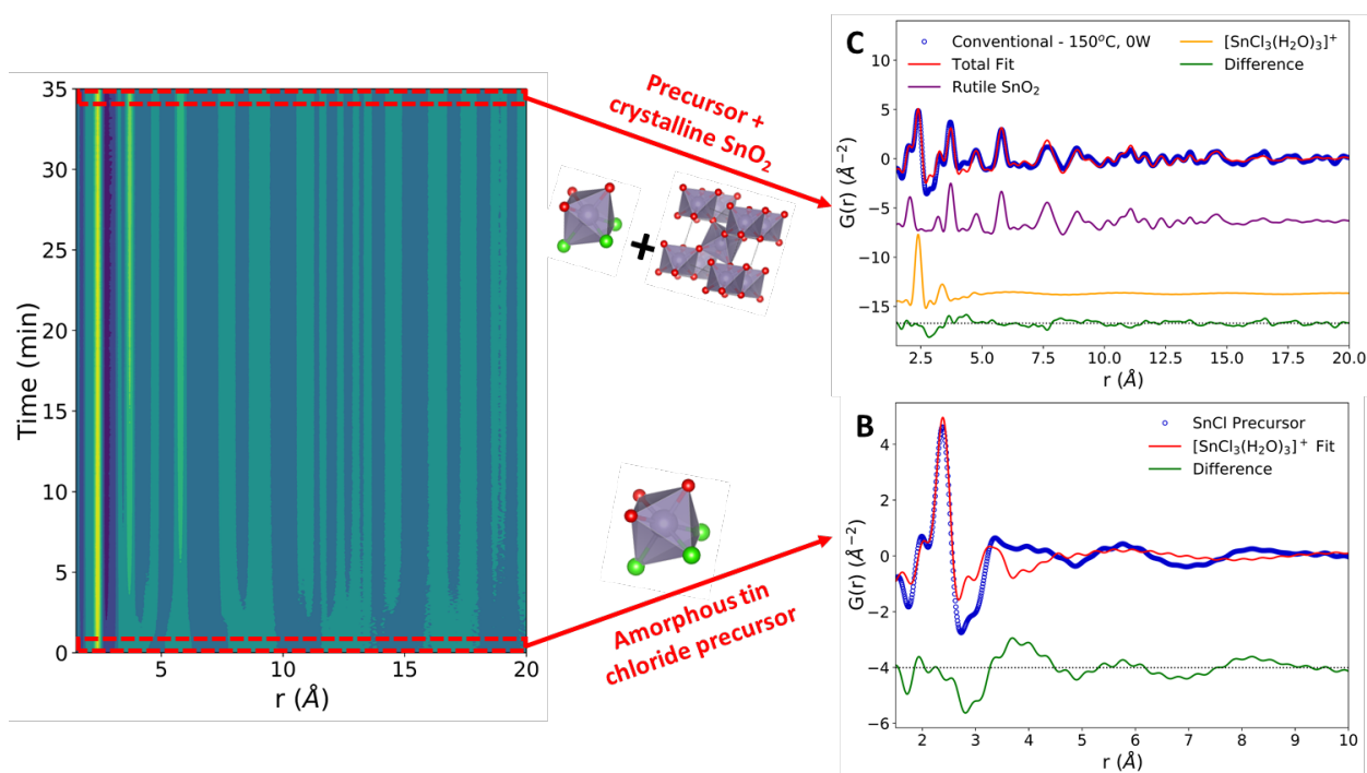
Figure 11: Conventional hydrothermal \text{SnO}_2 nanoparticle synthesis. (a) Contour plot demonstrating the growth of crystalline PDF peaks over time. (b) Experimental PDF data from the tin chloride precursor solution (blue) with the refinement to the [\text{SnCl}_3(\text{H}_2\text{O})_3]^+ complex (red). The difference between the experimental data and the fit is shown offset below in green. (c) PDF data of the final synthesis product (blue) refined to a two-phase model (red). The total two-phase fit is a mixture of the crystalline rutile phase (purple) and the [\text{SnCl}_3(\text{H}_2\text{O})_3]^+ complex (orange). The difference from the total fit is shown offset below in green.
