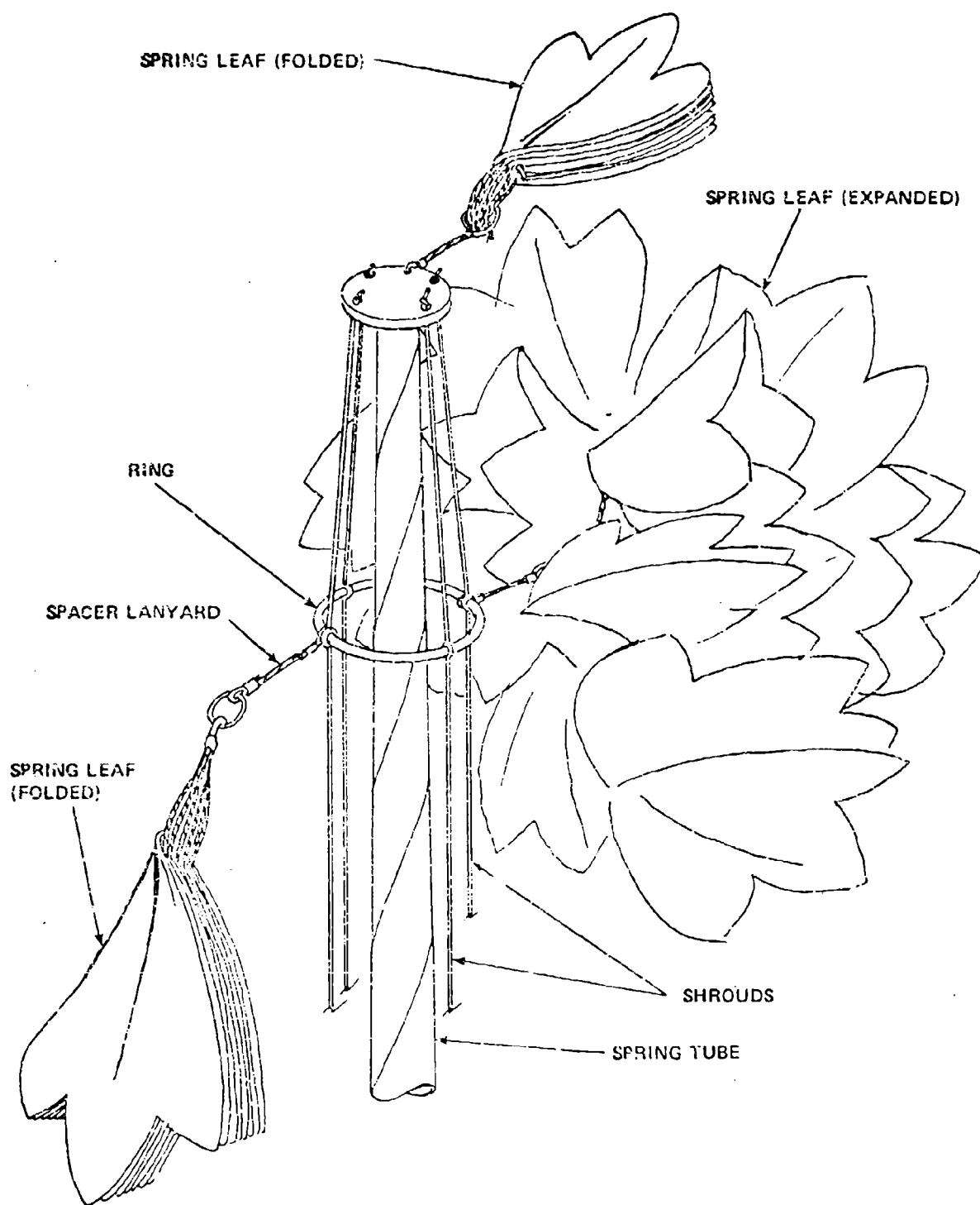
FIGURE 15. SCHEMATIC OF SPRING TUBE-SPRING LEAF CAMOUFLAGE CONCEPT
