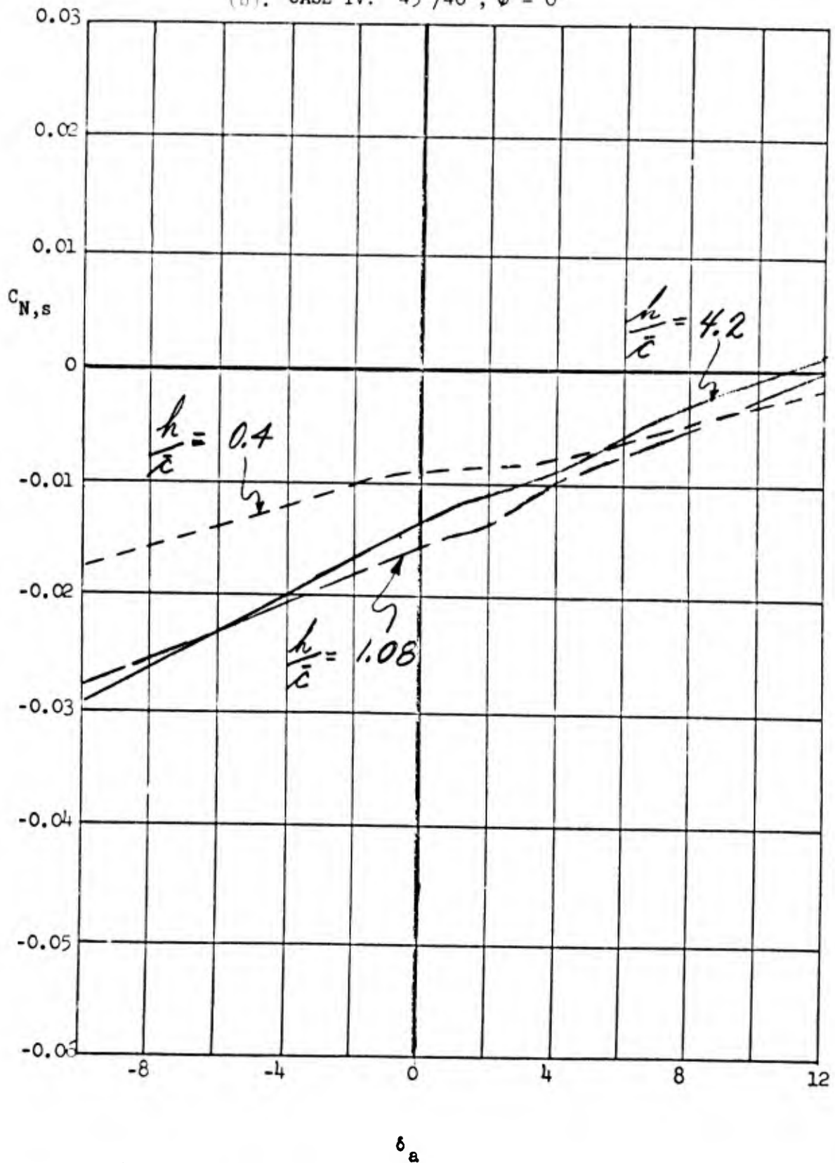
Figure 34. Yawing characteristic versus aileron deflection at three altitude ratios.
