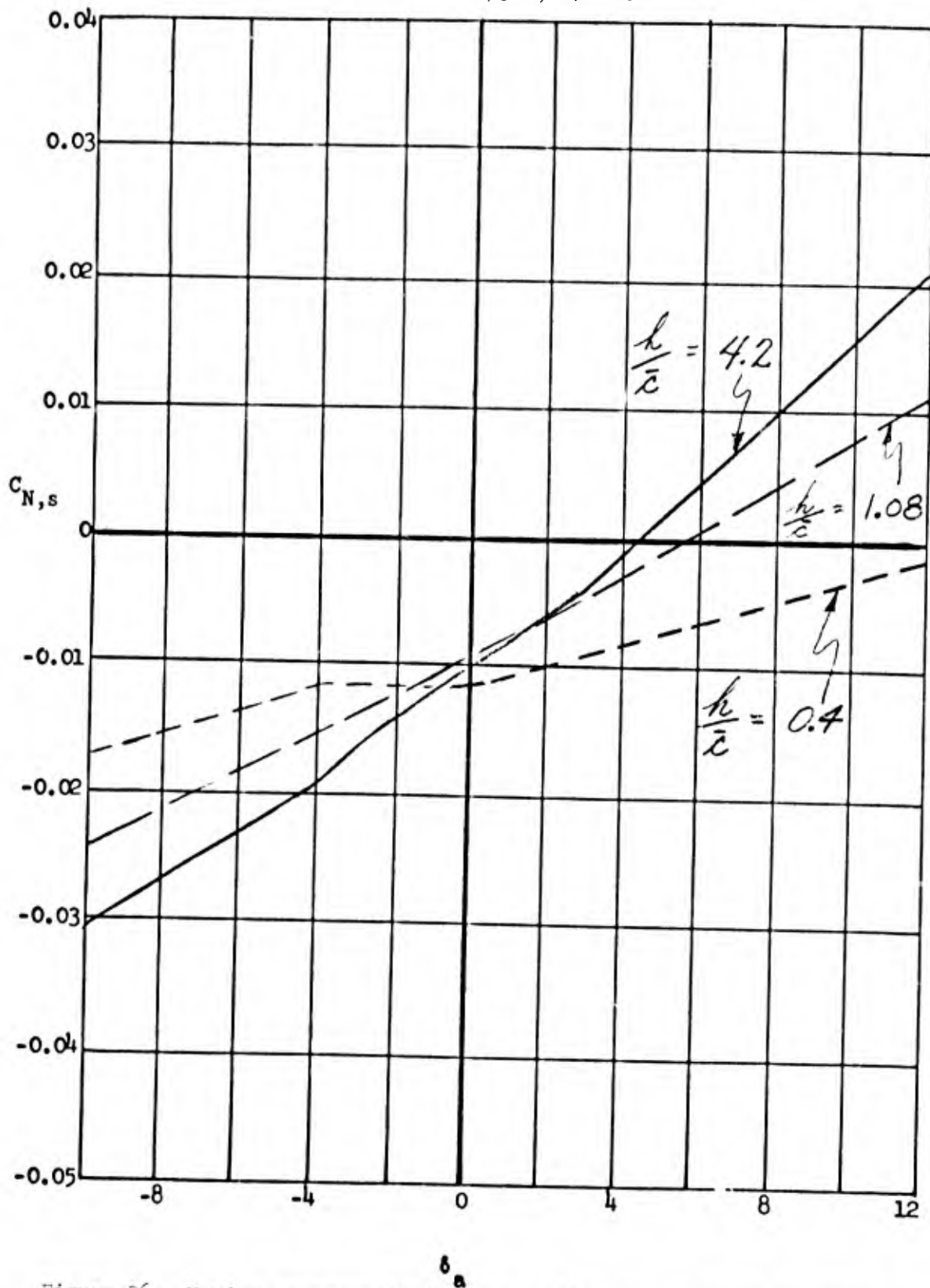
Figure 36. Yawing characteristic versus aileron deflection at three altitude ratios.
