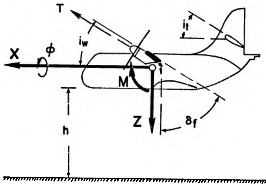
Figure 7. Model axis system and notation.
