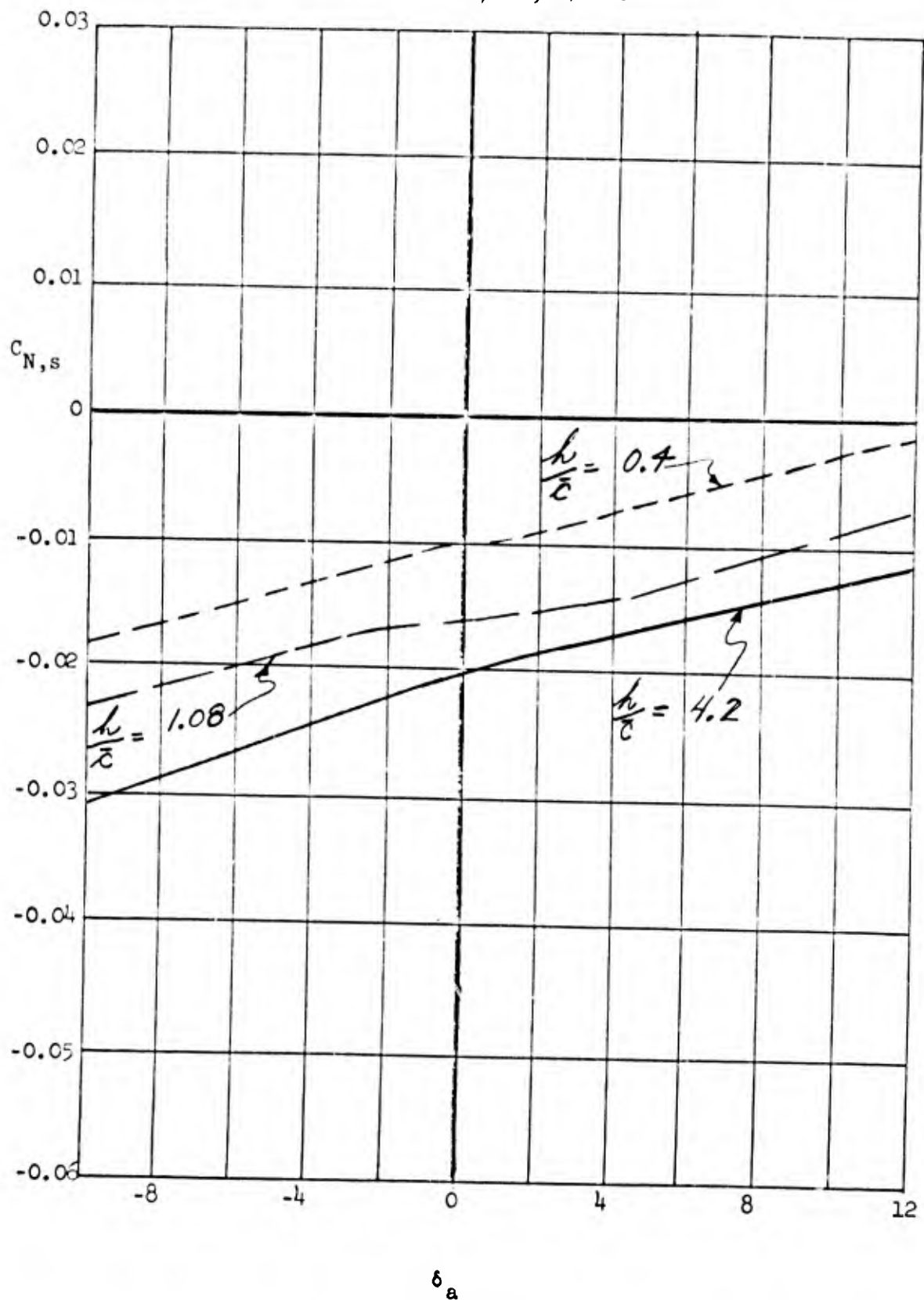
Figure 32. Yawing characteristic versus aileron deflection at three altitude ratios.
