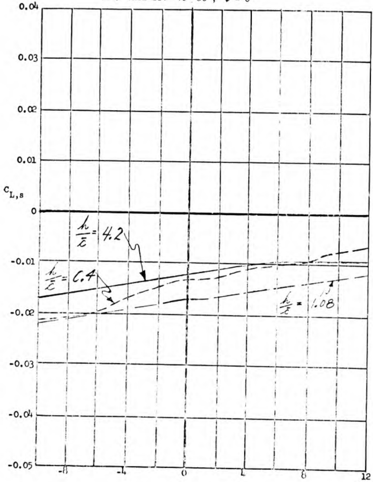
Figure 30. Rolling characteristic versus aileron deflection at three amplitude ratios.
