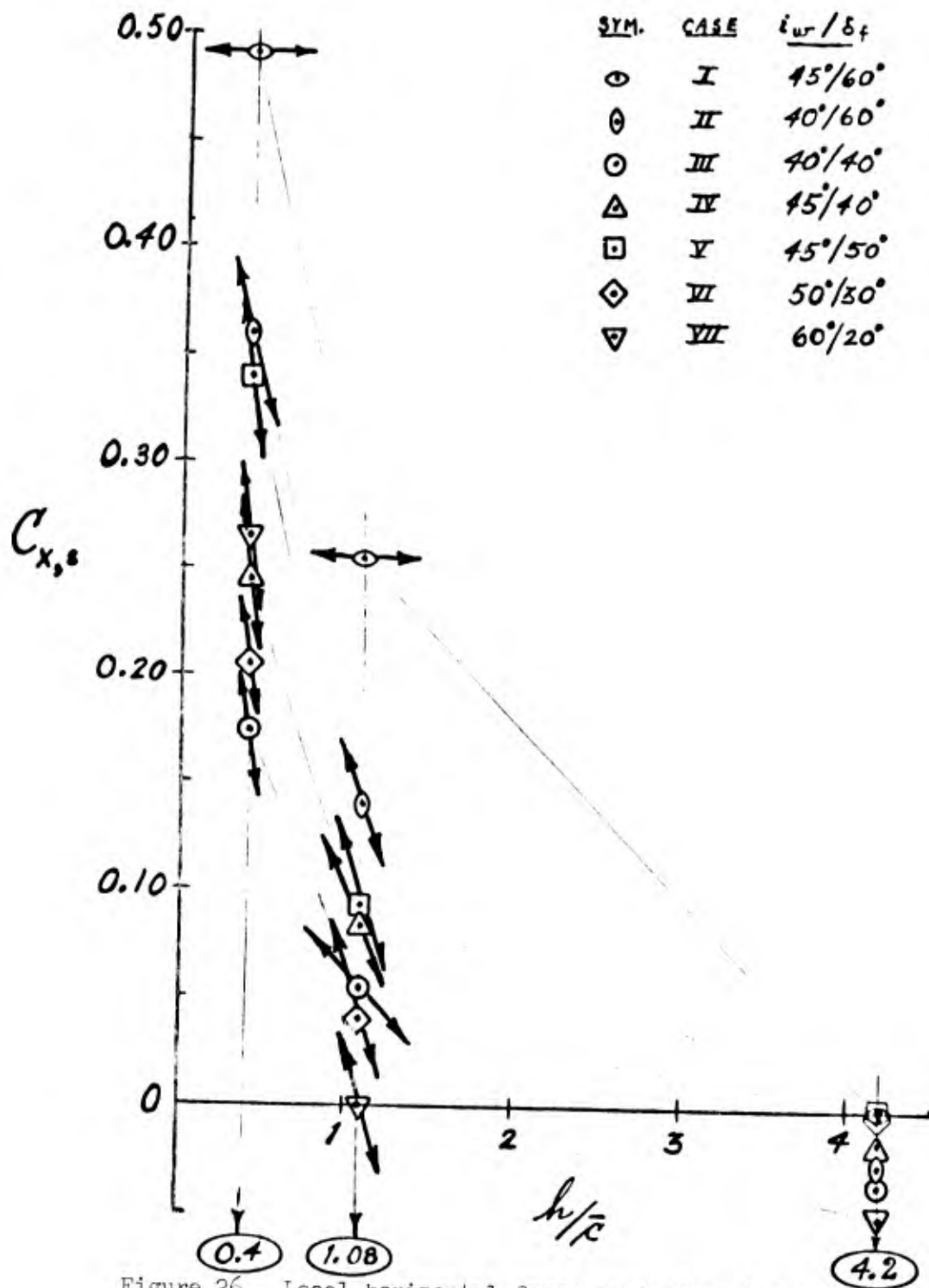
Figure 26. Local horizontal force variation with height predicted from yawing moment variation with roll angle.
