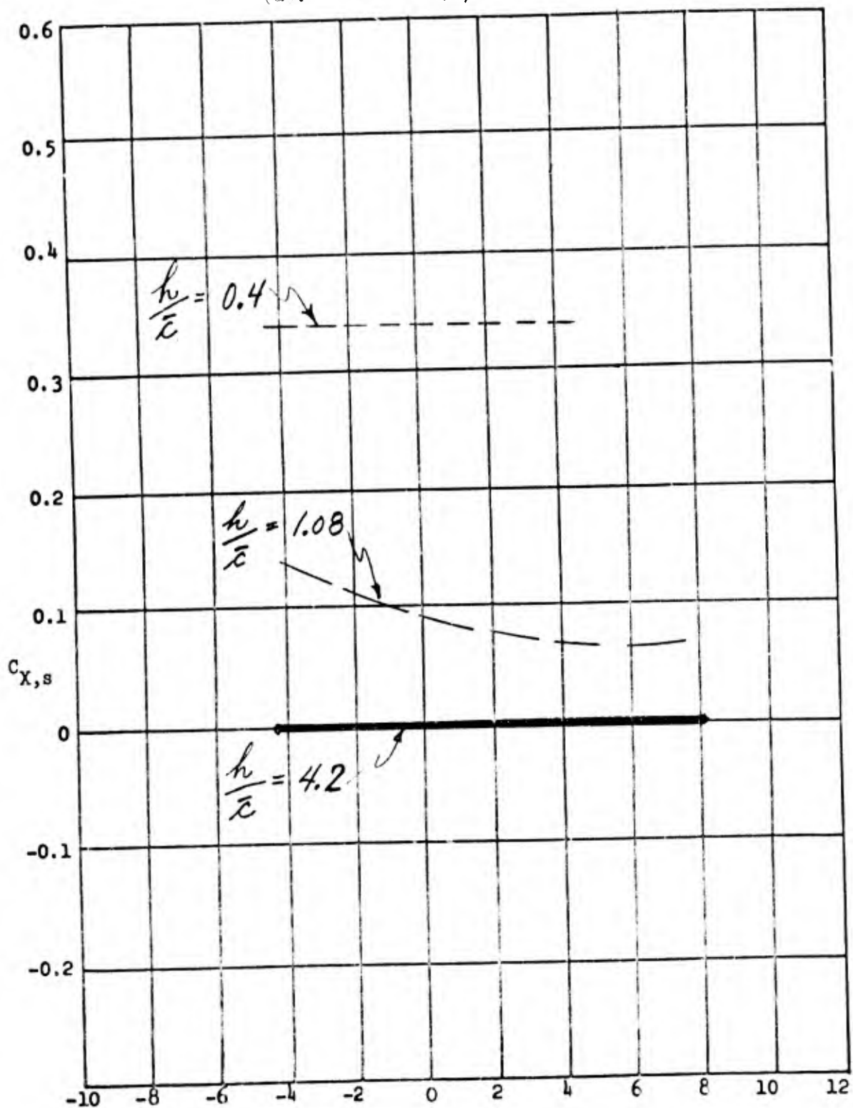
Figure 28. Longitudinal and lateral aerodynamic characteristics versus roll angle at three altitude ratios.
