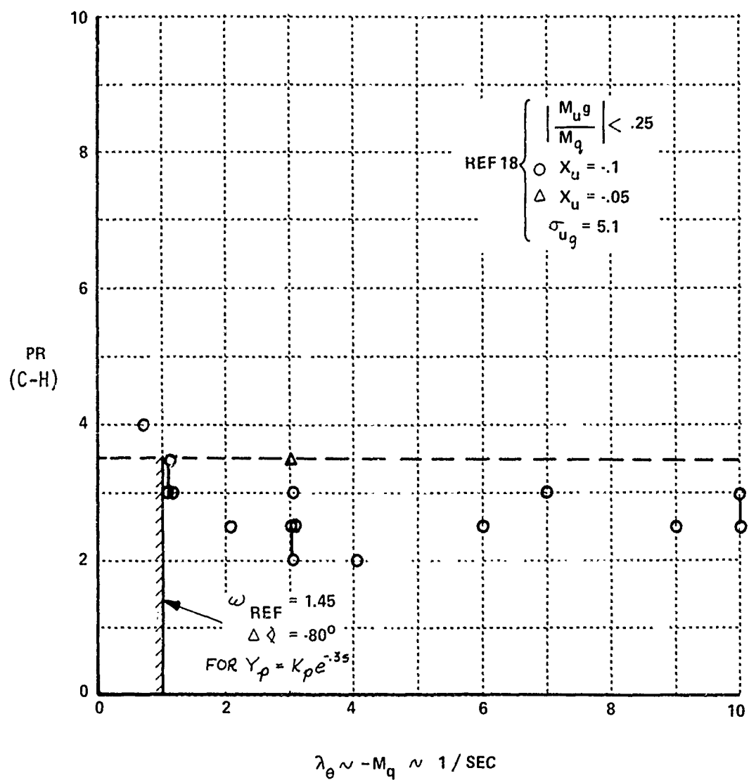
Figure 34 CORRELATION OF PILOT RATING WITH \lambda_\theta
