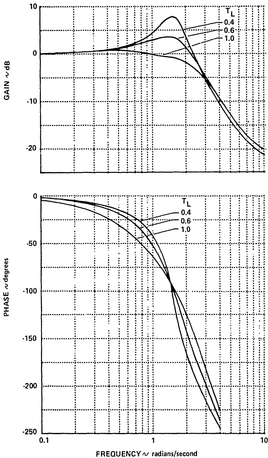
Figure 15 CLOSED-LOOP FREQUENCY RESPONSE AS A FUNCTION OF T_L FOR CONFIGURATION 3
