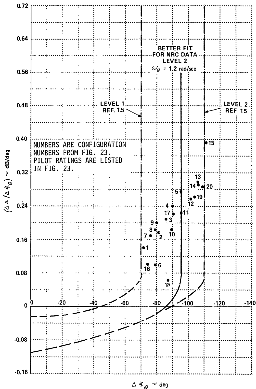
Figure 24 DATA FROM NRC GROUP I COMPARED TO PITCH MANEUVER RESPONSE REQUIREMENT OF REF. 15
