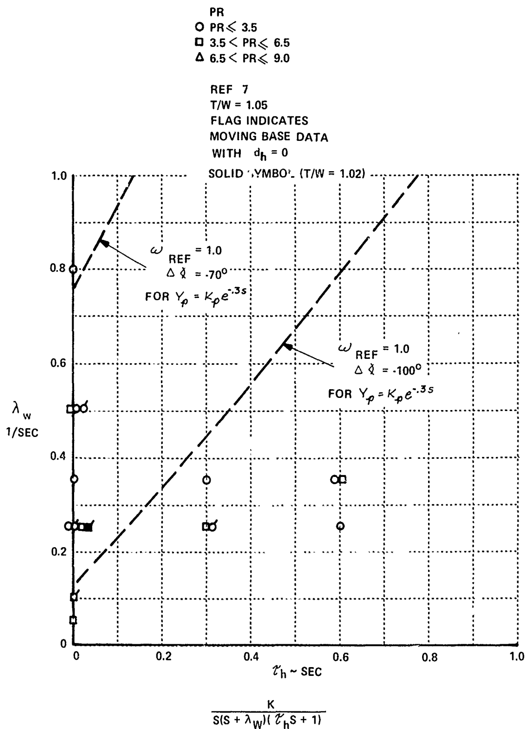
Figure 30 CORRELATION OF PILOT RATING WITH VERTICAL DAMPING INCLUDING A FIRST-ORDER CONTROL SYSTEM LAG, T/W \leq 1.05
