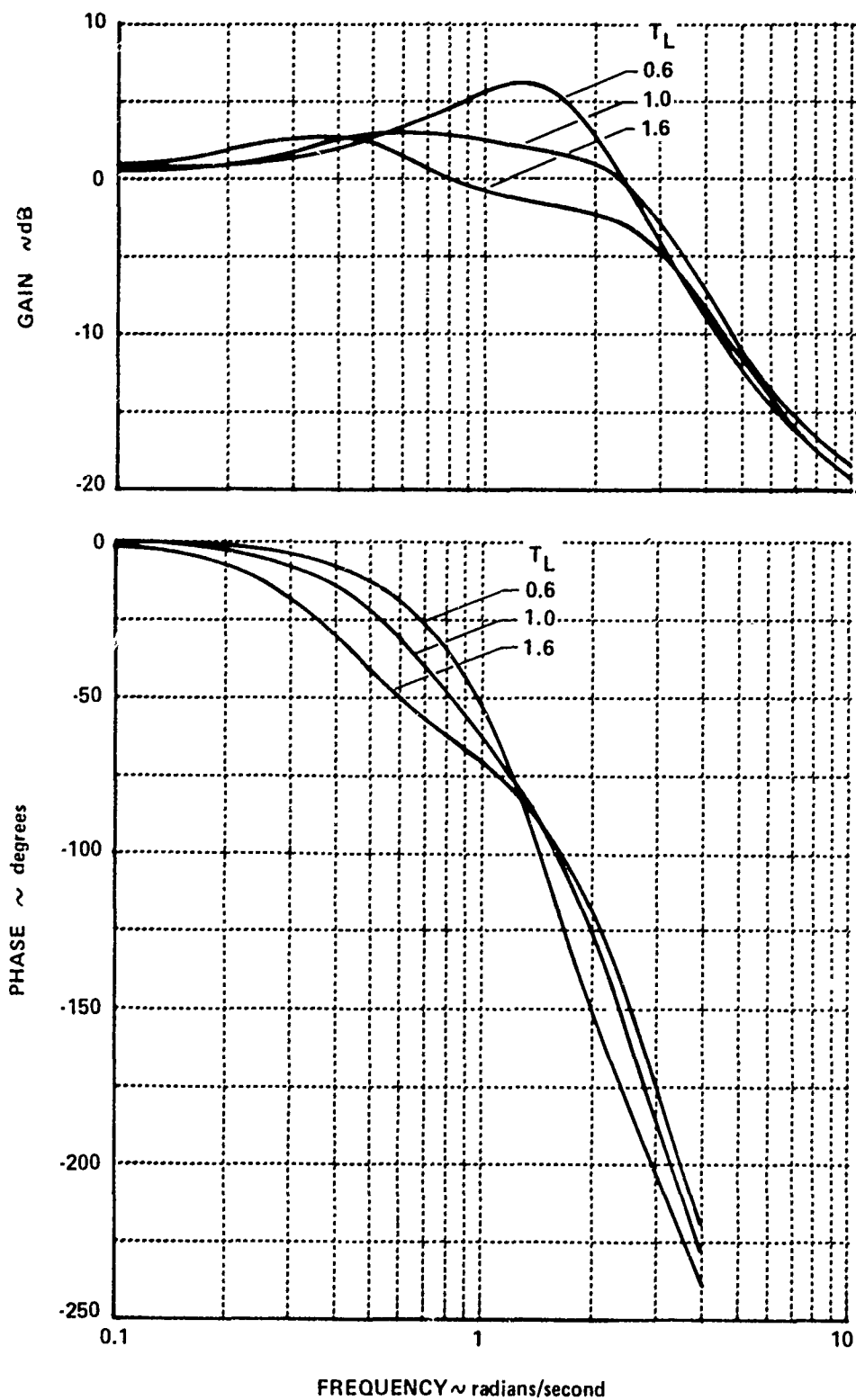
Figure 16 CLOSED-LOOP FREQUENCY RESPONSE AS A FUNCTION OF T_L FOR CONFIGURATION 5
