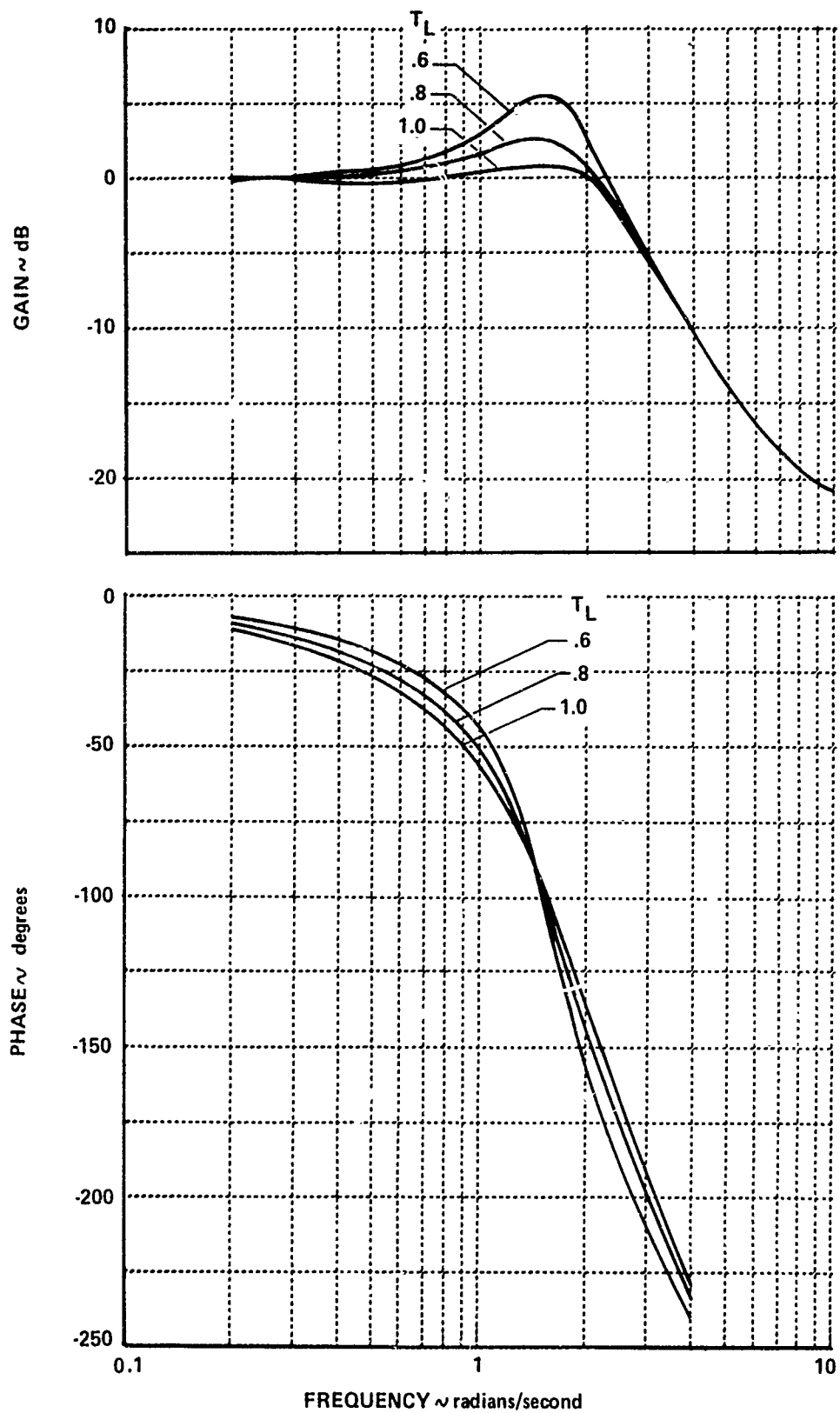
Figure 12 CLOSED-LOOP FREQUENCY RESPONSE AS A FUNCTION OF T_L FOR CONFIGURATION 10
