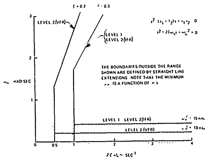
Figure 1 SHORT TERM LONGITUDINAL RESPONSE REQUIREMENTS (FROM REFERENCE 1)
