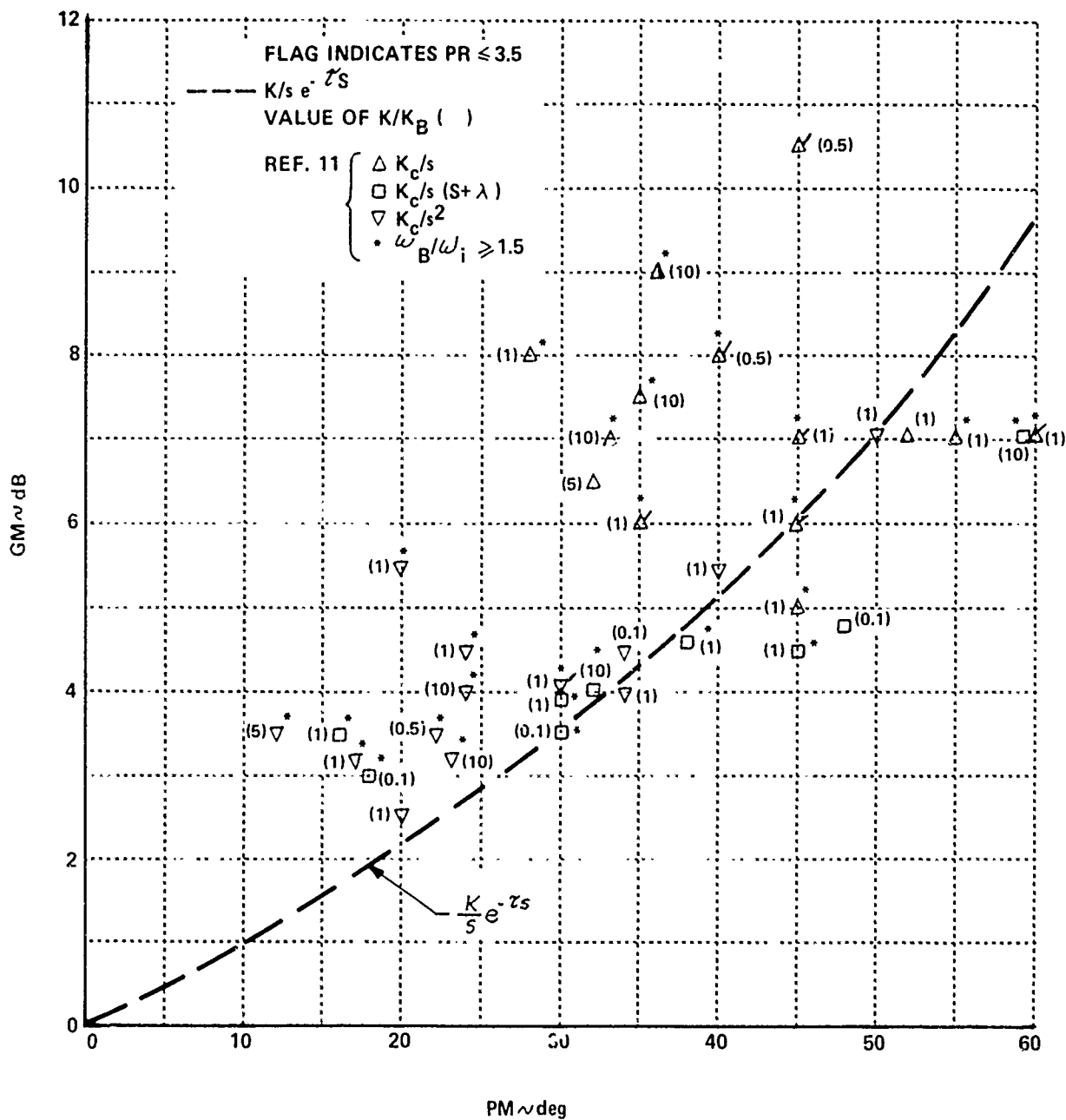
Figure 62 GAIN MARGIN AS A FUNCTION OF PHASE MARGIN FOR "MEASURED" PILOT LEAD EQUALIZATION
