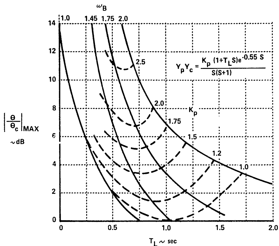
Figure 9 (a) RESONANCE MAGNITUDE AS A FUNCTION OF PILOT LEAD, GAIN AND BANDWIDTH FREQUENCY, Y_c = \frac{1}{S(S+1)}
