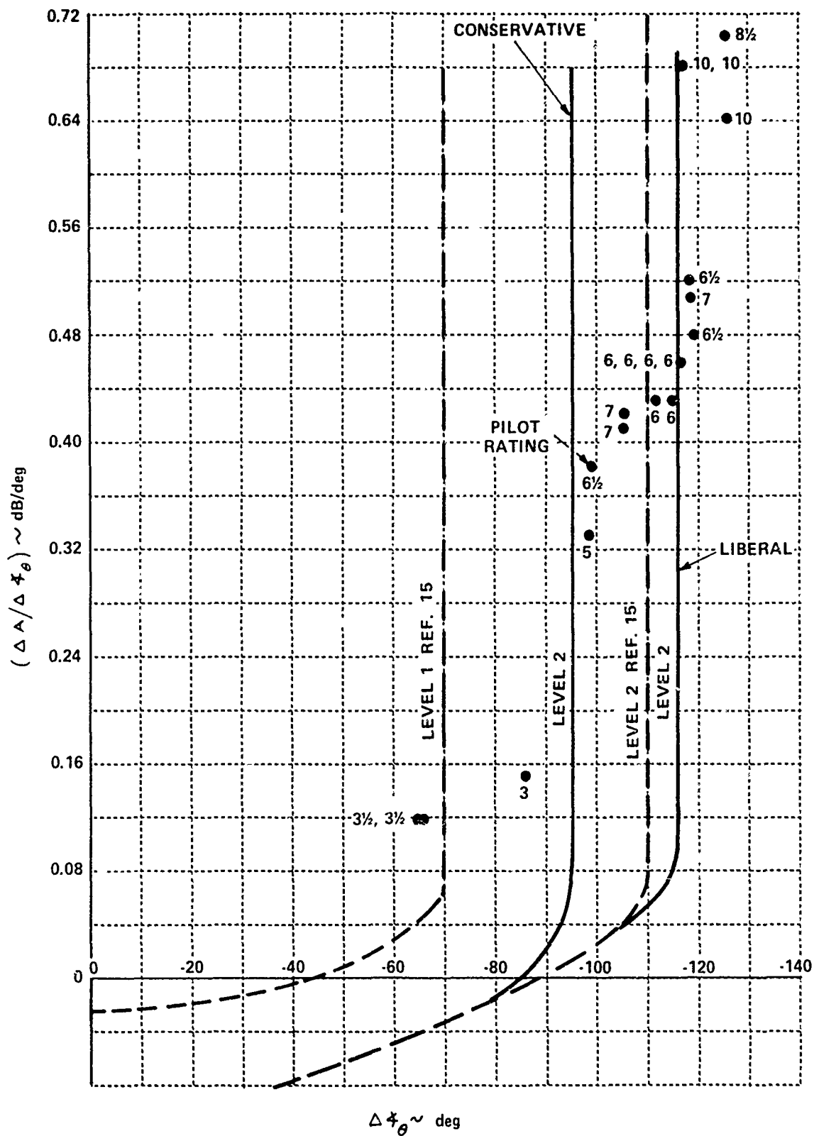
Figure 26 DATA FROM REF. 17 COMPARED TO PITCH MANEUVER RESPONSE REQUIREMENTS OF REF. 15
