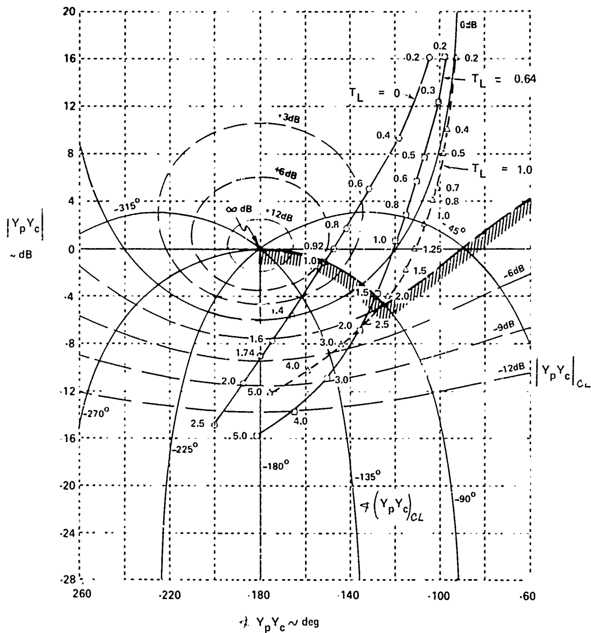
Figure 49 NICHOLS CHART FOR Y_p Y_c = \frac{1.25(T_L s + 1)e^{-.3s}}{s(s+1)} AS LEAD EQUALIZATION IS VARIED FROM 0 TO 1.0
