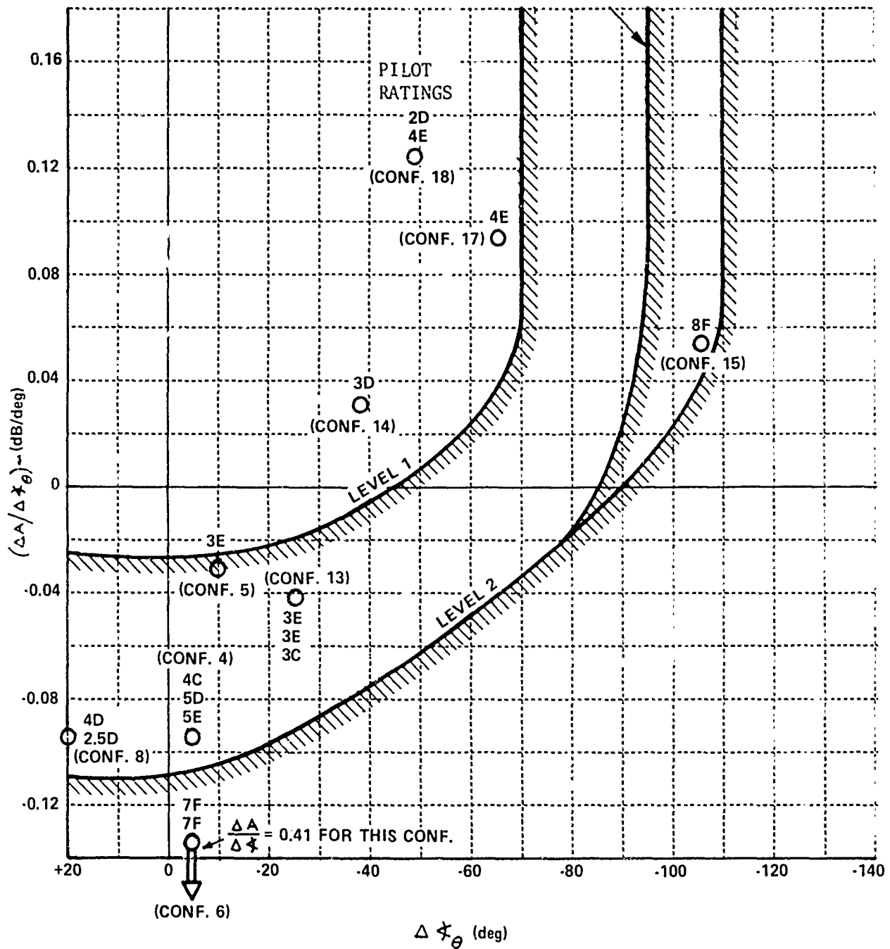
Figure 25 DATA FROM REF. 10 COMPARED TO PITCH MANEUVER RESPONSE REQUIREMENTS OF REF. 15
