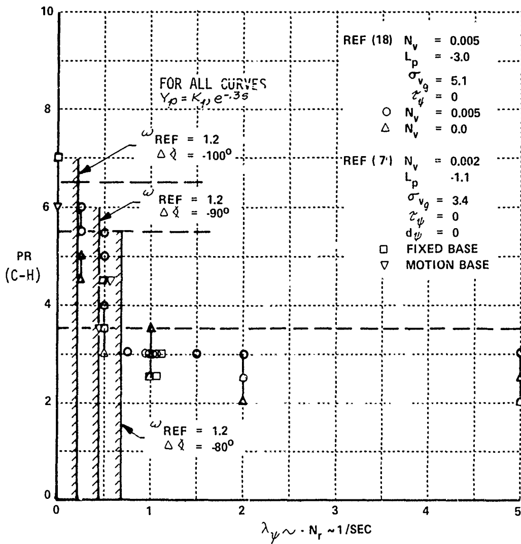
Figure 38 CORRELATION OF PILOT RATING WITH \lambda_\psi
