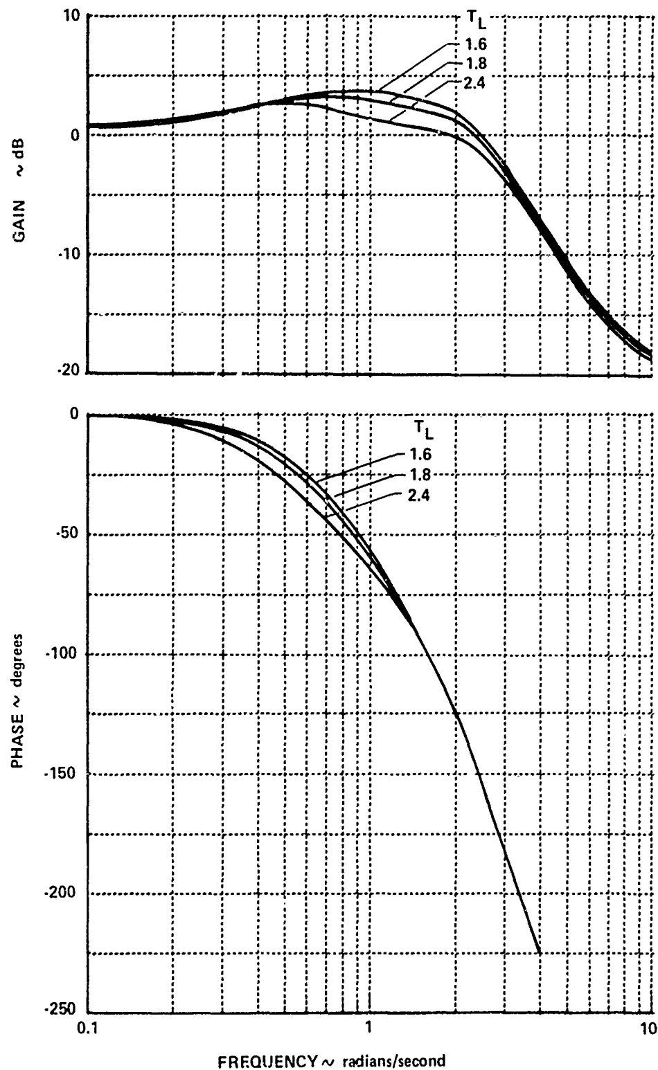
Figure 18 CLOSED-LOOP FREQUENCY RESPONSE AS A FUNCTION OF T_L FOR CONFIGURATION 15
