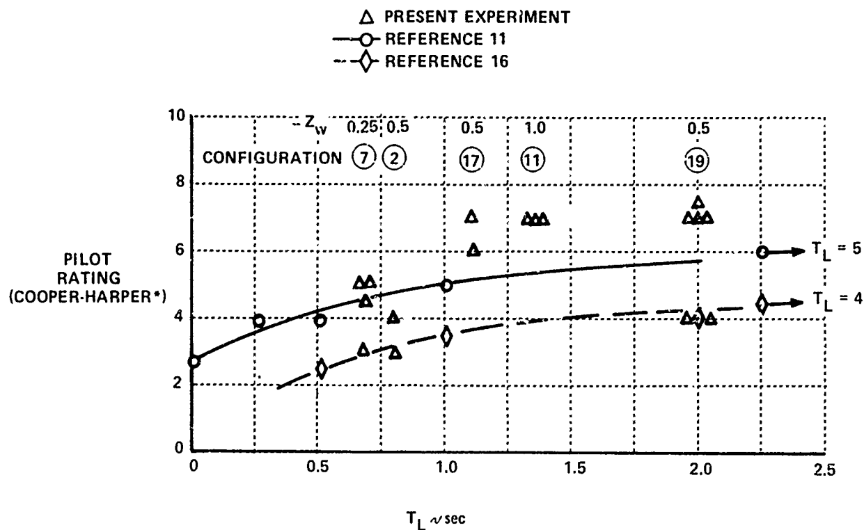
Figure 7 PILOT RATING VARIATION WITH LEAD COMPENSATION FOR CONTROL ELEMENT FORM Y_c = \frac{\theta(s)}{F_E(s)} = \frac{K_c}{s(s+\alpha)} ASSUMING T_L = 1/\alpha
