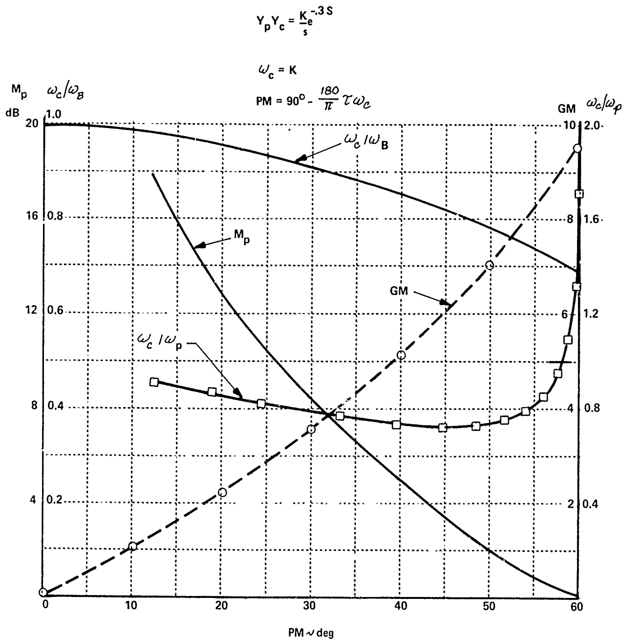
Figure 42 SYSTEM PARAMETERS FOR Y_p Y_c = \frac{K}{s} e^{-3s}
