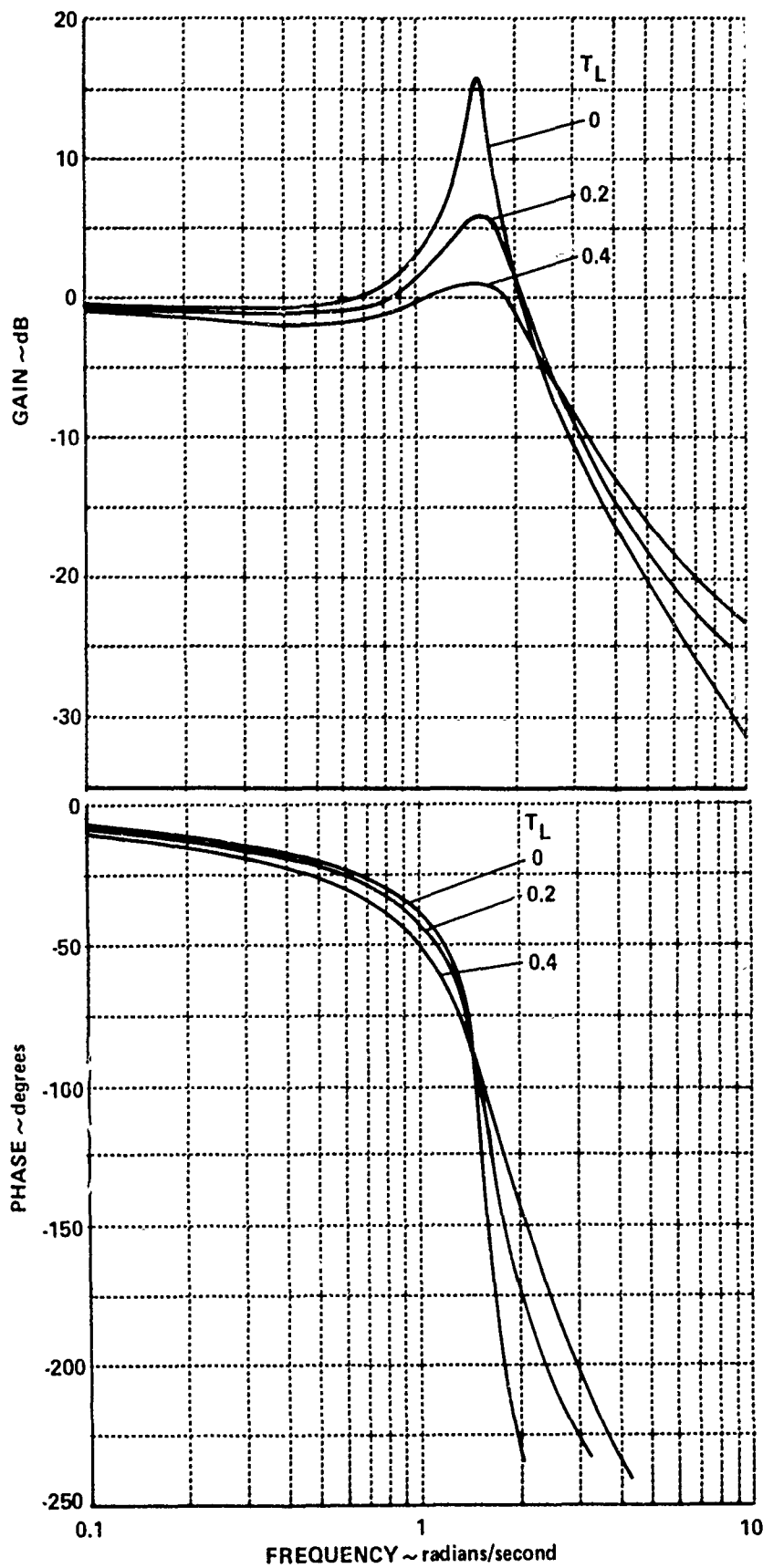
Figure 10 CLOSED-LOOP FREQUENCY RESPONSE AS A FUNCTION OF T_L FOR CONFIGURATION 6
