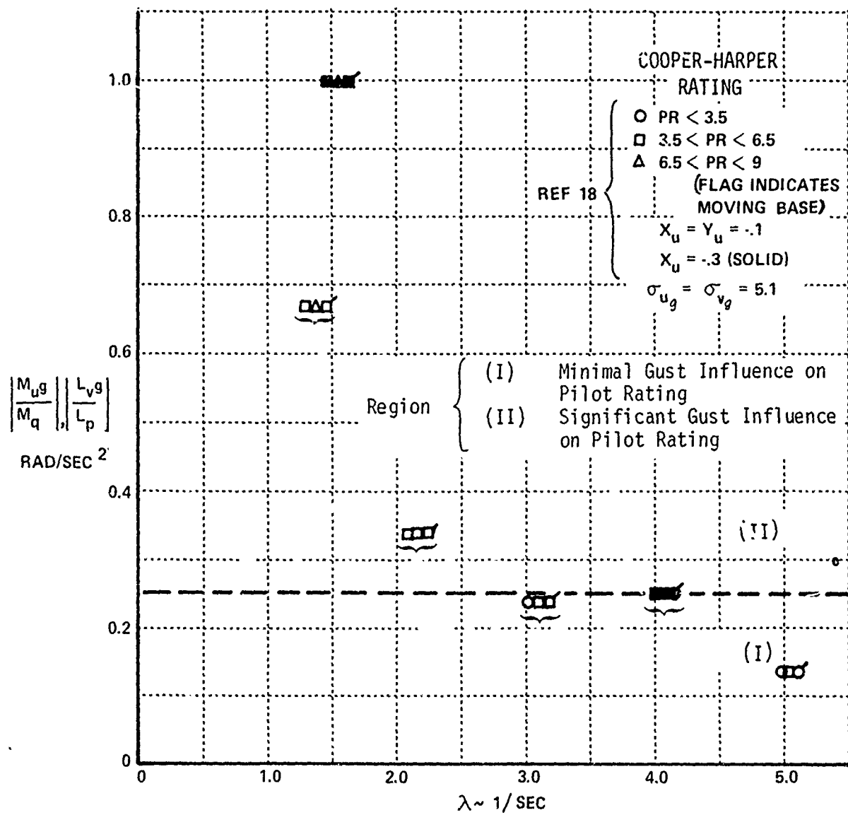
Figure 36 INFLUENCE OF GUST SENSITIVITY ON PILOT RATING
