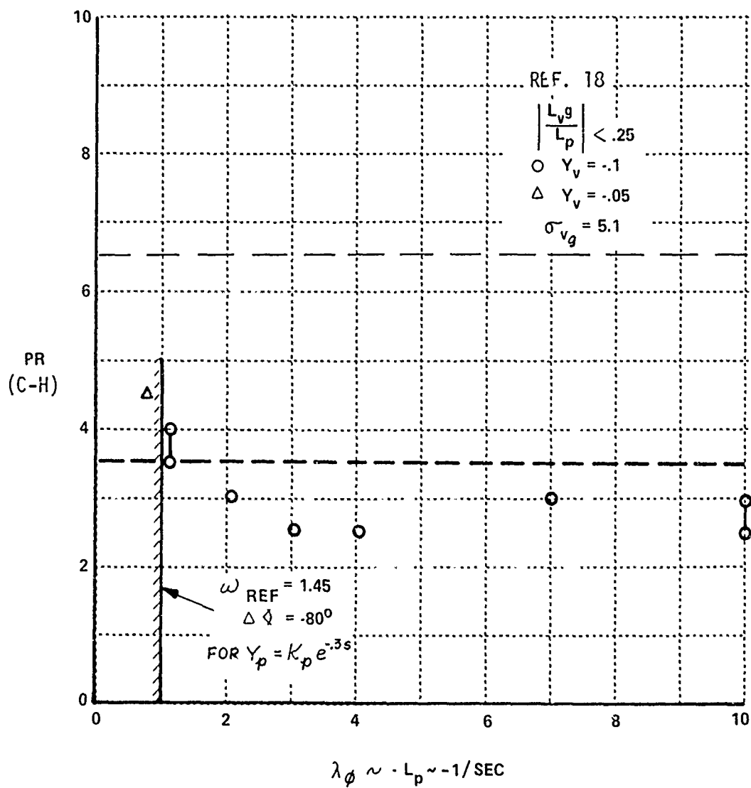
Figure 33 CORRELATION OF PILOT RATING WITH \lambda_r
