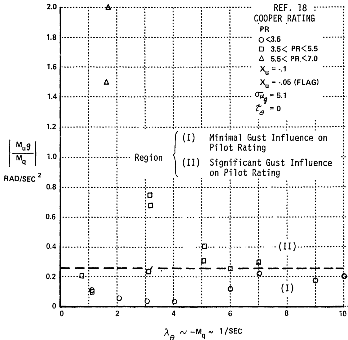
Figure 32 INFLUENCE OF GUST SENSITIVITY ON PILOT RATING (PITCH ATTITUDE CONTROL)
