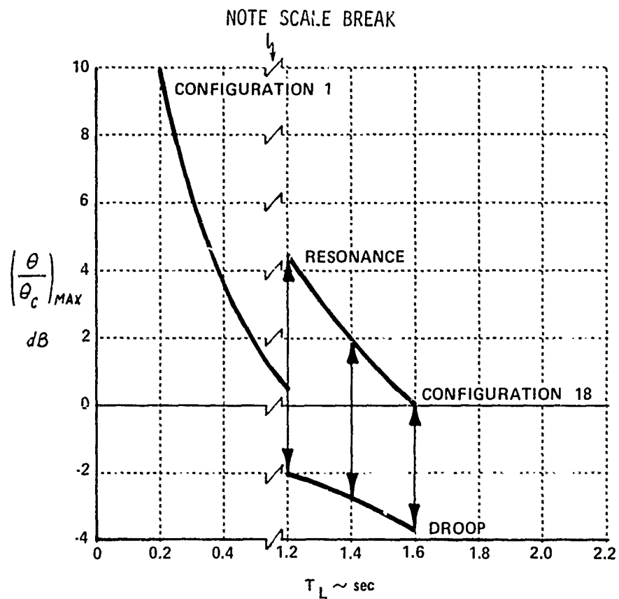
Figure 22 VARIATION IN MAXIMUM RESONANCE PEAK (\theta/\theta_c)_{MAX} WITH LEAD COMPENSATION FOR TWO VALUES OF SHORT PERIOD DAMPING
