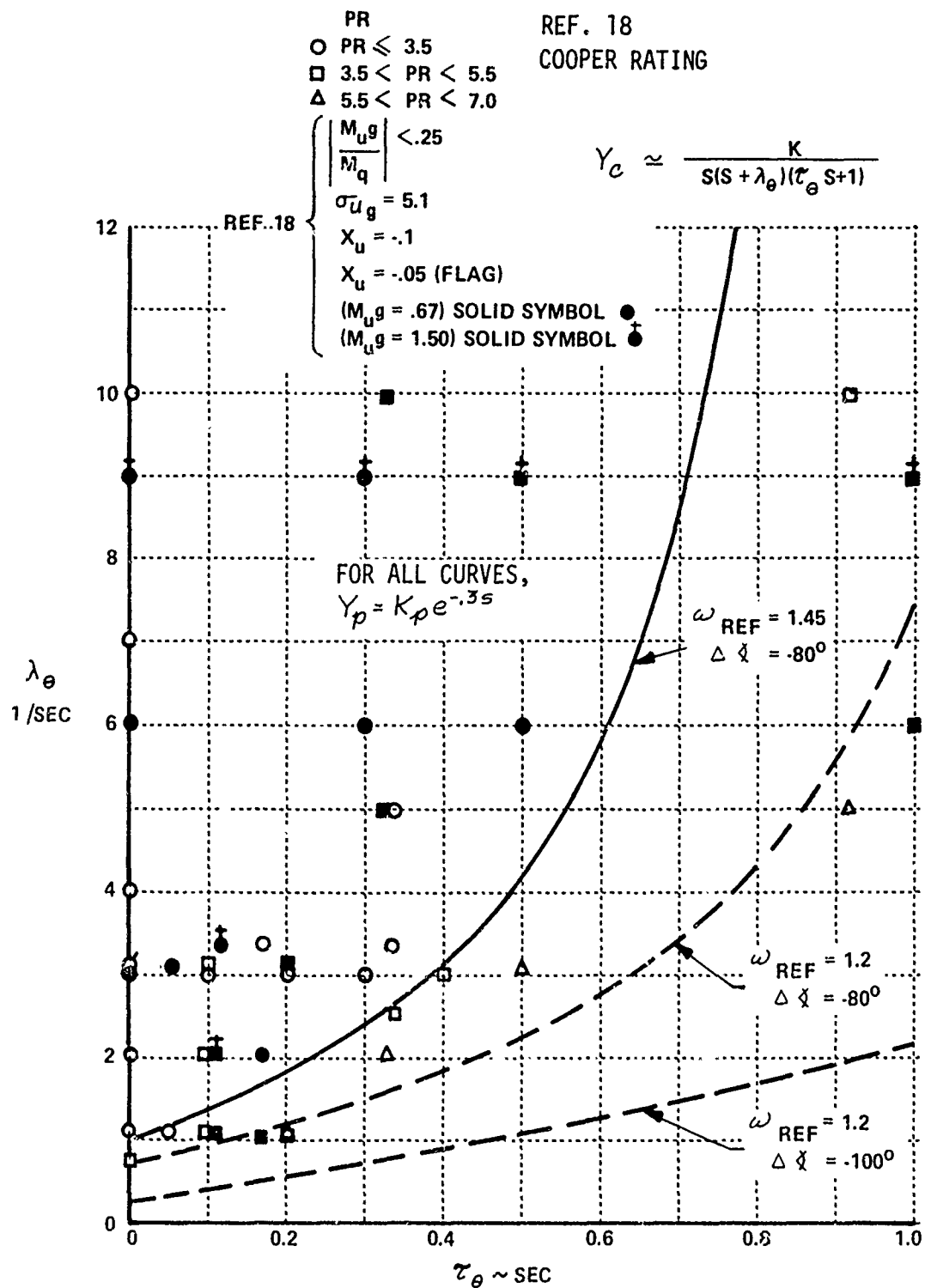
Figure 35 CORRELATION OF PILOT RATING WITH PITCH DAMPING INCLUDING A FIRST-ORDER CONTROL SYSTEM LAG
