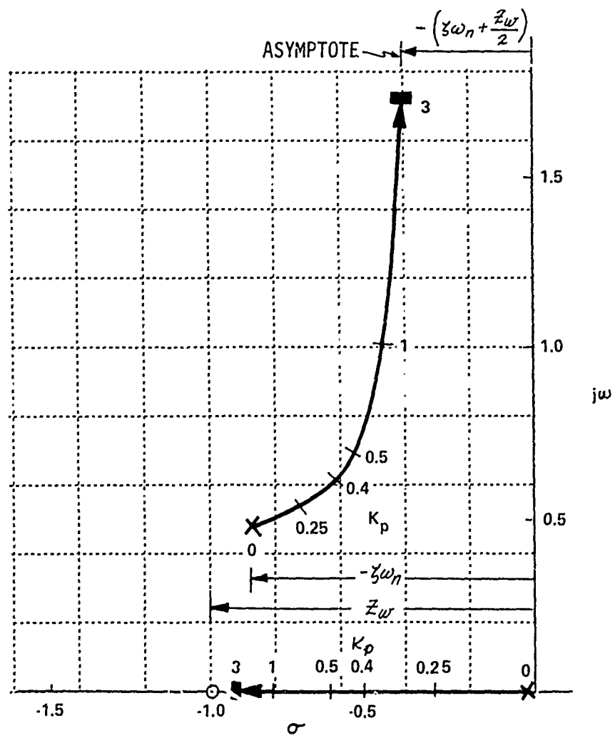
Figure 14 ROOT LOCUS FOR CONFIGURATION 10 WITH ATTITUDE FEEDBACK ONLY, T_L = \tau_e = 0
