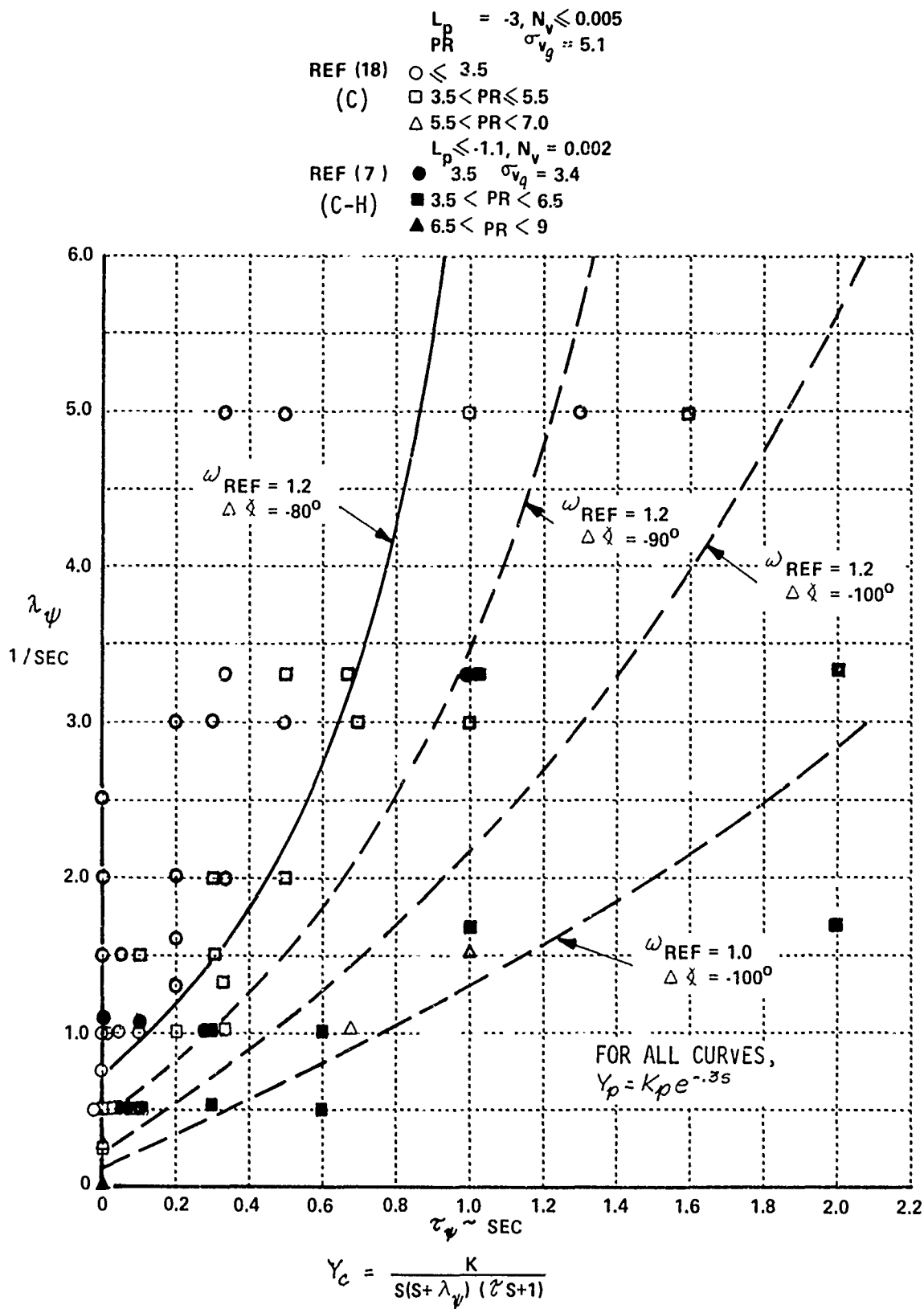
Figure 39 CORRELATION OF PILOT RATING FOR DIRECTIONAL CONTROL INCLUDING A FIRST-ORDER CONTROL SYSTEM LAG
