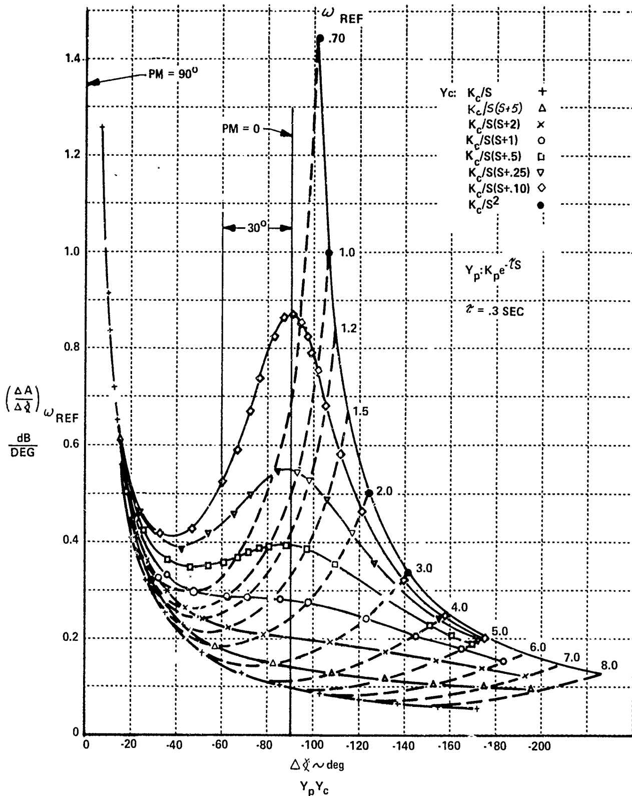
Figure 27 OPEN-LOOP PARAMETERS FOR LOW-ORDER CONTROLLED ELEMENTS
