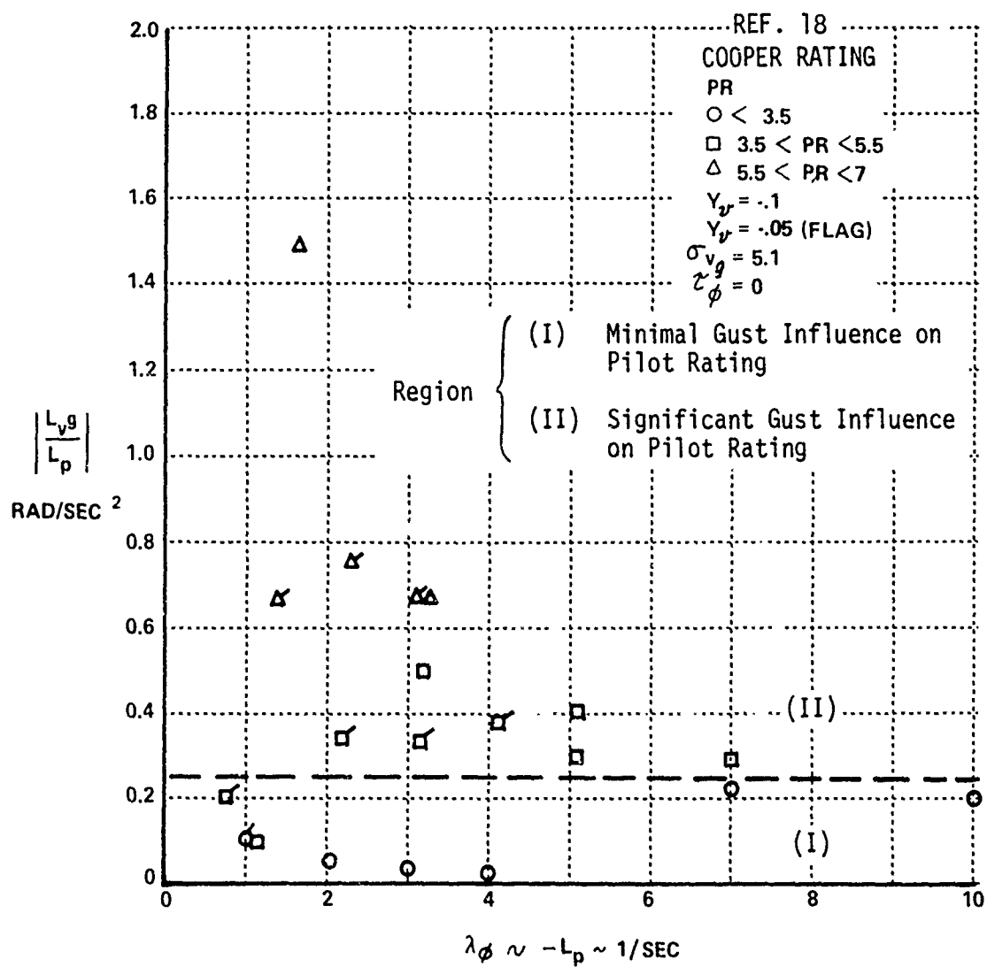
Figure 31 INFLUENCE OF GUST SENSITIVITY ON PILOT RATING (ROLL CONTROL)
