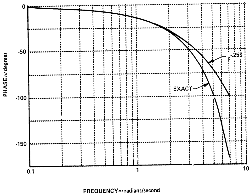
Figure 6 COMPARISON OF THE FREQUENCY RESPONSE OF COMBINED FORCE FEEL AND MODEL-FOLLOWING SYSTEM DYNAMICS WITH e^{-.25s}
