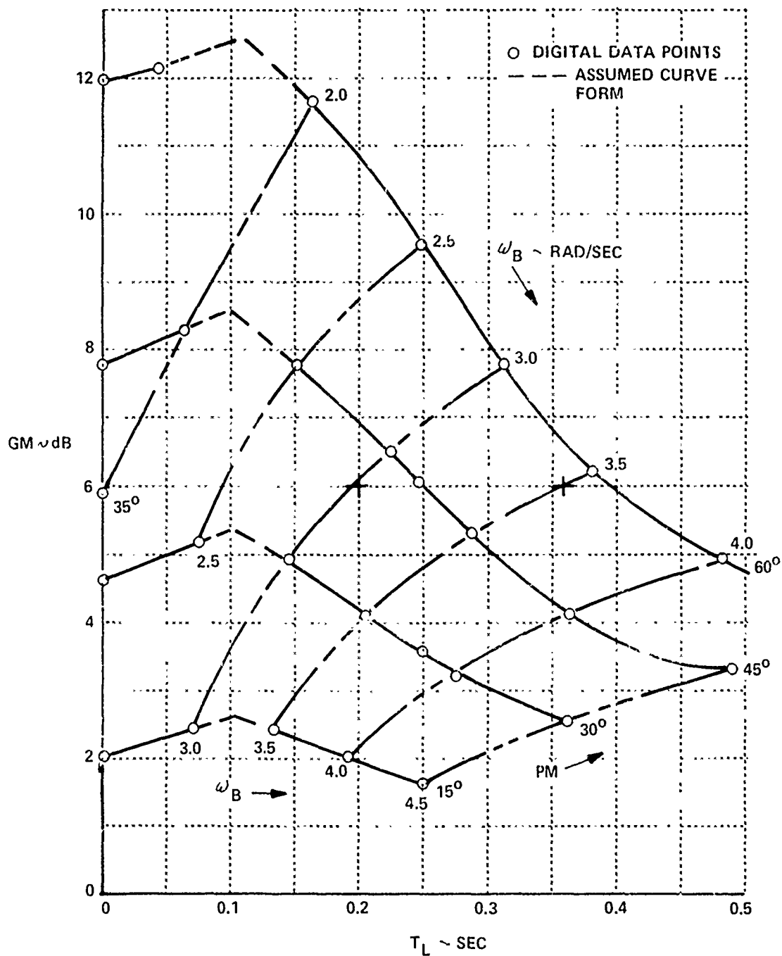
Figure 55 GAIN MARGIN FOR Y_p Y_c = \frac{K(T_L s + 1)e^{-3s}}{s(s+4)}
