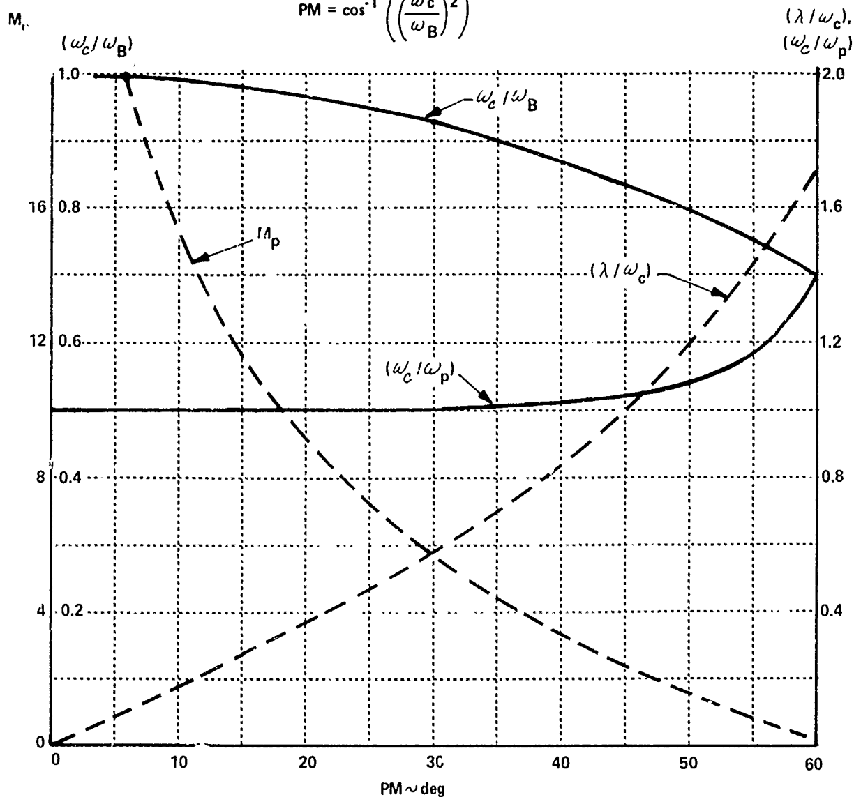
Figure 43 SYSTEM PARAMETERS FOR Y_p Y_c = \frac{K}{s(s+\lambda)}
