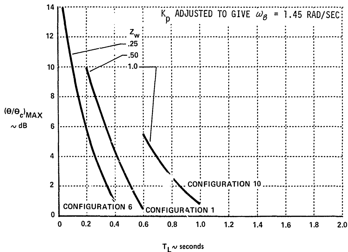
Figure 13 VARIATION IN MAXIMUM RESONANCE PEAK (\theta/\theta_c)_{MAX} WITH LEAD COMPENSATION T_L AND Z_w
