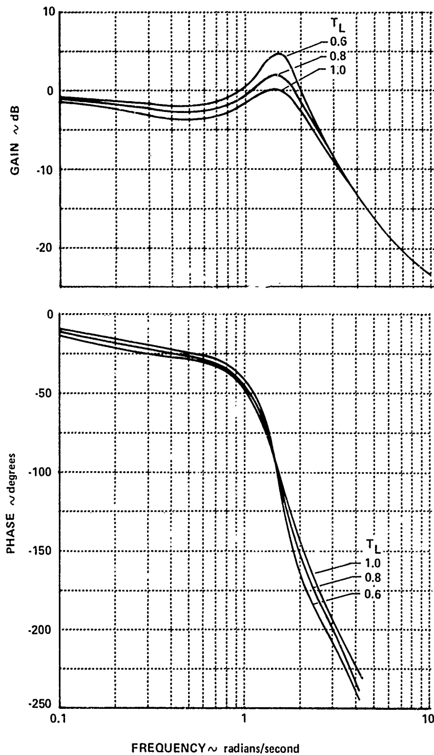
Figure 21 CLOSED-LOOP FREQUENCY RESPONSE AS A FUNCTION OF T_L FOR CONFIGURATION 18
