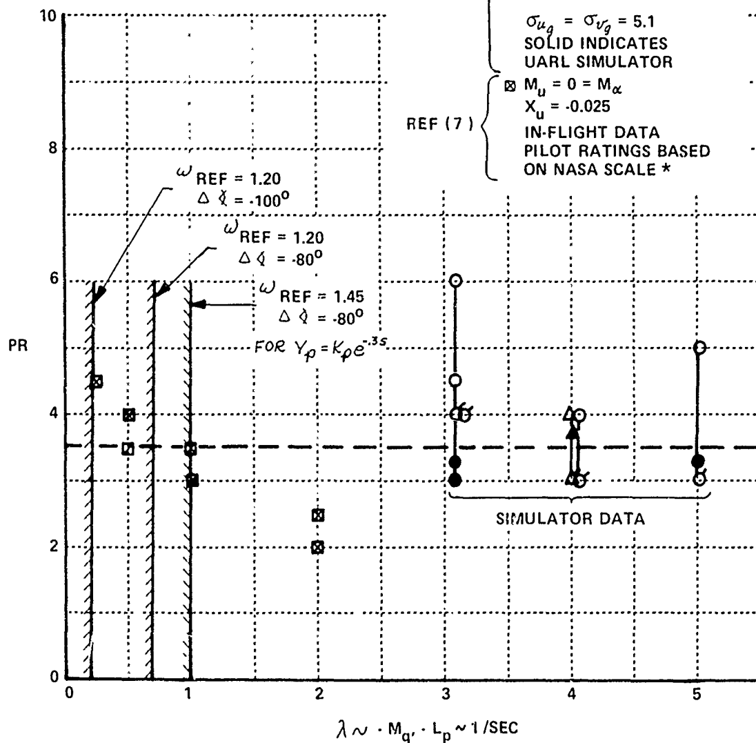
Figure 37 CORRELATION OF PILOT RATING (ATTITUDE CONTROL)
