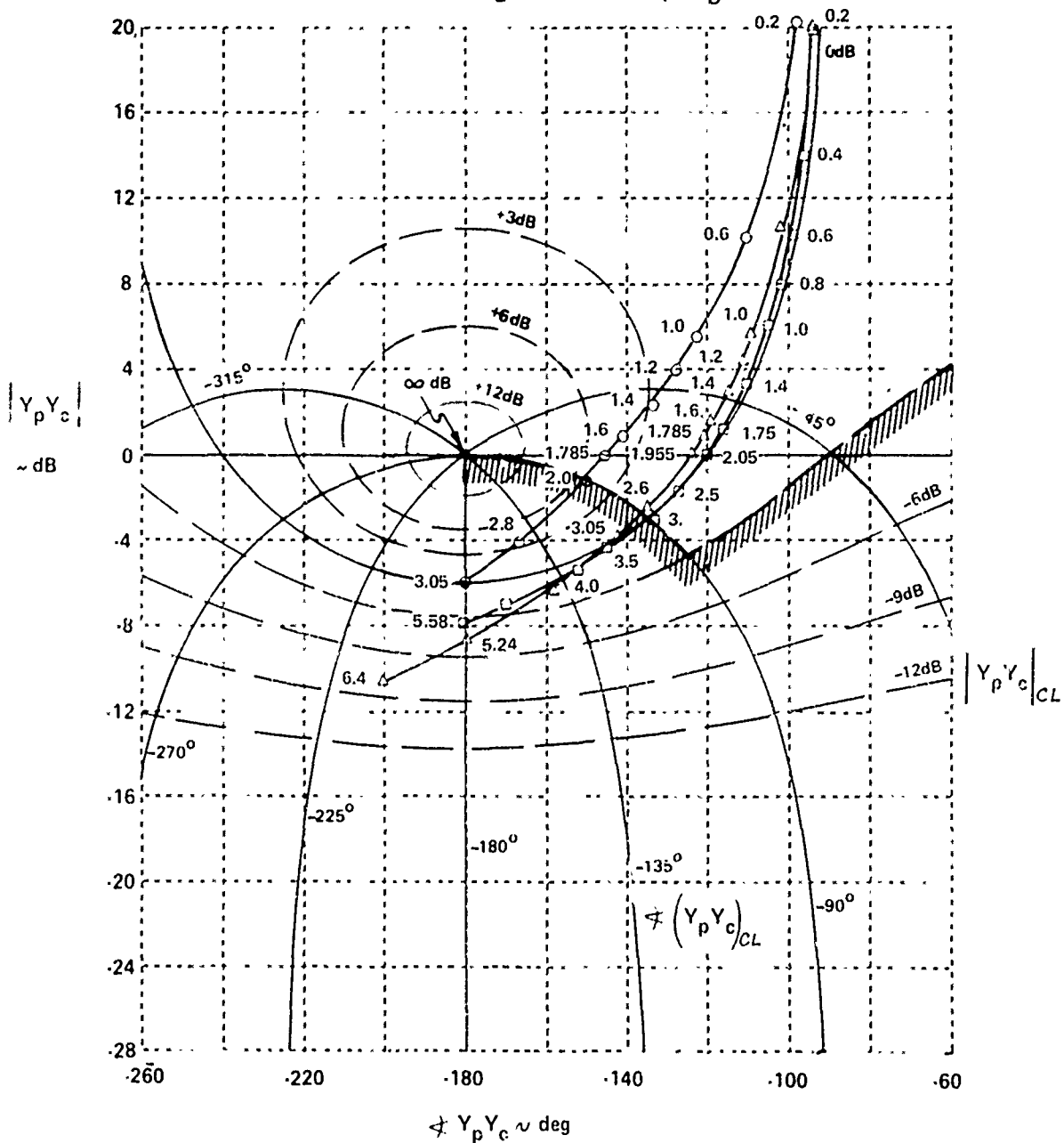
Figure 54 EFFECT OF LEAD EQUALIZATION AT ESSENTIALLY CONSTANT SYSTEM GAIN
