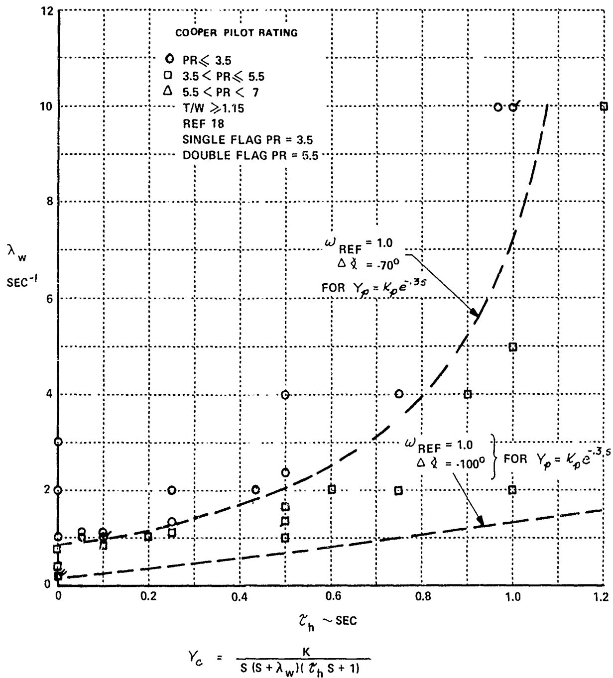
Figure 29 CORRELATION OF PILOT RATING WITH VERTICAL DAMPING INCLUDING A FIRST-ORDER CONTROL SYSTEM LAG, T/W \geq 1.15
