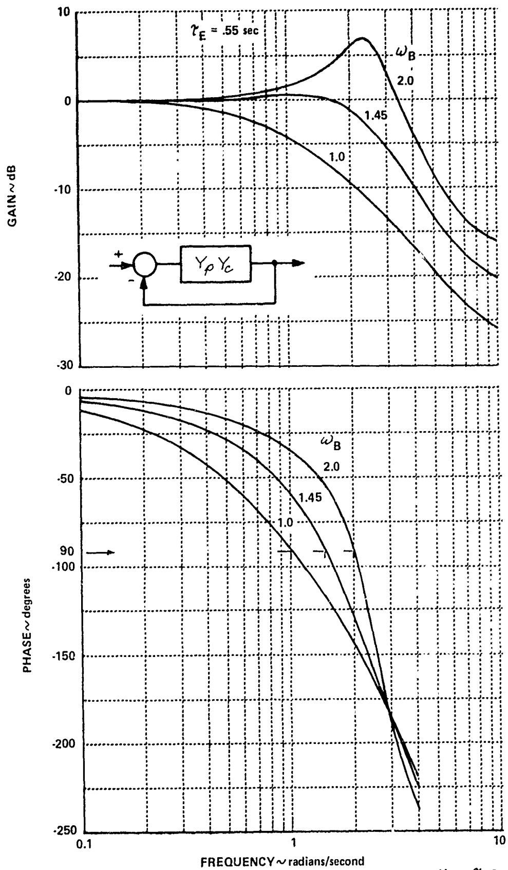
Figure 8 CLOSED-LOOP FREQUENCY RESPONSE FOR Y_p Y_c = \frac{K}{S} e^{-\tau_E S}
