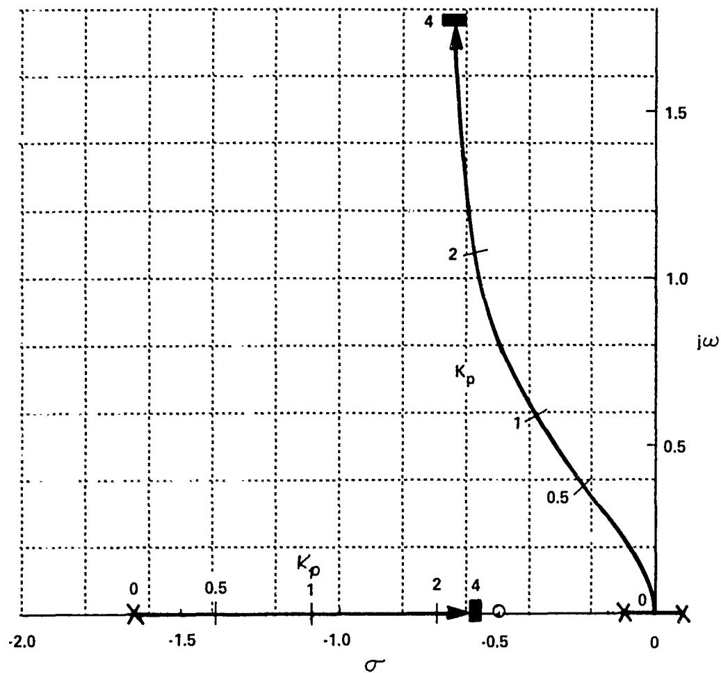
Figure 20 ROOT LOCUS FOR CONFIGURATION 5 WITH ATTITUDE FEEDBACK ONLY, T_L = \tau_e = 0
