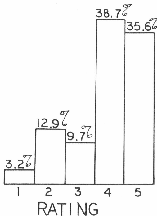
Figure 4: Percentage of castings in each group, grouped by fraction solid of the casting material, given a particular overall quality rating.
