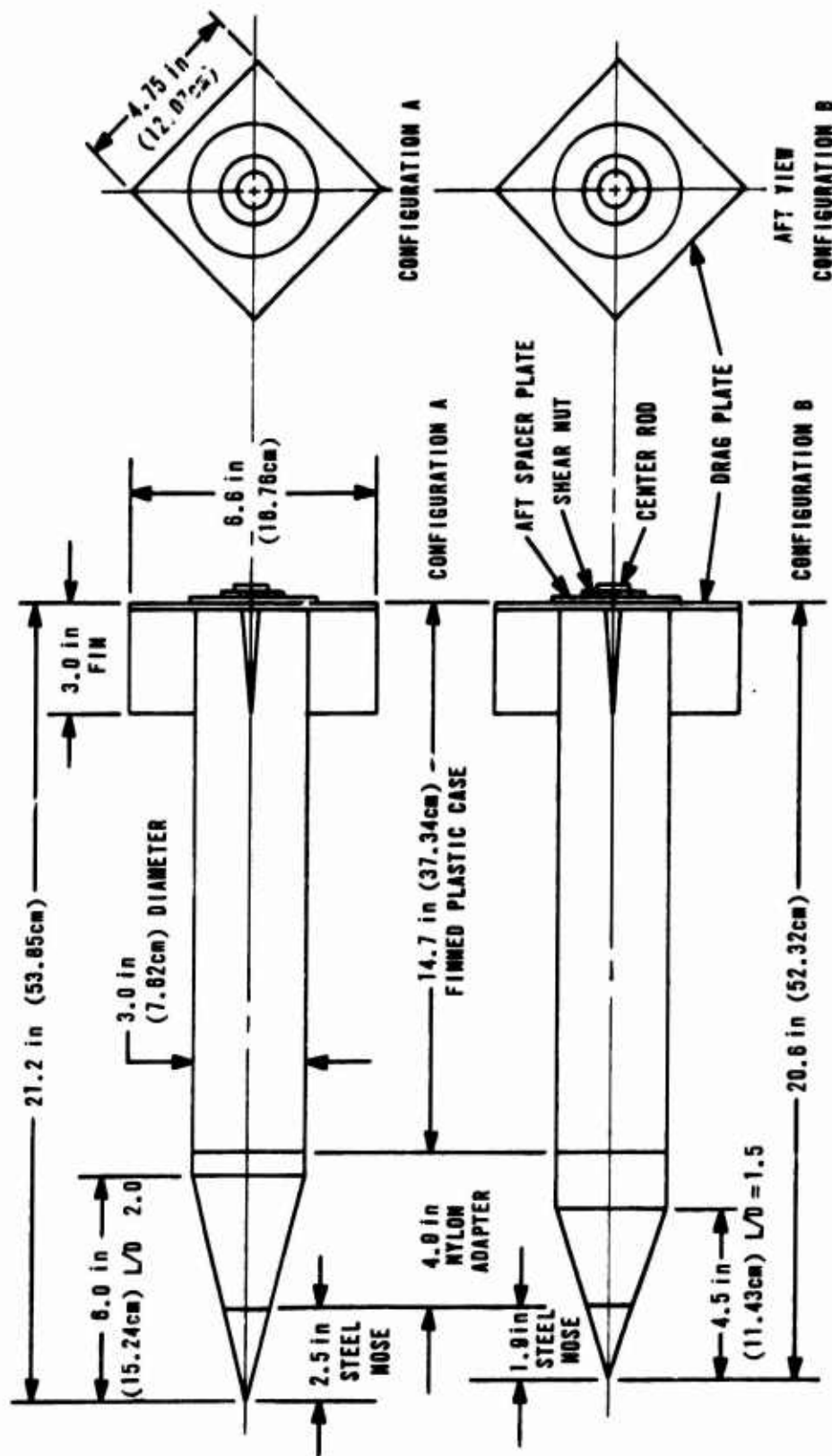
Figure 4. Basic Penetrorometer Designs
