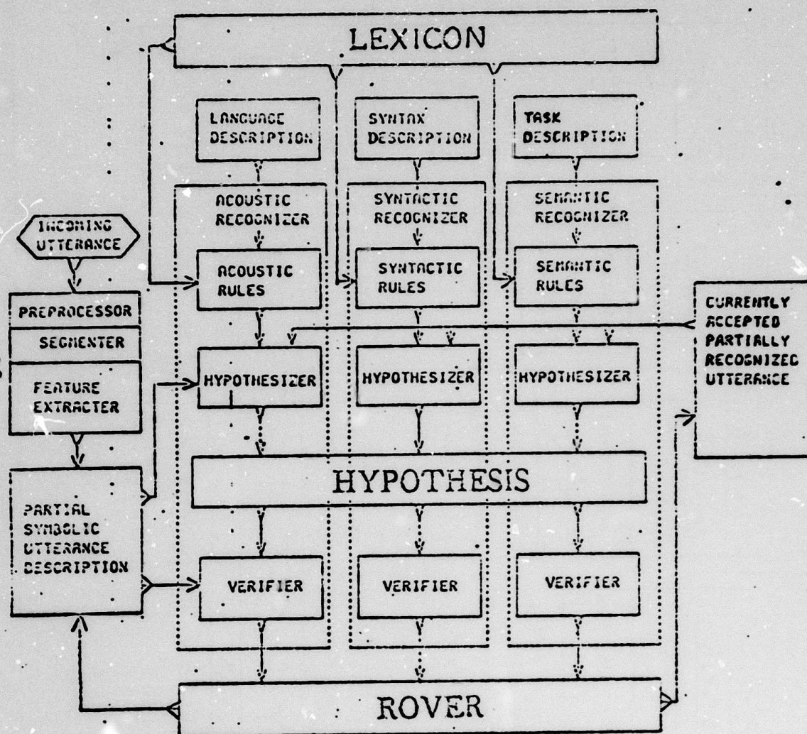
Fig. 1. Detail of the Recognition Process in the CMU-HEARSAY1 System
