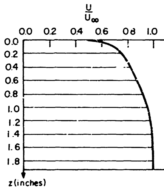
BOUNDARY LAYER AT RUDDER POSITION (DOWNSTREAM)
