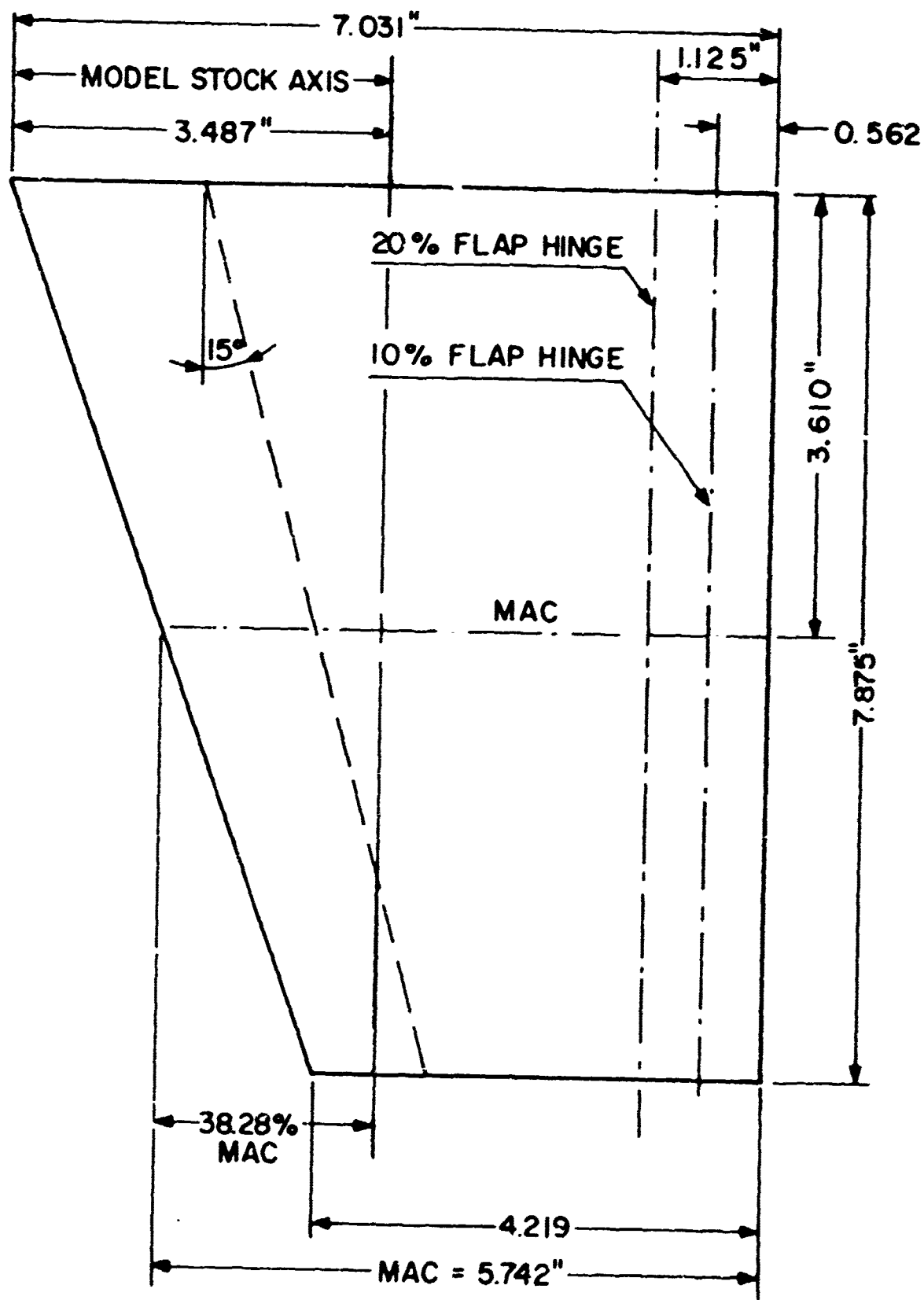
Figure 1 Planform of the 10% and 20% Flap Rudders.
