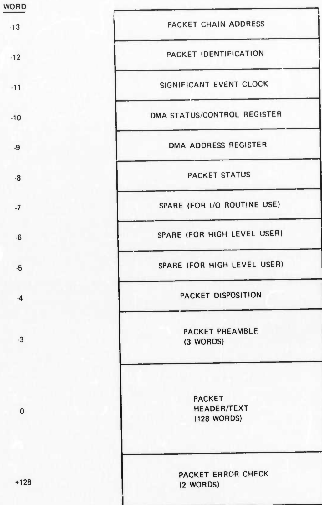
Figure 2-4. Packet Buffer Format.
