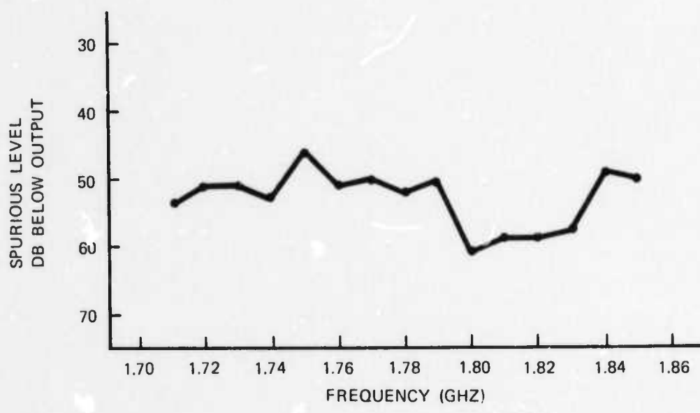
Figure 3-3. Transmit Chain Performance.
