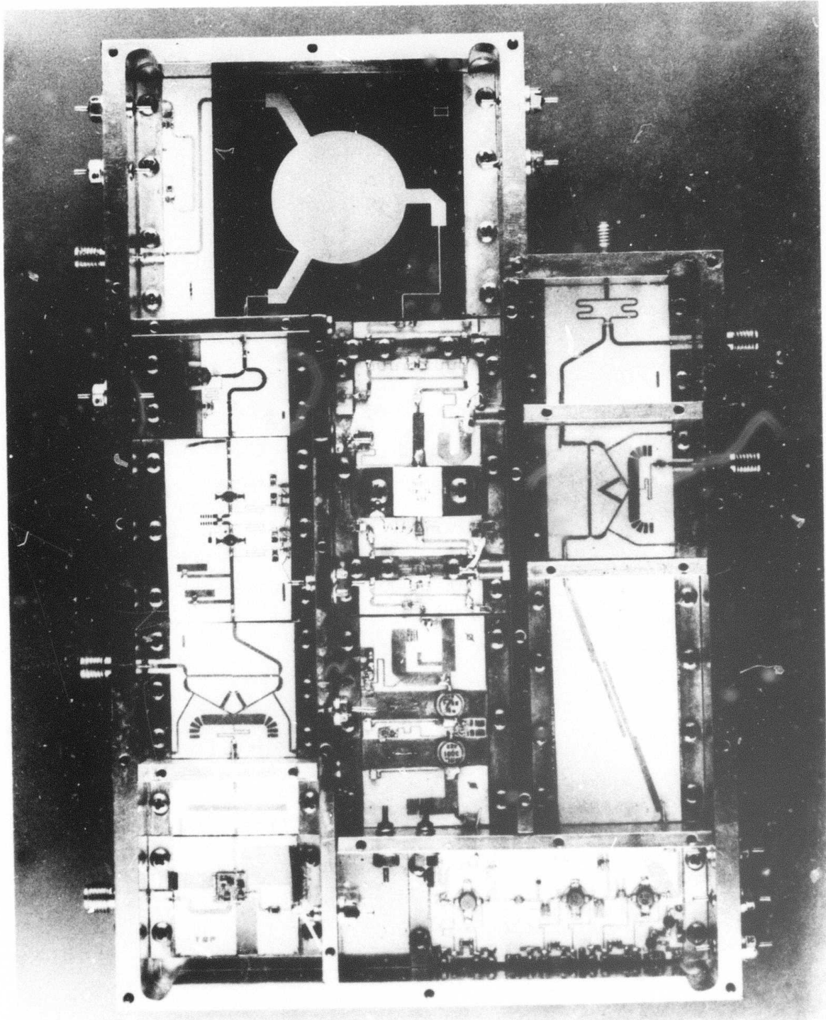
Figure 3-1. RF Head.
